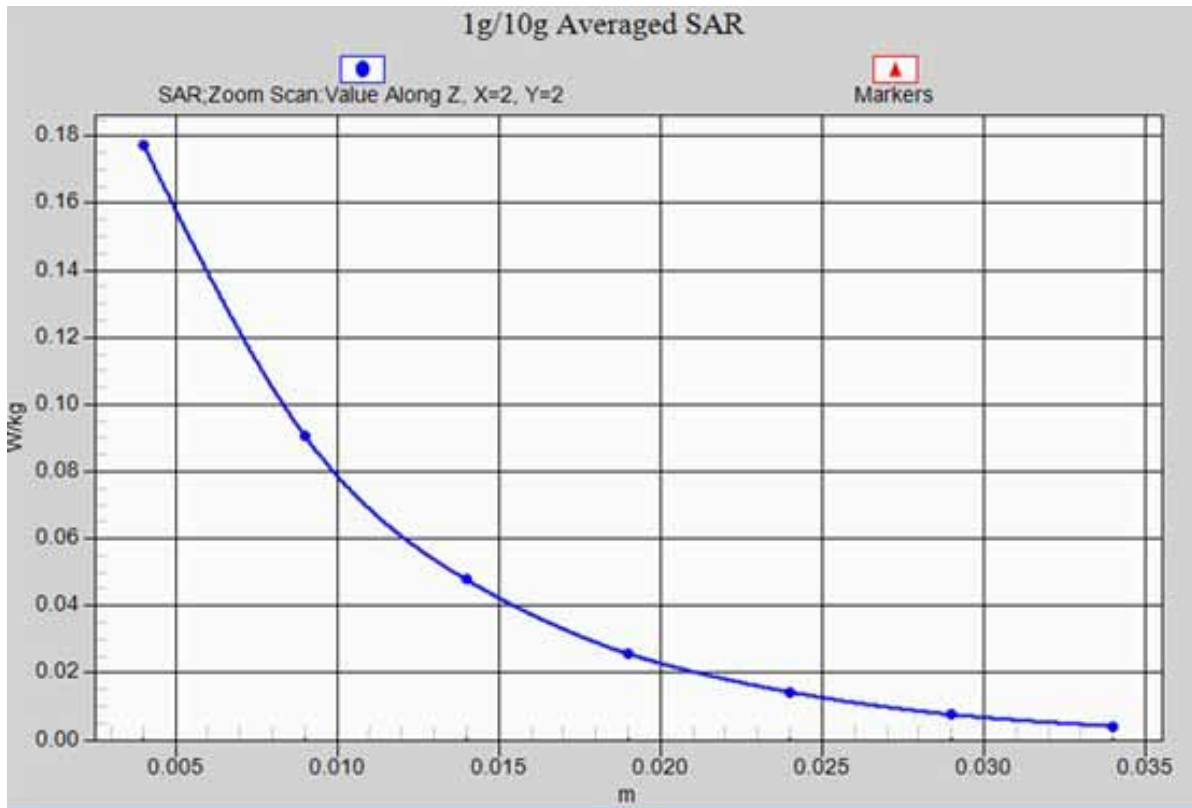
GSM1900 Back side-Mid with headset_ z-axis scan
