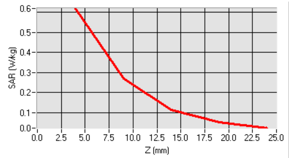
SAR, Z Axis Scan (X = -19, Y = -5)
