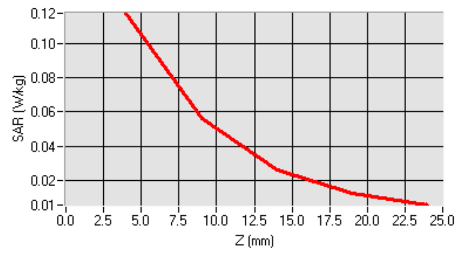
SAR, Z Axis Scan (X = 8, Y = -29)
