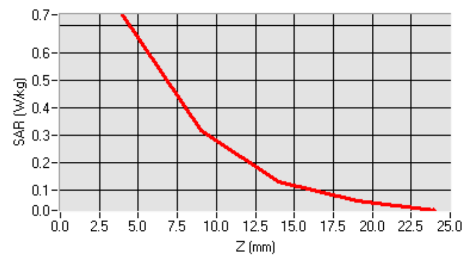
SAR, Z Axis Scan (X = -17, Y = 0)
