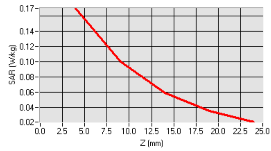
SAR, Z Axis Scan (X = 16, Y = -33)
