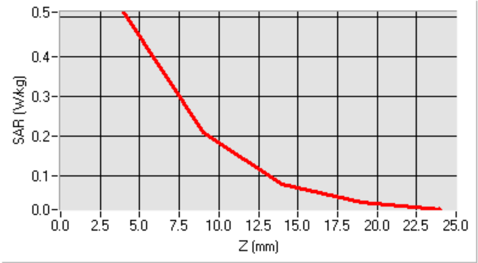
SAR, Z Axis Scan (X = -11, Y = -6)
