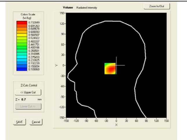
SAR, Z Axis Scan (X = -15, Y = -9)
