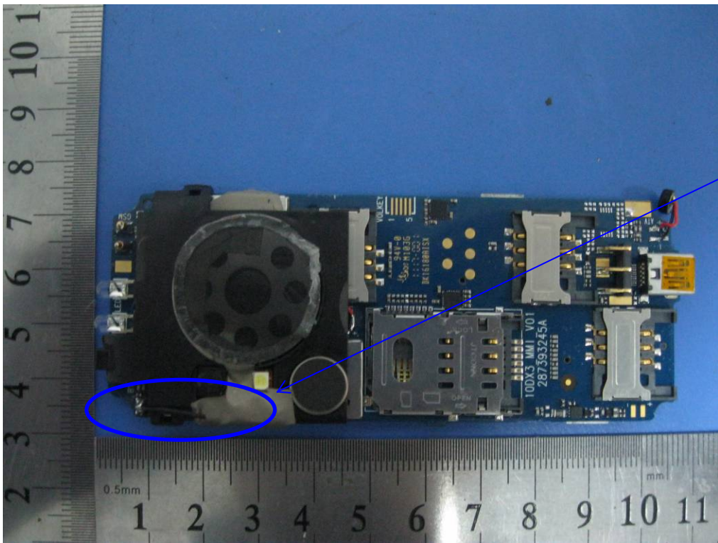
BT Antenna - Top View
