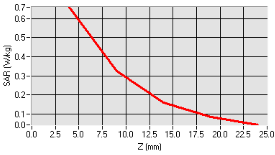
SAR, Z Axis Scan (X = -65, Y = -25)
