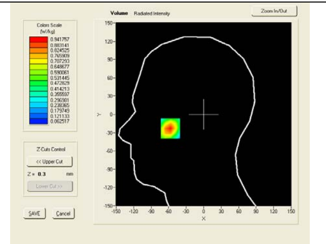
SAR, Z Axis Scan (X = -57, Y = -23)
