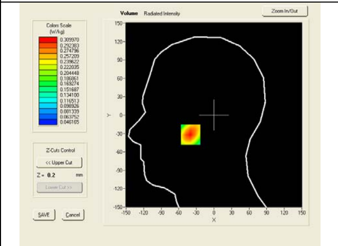
SAR, Z Axis Scan (X = -40, Y = -32)
