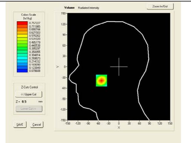
SAR, Z Axis Scan (X = -51, Y = -39)
