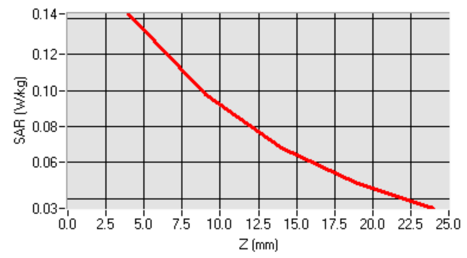
SAR, Z Axis Scan (X = 14, Y = -38)
