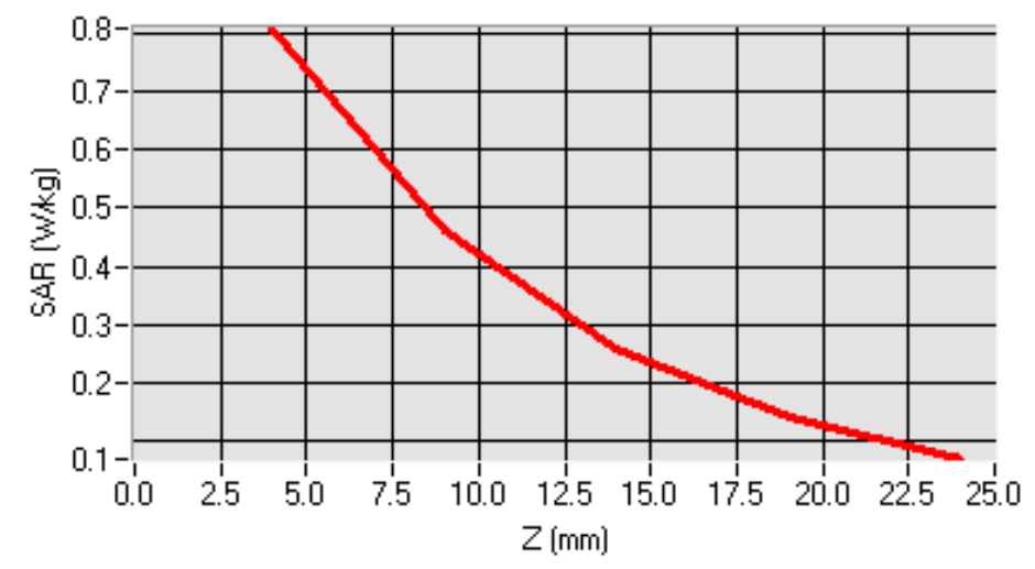
SAR, Z Axis Scan (X = -61, Y = -46)
