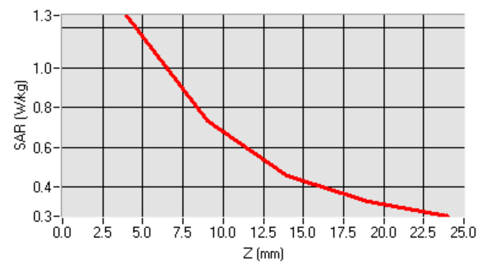
SAR, Z Axis Scan (X = -48, Y = -46)
