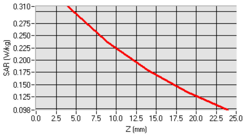
SAR, Z Axis Scan (X = -40, Y = -32)
