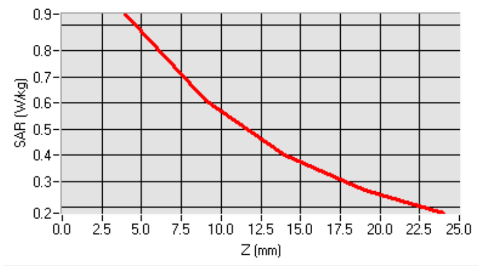
SAR, Z Axis Scan (X = -57, Y = -23)
