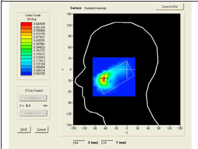
SAR, Z Axis Scan (X = -65, Y = -25)
