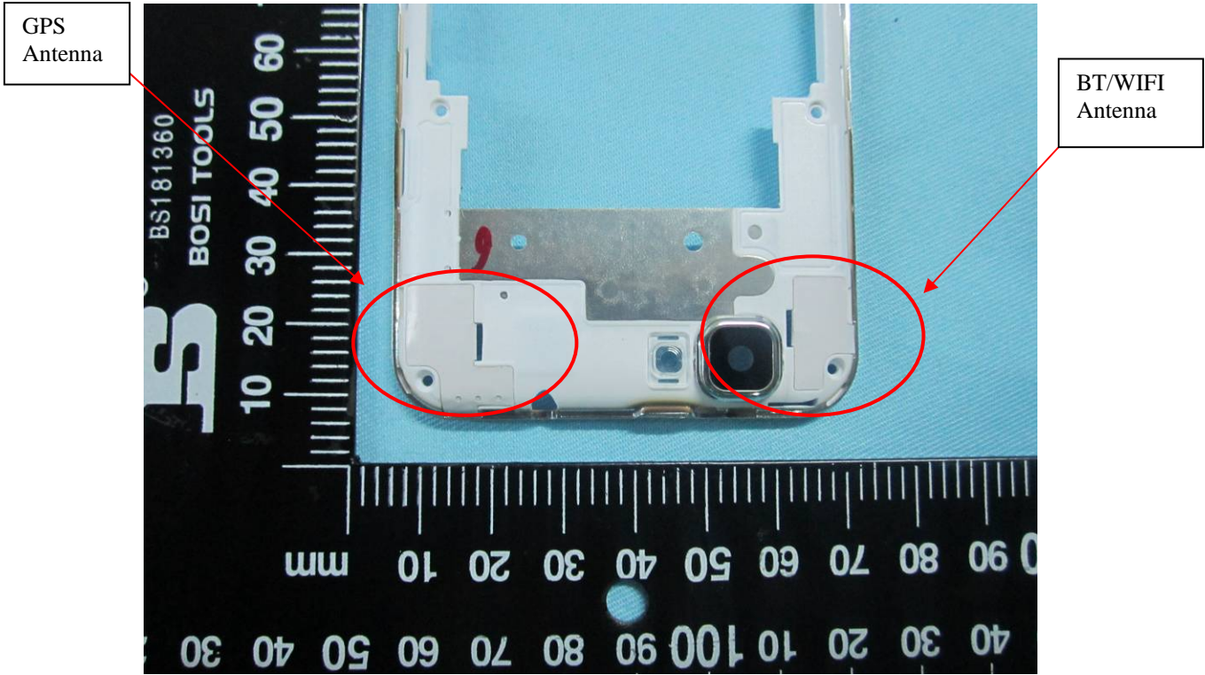
GPS/BT/WIFI Antenna View
