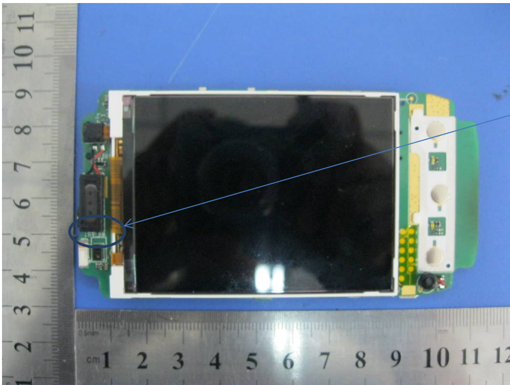
BT/Wifi Antenna - Top View
