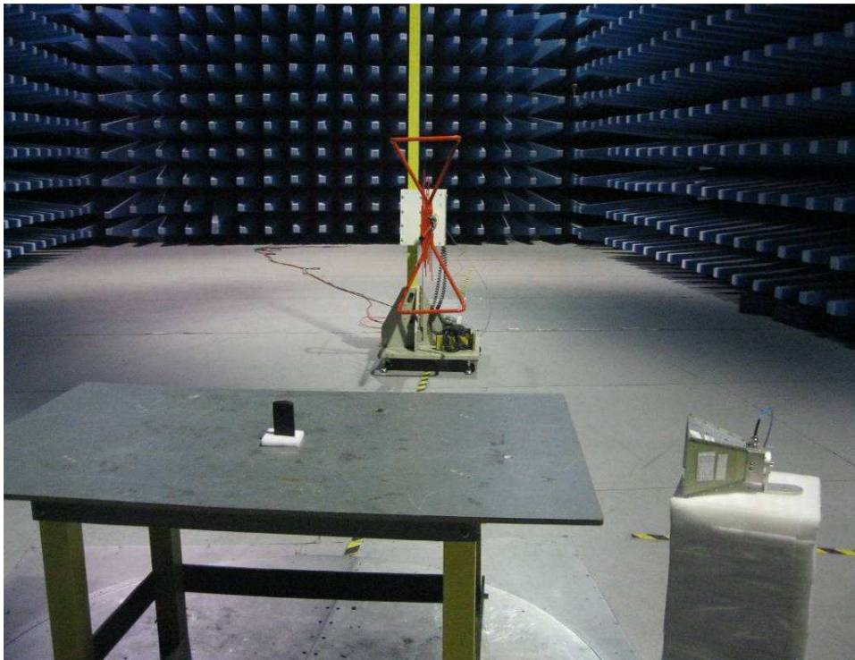
Below 1GHz: Radiated Emissions - Rear View
