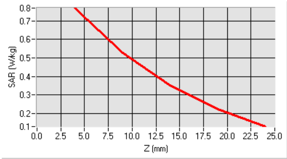
SAR, Z Axis Scan (X = 3, Y = 2)
