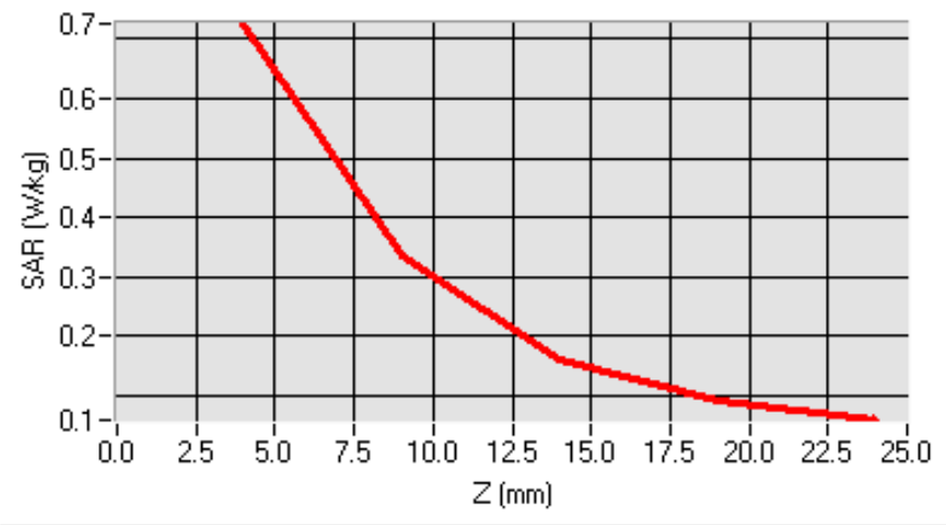
SAR, Z Axis Scan (X = 11, Y = -25)
