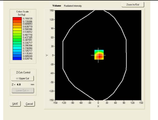
SAR, Z Axis Scan (X = 3, Y = 2)
