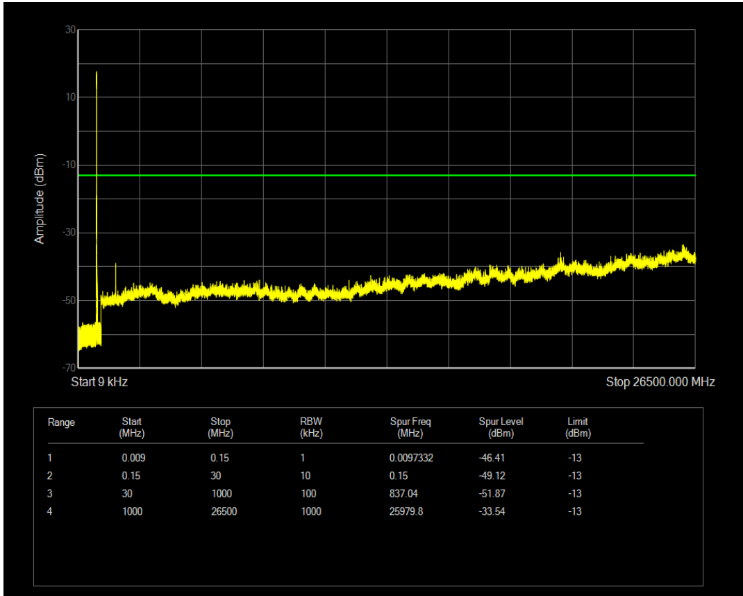
Band26a 16QAM BW=3MHz Channel=26705 RB Size=1 Position=#0
