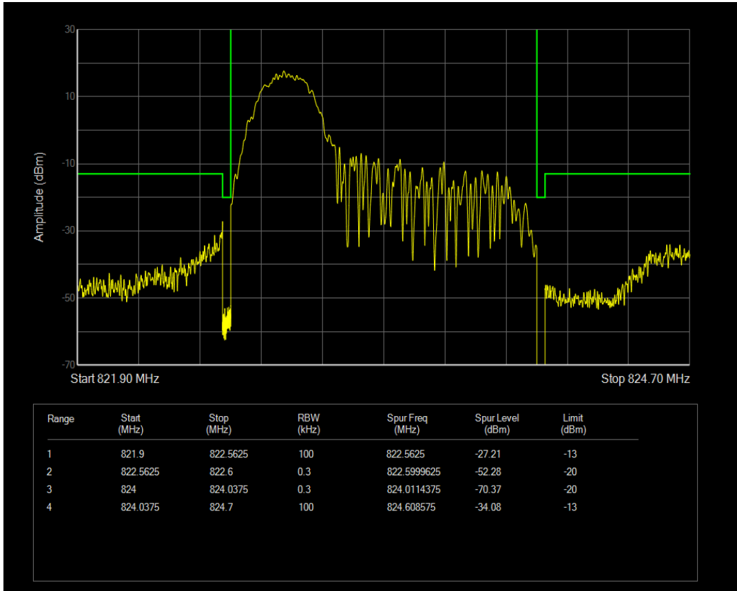
Band26a 16QAM BW=1.4MHz Channel=26783 RB Size=1 Position=#Max
