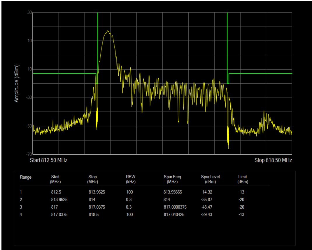
Band26a 16QAM BW=3MHz Channel=26705 RB Size=1 Position=#Max
