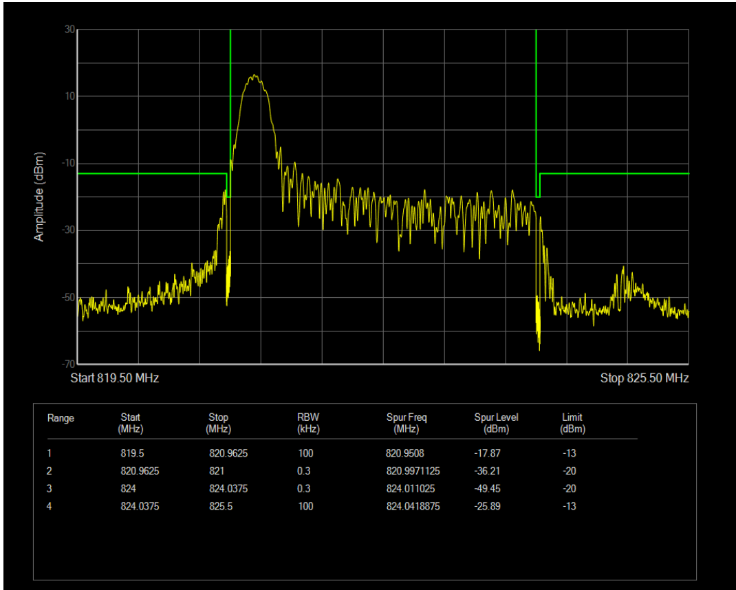
Band26a 16QAM BW=3MHz Channel=26775 RB Size=1 Position=#Max
