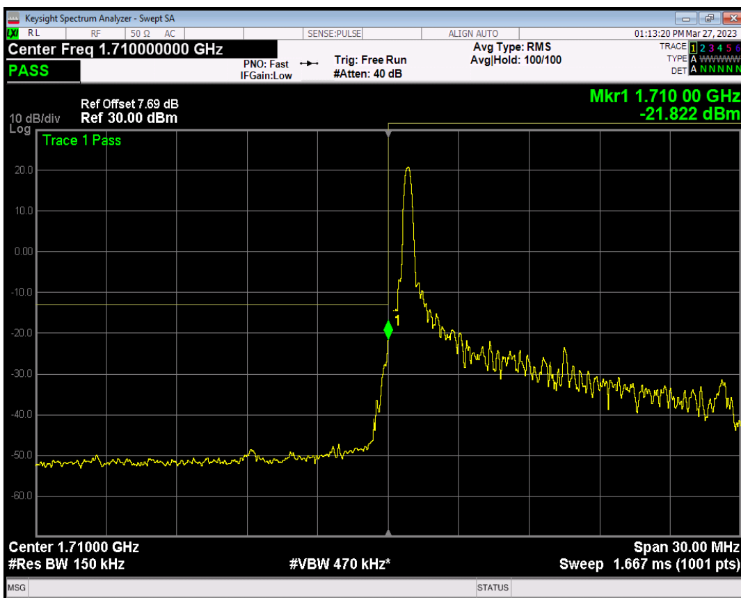
Band66 QAM16 BW=15MHz Channel=132047 RB Size=1 Position=#Max
