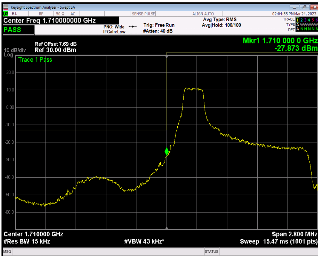
Band66 QAM16 BW=1.4MHz Channel=131979 RB Size=1 Position=#Max
