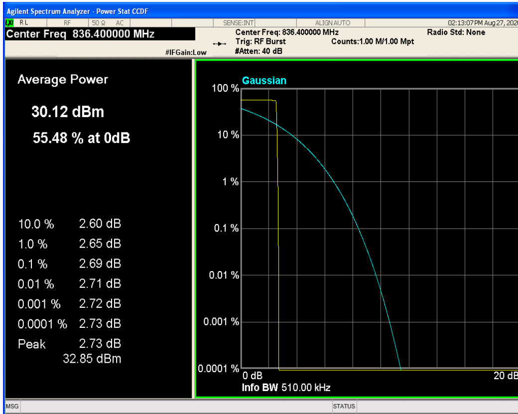
GSM850 Channel=189
