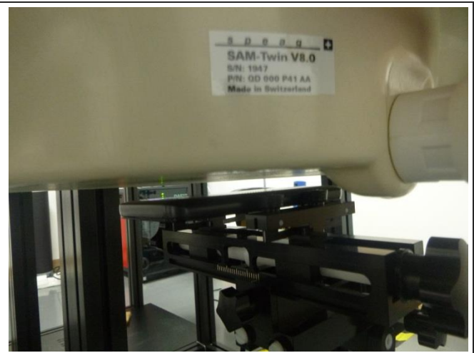
Body-worn Rear(10mm)
