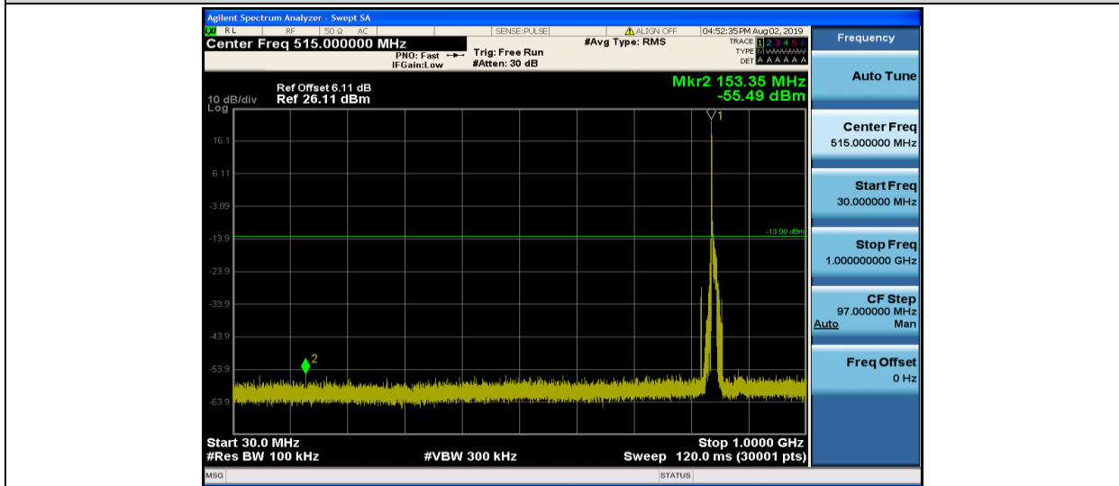
Band5-10MHz-QPSK-20600-1RB#0-30~1000MHz
