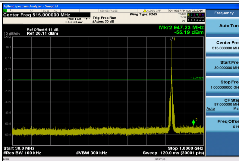
Band5-5MHz-QPSK-20525-1RB#0-30~1000MHz
