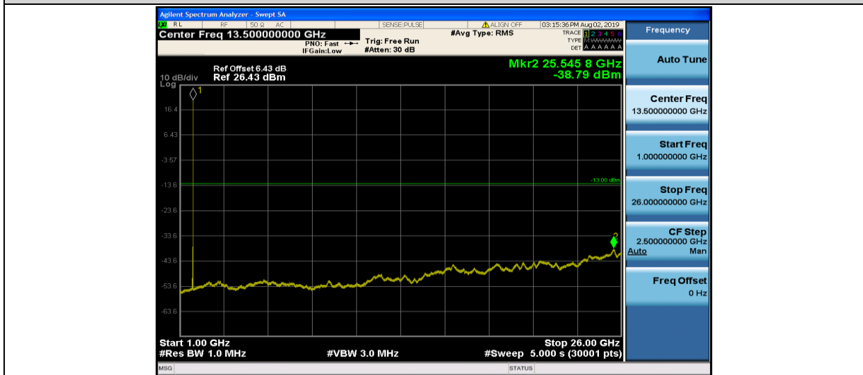
Band4-3MHz-QPSK-20385-1RB#0-1000~26000MHz
