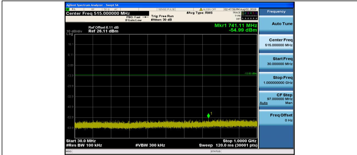
Band2-15MHz-16QAM-18675-1RB#0-30~1000MHz
