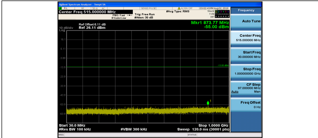
Band4-1.4MHz-QPSK-19957-1RB#0-30~1000MHz
