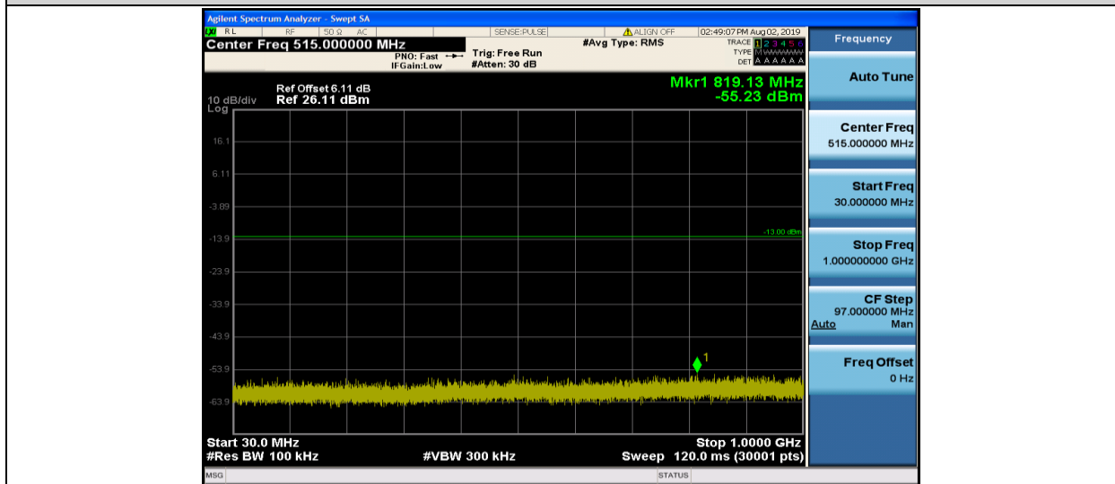
Band2-15MHz-16QAM-18900-1RB#0-30~1000MHz
