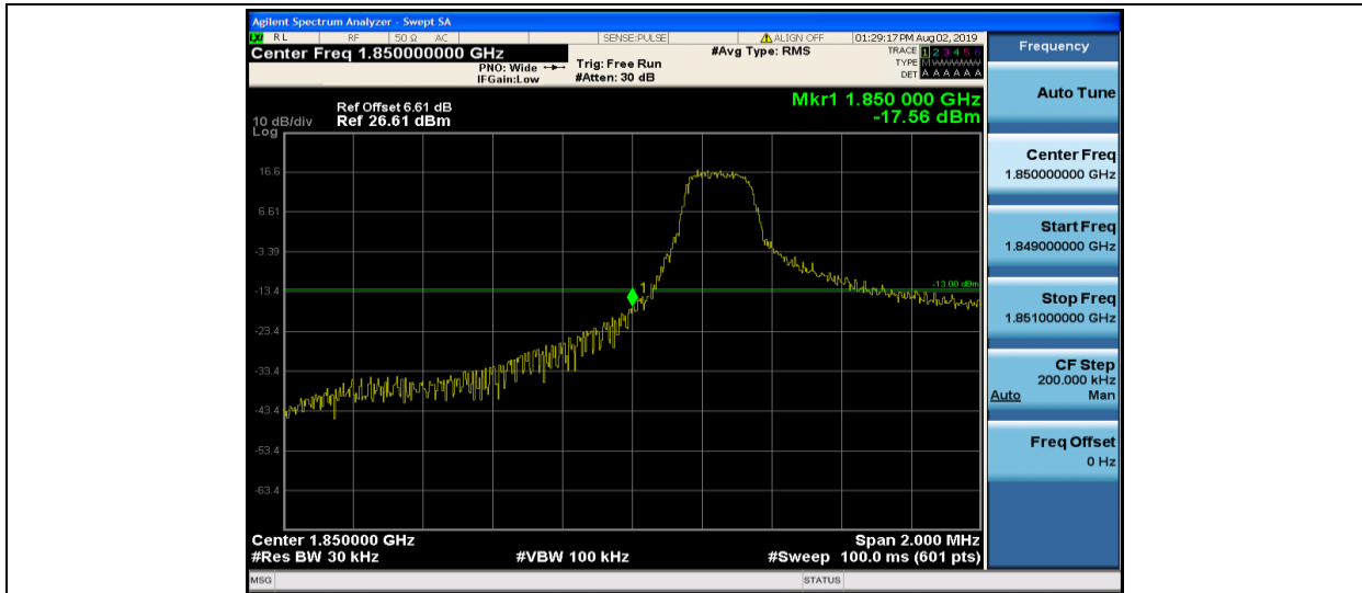
Band2-1.4MHz-QPSK-18607-1RB#0
