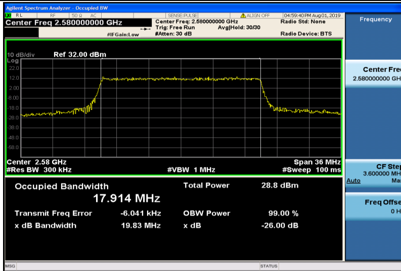
Band38-20MHz-16QAM-37850-100RB#0-17.914
