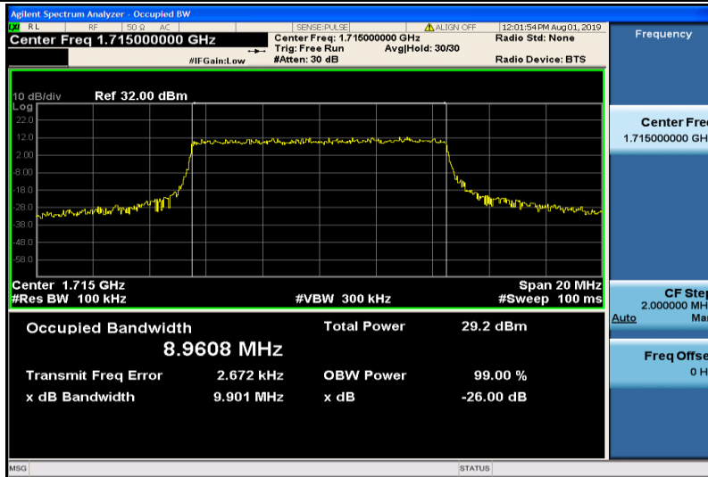
Band4-10MHz-QPSK-20000-50RB#0-8.9608
