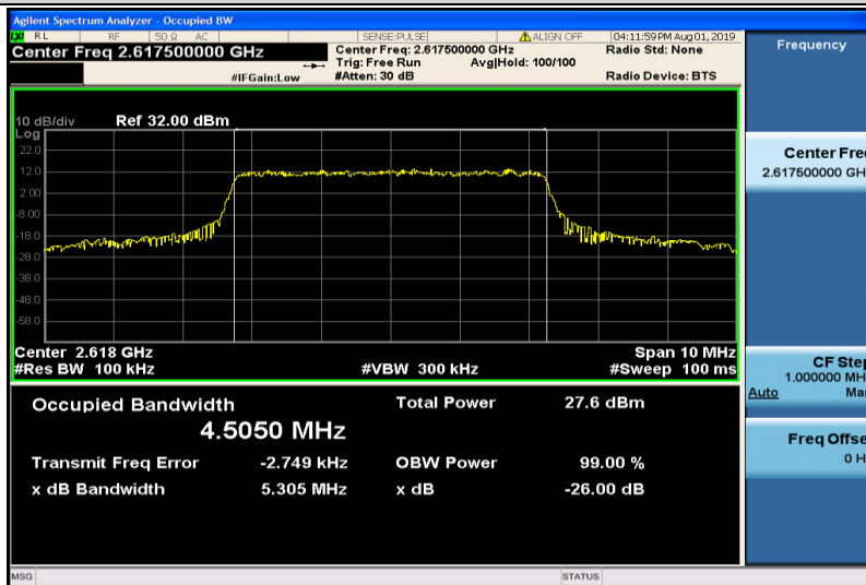
Band38-5MHz-16QAM-38225-25RB#0-4.5050
