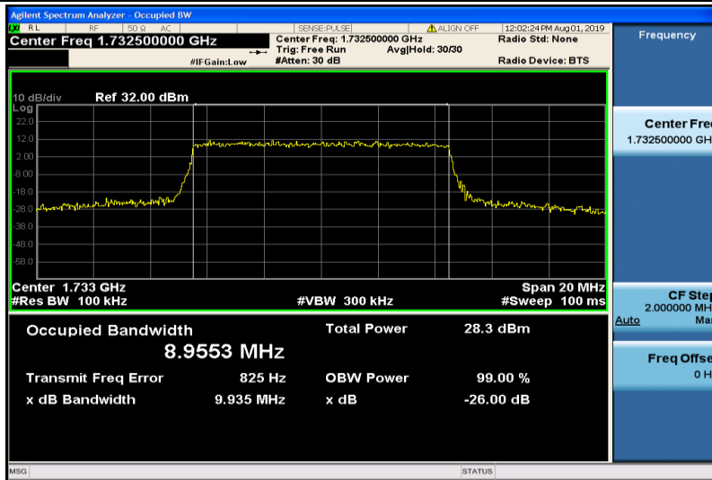
Band4-10MHz-16QAM-20175-50RB#0-8.9553
