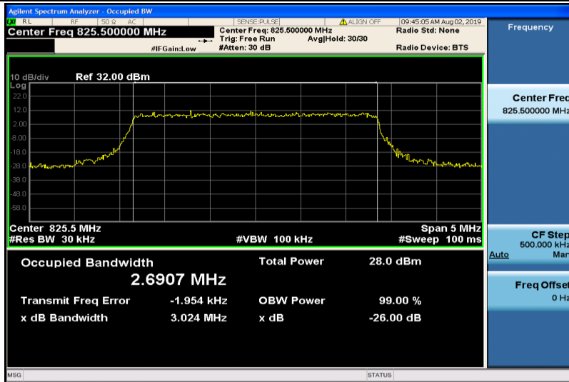
Band5-3MHz-16QAM-20415-15RB#0-2.6907
