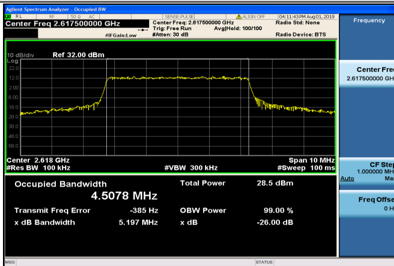
Band38-5MHz-QPSK-38225-25RB#0-4.5078
