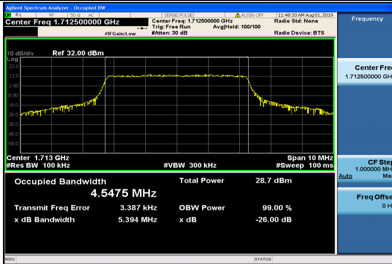
Band4-5MHz-16QAM-19975-25RB#0-4.5475
