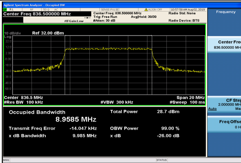
Band5-10MHz-16QAM-20525-50RB#0-8.9585
