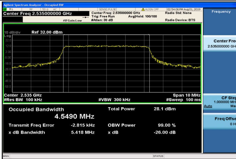
Band7-5MHz-16QAM-21100-25RB#0-4.5490
