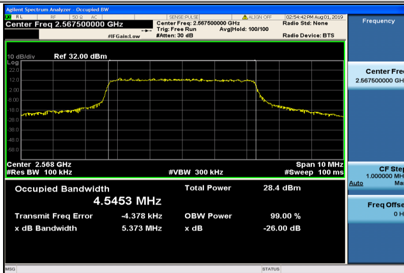
Band7-5MHz-16QAM-21425-25RB#0-4.5453
