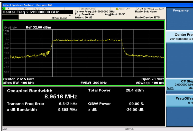
Band38-10MHz-QPSK-38200-50RB#0-8.9516
