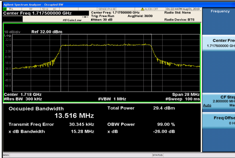
Band4-15MHz-QPSK-20025-75RB#0-13.516
