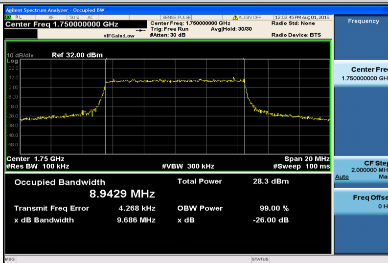
Band4-10MHz-16QAM-20350-50RB#0-8.9429
