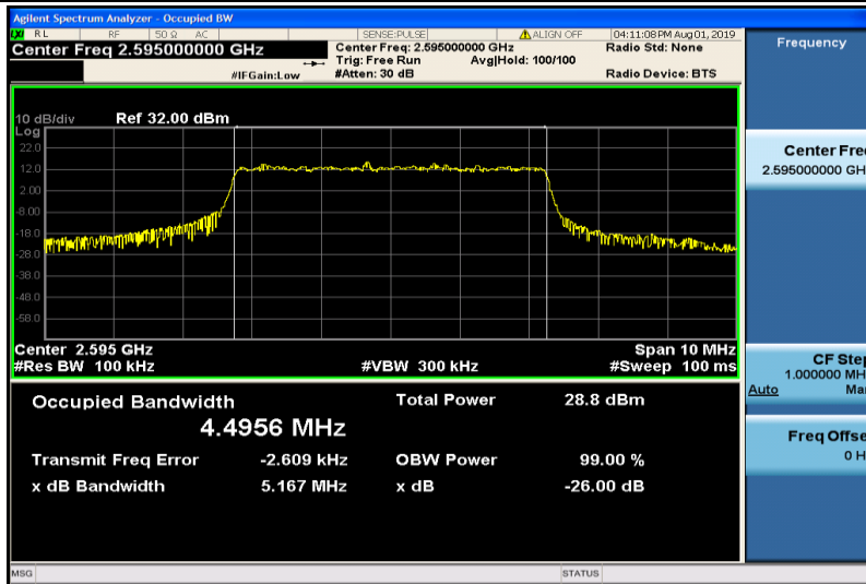
Band38-5MHz-QPSK-38000-25RB#0-4.4956
