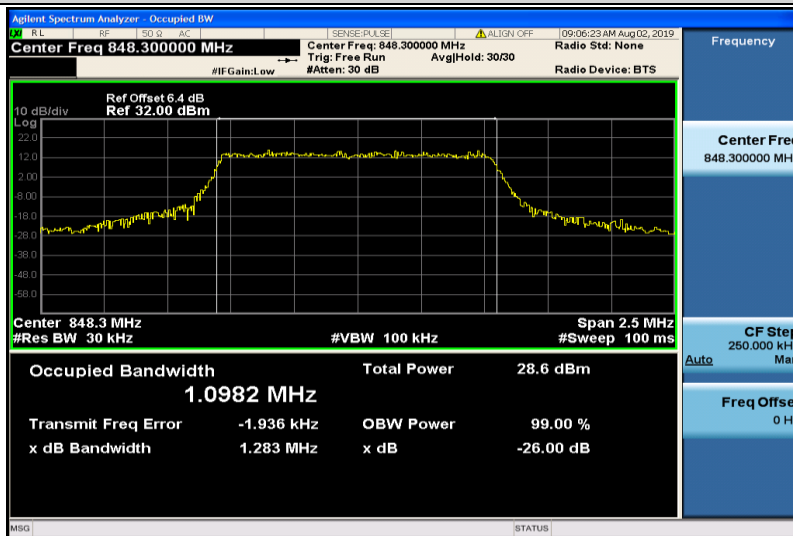
Band5-1.4MHz-QPSK-20643-6RB#0-1.0982
