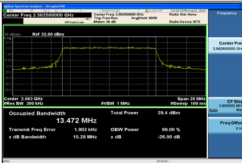
Band7-15MHz-QPSK-21375-75RB#0-13.472
