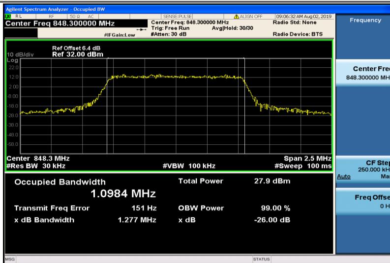
Band5-1.4MHz-16QAM-20643-6RB#0-1.0984
