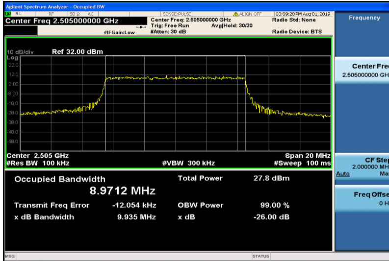
Band7-10MHz-16QAM-20800-50RB#0-8.9712
