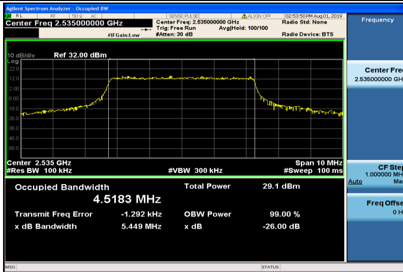
Band7-5MHz-QPSK-21100-25RB#0-4.5183
