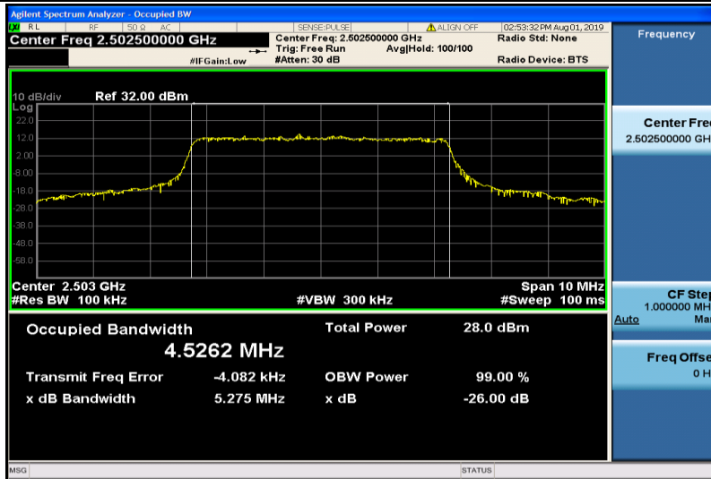
Band7-5MHz-16QAM-20775-25RB#0-4.5262
