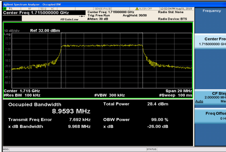
Band4-10MHz-16QAM-20000-50RB#0-8.9593
