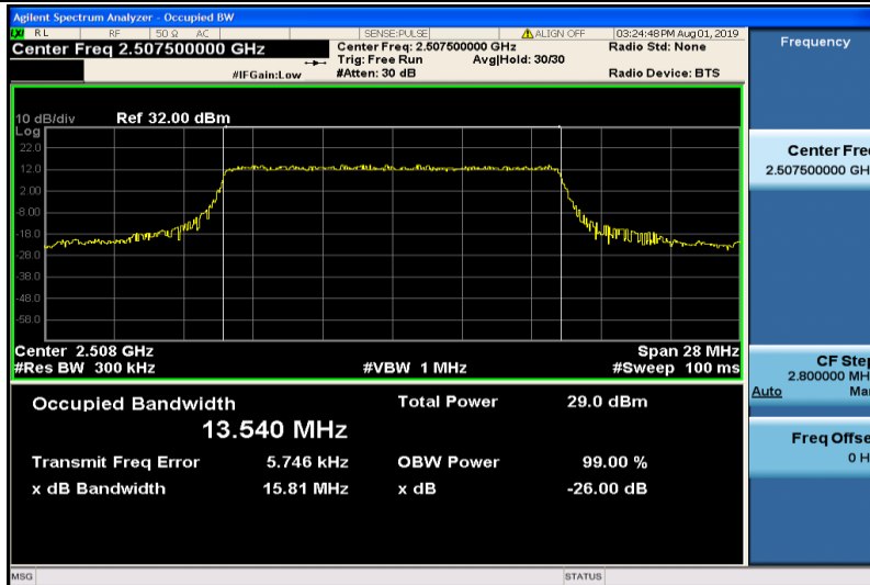
Band7-15MHz-QPSK-20825-75RB#0-13.540
