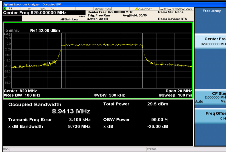
Band5-10MHz-QPSK-20450-50RB#0-8.9413
