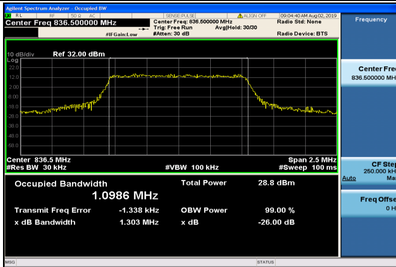
Band5-1.4MHz-QPSK-20525-6RB#0-1.0986
