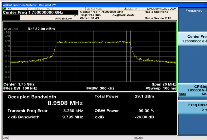
Band4-10MHz-QPSK-20350-50RB#0-8.9508
