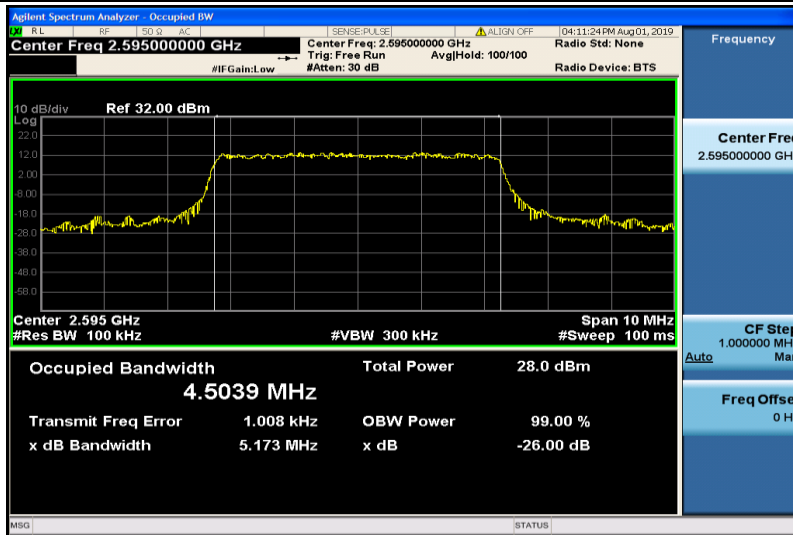
Band38-5MHz-16QAM-38000-25RB#0-4.5039
