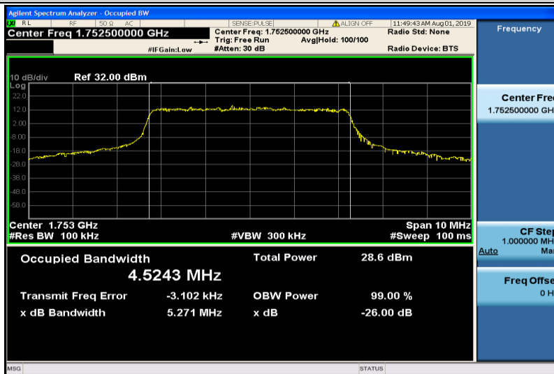
Band4-5MHz-16QAM-20375-25RB#0-4.5243
