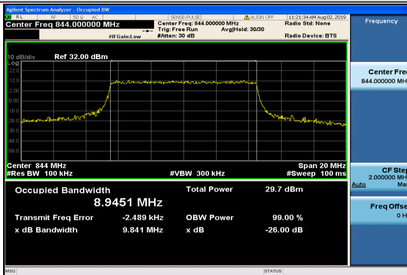
Band5-10MHz-QPSK-20600-50RB#0-8.9451
