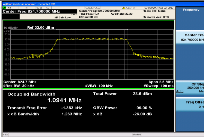
Band5-1.4MHz-QPSK-20407-6RB#0-1.0941
