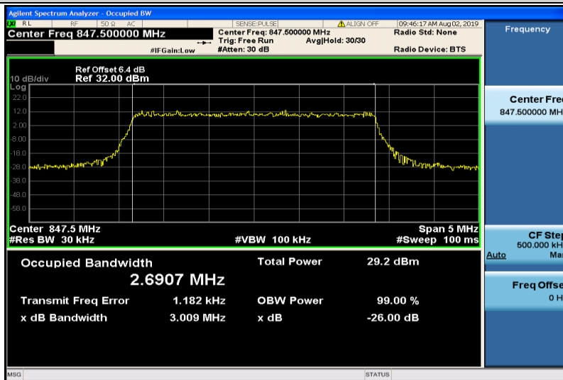
Band5-3MHz-QPSK-20635-15RB#0-2.6907
