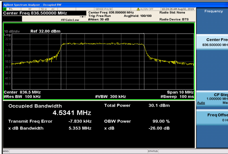
Band5-5MHz-QPSK-20525-25RB#0-4.5341
