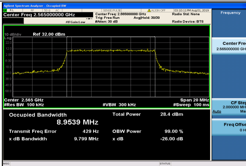
Band7-10MHz-16QAM-21400-50RB#0-8.9539
