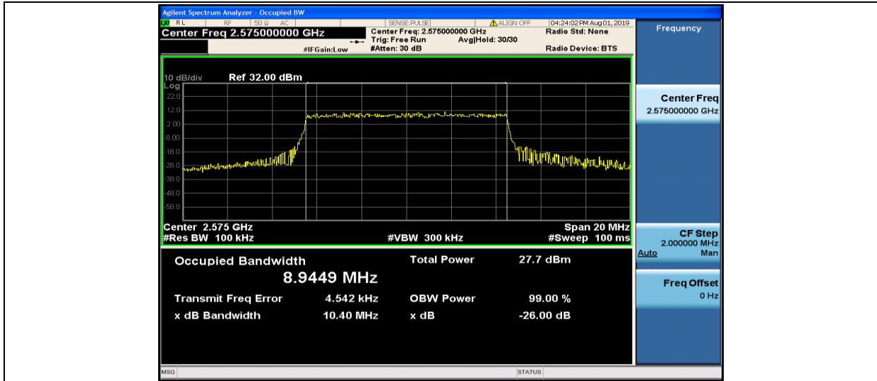
Band38-10MHz-16QAM-37800-50RB#0-8.9449
