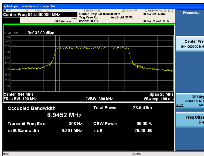
Band5-10MHz-16QAM-20600-50RB#0-8.9452
