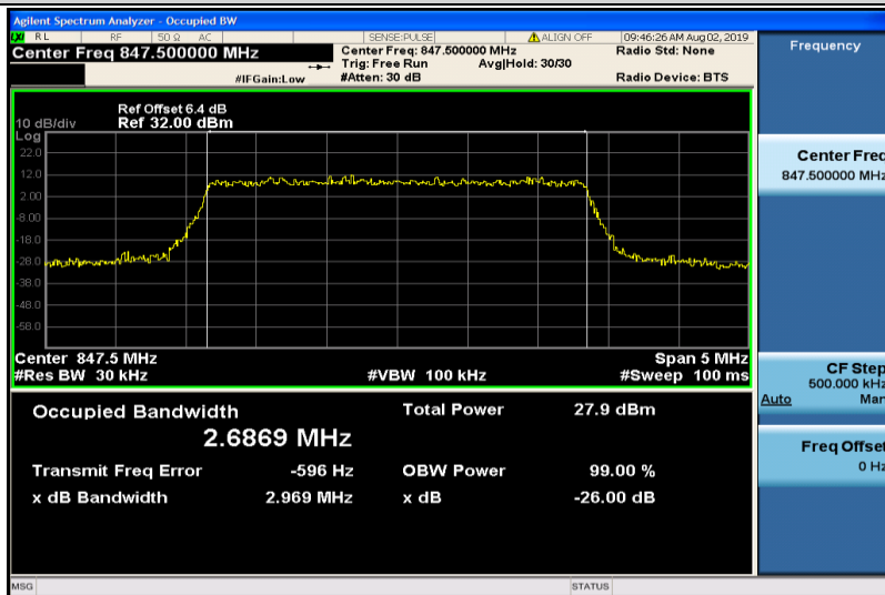
Band5-3MHz-16QAM-20635-15RB#0-2.6869
