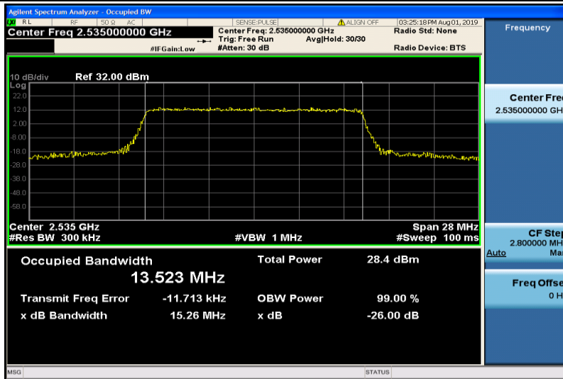
Band7-15MHz-16QAM-21100-75RB#0-13.523
