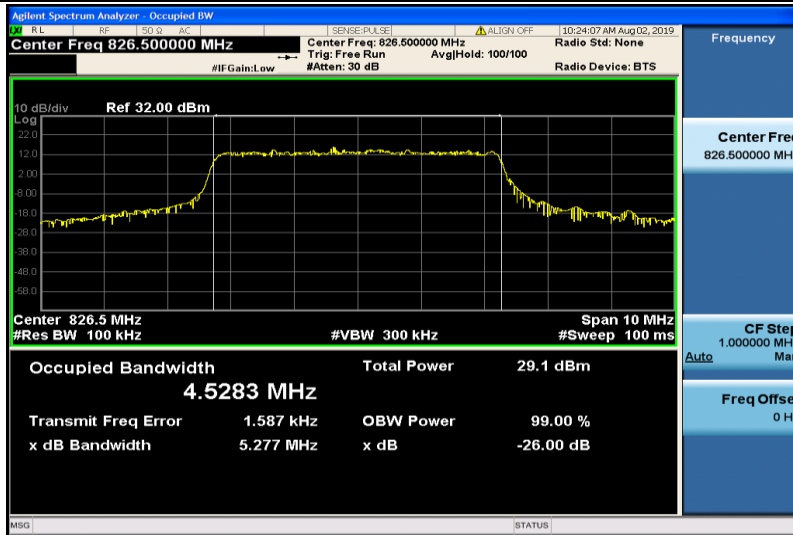
Band5-5MHz-16QAM-20425-25RB#0-4.5283
