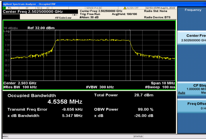
Band7-5MHz-QPSK-20775-25RB#0-4.5358
