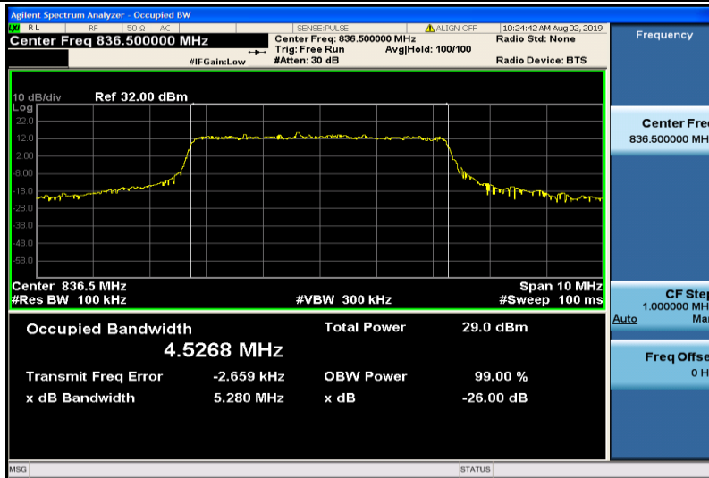
Band5-5MHz-16QAM-20525-25RB#0-4.5268
