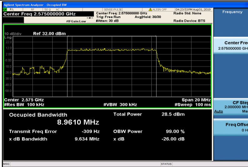
Band38-10MHz-QPSK-37800-50RB#0-8.9610
