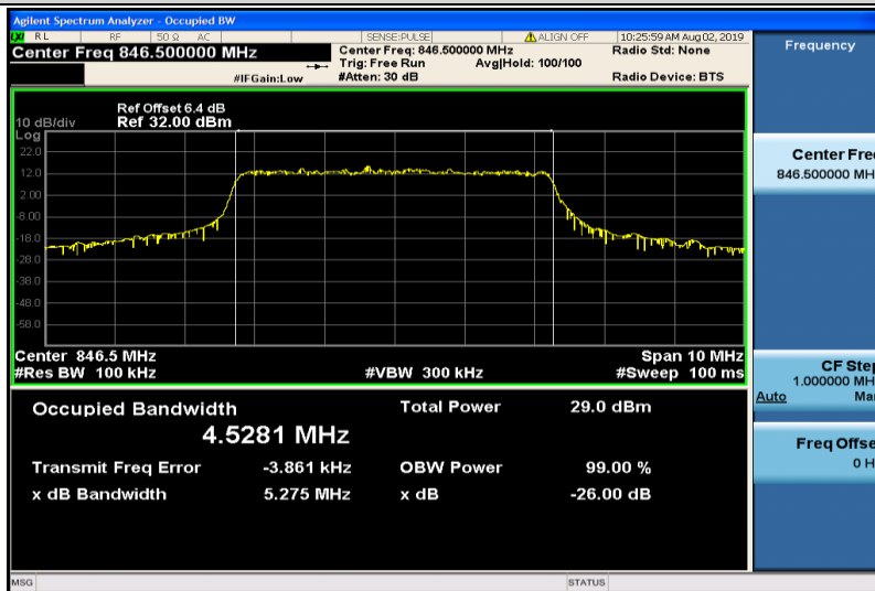
Band5-5MHz-16QAM-20625-25RB#0-4.5281
