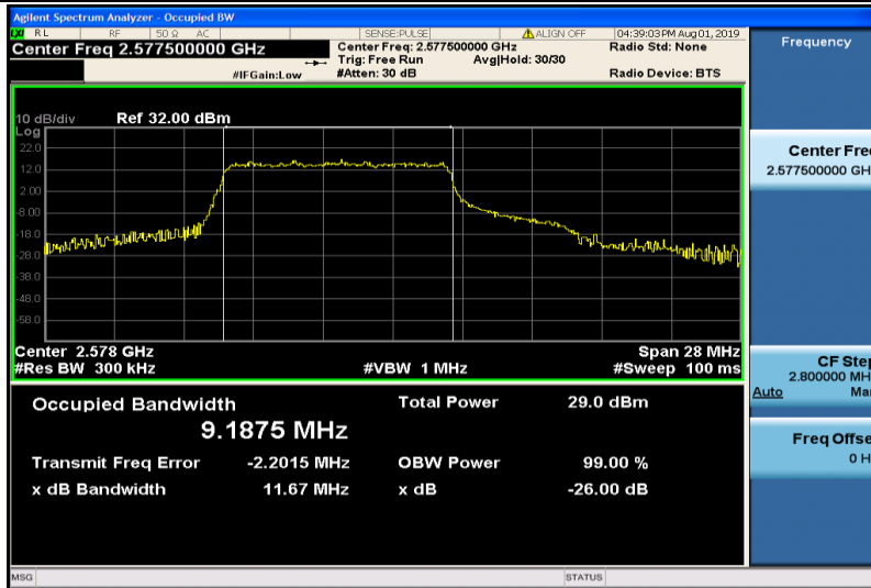
Band38-15MHz-QPSK-37825-75RB#0-9.1875
