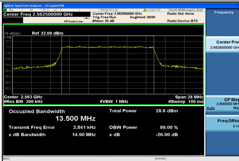
Band7-15MHz-16QAM-21375-75RB#0-13.500
