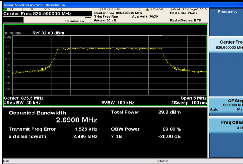
Band5-3MHz-QPSK-20415-15RB#0-2.6908
