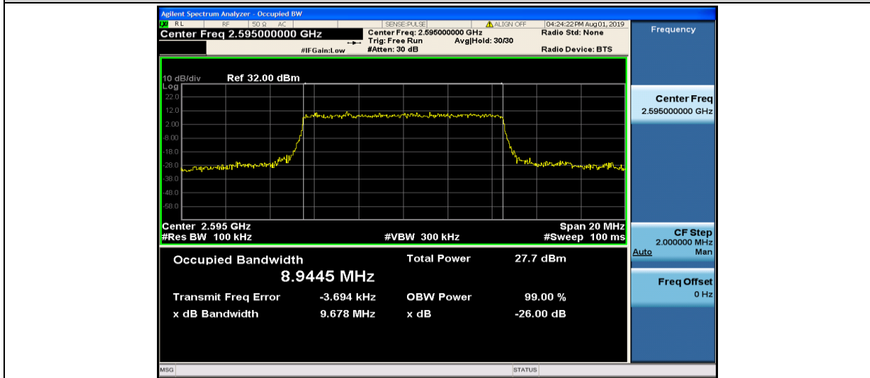
Band38-10MHz-16QAM-38000-50RB#0-8.9445
