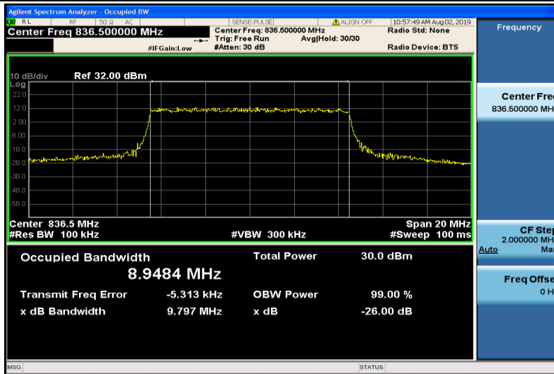
Band5-10MHz-QPSK-20525-50RB#0-8.9484
