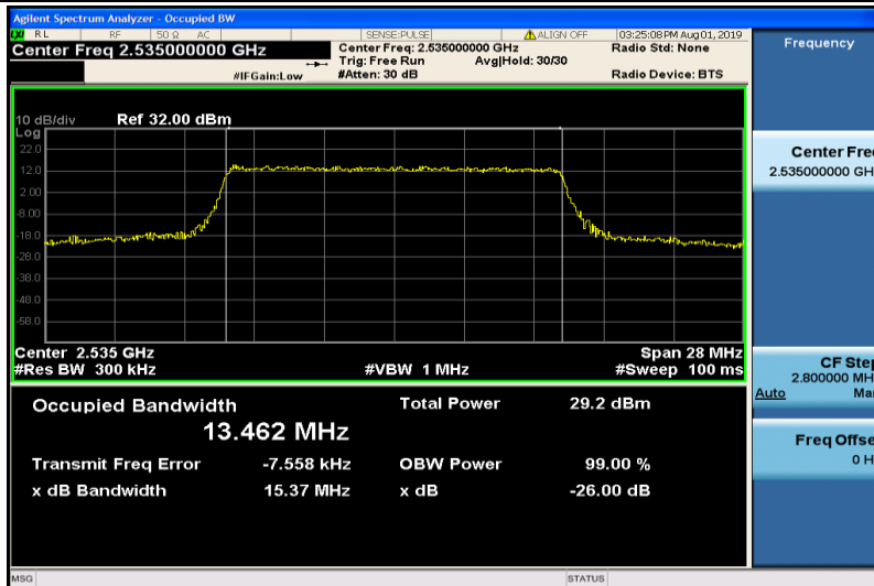
Band7-15MHz-QPSK-21100-75RB#0-13.462
