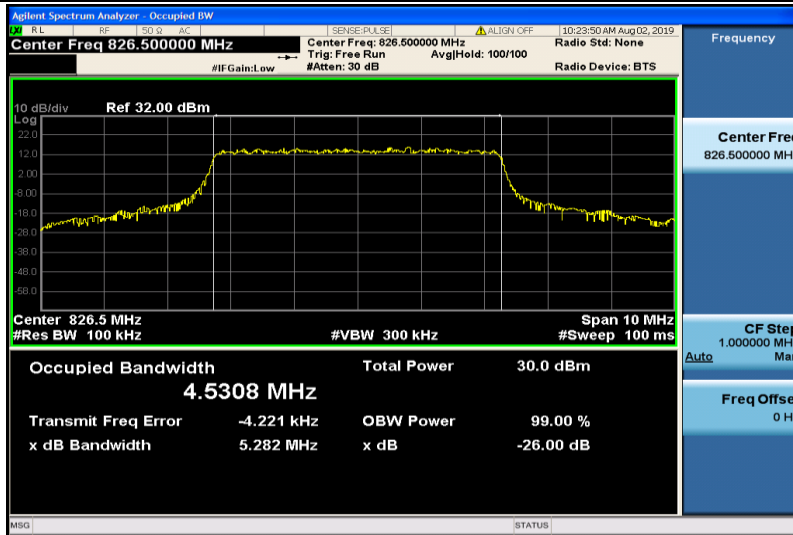
Band5-5MHz-QPSK-20425-25RB#0-4.5308
