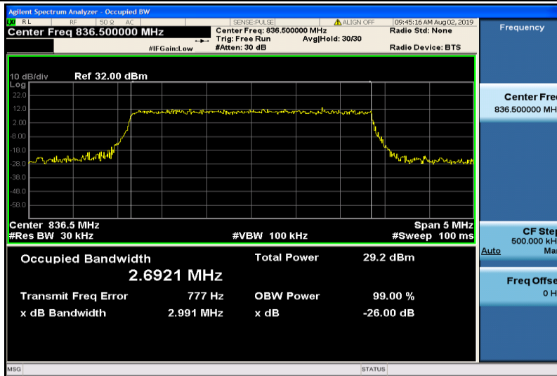
Band5-3MHz-QPSK-20525-15RB#0-2.6921
