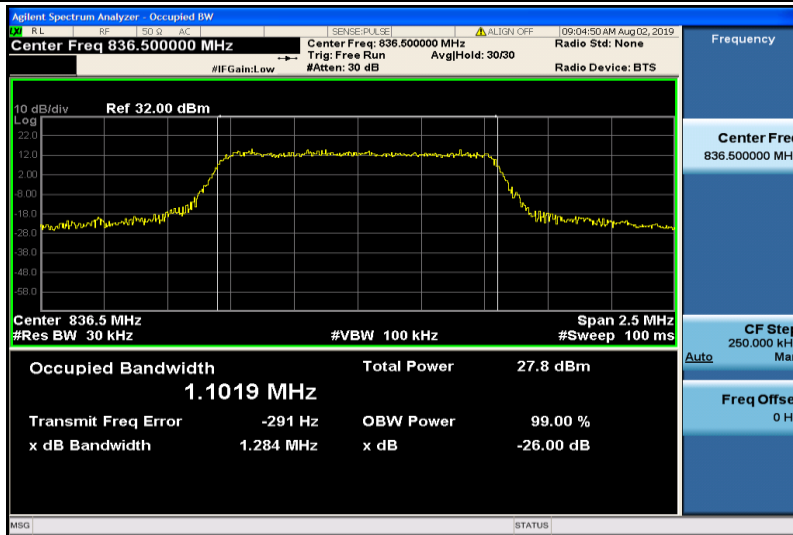
Band5-1.4MHz-16QAM-20525-6RB#0-1.1019
