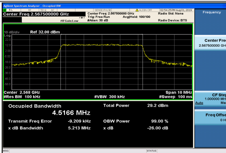
Band7-5MHz-QPSK-21425-25RB#0-4.5166
