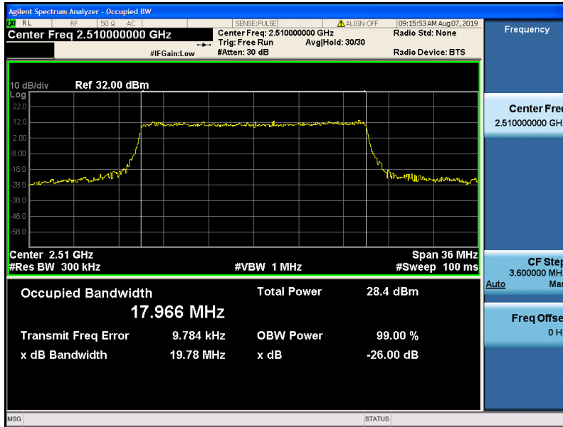
Band7-20MHz-QPSK-20850-100RB#0-9.4625
