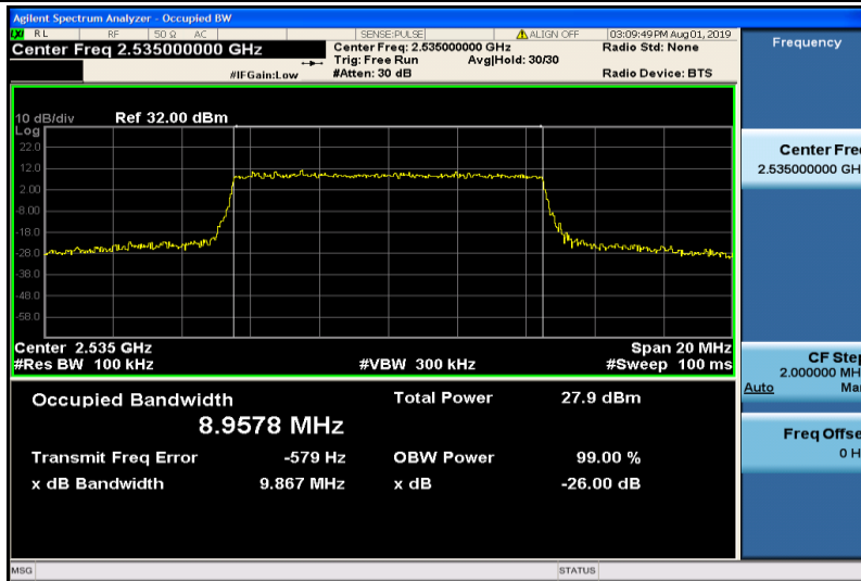
Band7-10MHz-16QAM-21100-50RB#0-8.9578
