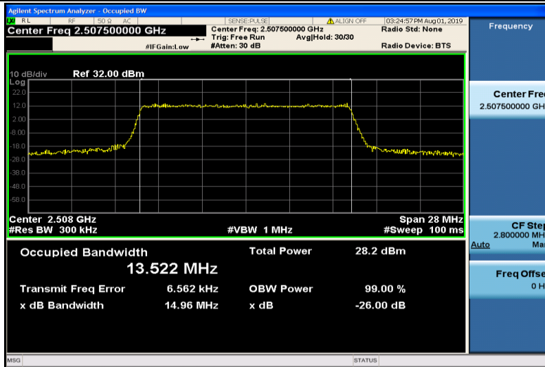
Band7-15MHz-16QAM-20825-75RB#0-13.522
