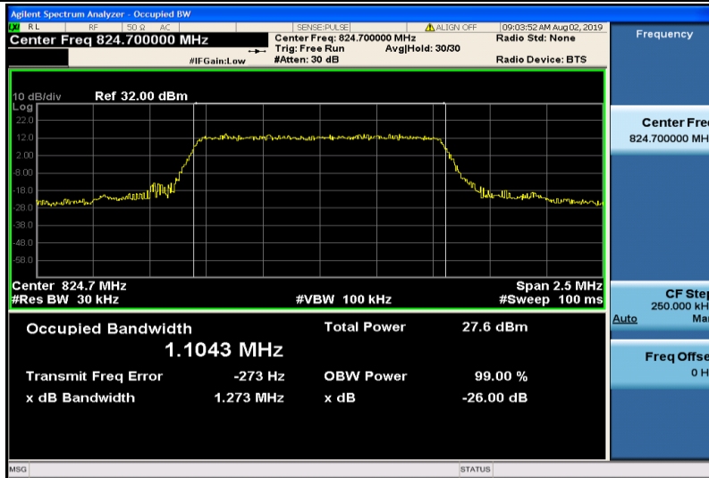
Band5-1.4MHz-16QAM-20407-6RB#0-1.1043
