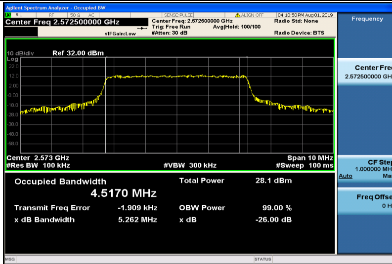
Band38-5MHz-16QAM-37775-25RB#0-4.5170
