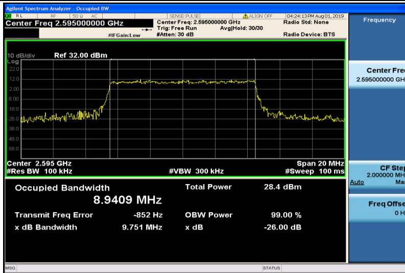
Band38-10MHz-QPSK-38000-50RB#0-8.9409
