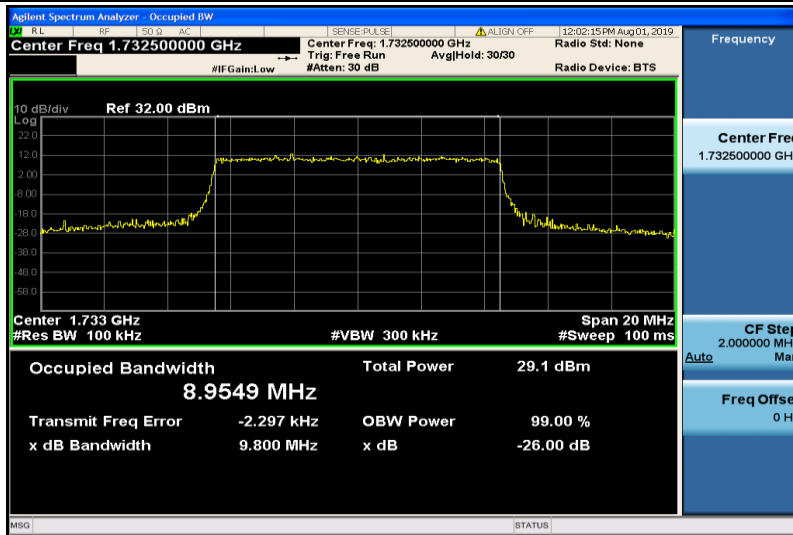
Band4-10MHz-QPSK-20175-50RB#0-8.9549
