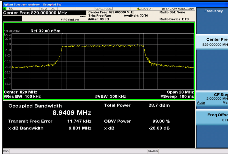
Band5-10MHz-16QAM-20450-50RB#0-8.9409
