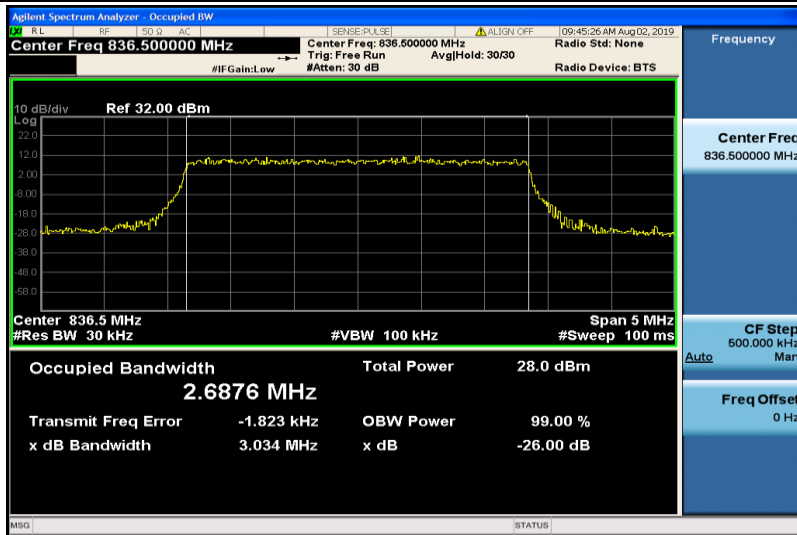
Band5-3MHz-16QAM-20525-15RB#0-2.6876
