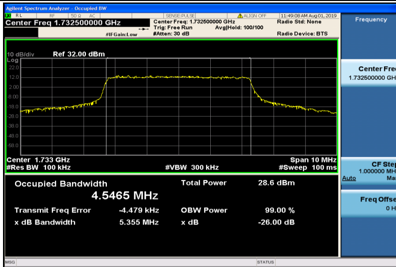
Band4-5MHz-16QAM-20175-25RB#0-4.5465
