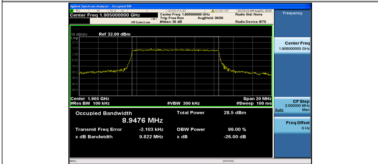
Band2-10MHz-16QAM-19150-50RB#0-8.9476
