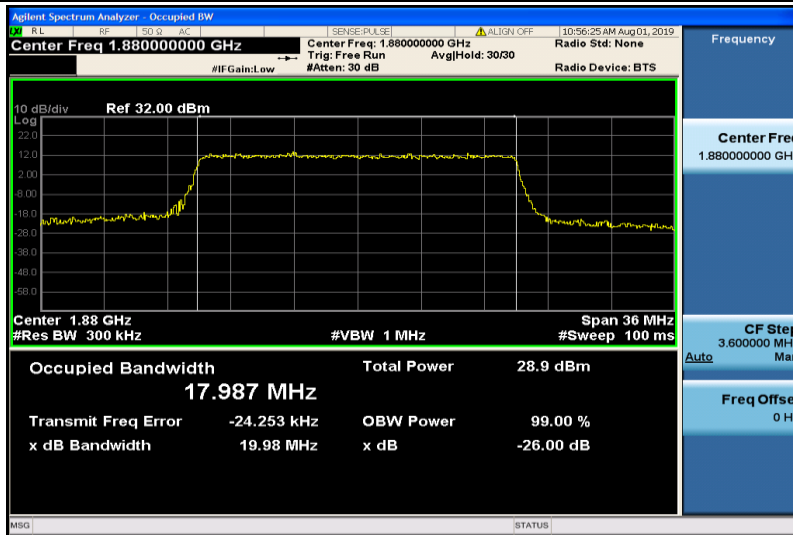
Band2-20MHz-16QAM-18900-100RB#0-17.987
