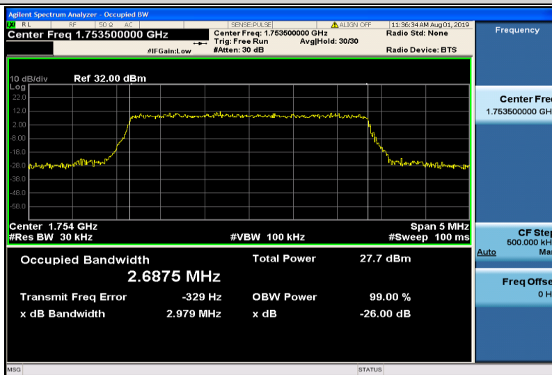
Band4-3MHz-QPSK-20385-15RB#0-2.6875
