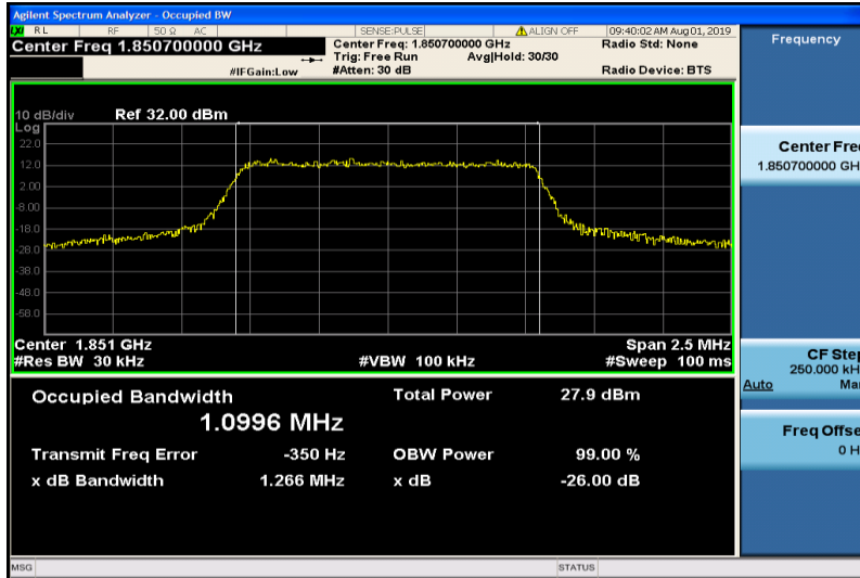
Band2-1.4MHz-16QAM-18607-6RB#0-1.0996
