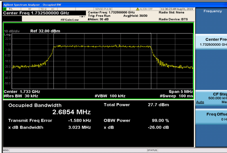
Band4-3MHz-16QAM-20175-15RB#0-2.6854
