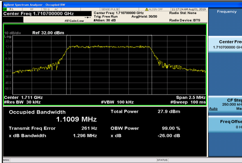
Band4-1.4MHz-16QAM-19957-6RB#0-1.1009
