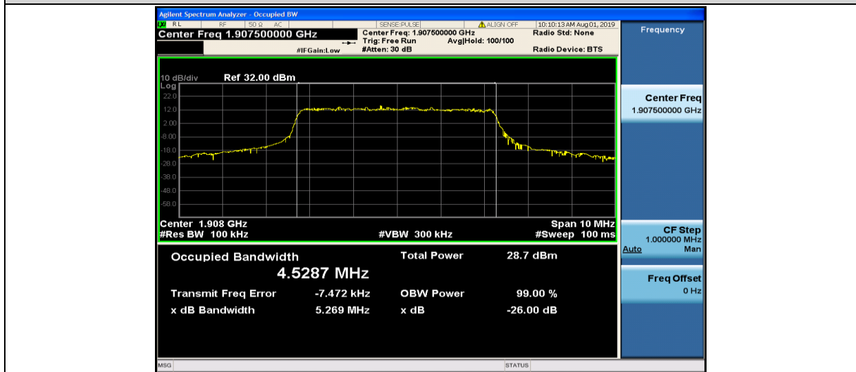
Band2-5MHz-16QAM-19175-25RB#0-4.5287
