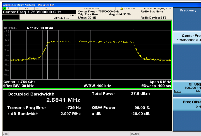
Band4-3MHz-16QAM-20385-15RB#0-2.6841
