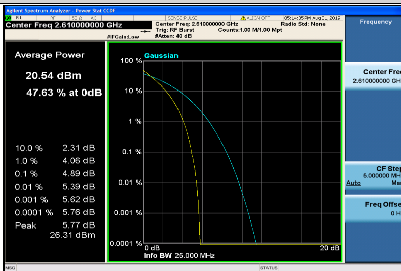
Band38-20MHz-QPSK-38150-100RB#0
