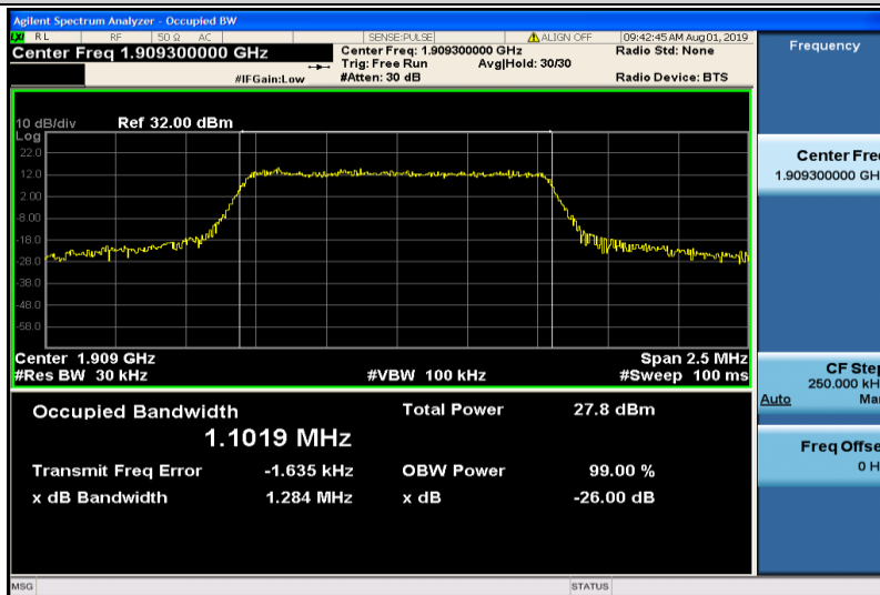
Band2-1.4MHz-16QAM-19193-6RB#0-1.1019
