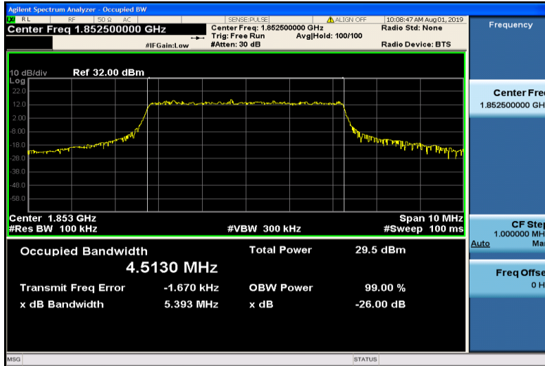
Band2-5MHz-QPSK-18625-25RB#0-4.5130
