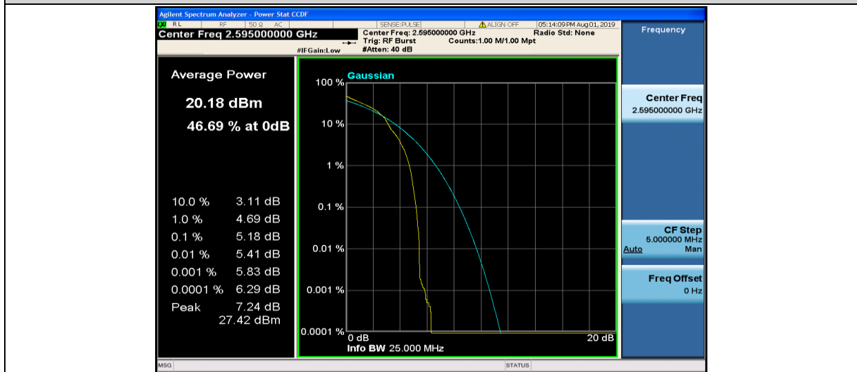
Band38-20MHz-16QAM-38000-1RB#0
