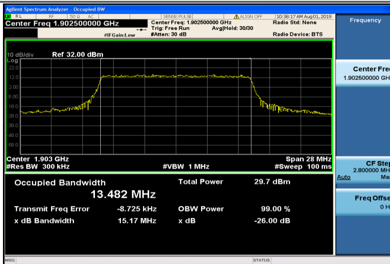
Band2-15MHz-QPSK-19125-75RB#0-13.482
