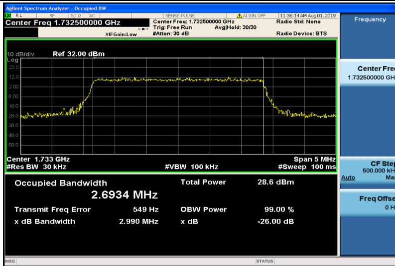
Band4-3MHz-QPSK-20175-15RB#0-2.6934
