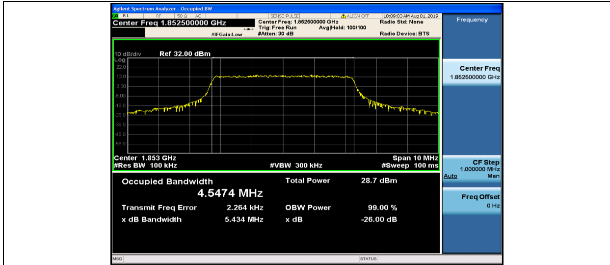
Band2-5MHz-16QAM-18625-25RB#0-4.5474
