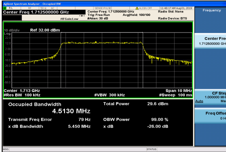
Band4-5MHz-QPSK-19975-25RB#0-4.5130
