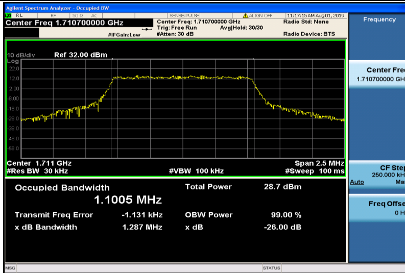
Band4-1.4MHz-QPSK-19957-6RB#0-1.1005
