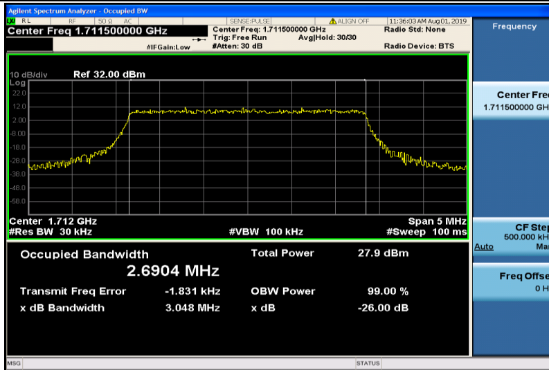
Band4-3MHz-16QAM-19965-15RB#0-2.6904
