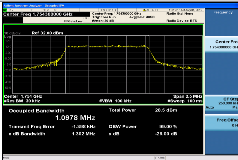
Band4-1.4MHz-QPSK-20393-6RB#0-1.0978
