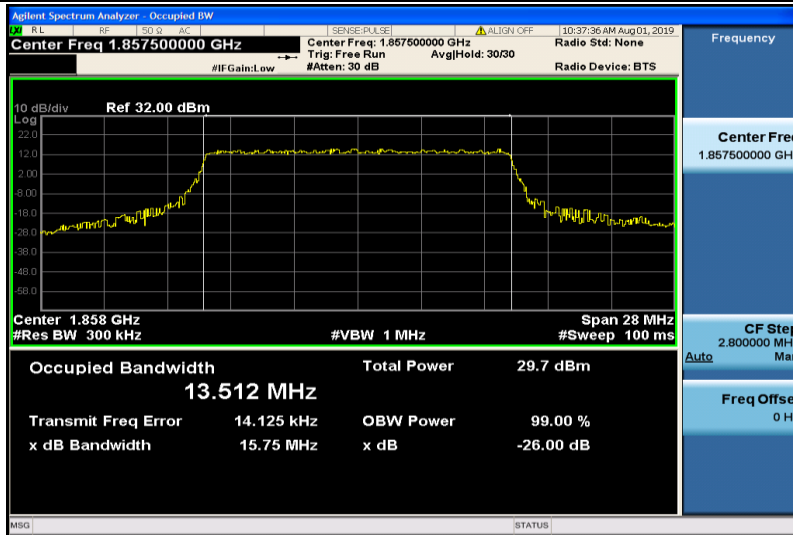
Band2-15MHz-QPSK-18675-75RB#0-13.512
