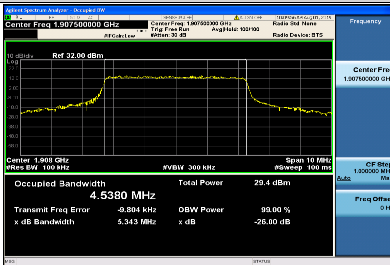
Band2-5MHz-QPSK-19175-25RB#0-4.5380
