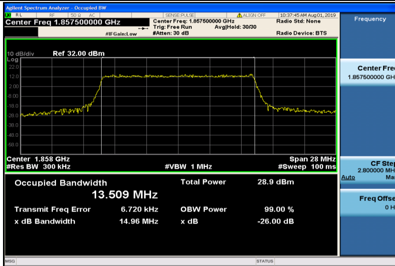
Band2-15MHz-16QAM-18675-75RB#0-13.509
