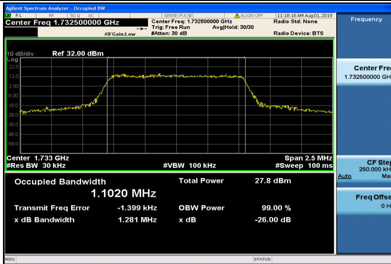
Band4-1.4MHz-16QAM-20175-6RB#0-1.1020
