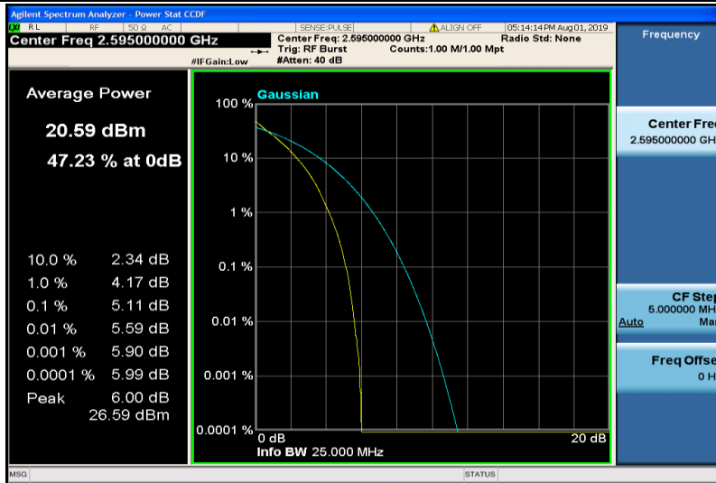
Band38-20MHz-QPSK-38000-100RB#0
