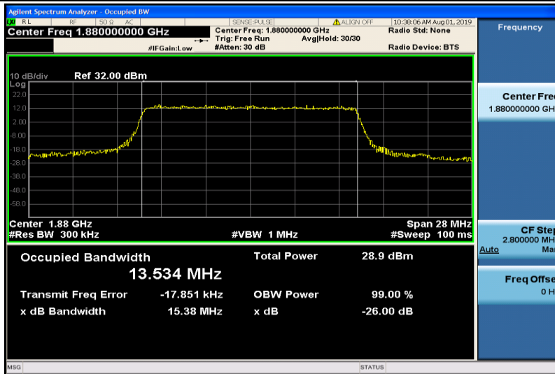
Band2-15MHz-16QAM-18900-75RB#0-13.534
