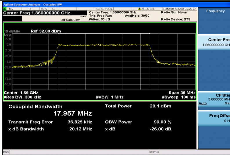
Band2-20MHz-16QAM-18700-100RB#0-17.957
