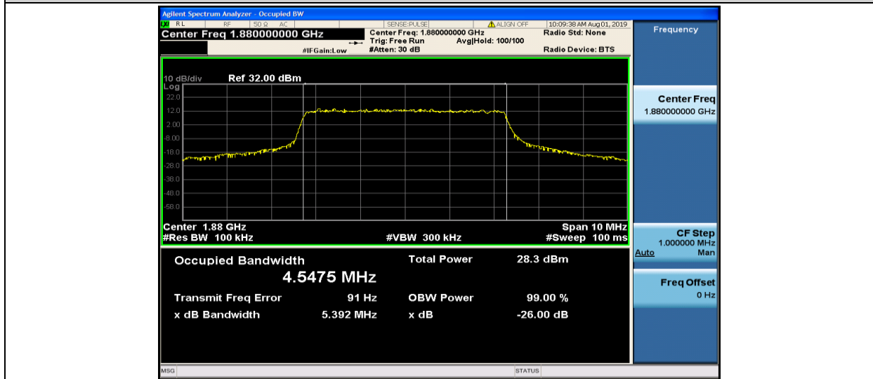
Band2-5MHz-16QAM-18900-25RB#0-4.5475
