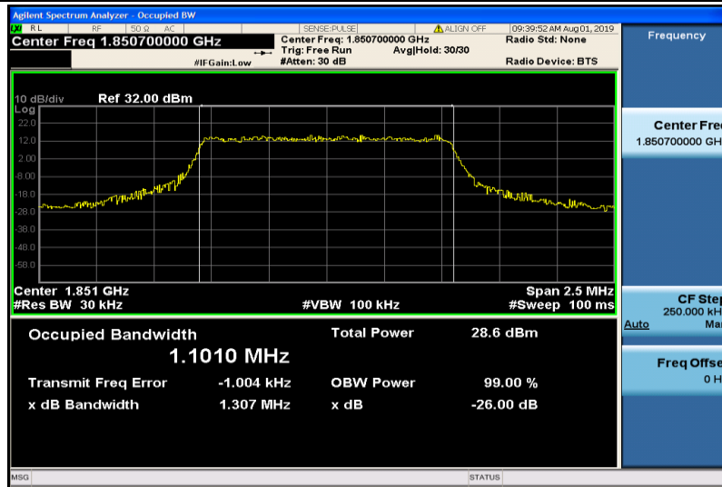
Band2-1.4MHz-QPSK-18607-6RB#0-1.1010
