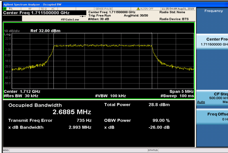
Band4-3MHz-QPSK-19965-15RB#0-2.6885
