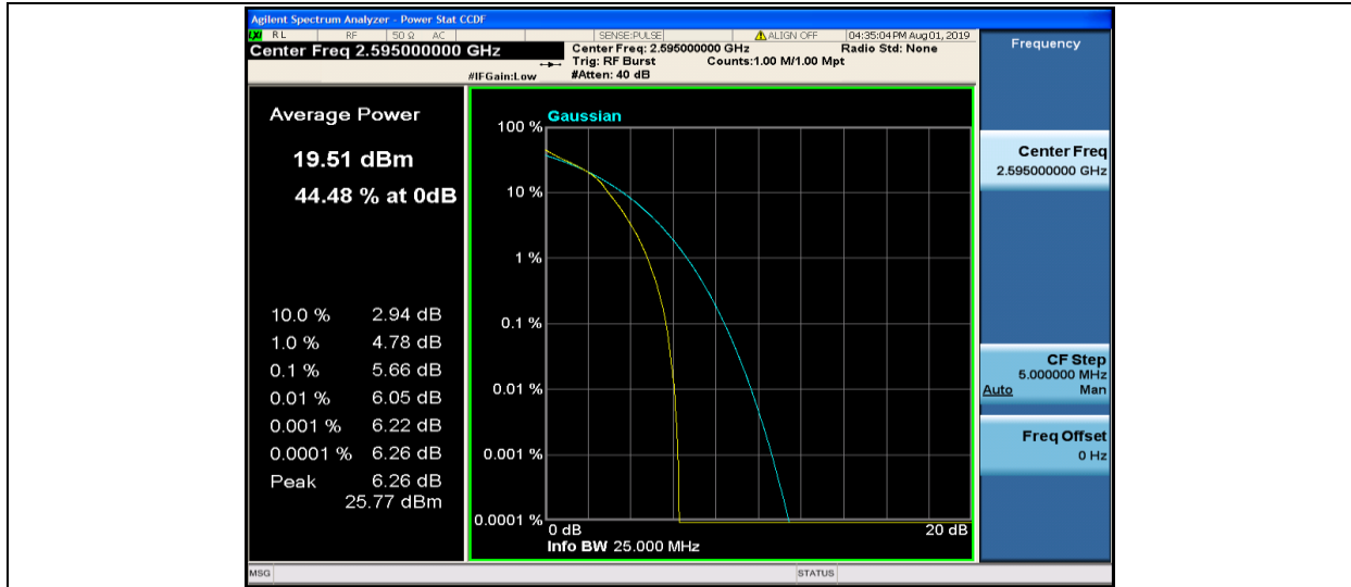
Band38-10MHz-16QAM-38000-50RB#0
