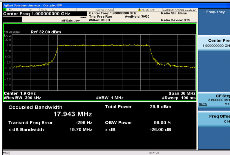
Band2-20MHz-QPSK-19100-100RB#0-17.943
