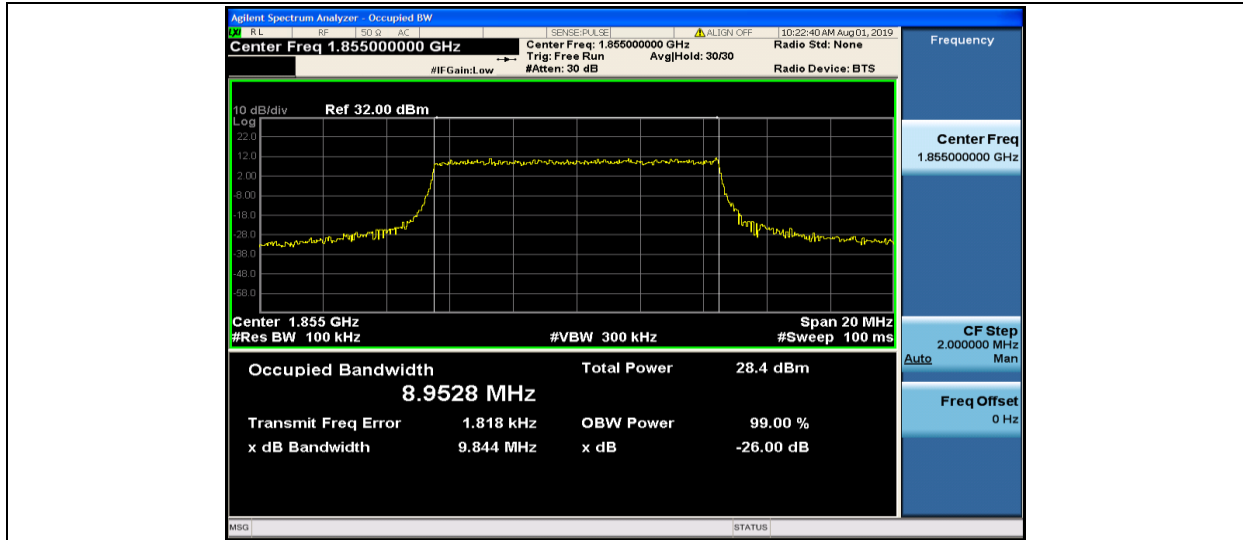
Band2-10MHz-16QAM-18650-50RB#0-8.9528
