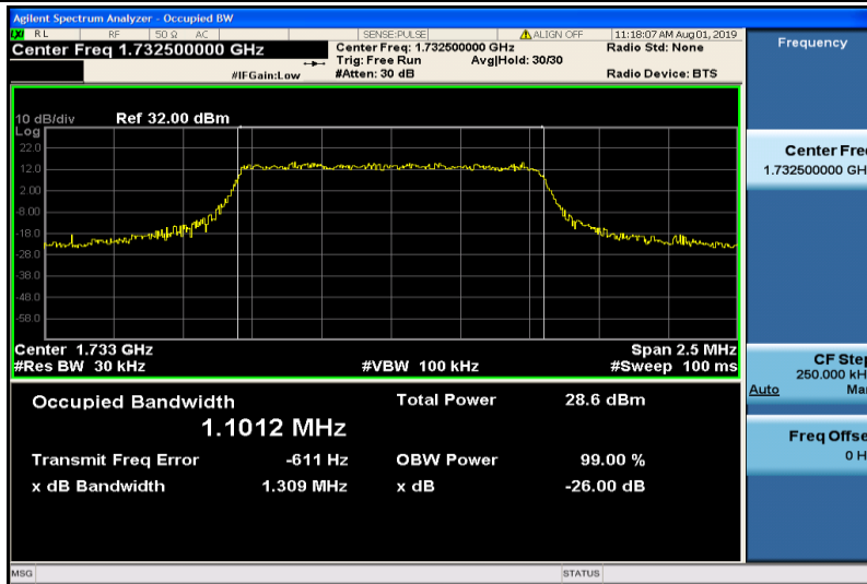
Band4-1.4MHz-QPSK-20175-6RB#0-1.1012
