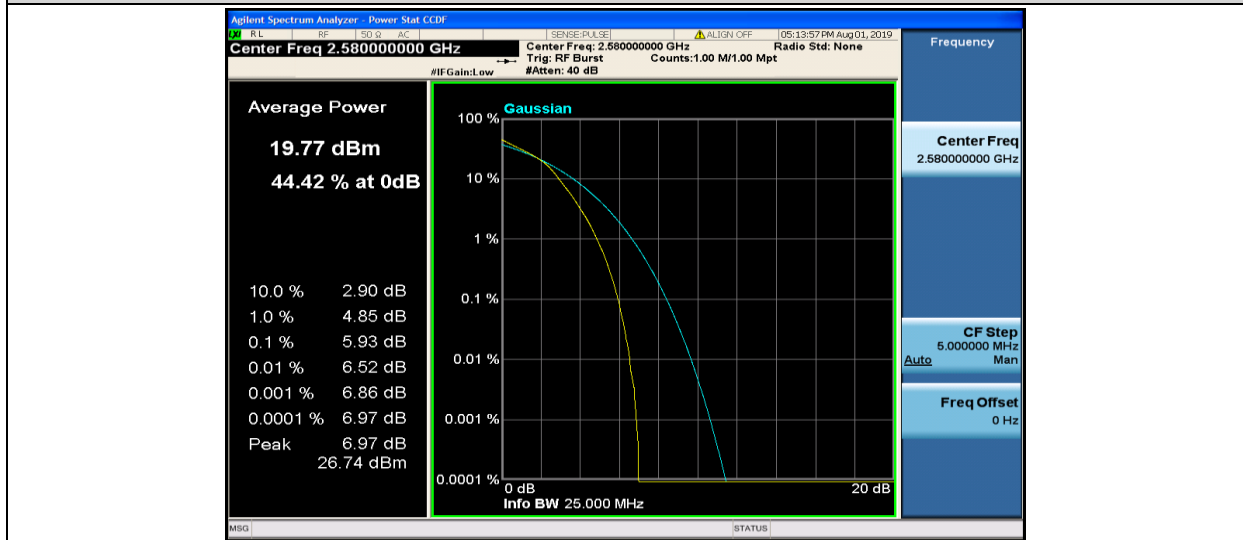
Band38-20MHz-16QAM-37850-100RB#0
