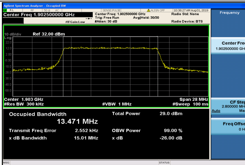
Band2-15MHz-16QAM-19125-75RB#0-13.471
