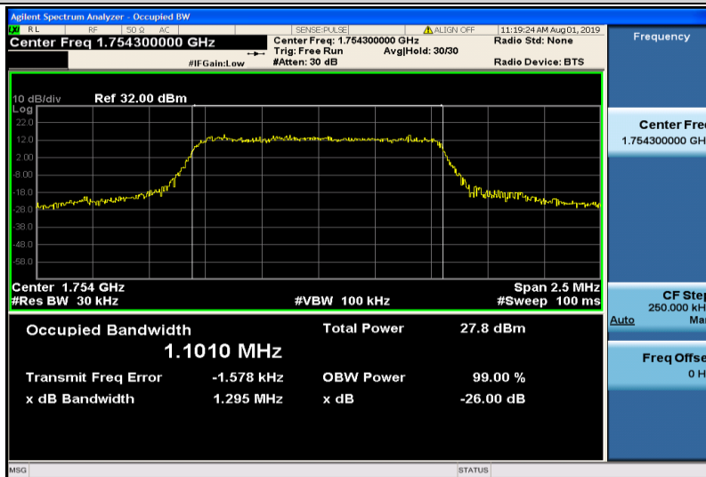
Band4-1.4MHz-16QAM-20393-6RB#0-1.1010
