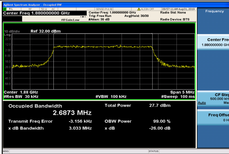
Band2-3MHz-16QAM-18900-15RB#0-2.6873
