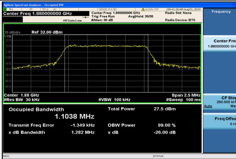
Band2-1.4MHz-16QAM-18900-6RB#0-1.1038
