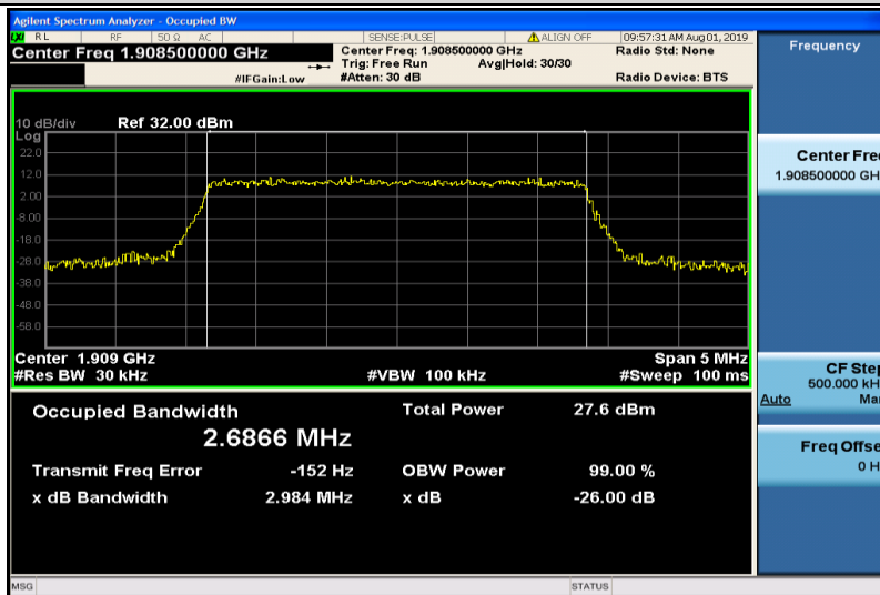
Band2-3MHz-16QAM-19185-15RB#0-2.6866
