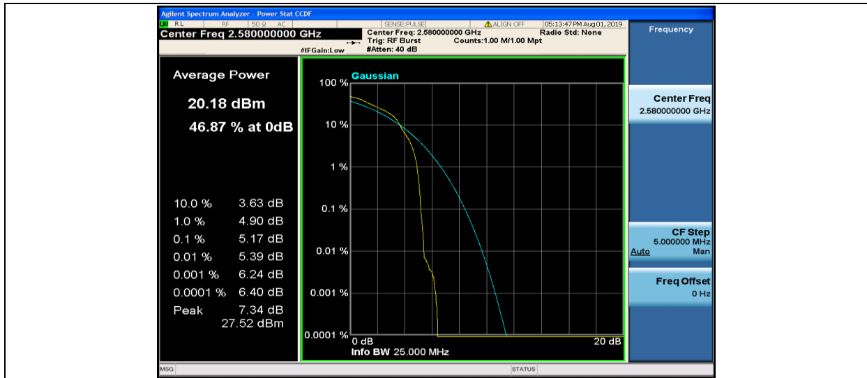
Band38-20MHz-16QAM-37850-1RB#0
