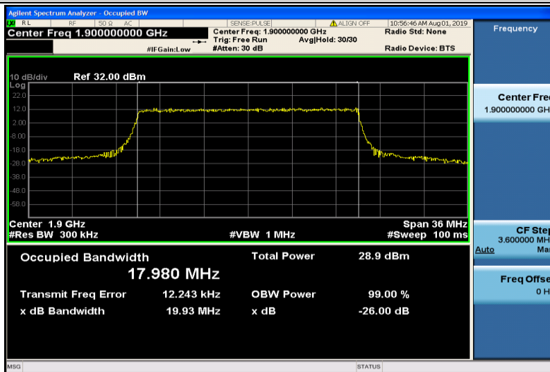
Band2-20MHz-16QAM-19100-100RB#0-17.980
