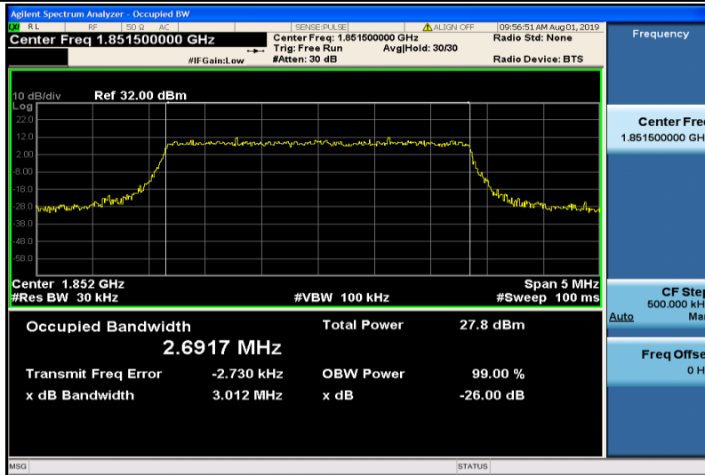
Band2-3MHz-16QAM-18615-15RB#0-2.6917
