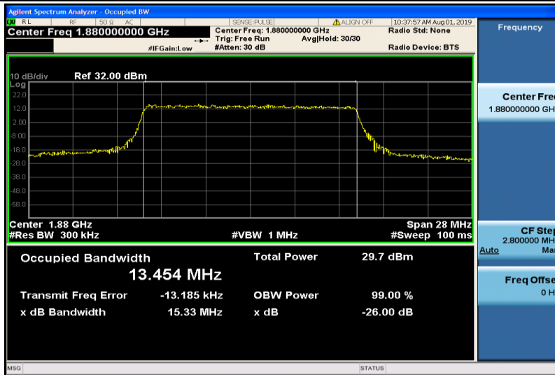
Band2-15MHz-QPSK-18900-75RB#0-13.454
