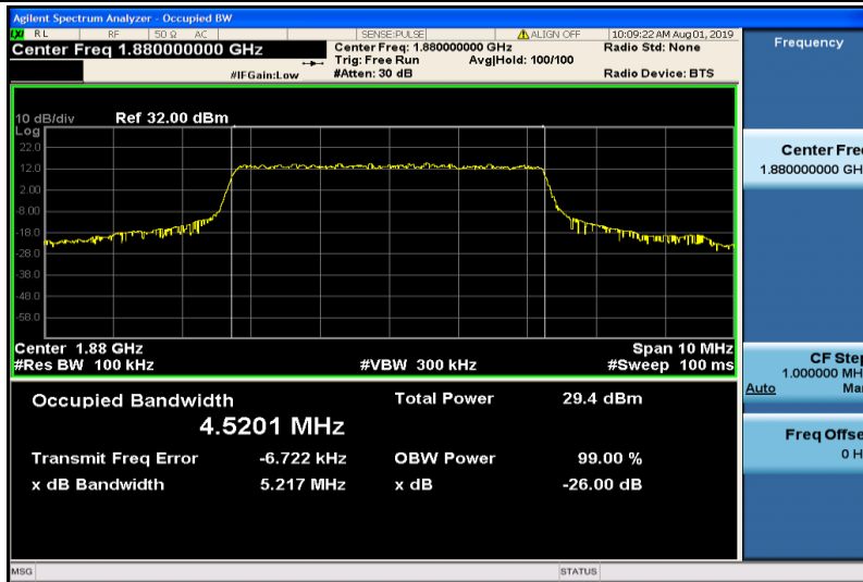
Band2-5MHz-QPSK-18900-25RB#0-4.5201
