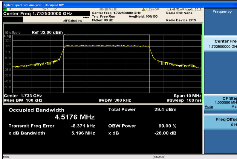
Band4-5MHz-QPSK-20175-25RB#0-4.5176
