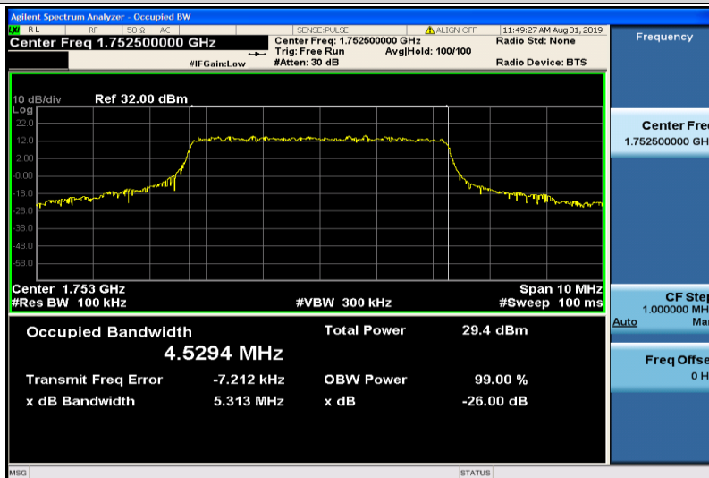
Band4-5MHz-QPSK-20375-25RB#0-4.5294
