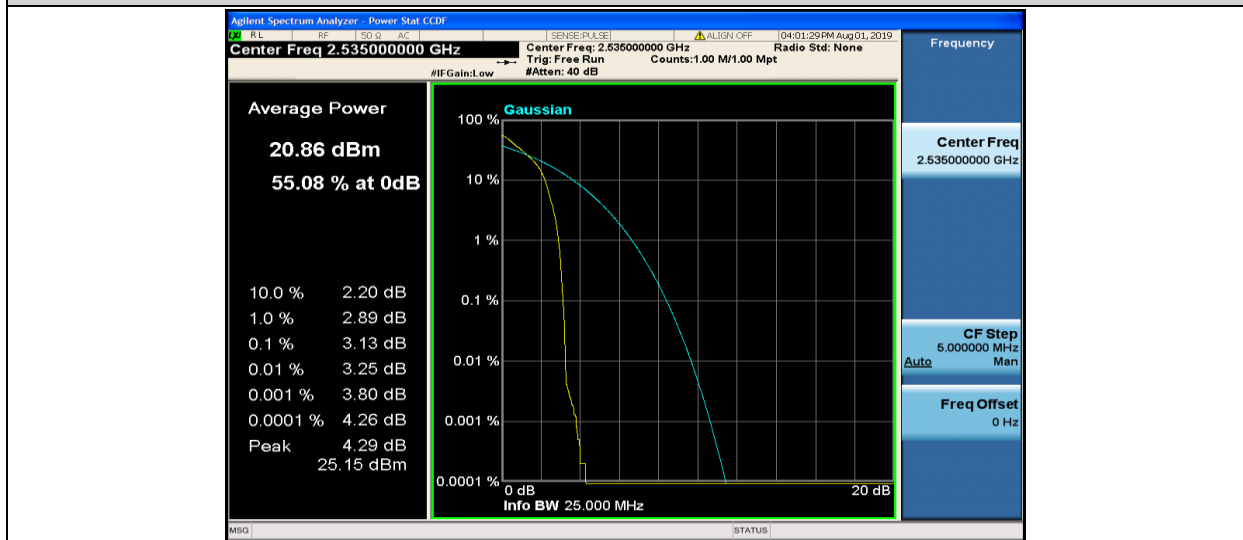
Band7-20MHz-QPSK-21100-1RB#0
