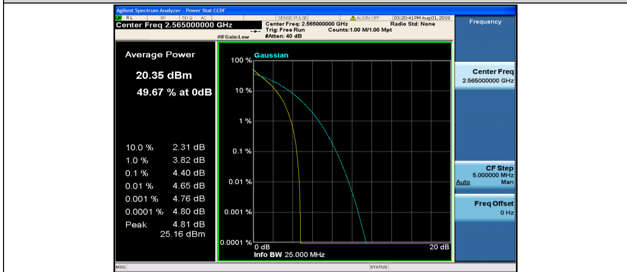
Band7-10MHz-QPSK-21400-50RB#0
