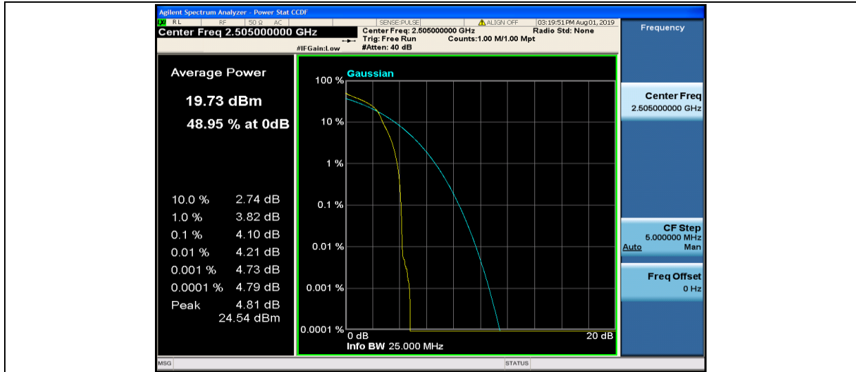
Band7-10MHz-16QAM-20800-1RB#0
