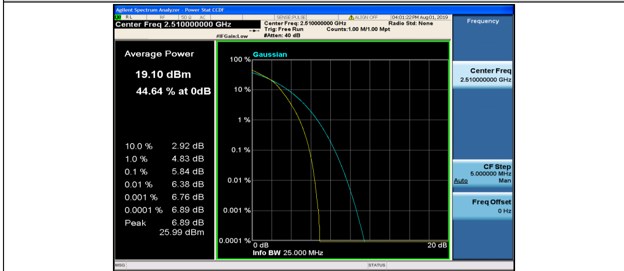
Band7-20MHz-16QAM-20850-100RB#0
