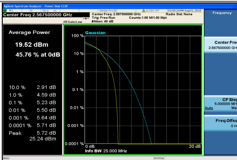
Band7-5MHz-16QAM-21425-25RB#0
