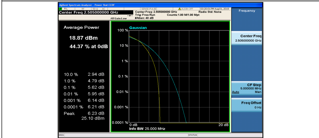
Band7-10MHz-16QAM-20800-50RB#0
