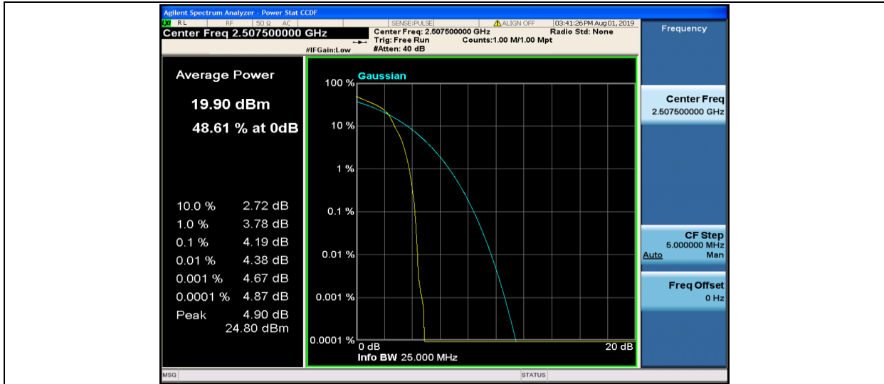
Band7-15MHz-16QAM-20825-1RB#0
