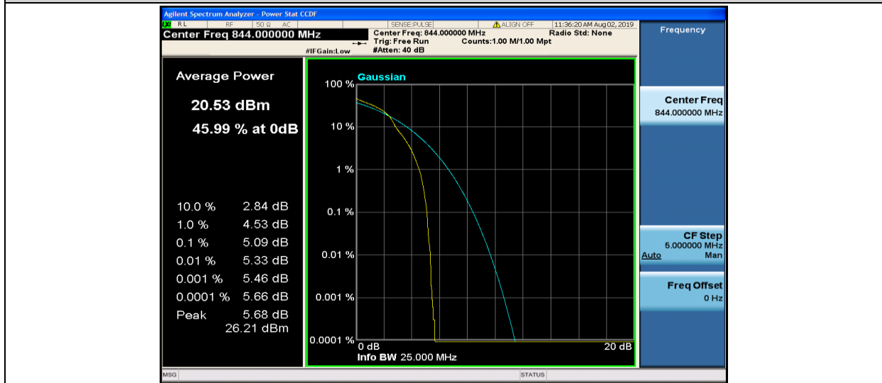
Band5-10MHz-16QAM-20600-1RB#0
