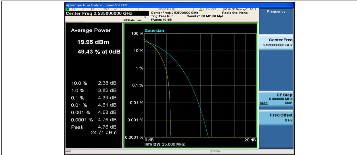
Band7-5MHz-QPSK-21100-25RB#0
