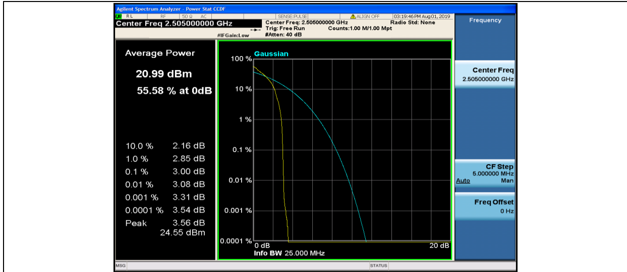
Band7-10MHz-QPSK-20800-1RB#0
