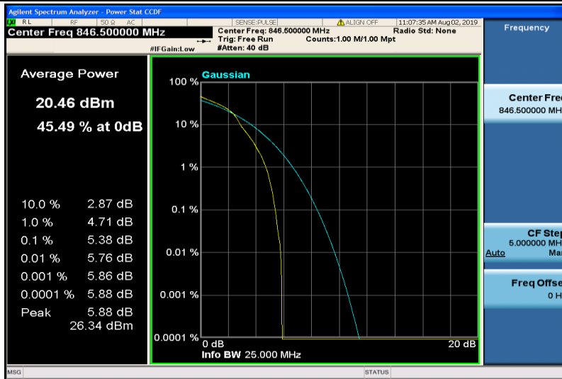
Band5-5MHz-16QAM-20625-1RB#0
