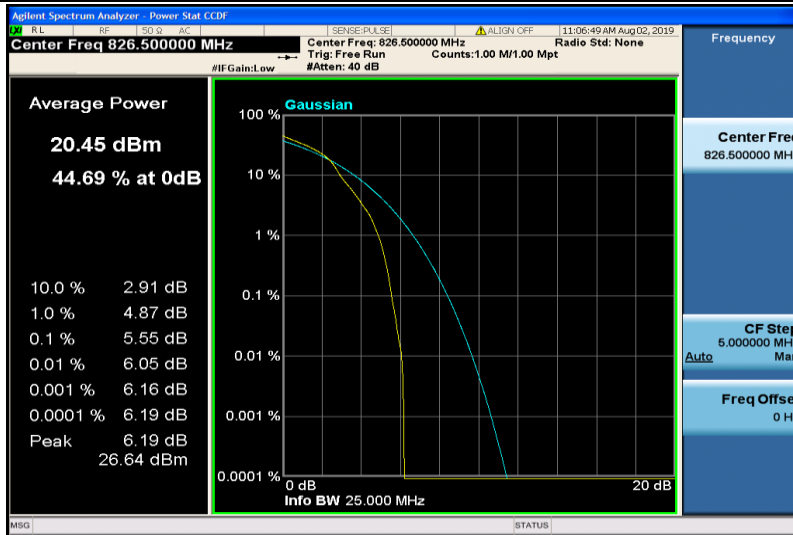
Band5-5MHz-16QAM-20425-1RB#0
