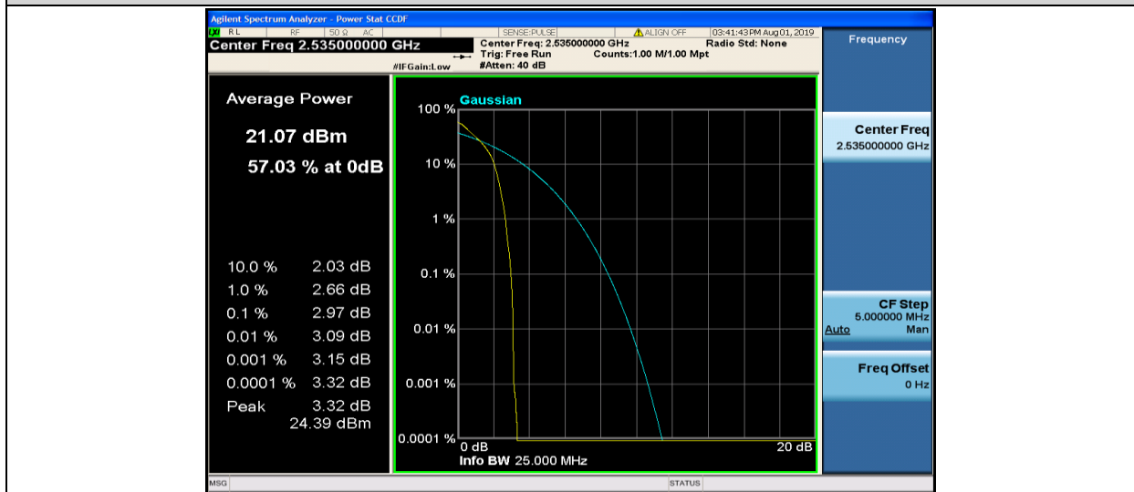
Band7-15MHz-QPSK-21100-1RB#0
