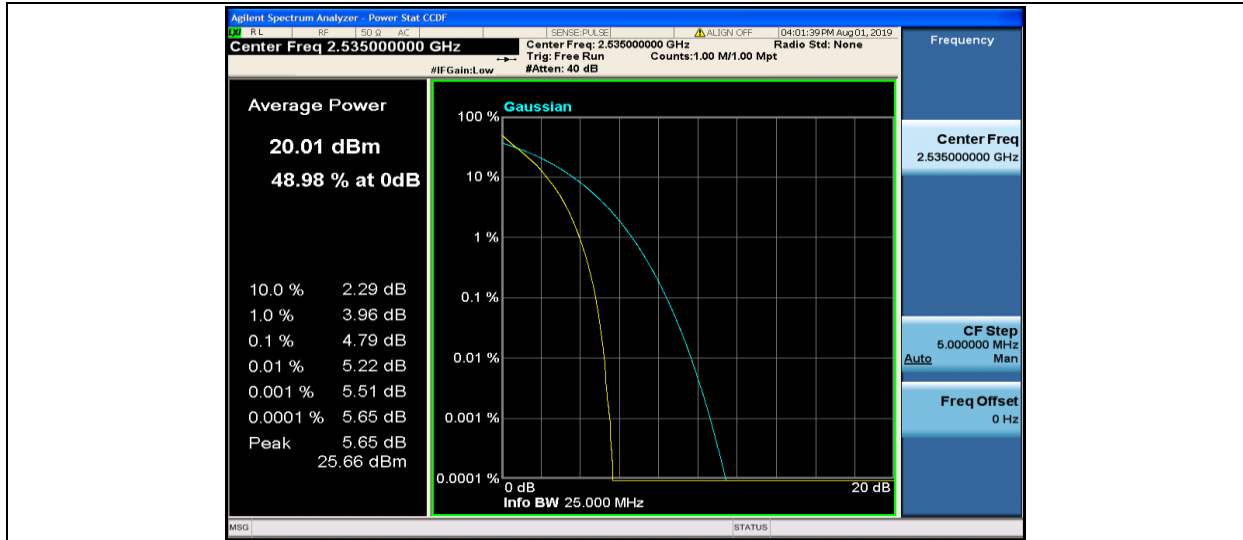
Band7-20MHz-QPSK-21100-100RB#0
