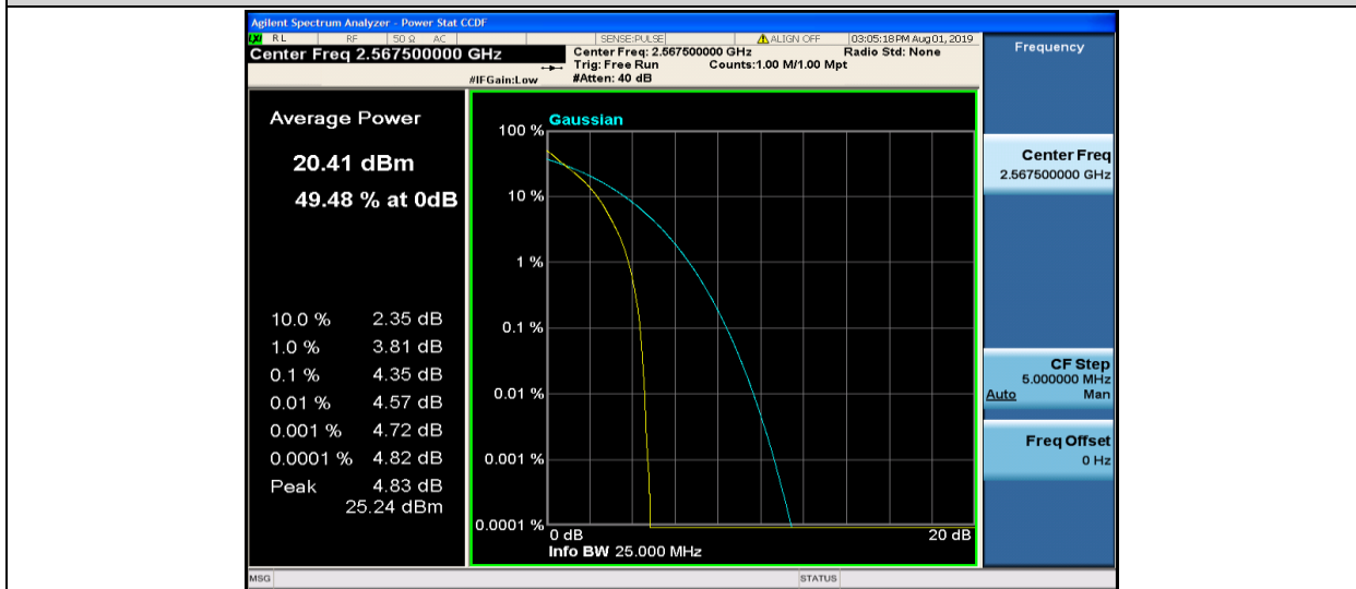
Band7-5MHz-QPSK-21425-25RB#0
