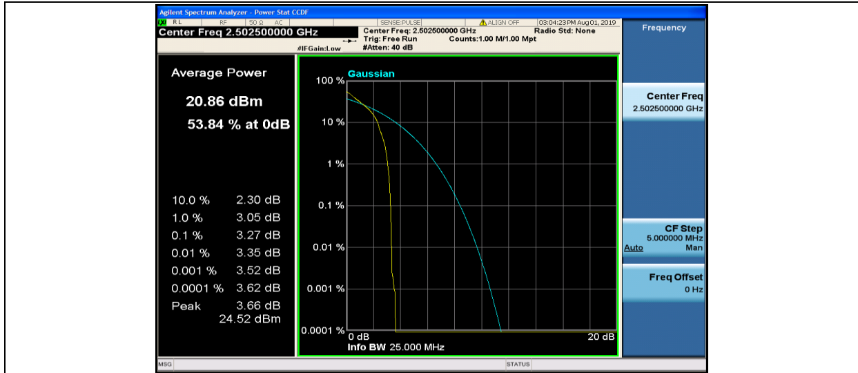
Band7-5MHz-QPSK-20775-1RB#0
