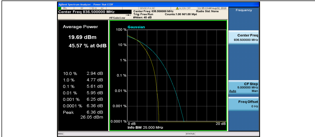
Band5-10MHz-16QAM-20525-50RB#0
