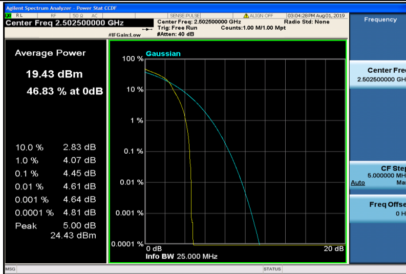
Band7-5MHz-16QAM-20775-1RB#0
