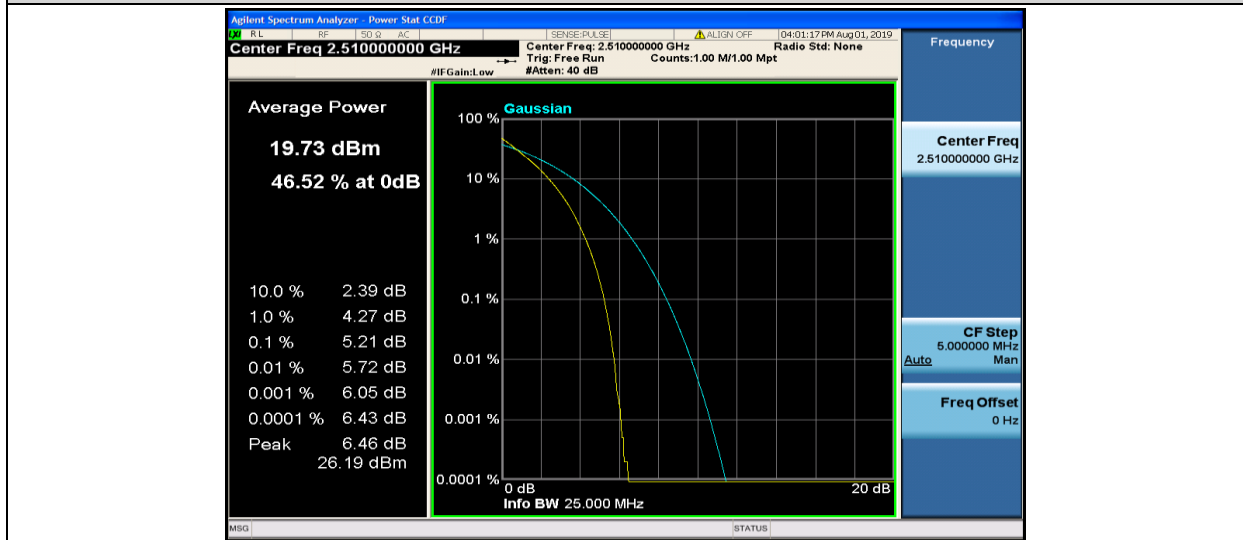
Band7-20MHz-QPSK-20850-100RB#0
