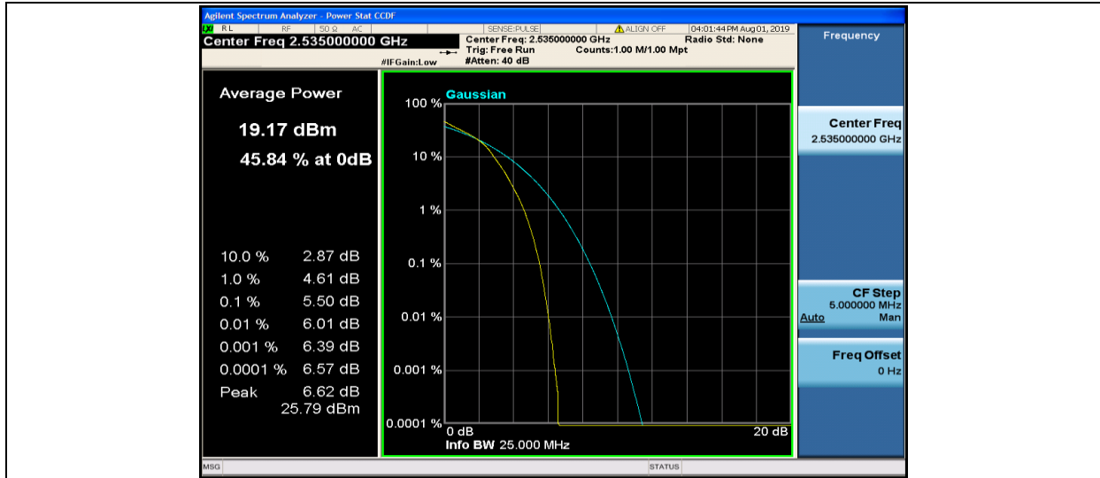
Band7-20MHz-16QAM-21100-100RB#0
