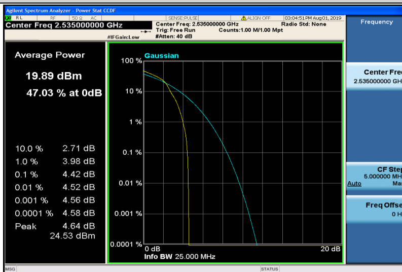
Band7-5MHz-16QAM-21100-1RB#0
