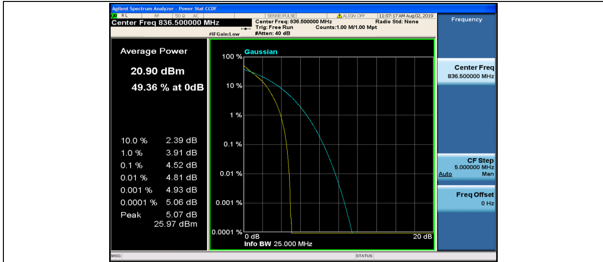
Band5-5MHz-QPSK-20525-25RB#0
