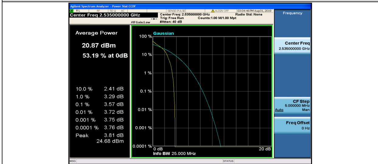
Band7-5MHz-QPSK-21100-1RB#0
