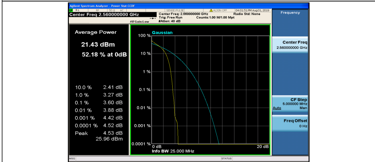
Band7-20MHz-QPSK-21350-1RB#0
