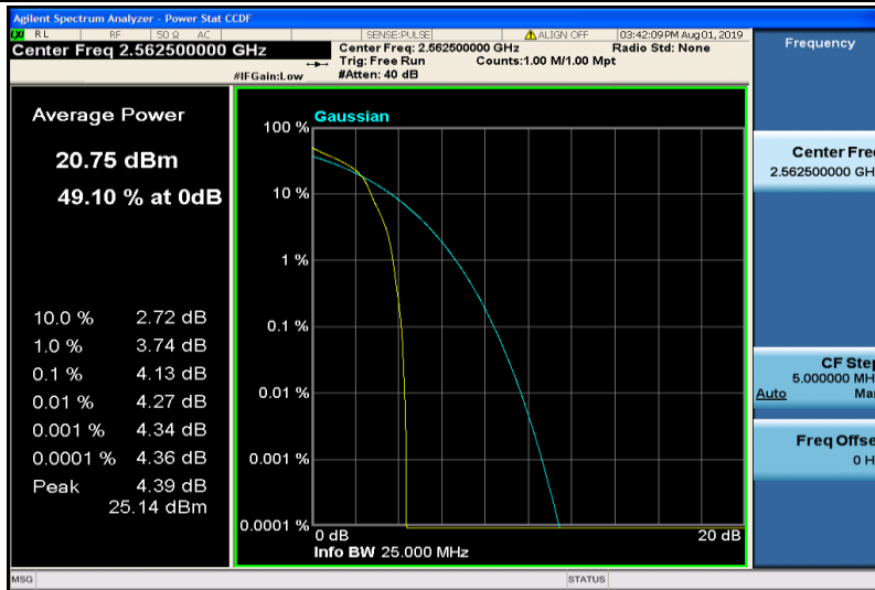
Band7-15MHz-16QAM-21375-1RB#0
