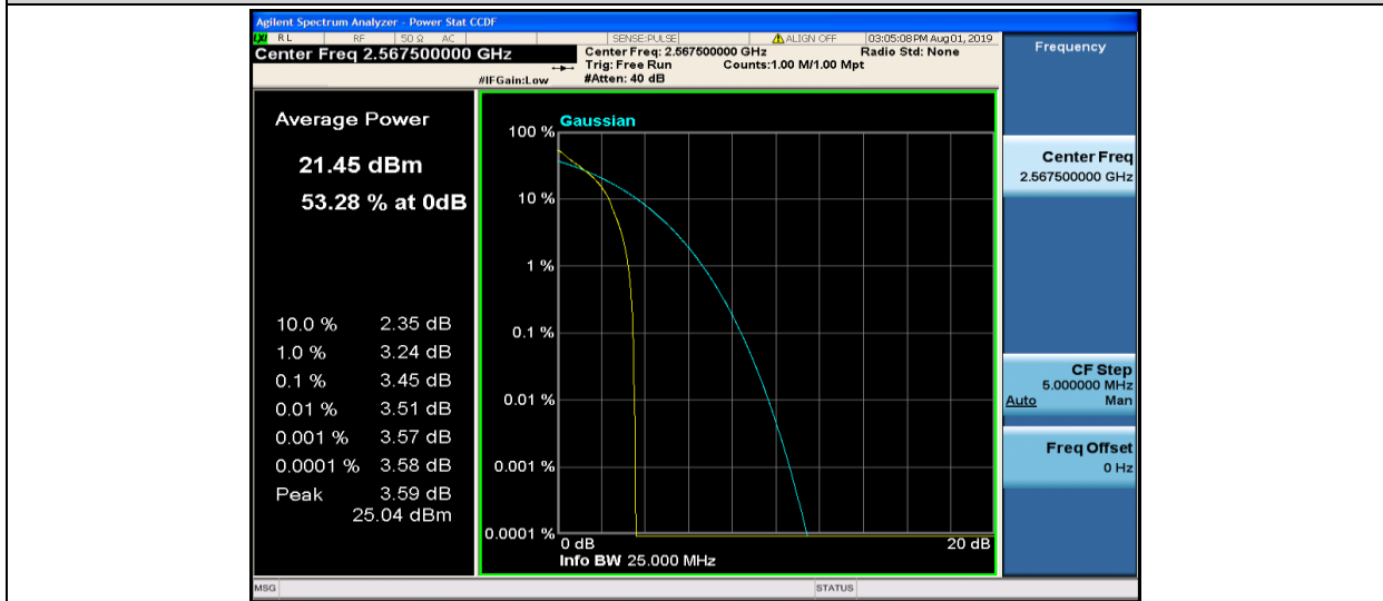
Band7-5MHz-QPSK-21425-1RB#0
