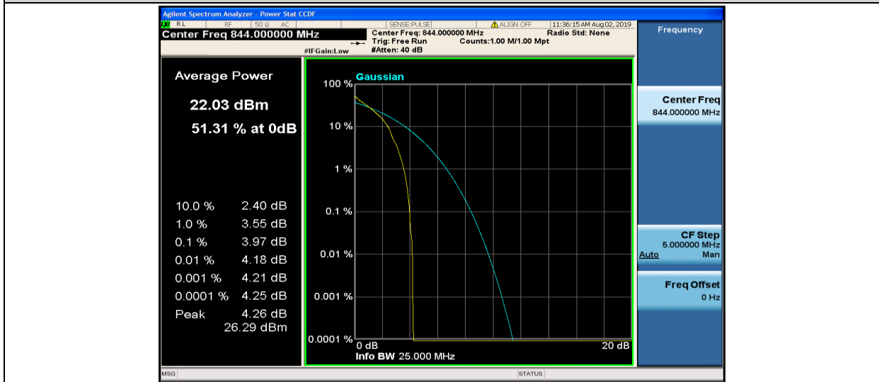
Band5-10MHz-QPSK-20600-1RB#0
