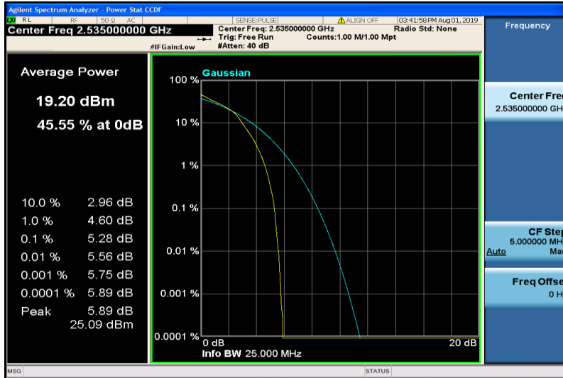
Band7-15MHz-16QAM-21100-75RB#0
