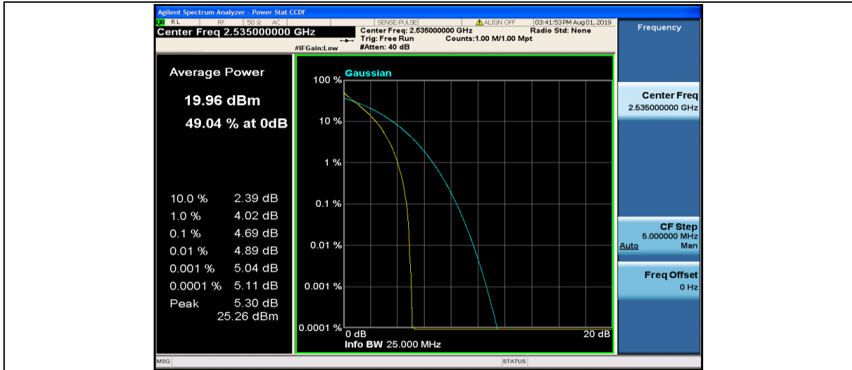
Band7-15MHz-QPSK-21100-75RB#0
