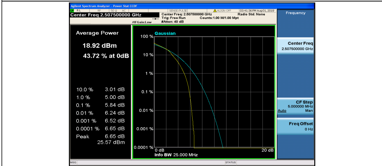
Band7-15MHz-16QAM-20825-75RB#0
