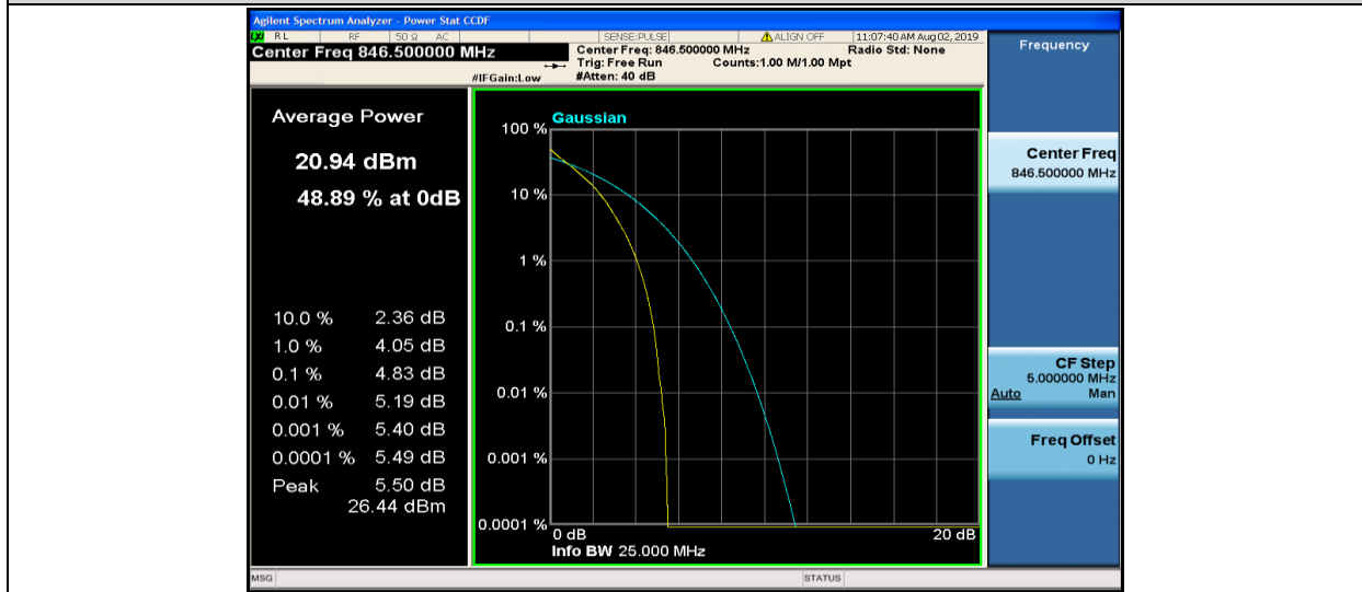
Band5-5MHz-QPSK-20625-25RB#0
