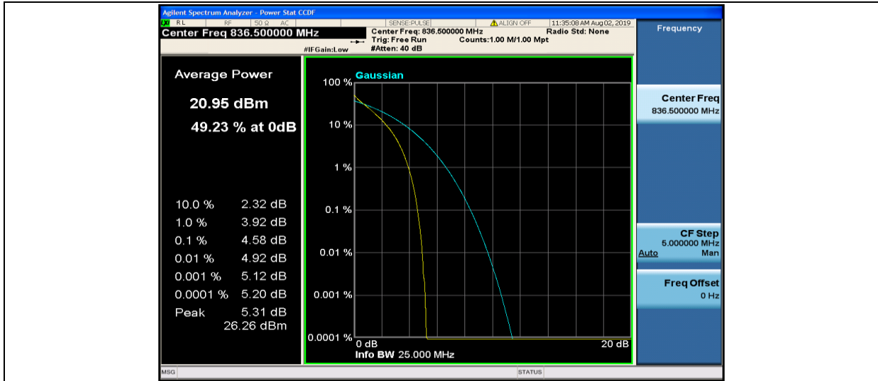
Band5-10MHz-QPSK-20525-50RB#0
