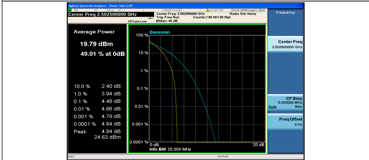
Band7-5MHz-QPSK-20775-25RB#0
