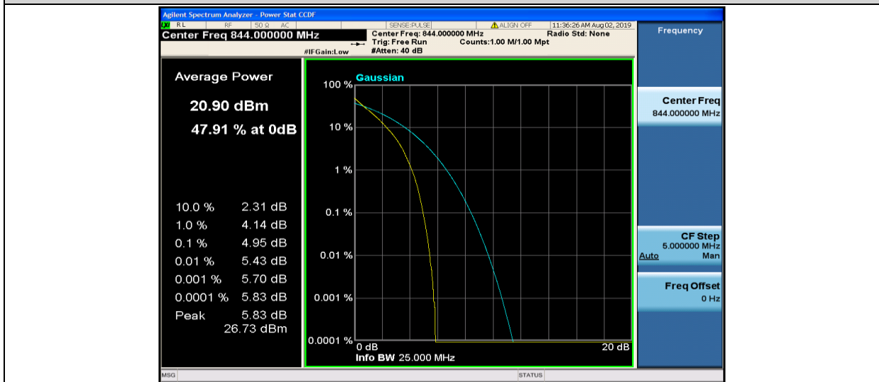
Band5-10MHz-QPSK-20600-50RB#0
