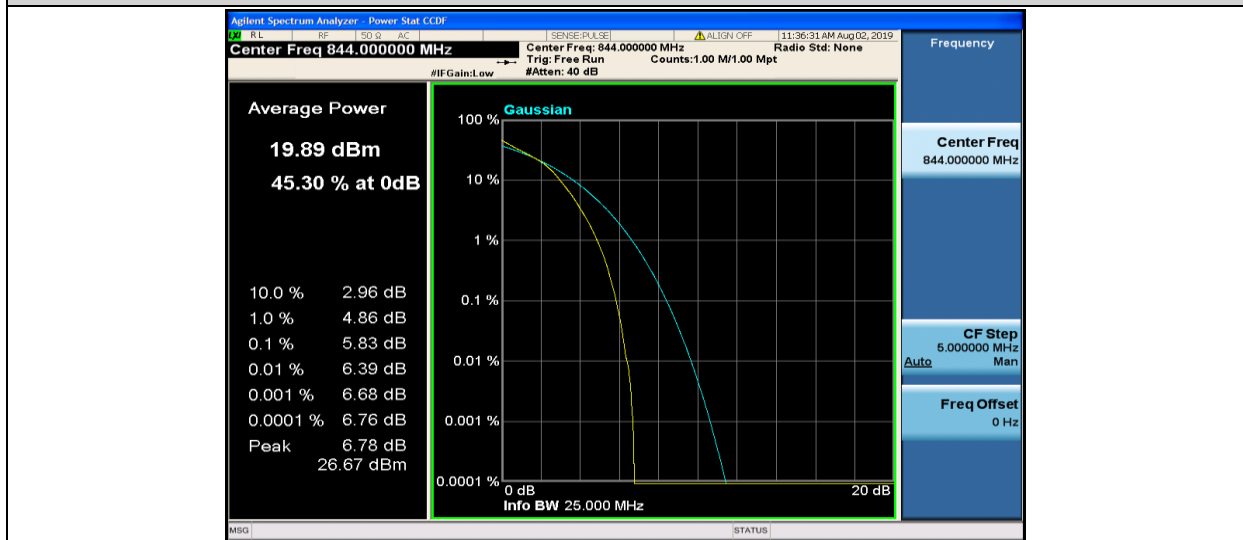
Band5-10MHz-16QAM-20600-50RB#0
