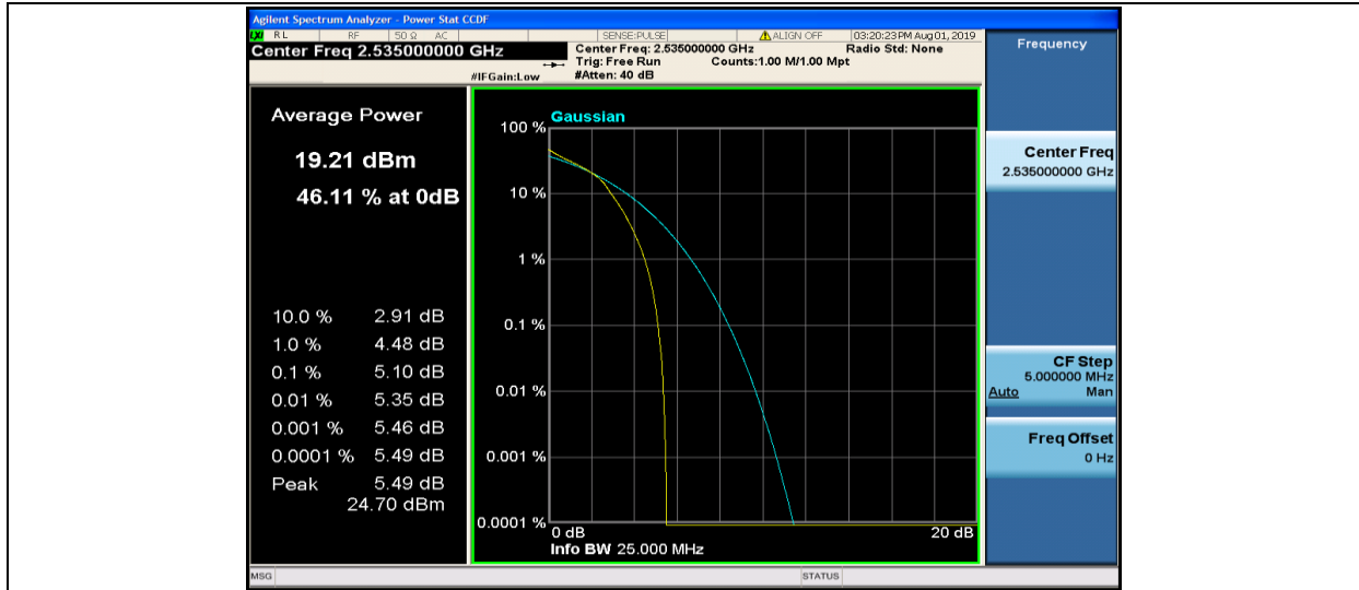
Band7-10MHz-16QAM-21100-50RB#0
