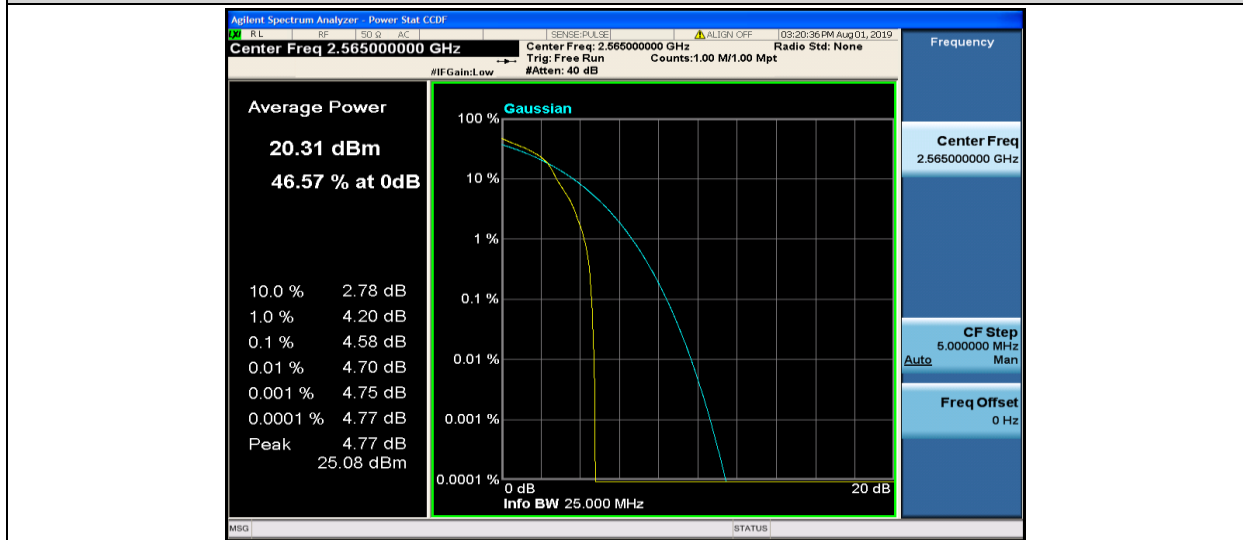
Band7-10MHz-16QAM-21400-1RB#0
