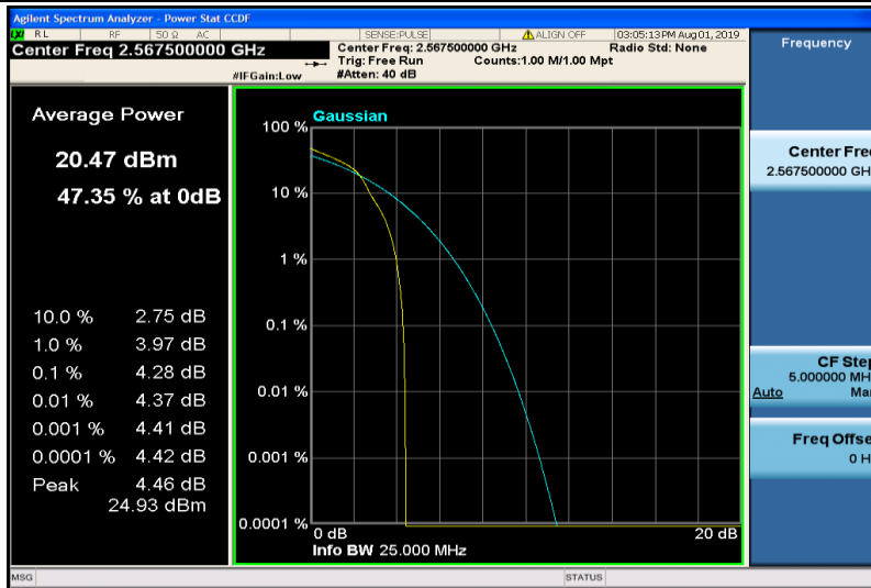
Band7-5MHz-16QAM-21425-1RB#0
