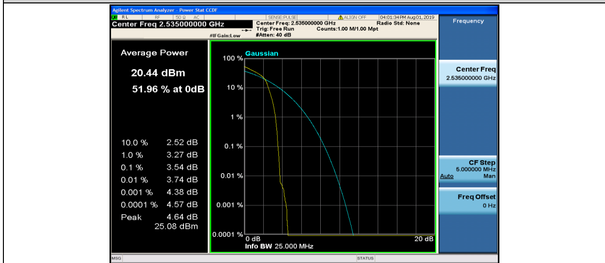
Band7-20MHz-16QAM-21100-1RB#0
