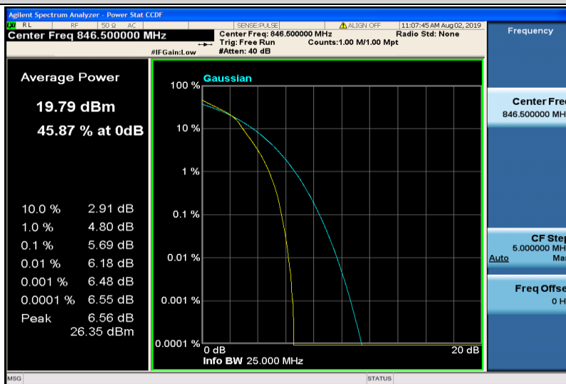
Band5-5MHz-16QAM-20625-25RB#0
