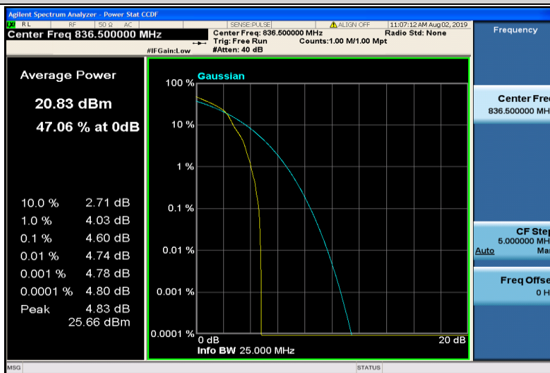
Band5-5MHz-16QAM-20525-1RB#0
