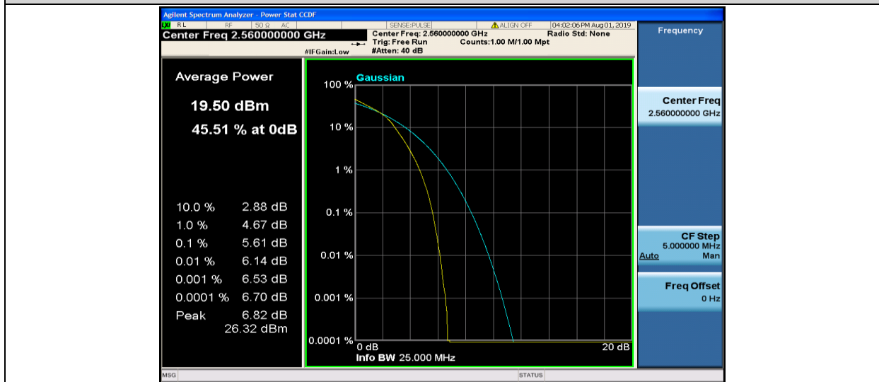
Band7-20MHz-16QAM-21350-100RB#0
