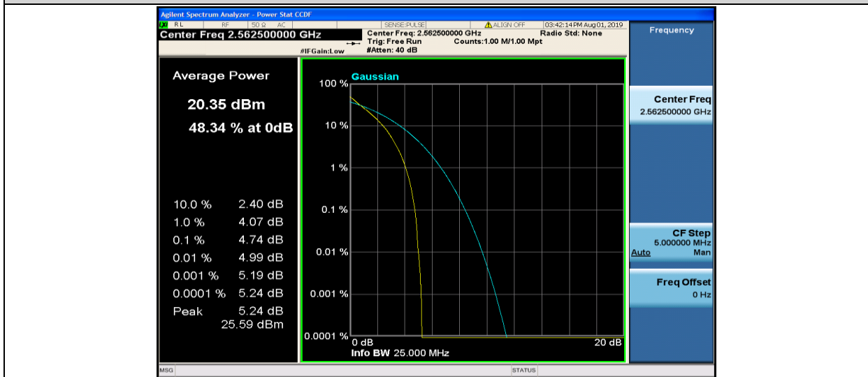
Band7-15MHz-QPSK-21375-75RB#0
