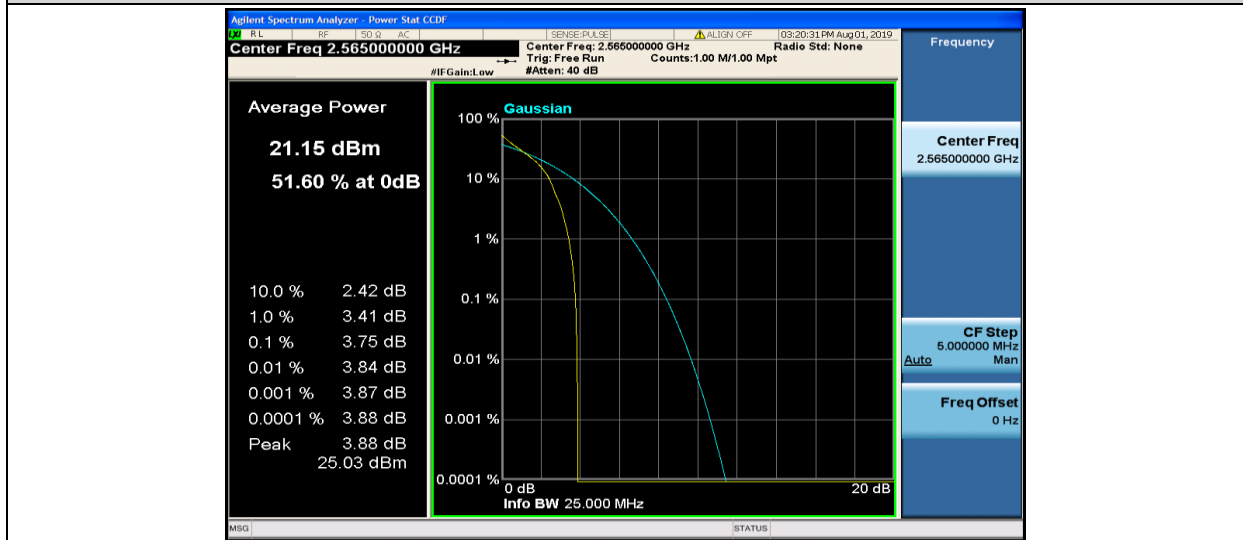
Band7-10MHz-QPSK-21400-1RB#0
