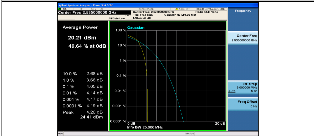
Band7-10MHz-16QAM-21100-1RB#0
