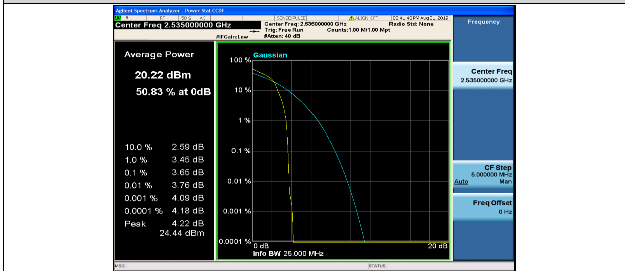
Band7-15MHz-16QAM-21100-1RB#0
