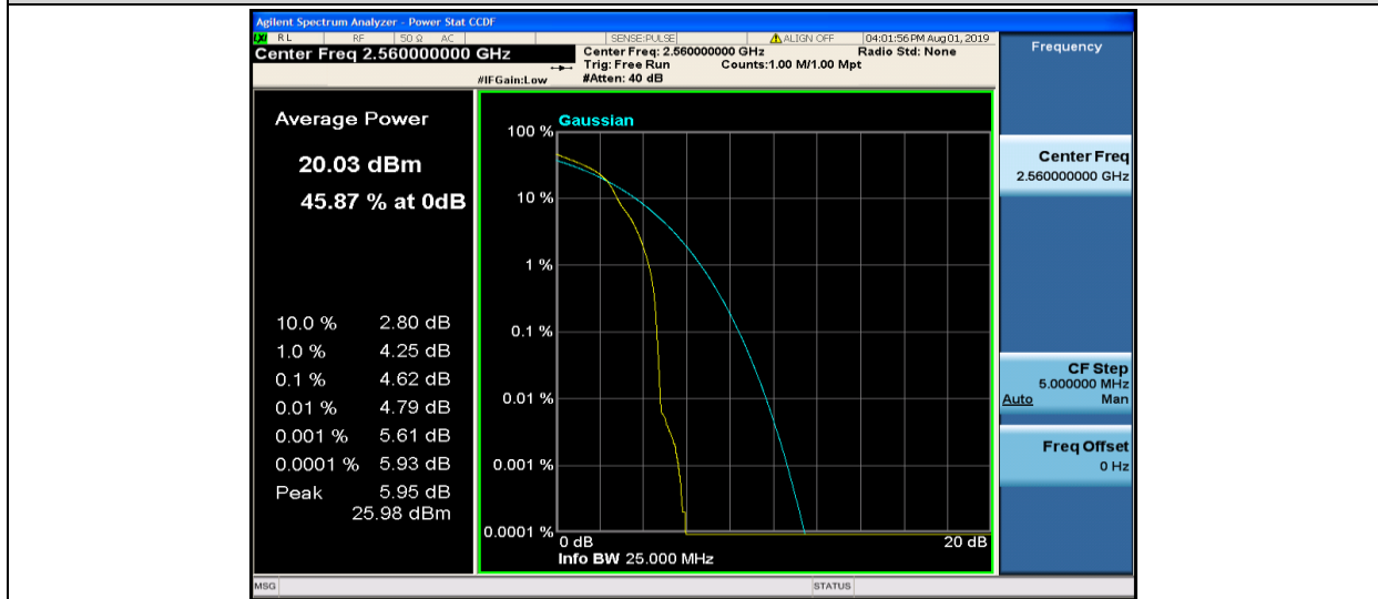
Band7-20MHz-16QAM-21350-1RB#0
