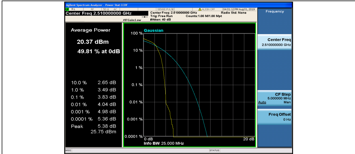
Band7-20MHz-16QAM-20850-1RB#0
