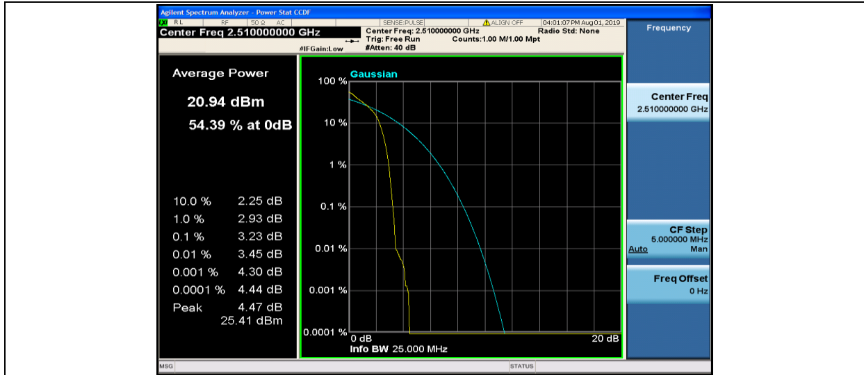
Band7-20MHz-QPSK-20850-1RB#0
