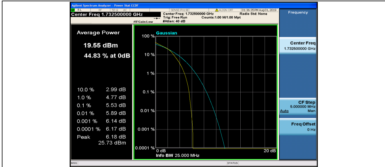
Band4-15MHz-16QAM-20175-75RB#0
