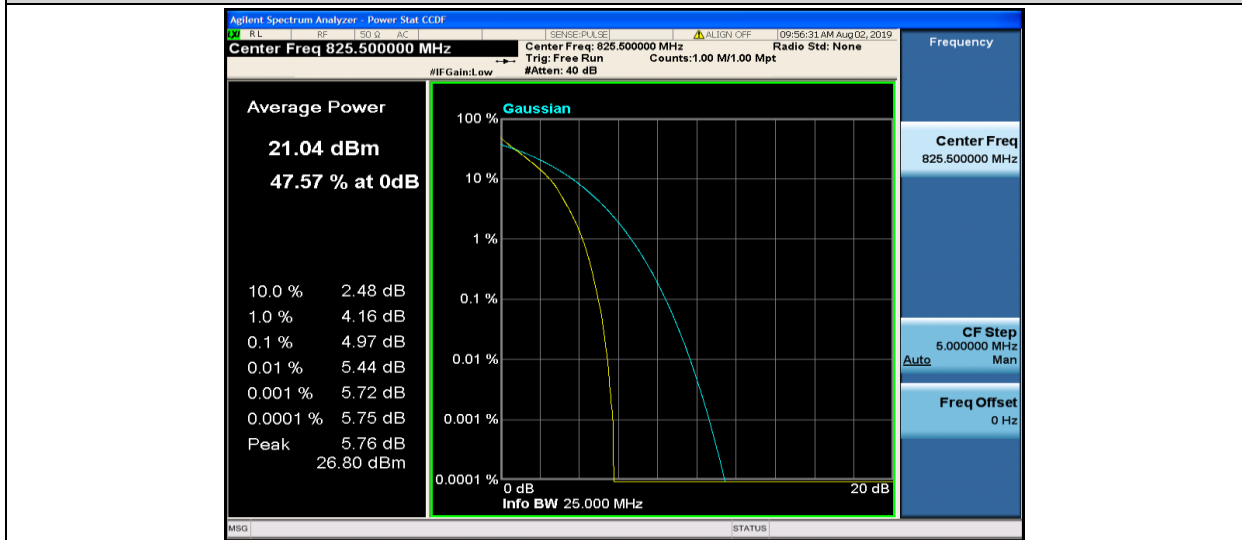
Band5-3MHz-QPSK-20415-15RB#0
