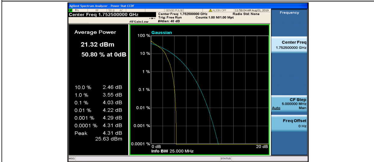
Band4-5MHz-QPSK-20375-1RB#0
