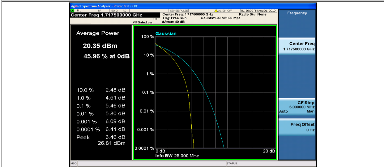
Band4-15MHz-QPSK-20025-75RB#0
