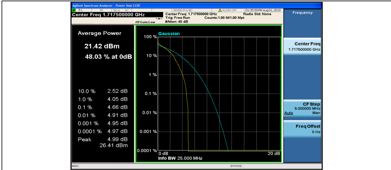
Band4-15MHz-QPSK-20025-1RB#0
