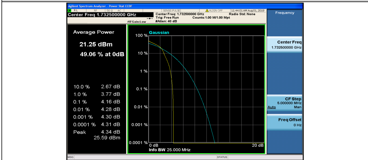
Band4-3MHz-16QAM-20175-1RB#0
