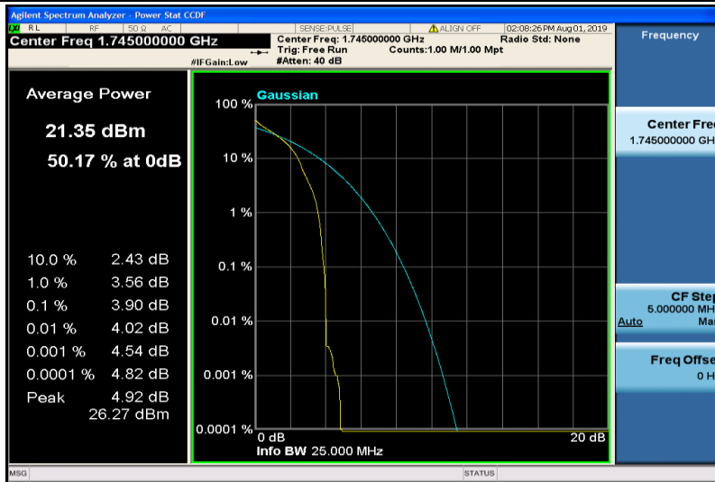
Band4-20MHz-QPSK-20300-1RB#0
