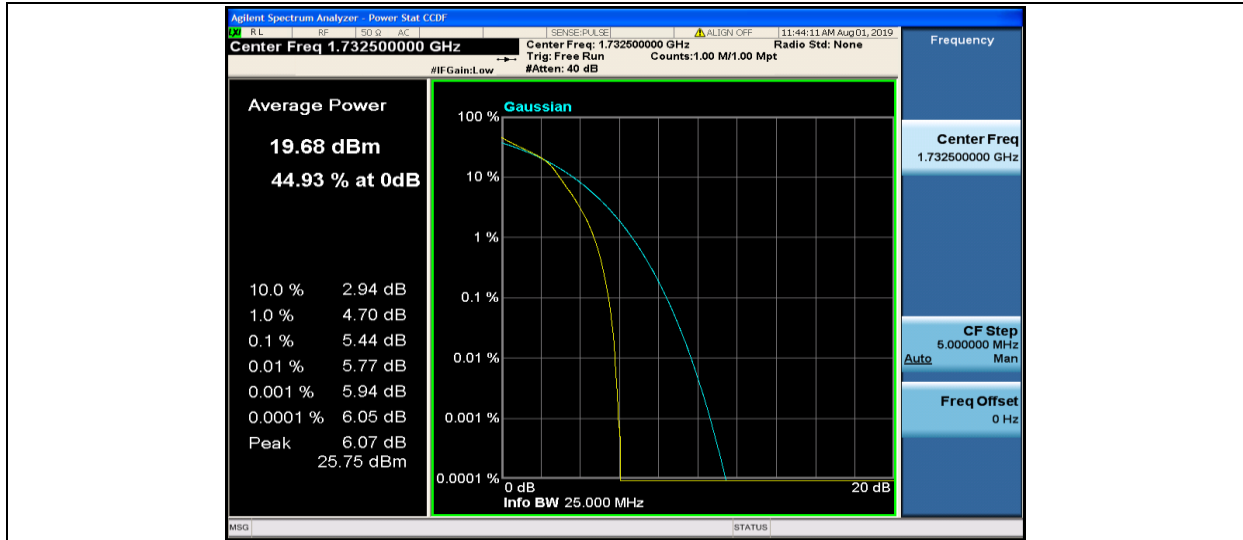
Band4-3MHz-16QAM-20175-15RB#0
