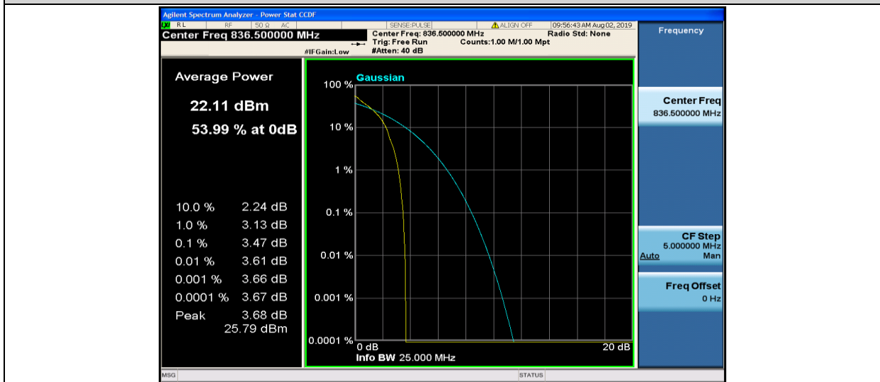
Band5-3MHz-QPSK-20525-1RB#0
