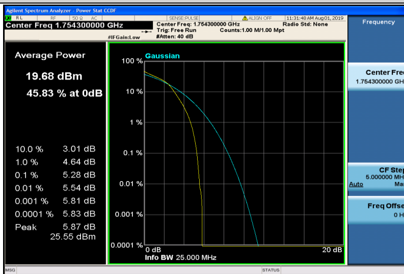
Band4-1.4MHz-16QAM-20393-6RB#0
