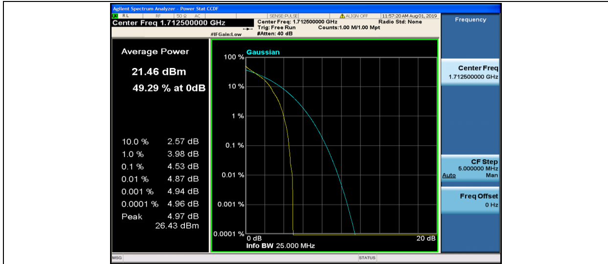
Band4-5MHz-QPSK-19975-1RB#0
