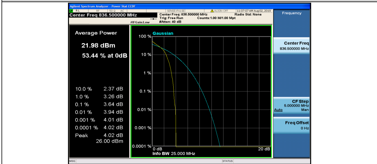
Band5-5MHz-QPSK-20525-1RB#0
