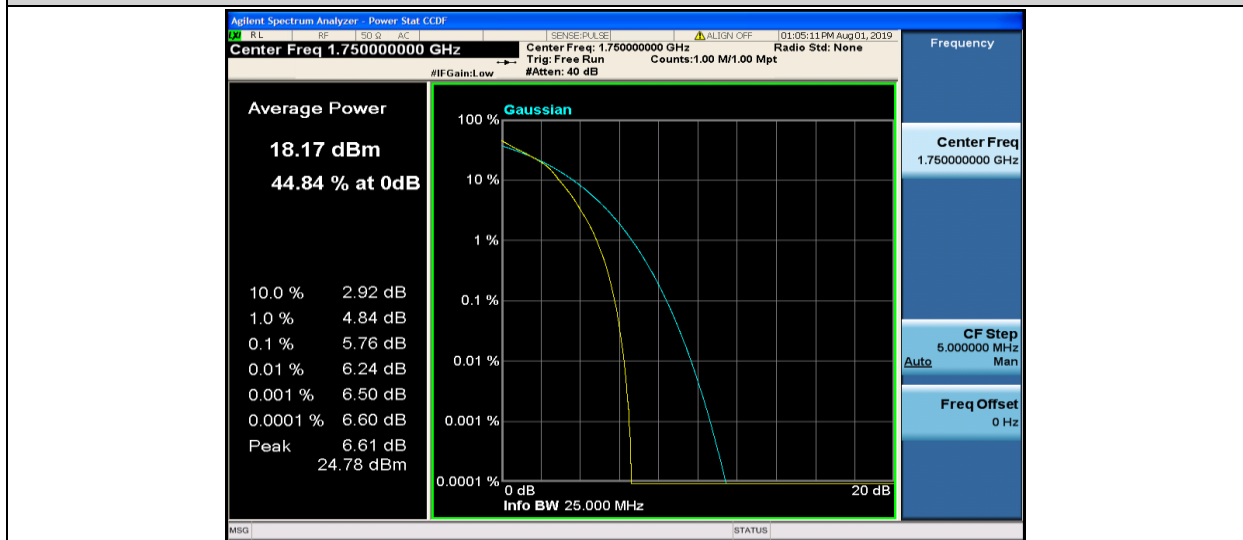
Band4-10MHz-16QAM-20350-50RB#0
