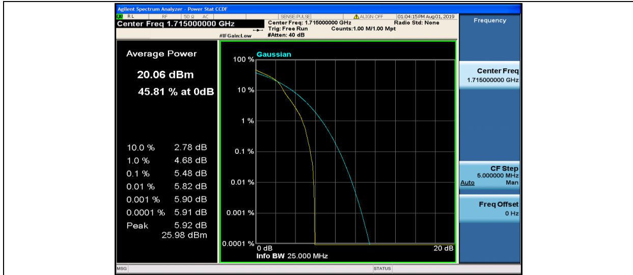
Band4-10MHz-16QAM-20000-1RB#0
