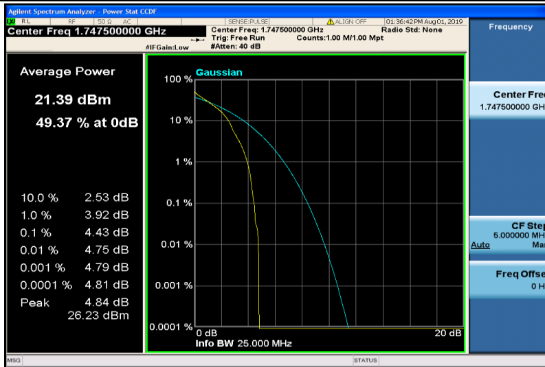
Band4-15MHz-QPSK-20325-1RB#0
