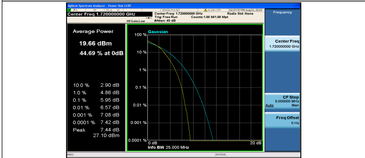
Band4-20MHz-16QAM-20050-100RB#0
