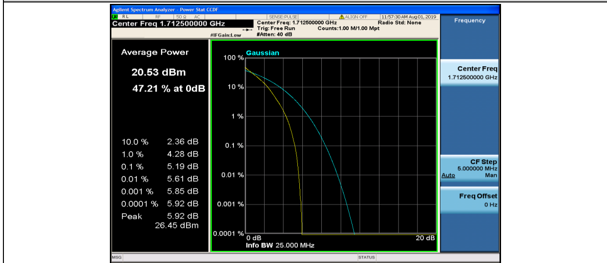
Band4-5MHz-QPSK-19975-25RB#0
