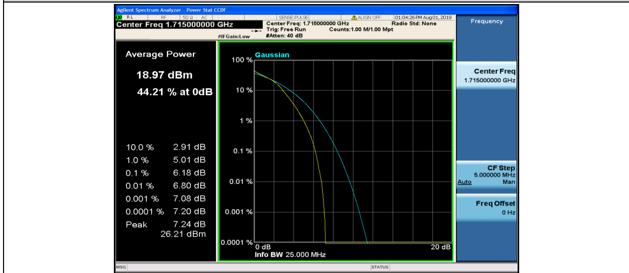
Band4-10MHz-16QAM-20000-50RB#0
