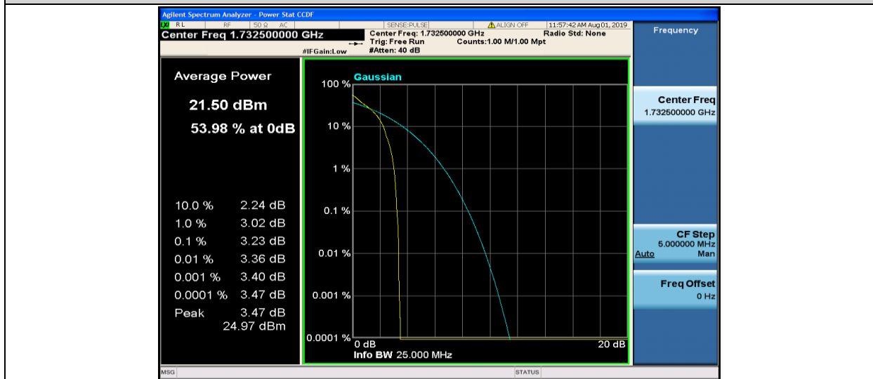
Band4-5MHz-QPSK-20175-1RB#0
