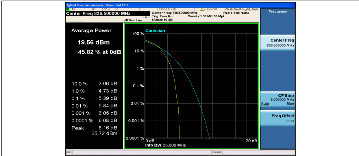
Band5-1.4MHz-16QAM-20525-6RB#0
