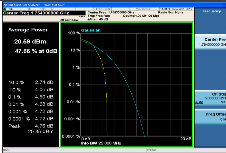
Band4-1.4MHz-16QAM-20393-1RB#0
