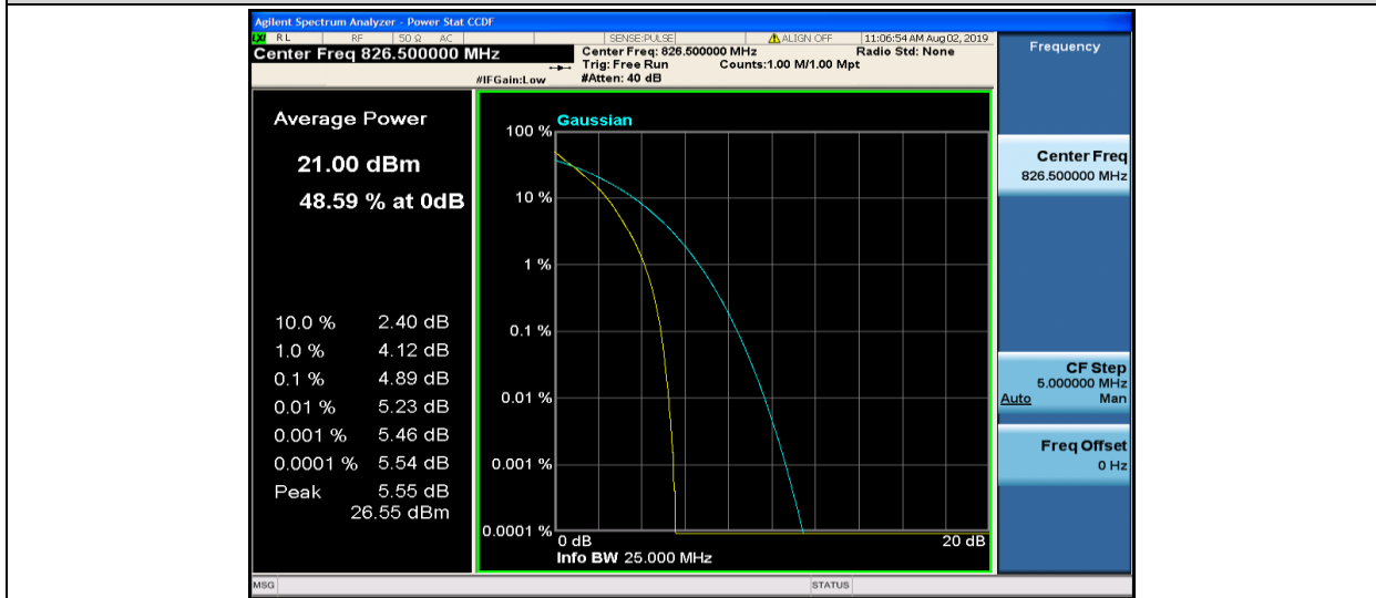
Band5-5MHz-QPSK-20425-25RB#0
