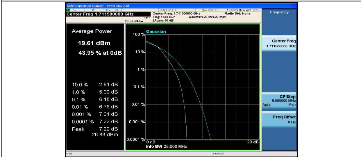
Band4-3MHz-16QAM-19965-15RB#0
