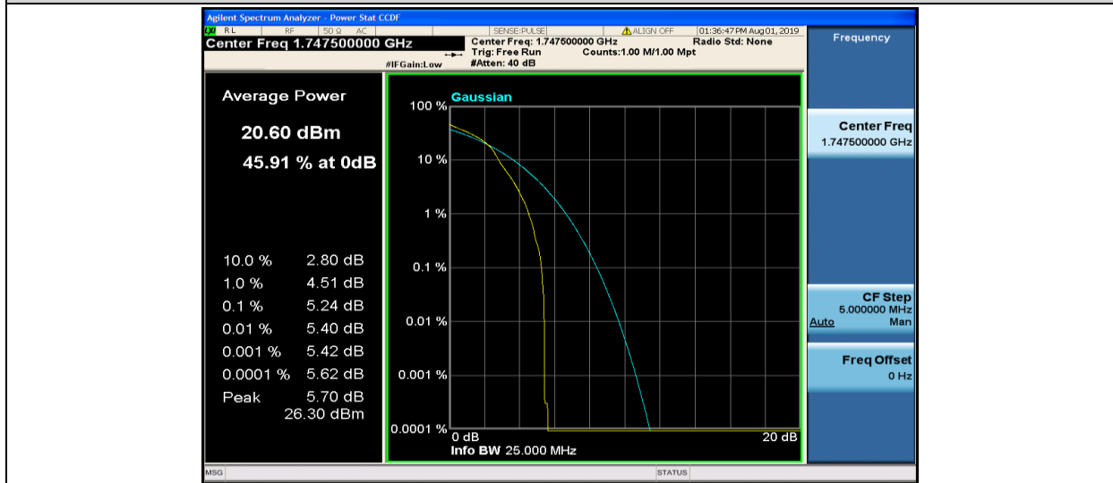
Band4-15MHz-16QAM-20325-1RB#0
