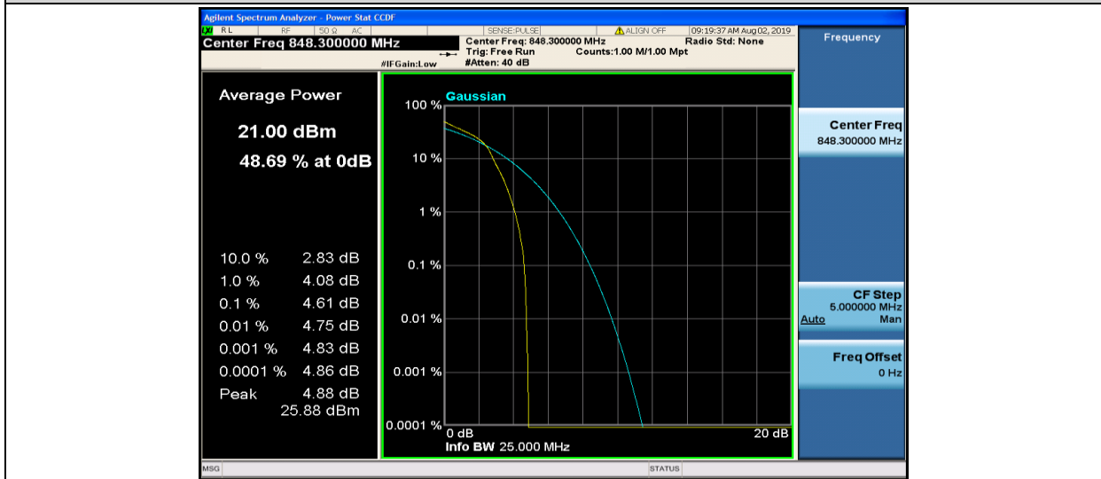
Band5-1.4MHz-16QAM-20643-1RB#0
