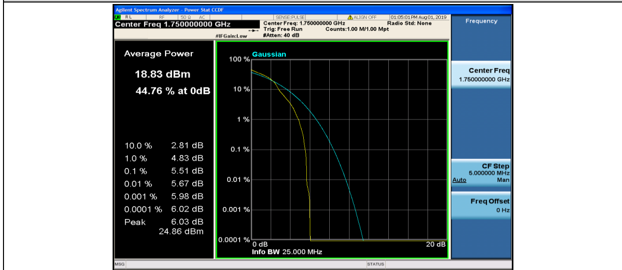
Band4-10MHz-16QAM-20350-1RB#0
