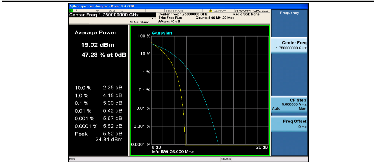
Band4-10MHz-QPSK-20350-50RB#0
