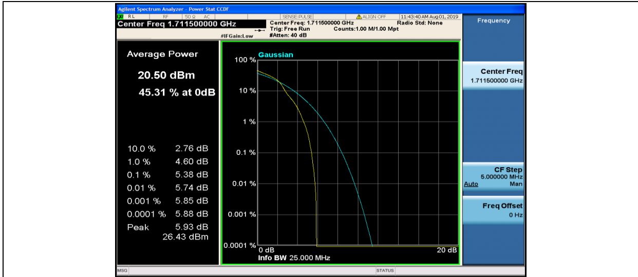
Band4-3MHz-16QAM-19965-1RB#0
