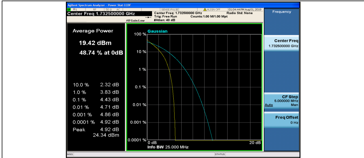
Band4-10MHz-QPSK-20175-50RB#0
