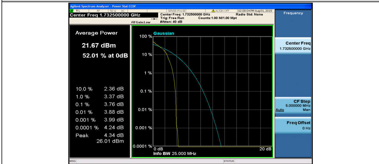
Band4-20MHz-QPSK-20175-1RB#0
