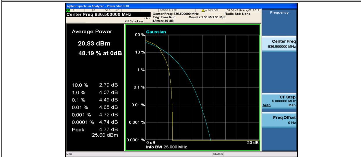
Band5-3MHz-16QAM-20525-1RB#0
