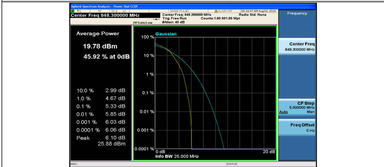
Band5-1.4MHz-16QAM-20643-6RB#0
