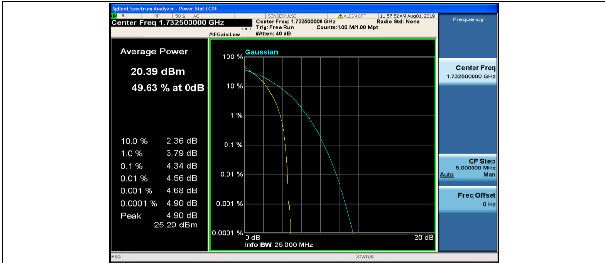
Band4-5MHz-QPSK-20175-25RB#0
