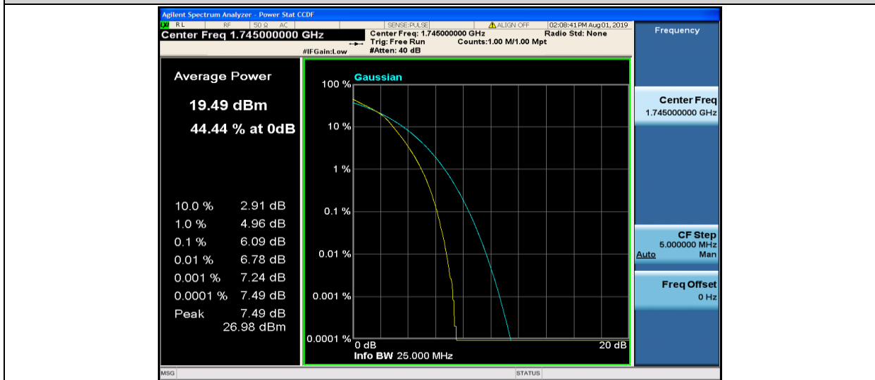
Band4-20MHz-16QAM-20300-100RB#0
