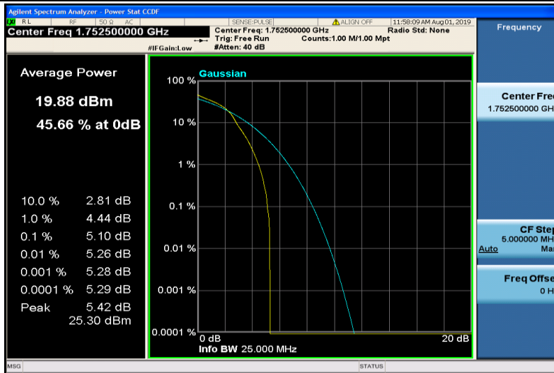
Band4-5MHz-16QAM-20375-1RB#0
