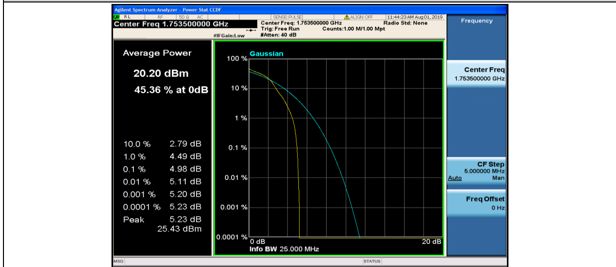
Band4-3MHz-16QAM-20385-1RB#0
