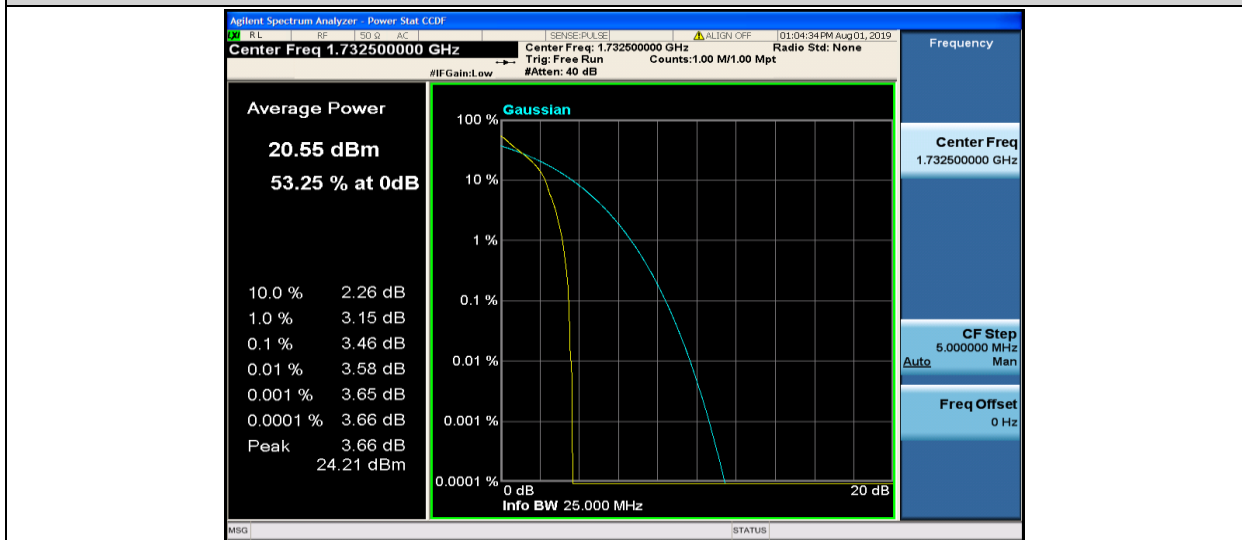
Band4-10MHz-QPSK-20175-1RB#0
