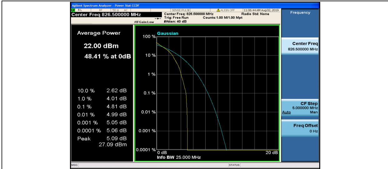
Band5-5MHz-QPSK-20425-1RB#0
