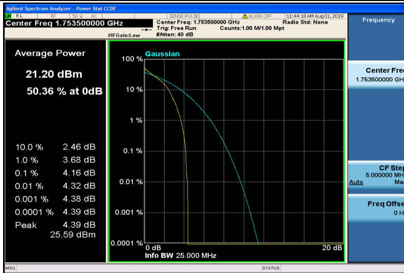
Band4-3MHz-QPSK-20385-1RB#0
