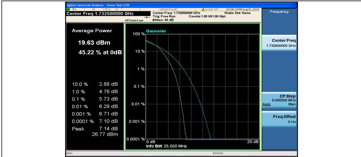
Band4-20MHz-16QAM-20175-100RB#0
