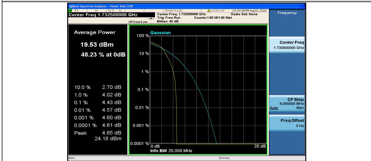
Band4-10MHz-16QAM-20175-1RB#0
