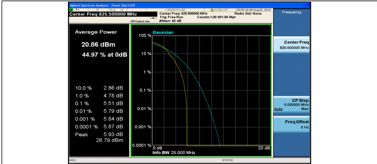
Band5-3MHz-16QAM-20415-1RB#0
