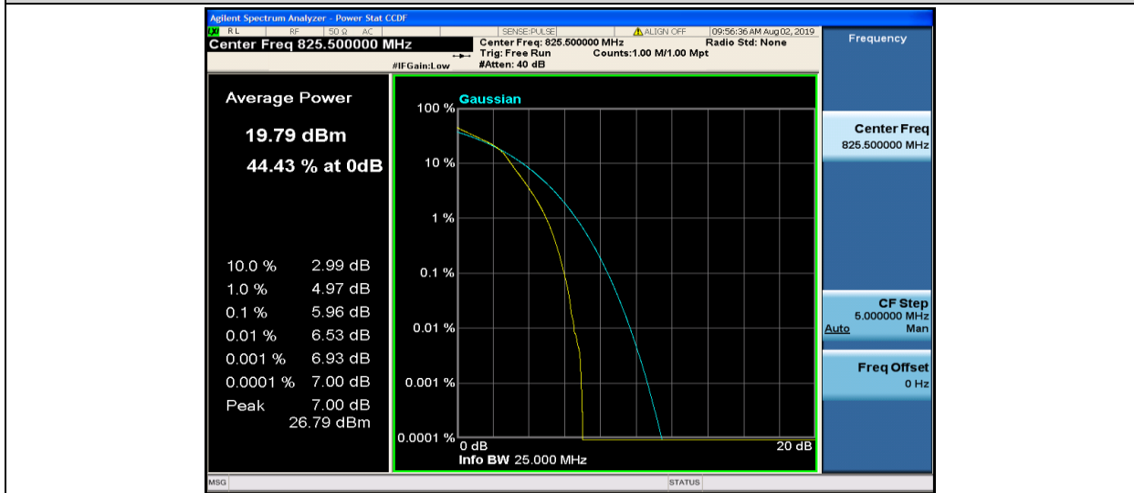
Band5-3MHz-16QAM-20415-15RB#0
