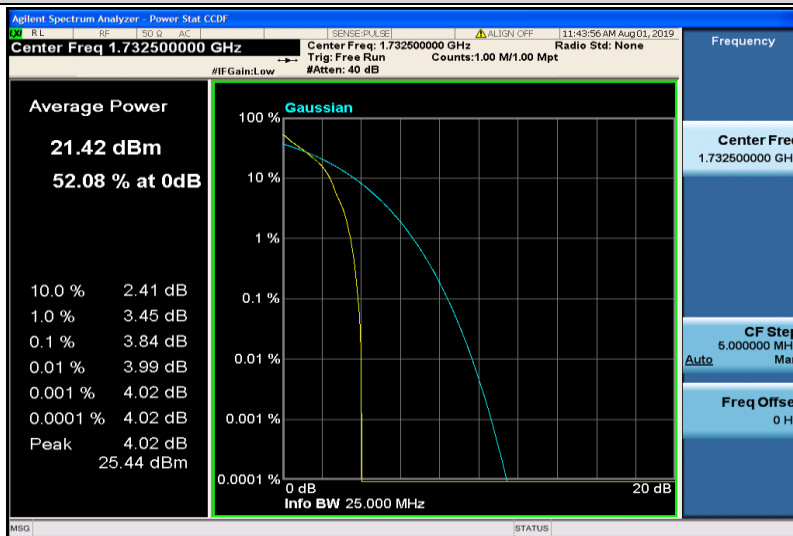
Band4-3MHz-QPSK-20175-1RB#0
