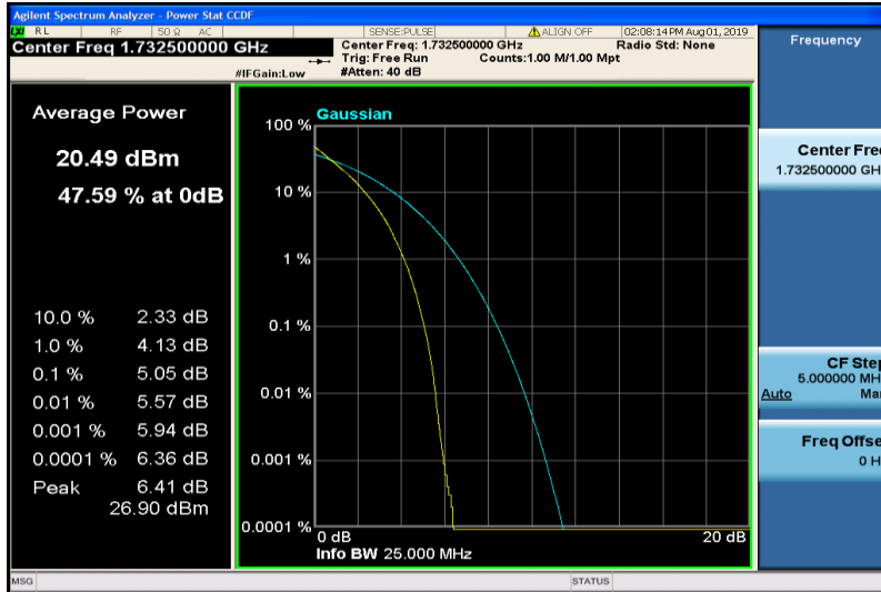
Band4-20MHz-QPSK-20175-100RB#0
