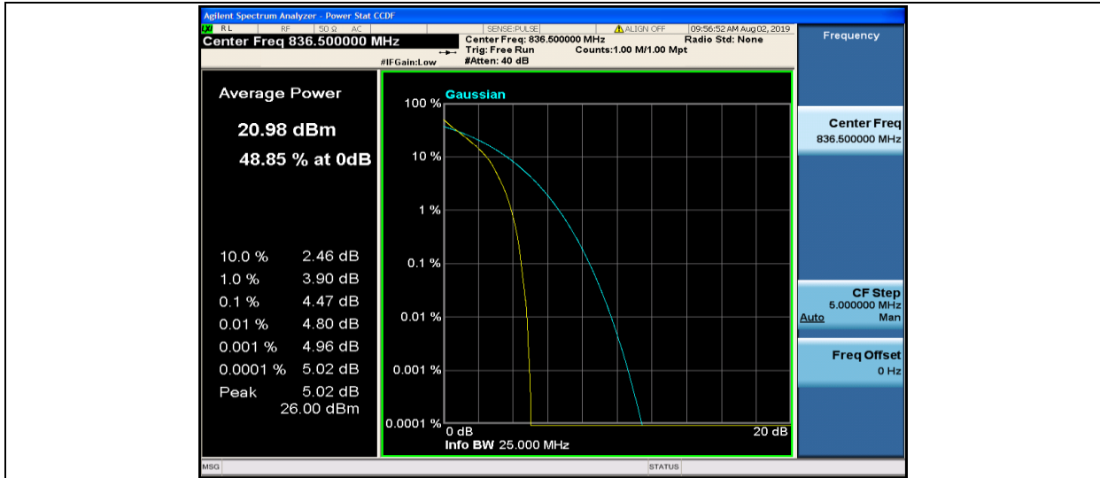
Band5-3MHz-QPSK-20525-15RB#0
