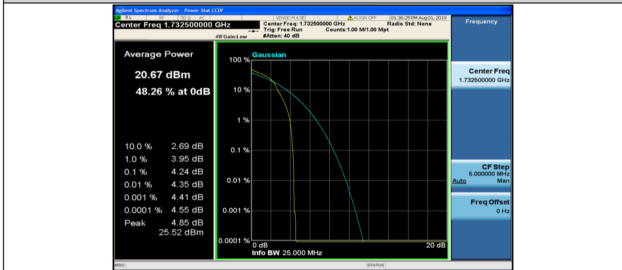
Band4-15MHz-16QAM-20175-1RB#0
