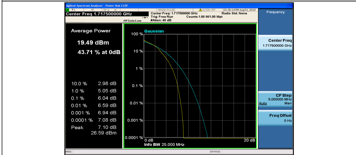
Band4-15MHz-16QAM-20025-75RB#0
