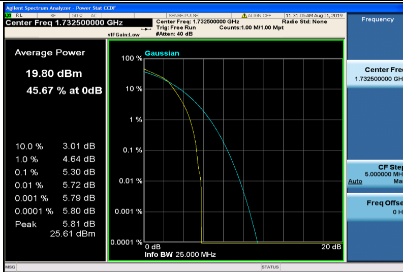
Band4-1.4MHz-16QAM-20175-6RB#0
