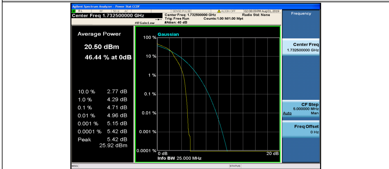
Band4-20MHz-16QAM-20175-1RB#0
