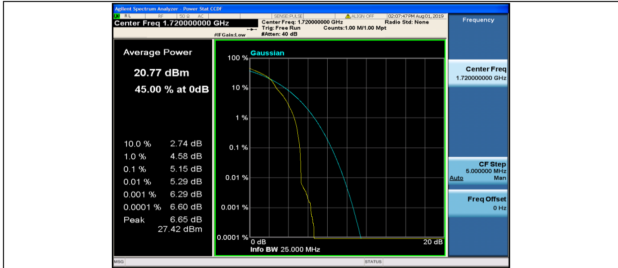
Band4-20MHz-16QAM-20050-1RB#0
