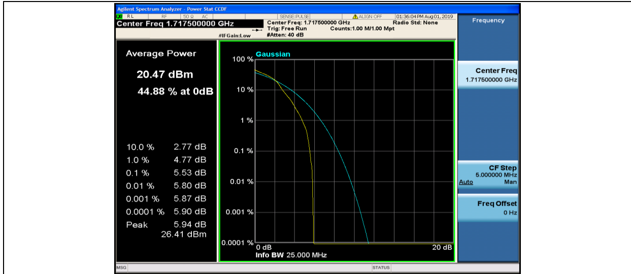
Band4-15MHz-16QAM-20025-1RB#0
