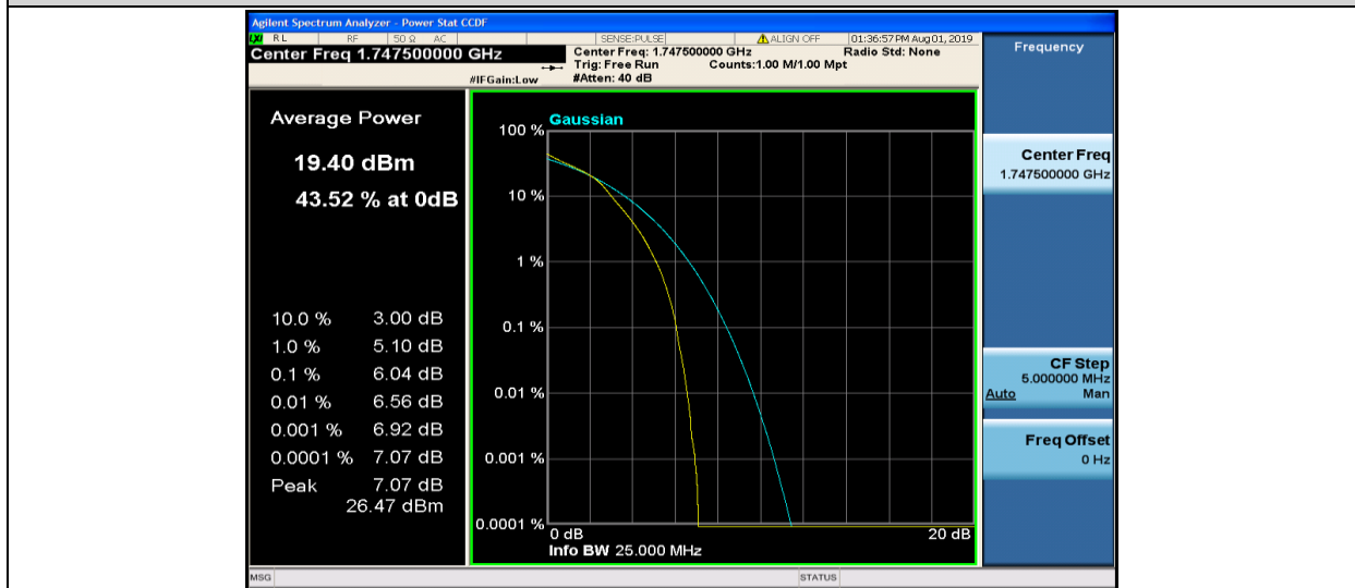
Band4-15MHz-16QAM-20325-75RB#0
