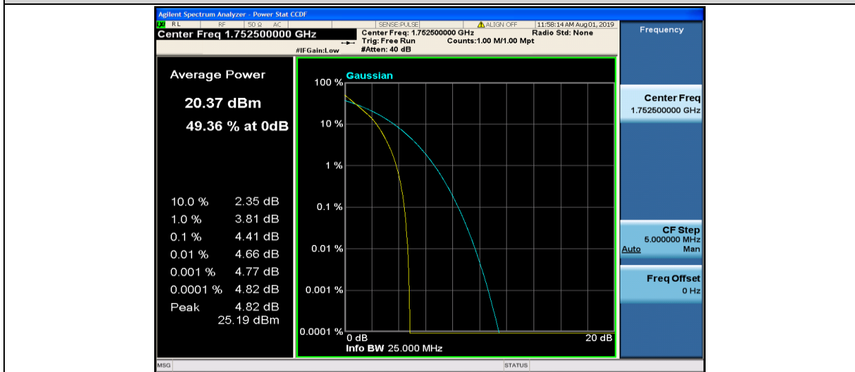
Band4-5MHz-QPSK-20375-25RB#0
