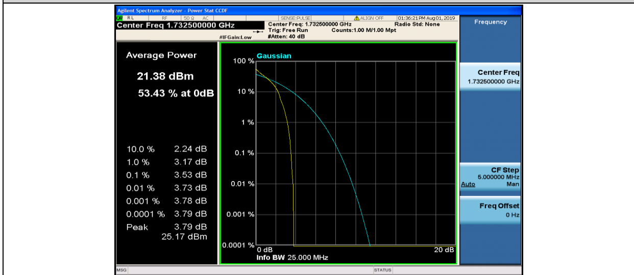
Band4-15MHz-QPSK-20175-1RB#0
