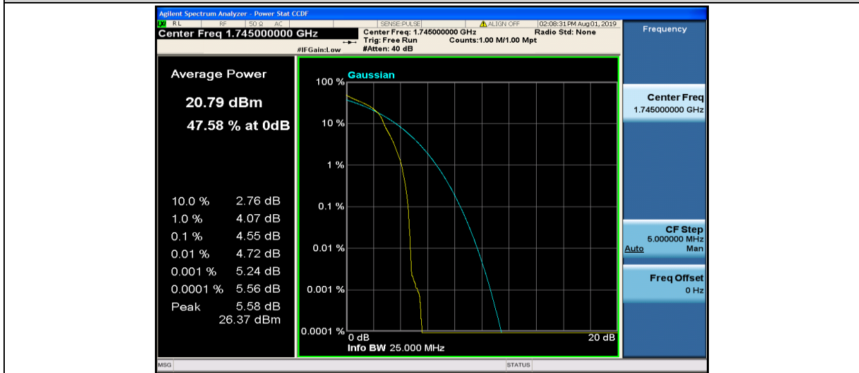
Band4-20MHz-16QAM-20300-1RB#0
