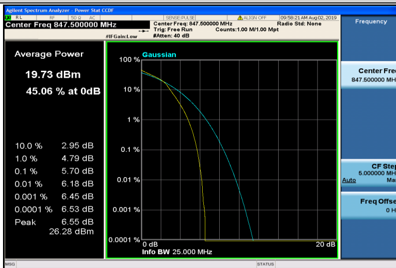
Band5-3MHz-16QAM-20635-15RB#0
