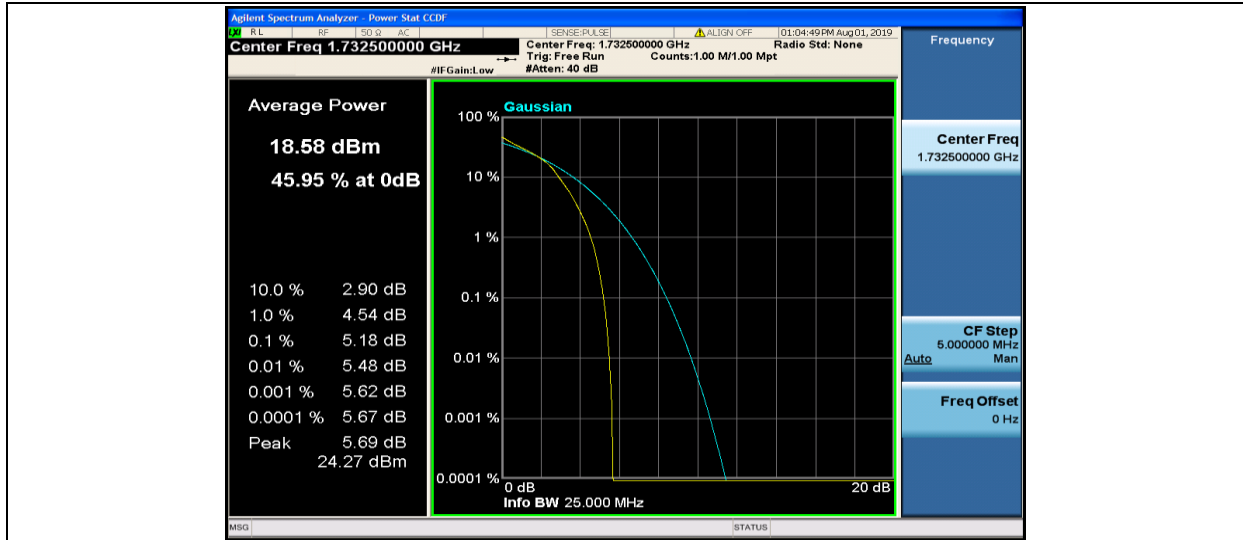
Band4-10MHz-16QAM-20175-50RB#0
