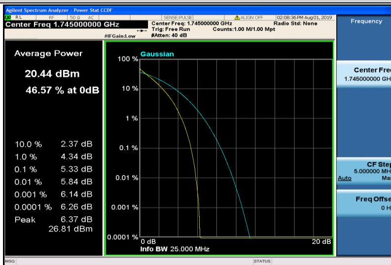
Band4-20MHz-QPSK-20300-100RB#0
