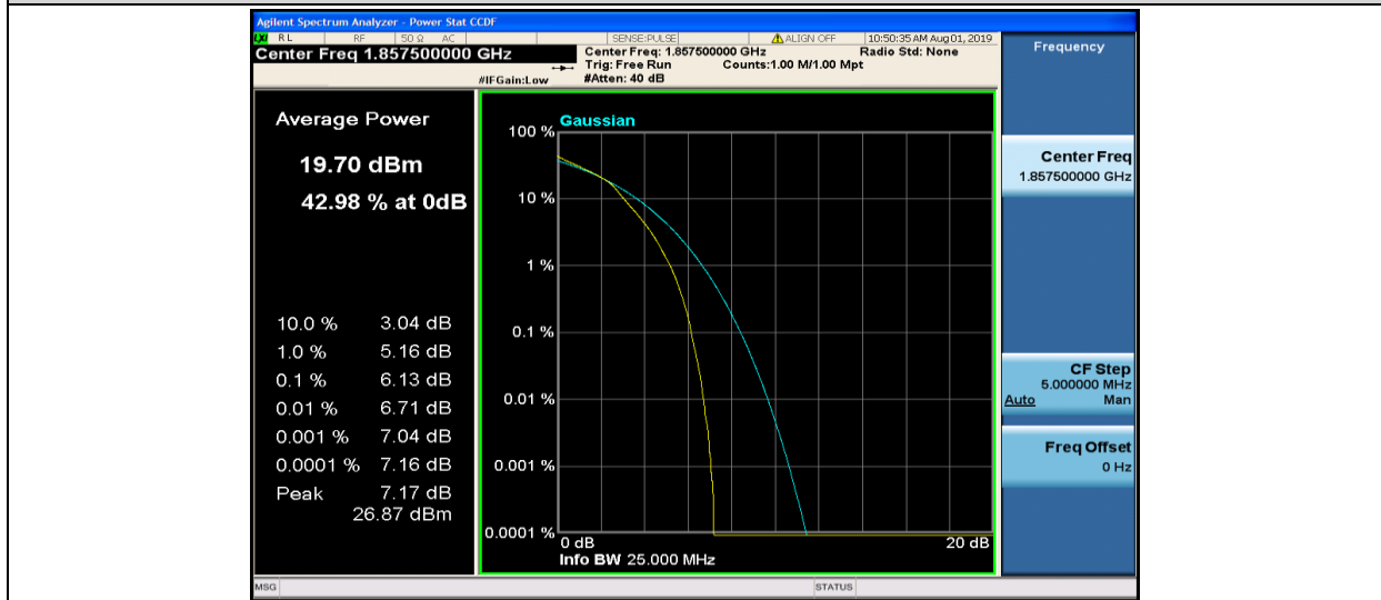
Band2-15MHz-16QAM-18675-75RB#0
