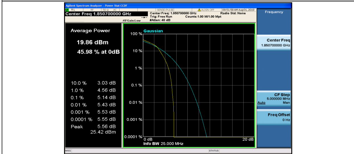
Band2-1.4MHz-16QAM-18607-6RB#0
