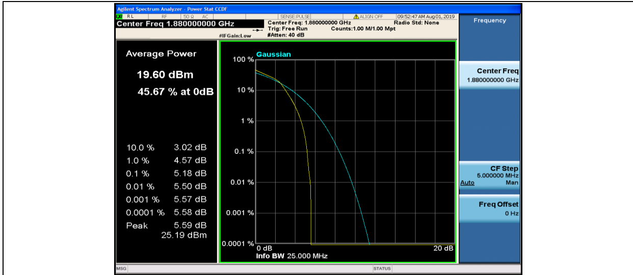
Band2-1.4MHz-16QAM-18900-6RB#0
