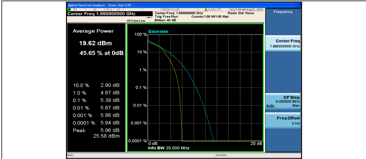
Band2-5MHz-16QAM-18900-25RB#0
