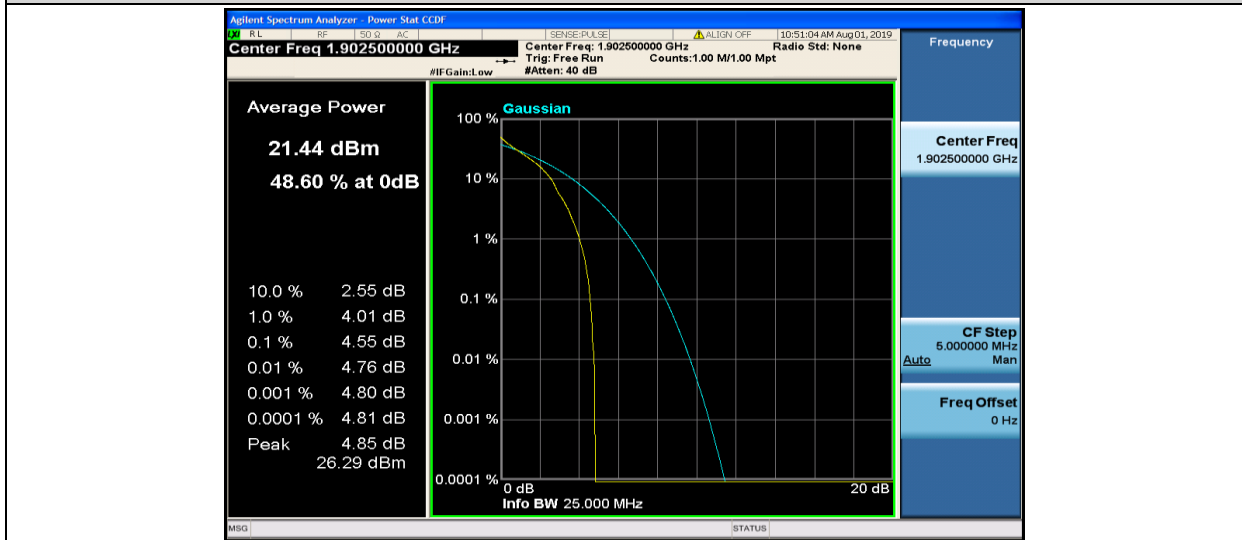
Band2-15MHz-QPSK-19125-1RB#0
