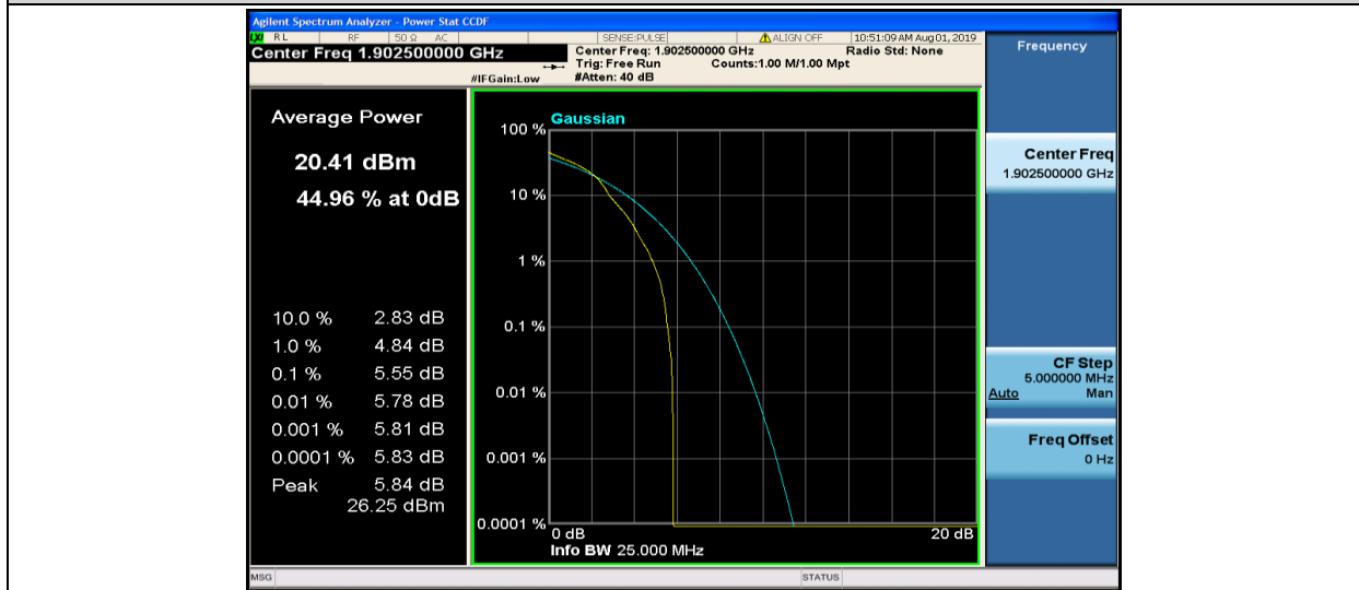
Band2-15MHz-16QAM-19125-1RB#0
