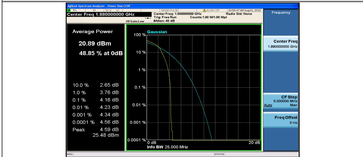
Band2-15MHz-16QAM-18900-1RB#0
