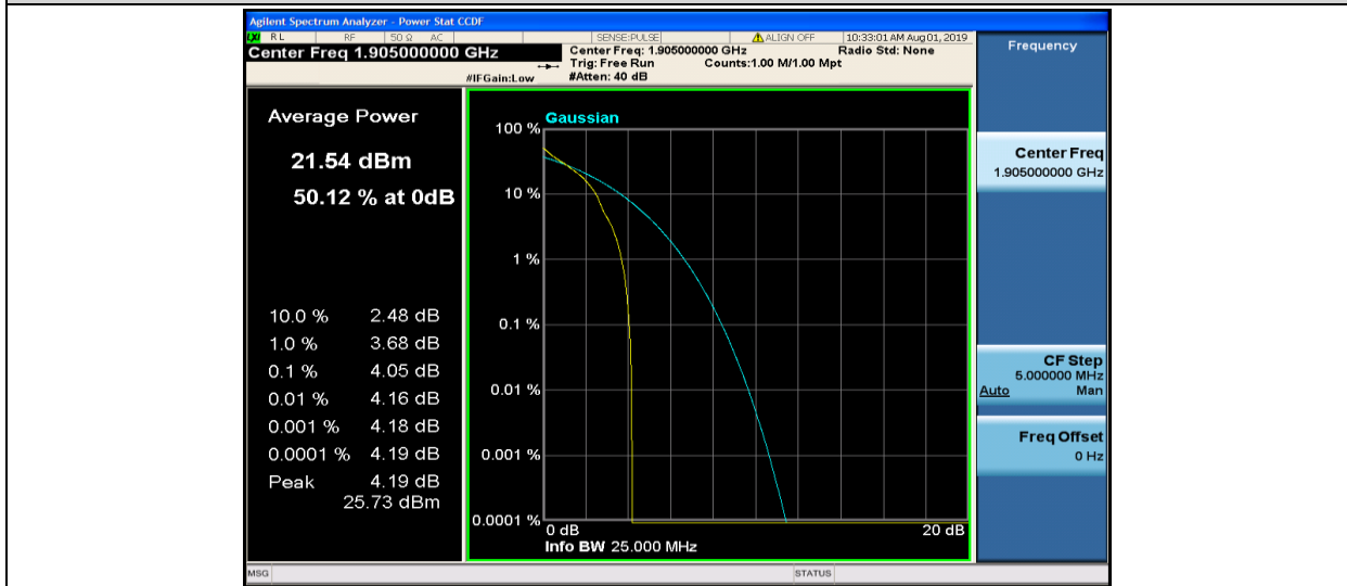
Band2-10MHz-QPSK-19150-1RB#0
