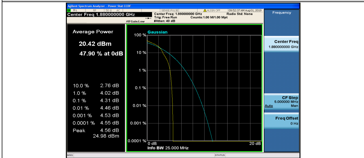
Band2-1.4MHz-16QAM-18900-1RB#0
