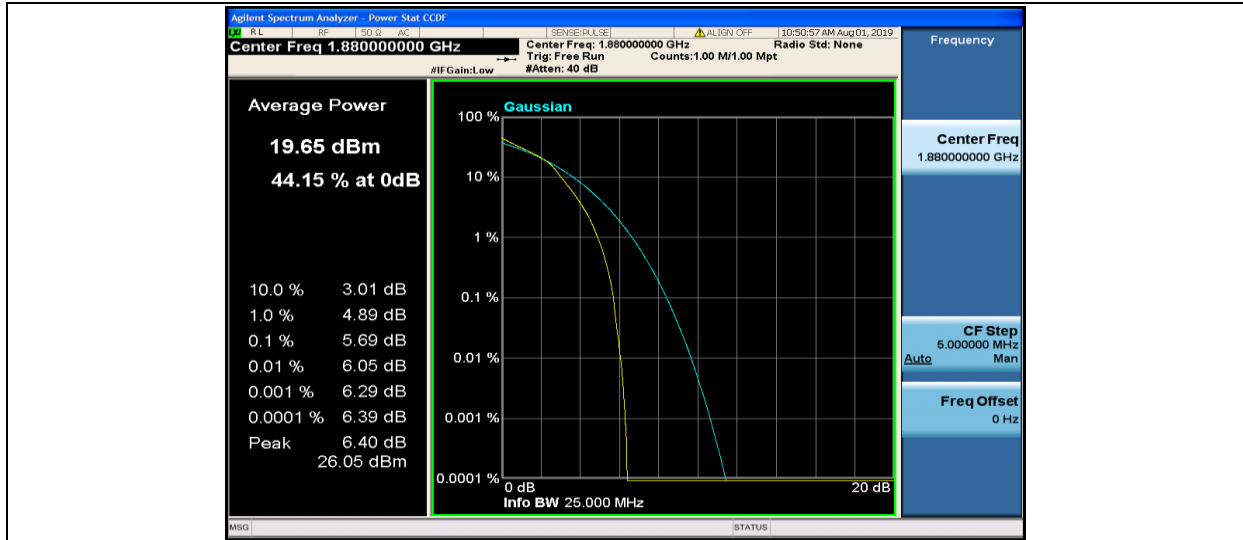
Band2-15MHz-16QAM-18900-75RB#0
