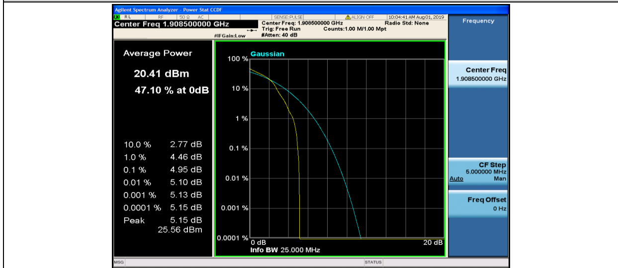
Band2-3MHz-16QAM-19185-1RB#0
