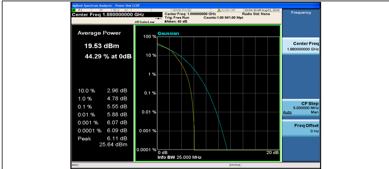
Band2-3MHz-16QAM-18900-15RB#0
