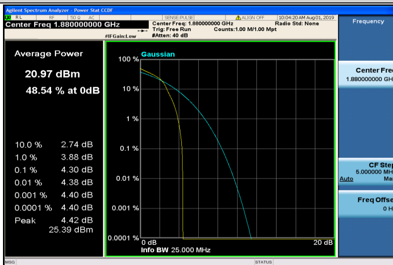
Band2-3MHz-16QAM-18900-1RB#0
