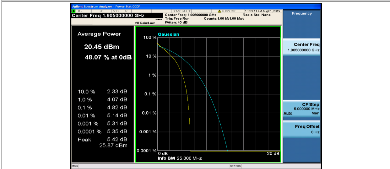
Band2-10MHz-QPSK-19150-50RB#0
