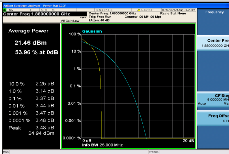
Band2-1.4MHz-QPSK-18900-1RB#0
