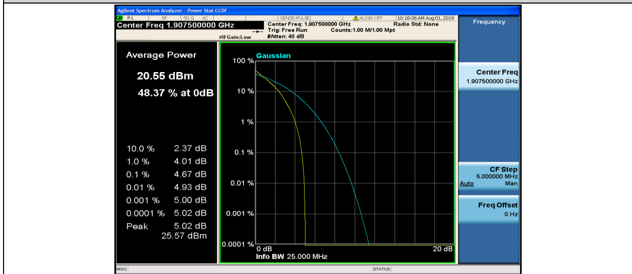
Band2-5MHz-QPSK-19175-25RB#0
