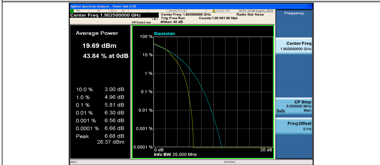
Band2-15MHz-16QAM-19125-75RB#0
