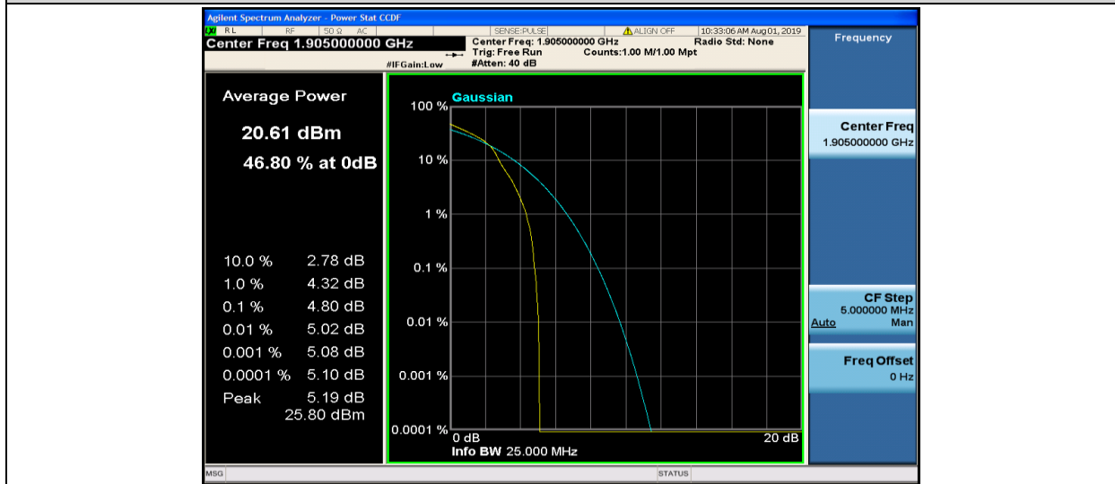
Band2-10MHz-16QAM-19150-1RB#0
