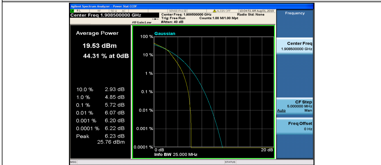
Band2-3MHz-16QAM-19185-15RB#0
