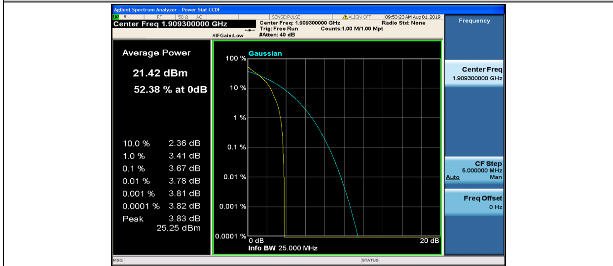
Band2-1.4MHz-QPSK-19193-1RB#0
