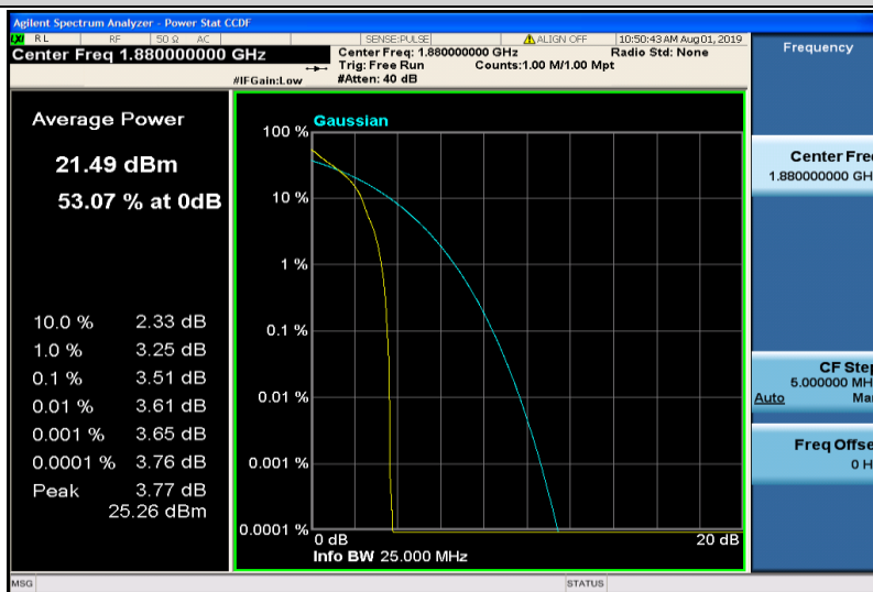
Band2-15MHz-QPSK-18900-1RB#0
