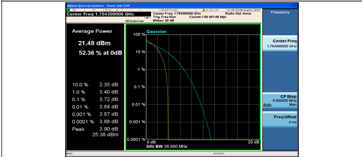
Band4-1.4MHz-QPSK-20393-1RB#0
