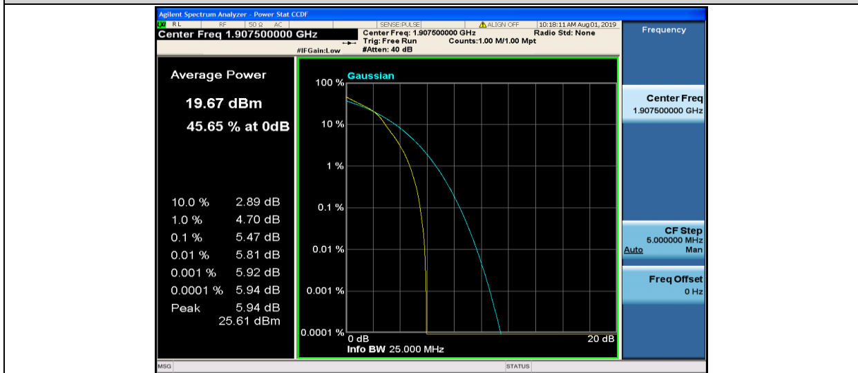
Band2-5MHz-16QAM-19175-25RB#0
