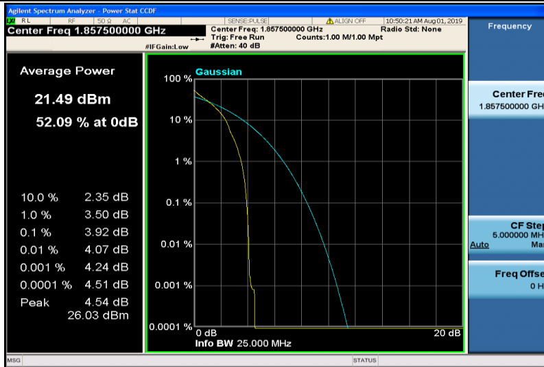
Band2-15MHz-QPSK-18675-1RB#0
