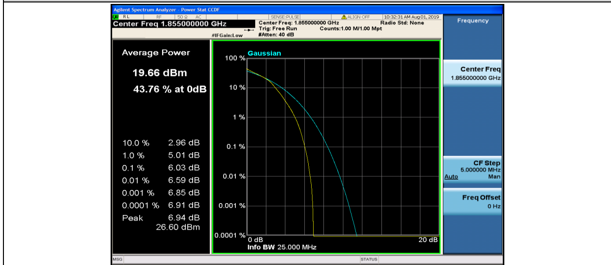
Band2-10MHz-16QAM-18650-50RB#0
