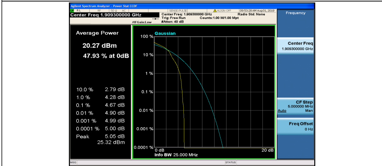
Band2-1.4MHz-16QAM-19193-1RB#0
