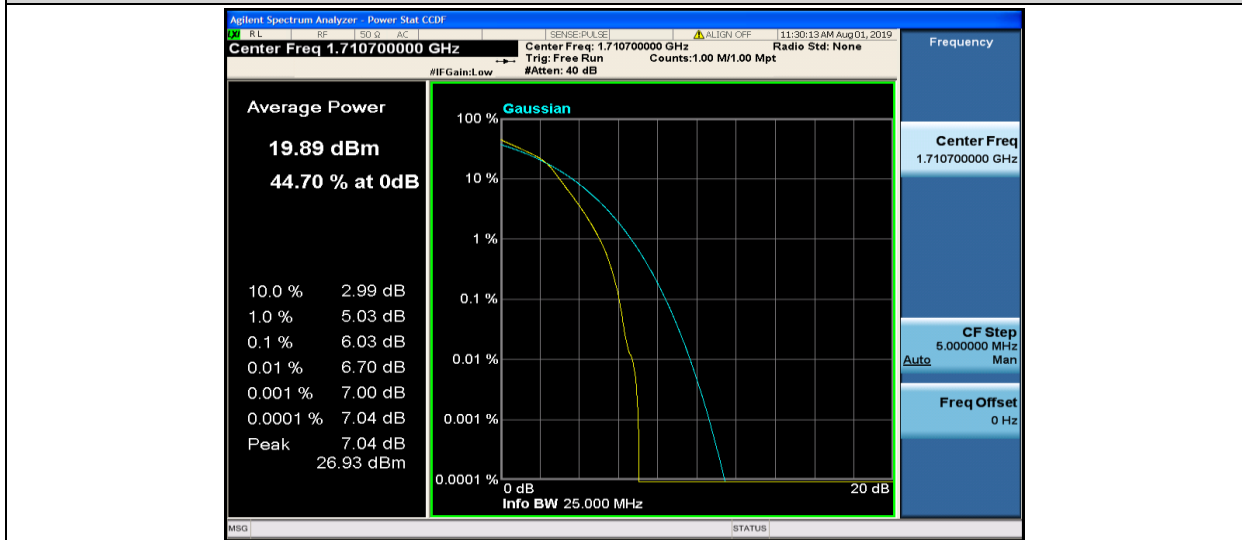
Band4-1.4MHz-16QAM-19957-6RB#0
