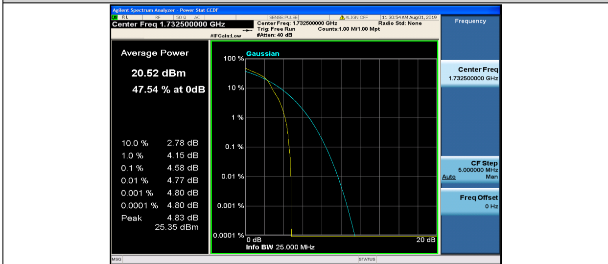
Band4-1.4MHz-16QAM-20175-1RB#0
