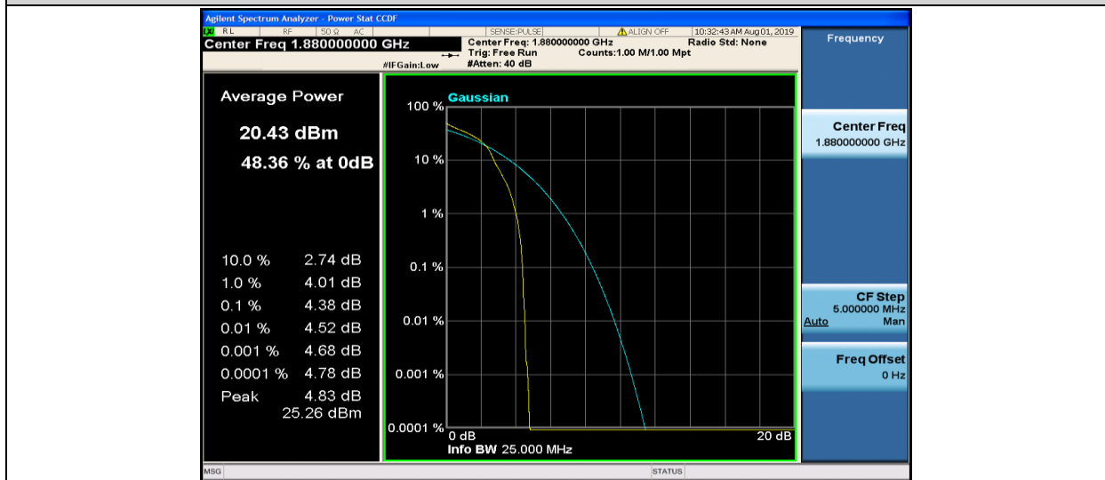
Band2-10MHz-16QAM-18900-1RB#0
