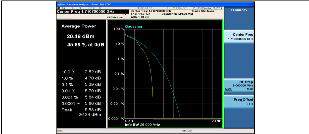
Band4-1.4MHz-16QAM-19957-1RB#0
