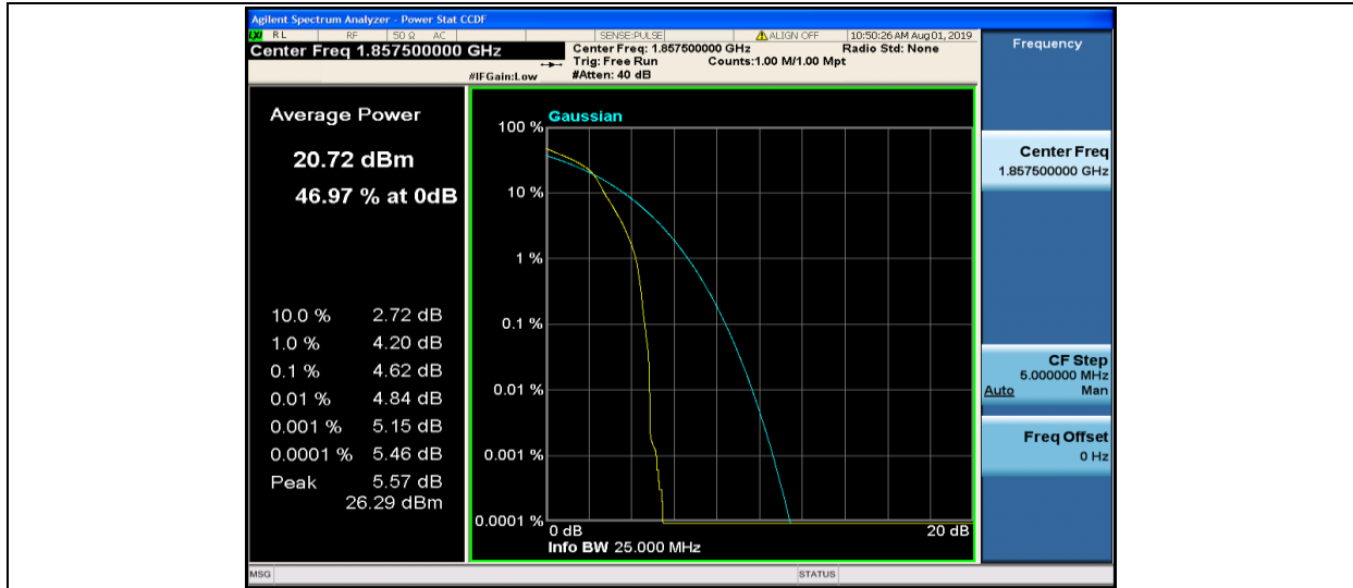
Band2-15MHz-16QAM-18675-1RB#0
