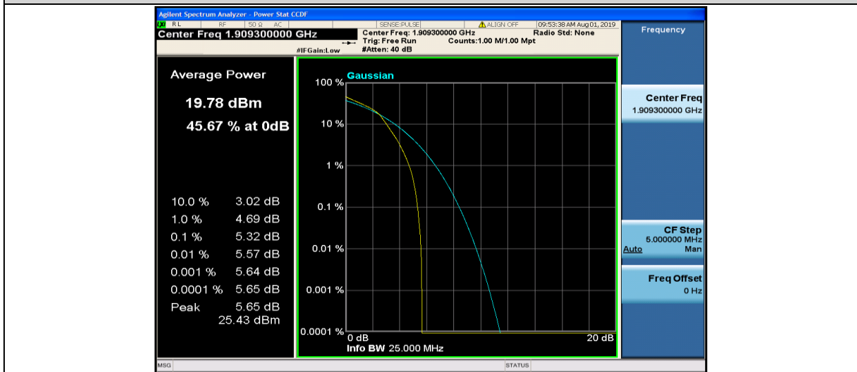
Band2-1.4MHz-16QAM-19193-6RB#0
