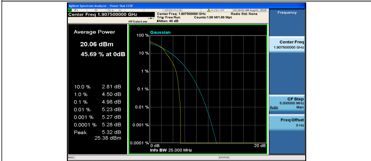
Band2-5MHz-16QAM-19175-1RB#0
