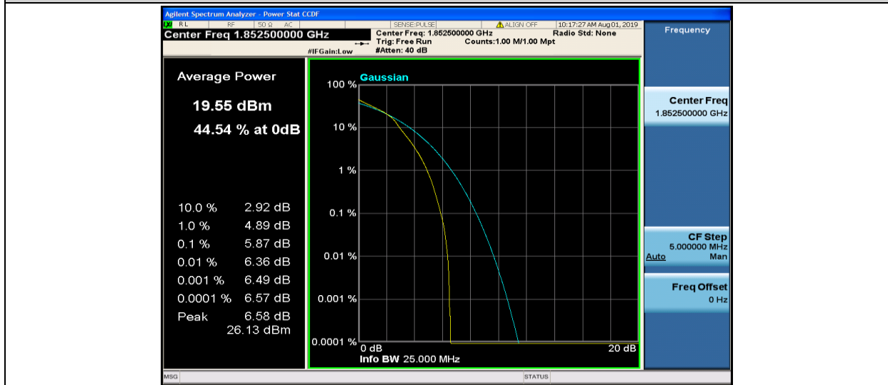
Band2-5MHz-16QAM-18625-25RB#0
