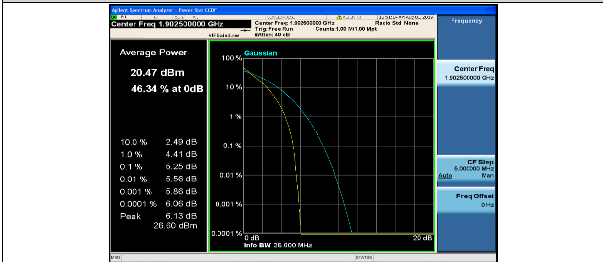
Band2-15MHz-QPSK-19125-75RB#0
