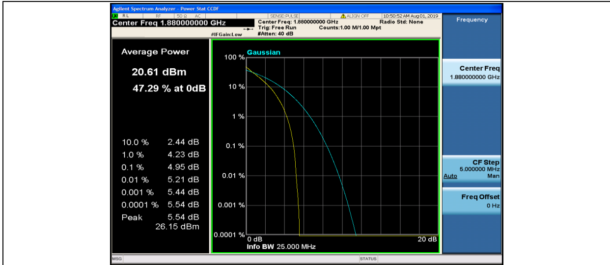
Band2-15MHz-QPSK-18900-75RB#0
