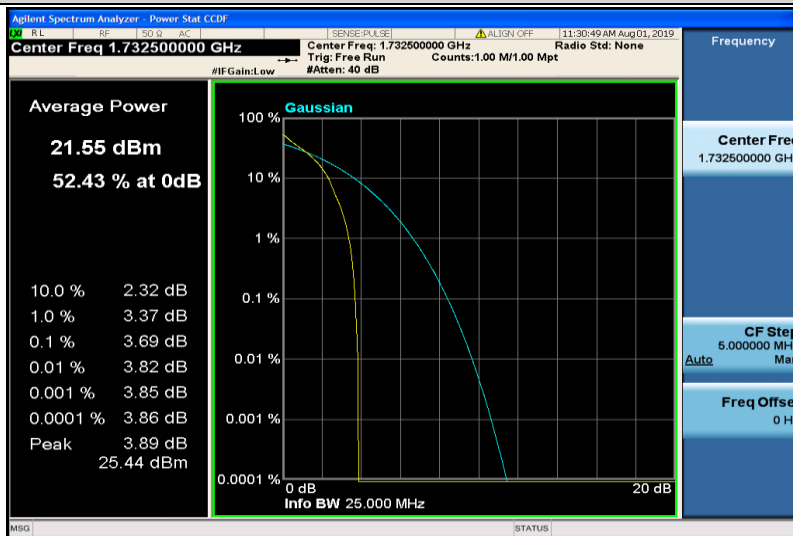
Band4-1.4MHz-QPSK-20175-1RB#0
