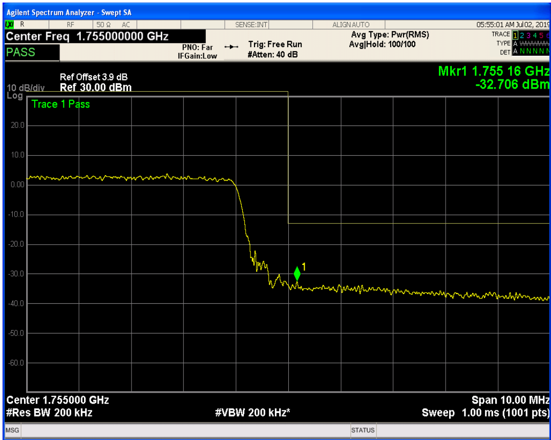
LTE Band4 QAM16 BW=20MHz Channel=20300 RB Size=50 Position=#Max
