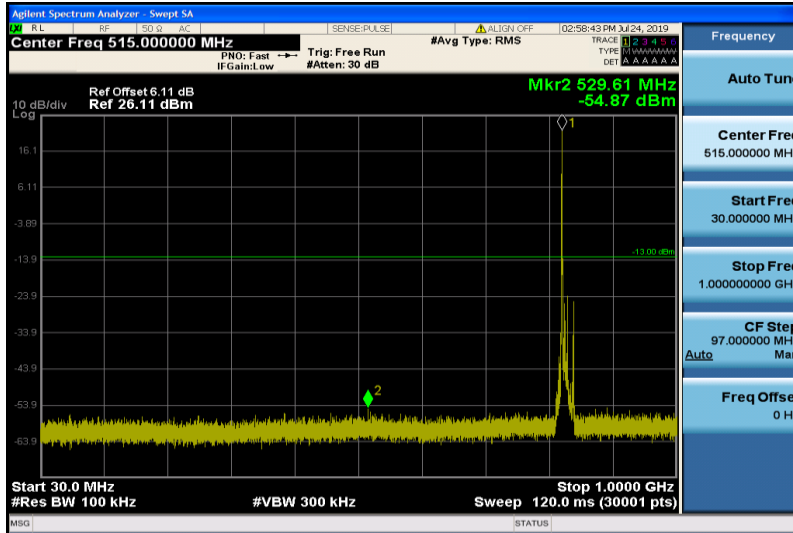
Band5-10MHz-16QAM-20450-1RB#0-30~1000MHz
