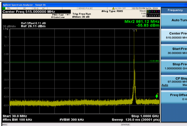
Band5-5MHz-16QAM-20525-1RB#0-30~1000MHz
