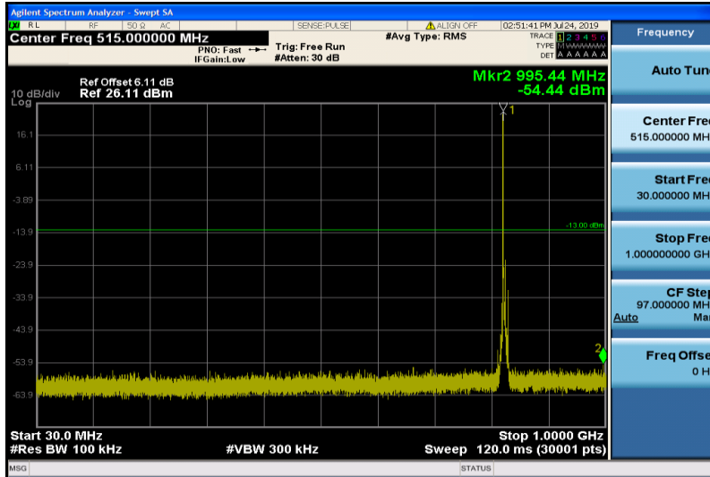
Band5-5MHz-16QAM-20425-1RB#0-30~1000MHz
