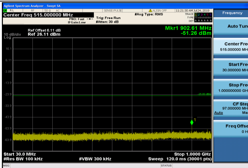
Band7-5MHz-16QAM-21100-1RB#0-30~1000MHz
