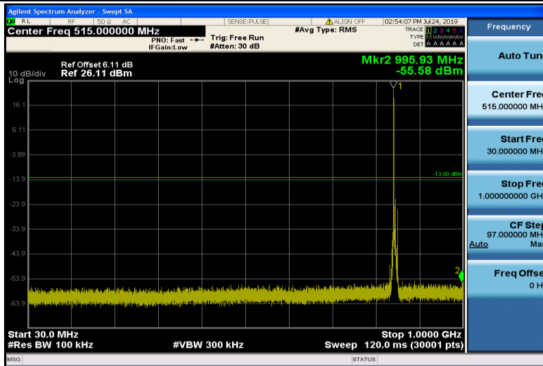
Band5-5MHz-16QAM-20625-1RB#0-30~1000MHz
