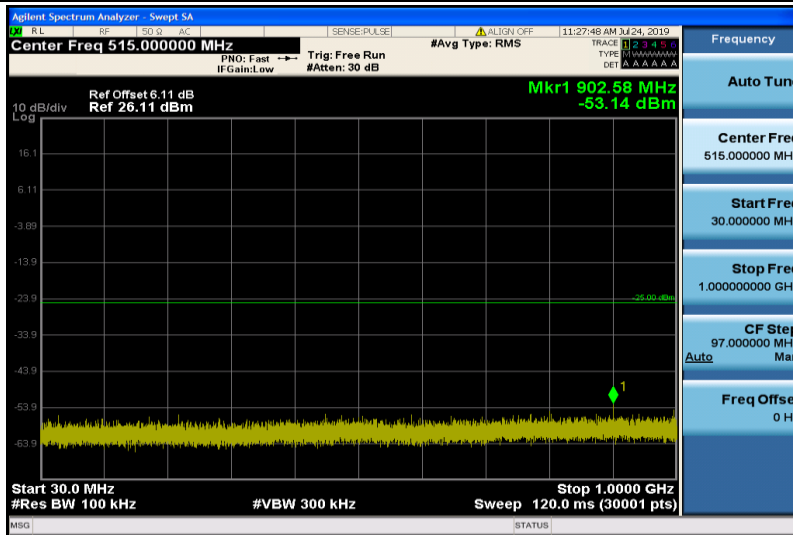
Band7-10MHz-QPSK-21400-1RB#0-30~1000MHz
