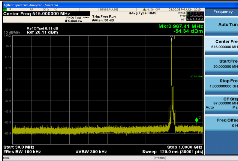
Band5-10MHz-QPSK-20600-1RB#0-30~1000MHz
