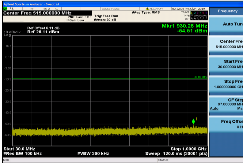
Band4-20MHz-16QAM-20050-1RB#0-30~1000MHz
