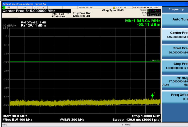
Band4-20MHz-16QAM-20300-1RB#0-30~1000MHz
