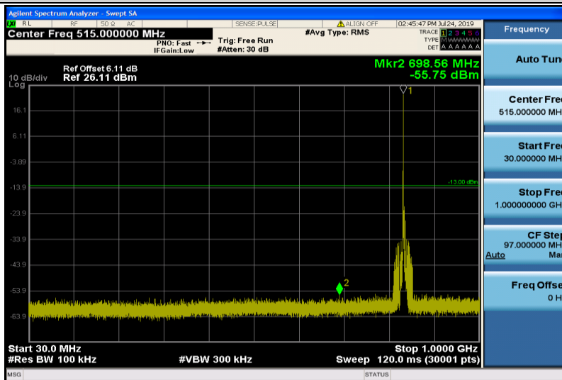
Band5-3MHz-16QAM-20525-1RB#0-30~1000MHz
