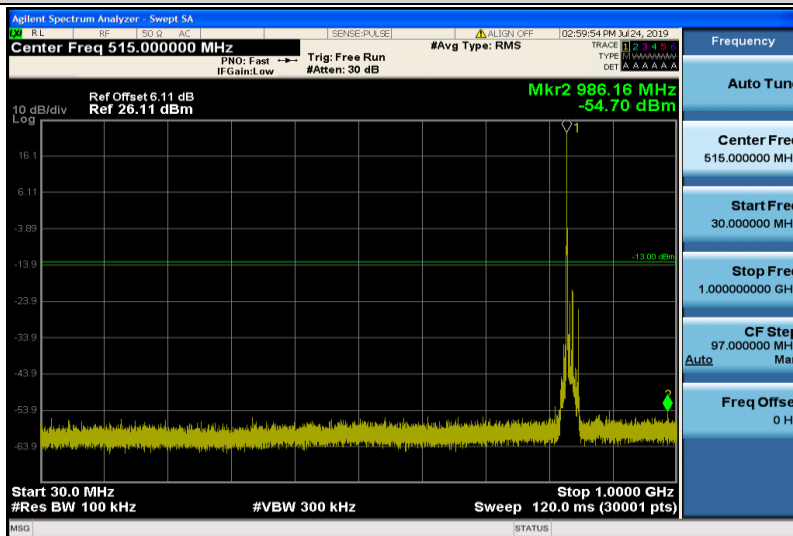
Band5-10MHz-16QAM-20525-1RB#0-30~1000MHz
