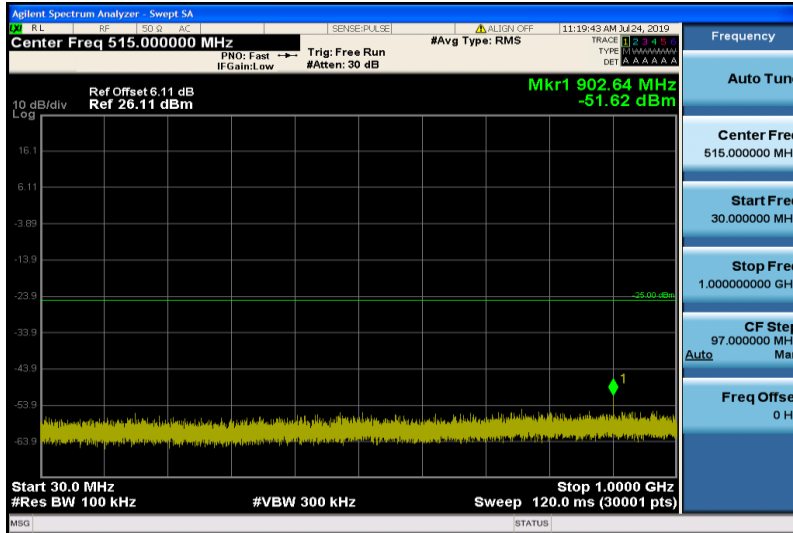
Band7-5MHz-QPSK-20775-1RB#0-30~1000MHz
