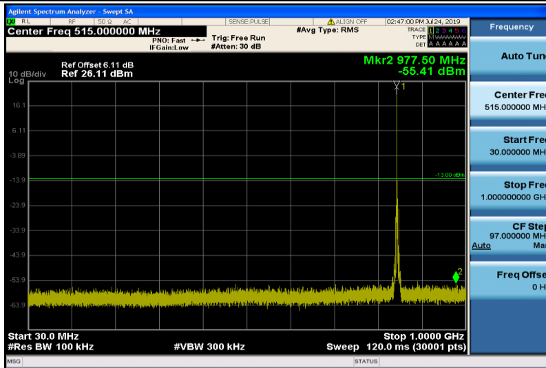
Band5-3MHz-16QAM-20635-1RB#0-30~1000MHz
