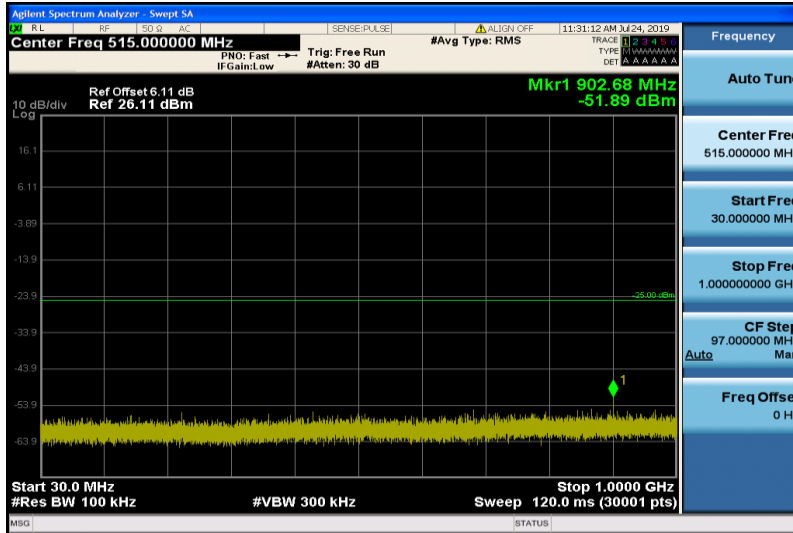
Band7-15MHz-QPSK-20825-1RB#0-30~1000MHz
