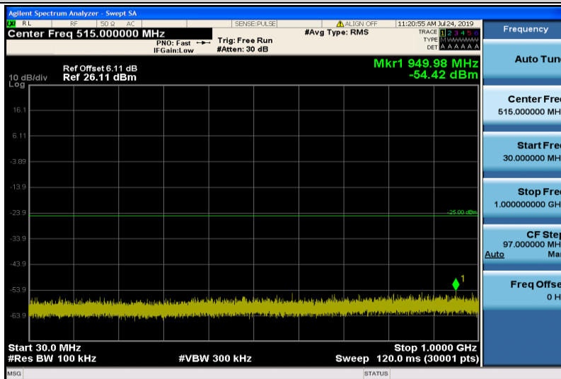
Band7-5MHz-QPSK-21100-1RB#0-30~1000MHz
