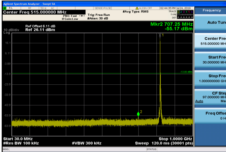
Band5-3MHz-16QAM-20415-1RB#0-30~1000MHz
