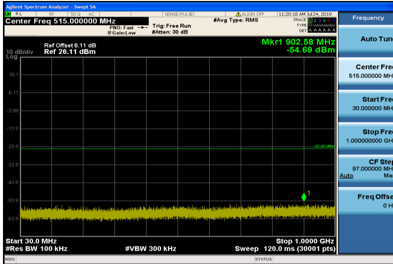
Band7-5MHz-16QAM-20775-1RB#0-30~1000MHz
