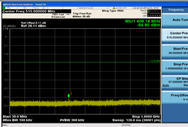
Band2-10MHz-QPSK-18900-1RB#0-30~1000MHz
