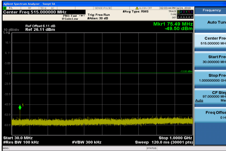
Band4-3MHz-16QAM-19965-1RB#0-30~1000MHz
