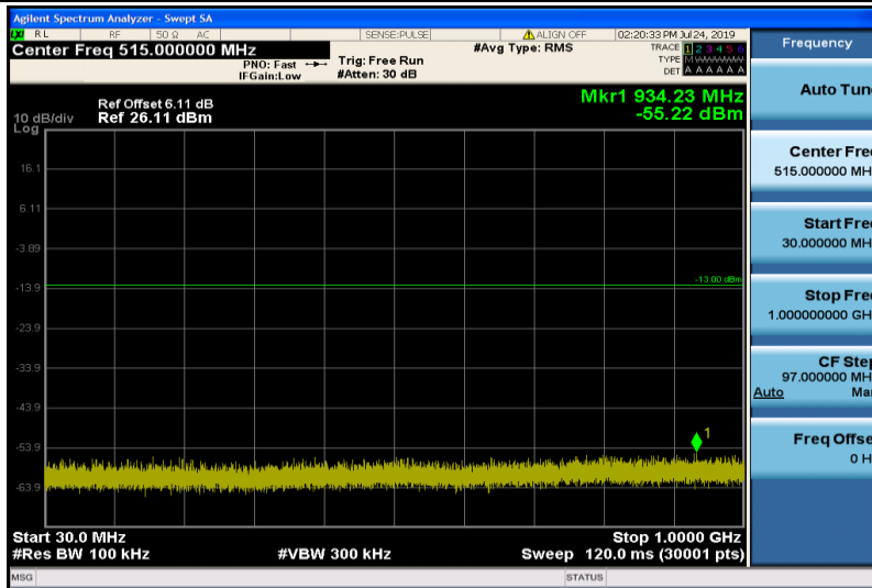
Band4-10MHz-16QAM-20350-1RB#0-30~1000MHz
