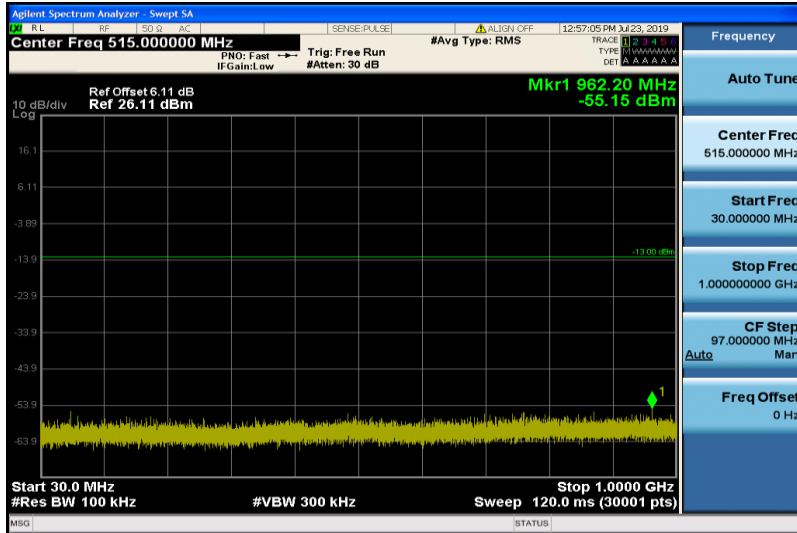
Band2-15MHz-QPSK-18675-1RB#0-30~1000MHz
