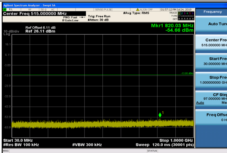
Band4-1.4MHz-QPSK-20175-1RB#0-30~1000MHz
