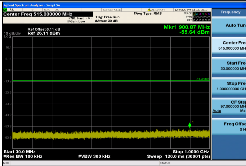
Band2-15MHz-QPSK-19125-1RB#0-30~1000MHz
