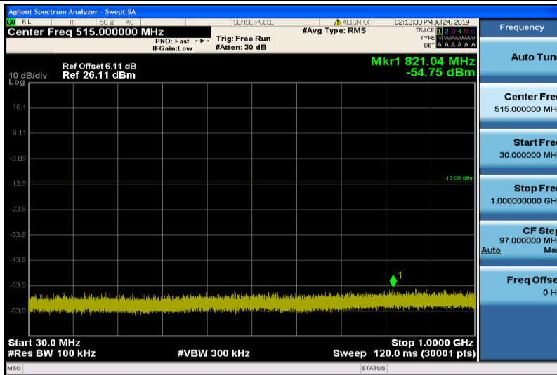
Band4-5MHz-16QAM-20375-1RB#0-30~1000MHz
