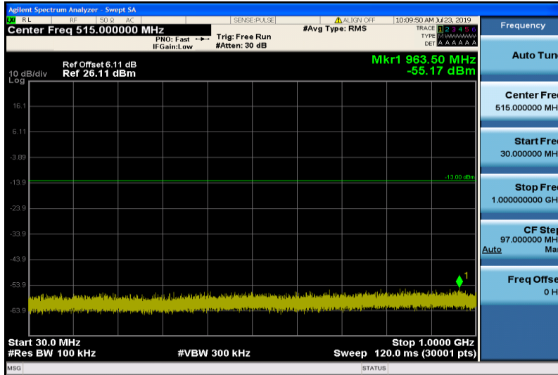
Band2-10MHz-16QAM-18650-1RB#0-30~1000MHz
