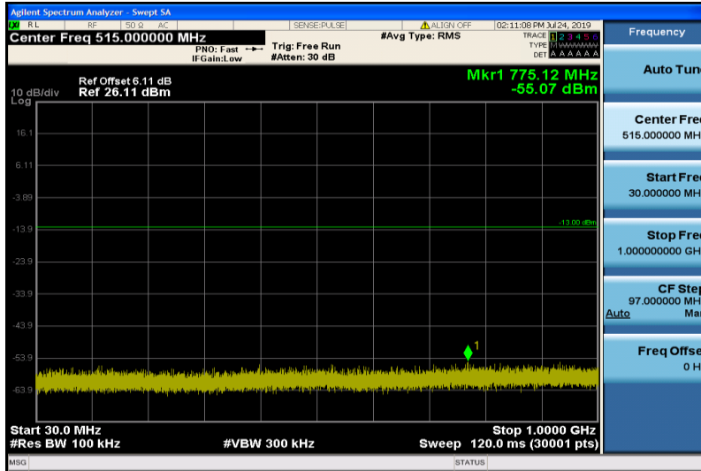
Band4-5MHz-16QAM-19975-1RB#0-30~1000MHz
