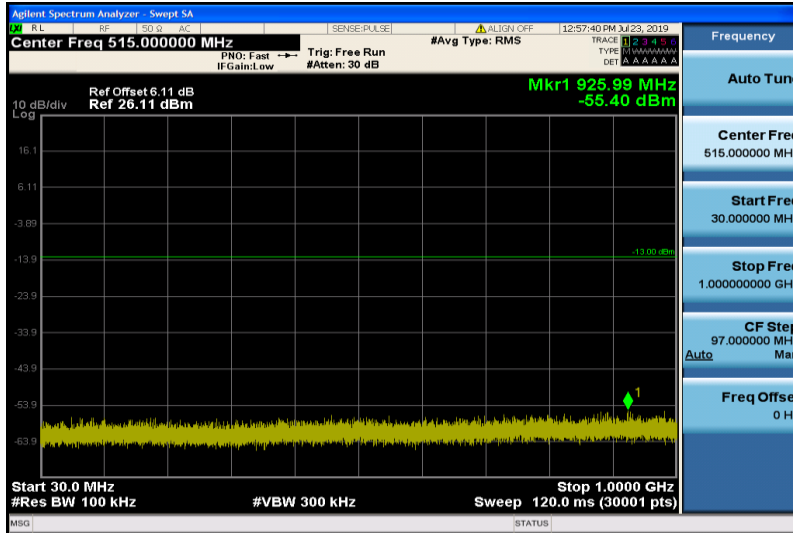
Band2-15MHz-16QAM-18675-1RB#0-30~1000MHz
