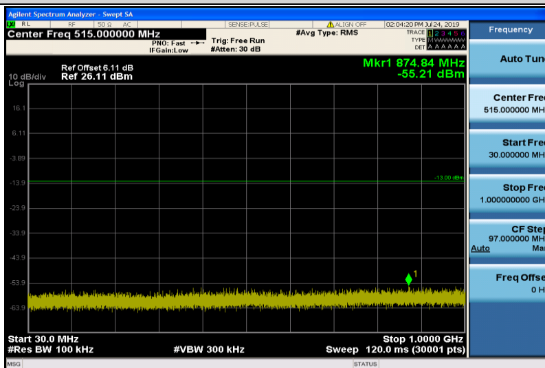
Band4-3MHz-QPSK-20175-1RB#0-30~1000MHz
