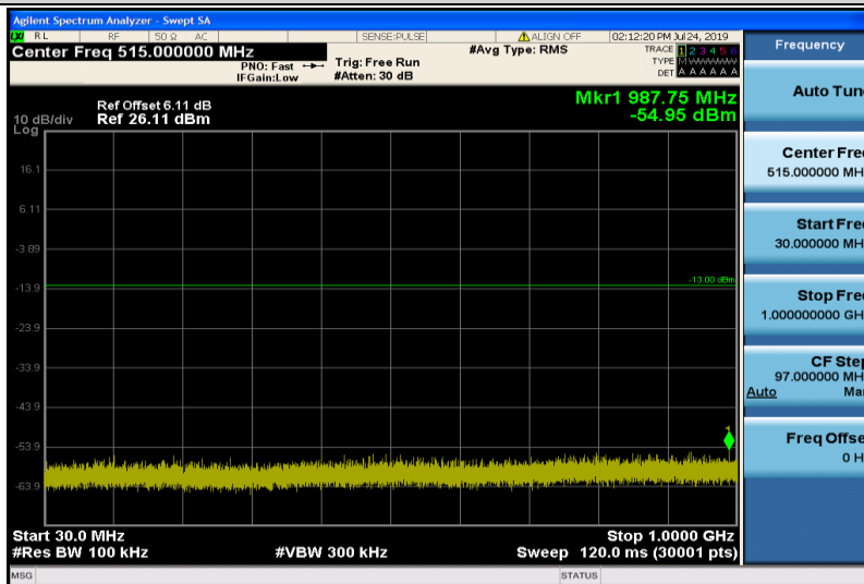
Band4-5MHz-16QAM-20175-1RB#0-30~1000MHz
