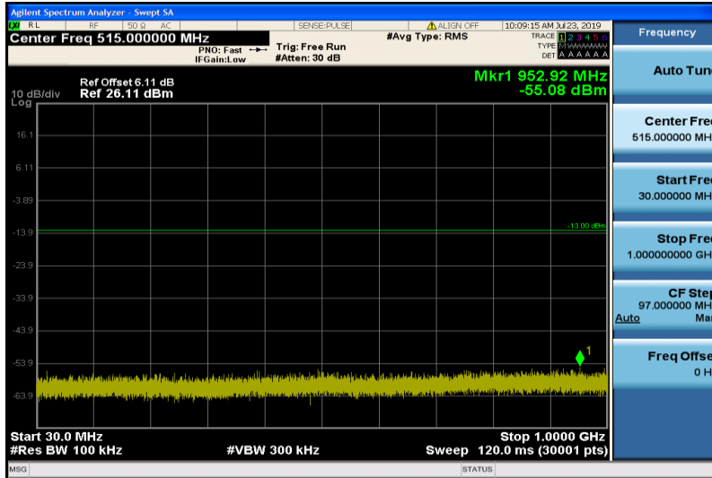
Band2-10MHz-QPSK-18650-1RB#0-30~1000MHz
