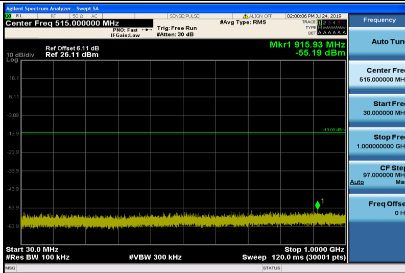
Band4-1.4MHz-16QAM-20393-1RB#0-30~1000MHz
