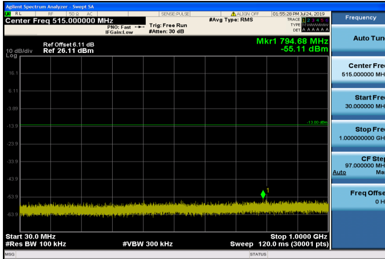
Band4-1.4MHz-QPSK-19957-1RB#0-30~1000MHz
