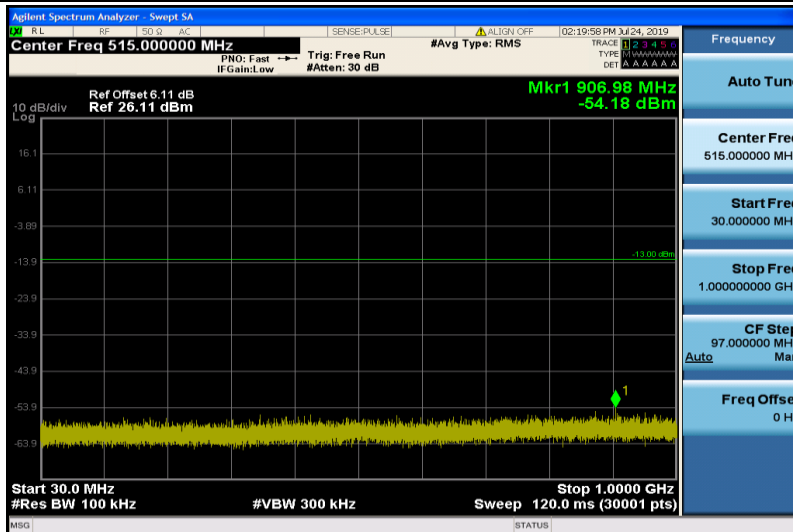
Band4-10MHz-QPSK-20350-1RB#0-30~1000MHz
