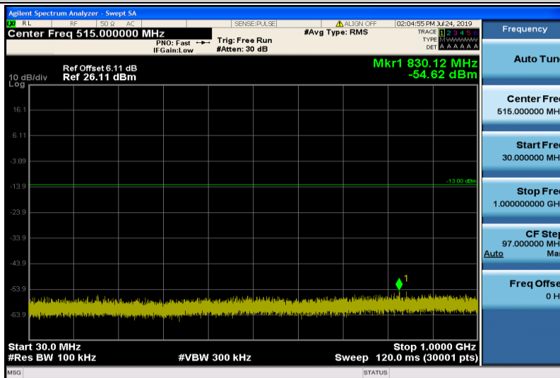
Band4-3MHz-16QAM-20175-1RB#0-30~1000MHz
