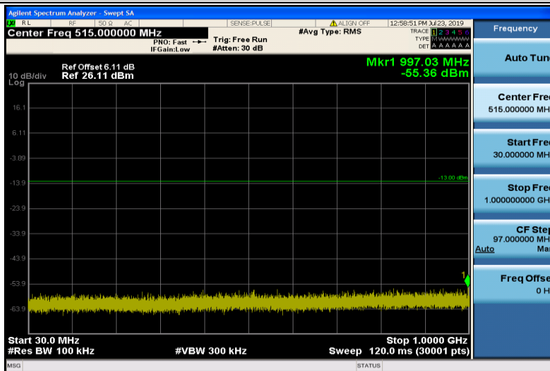
Band2-15MHz-16QAM-18900-1RB#0-30~1000MHz
