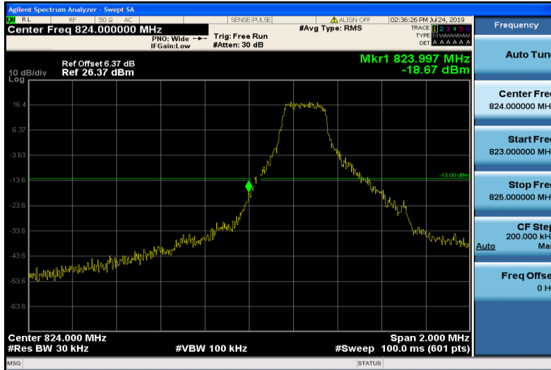
Band5-1.4MHz-QPSK-20407-1RB#0
