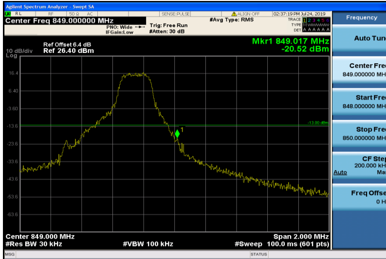
Band5-1.4MHz-16QAM-20643-1RB#5
