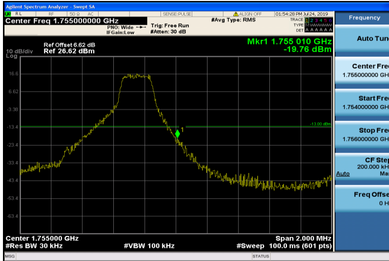
Band4-1.4MHz-16QAM-20393-1RB#5
