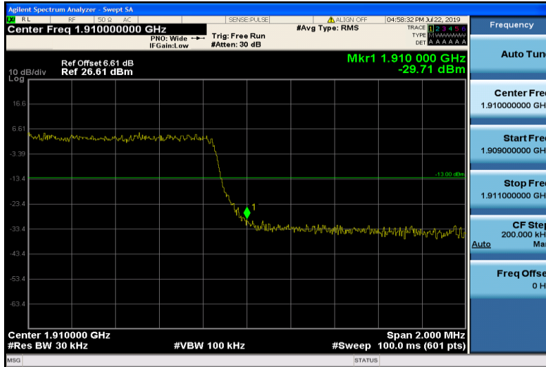
Band2-3MHz-16QAM-19185-15RB#0
