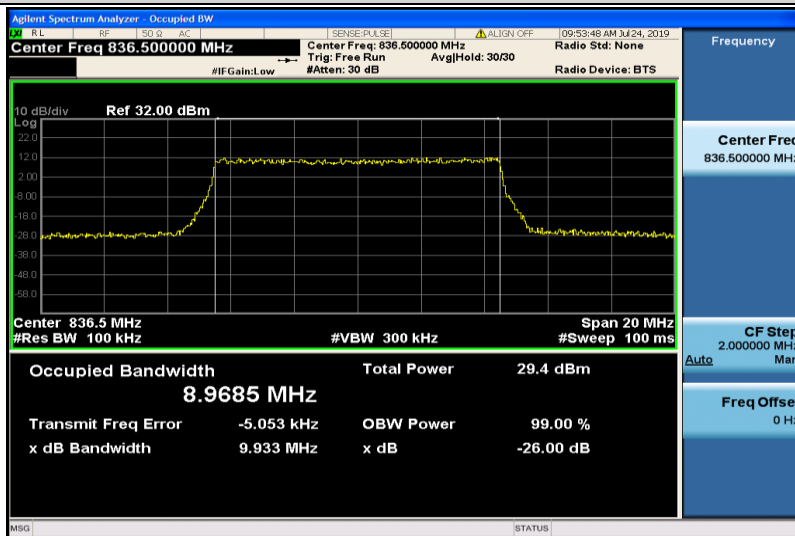
Band5-10MHz-16QAM-20525-50RB#0-8.9685
