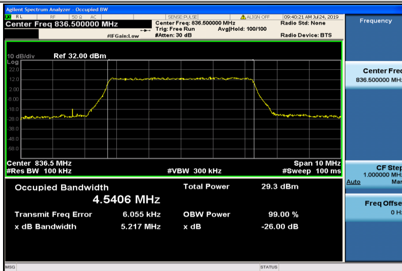
Band5-5MHz-16QAM-20525-25RB#0-4.5406
