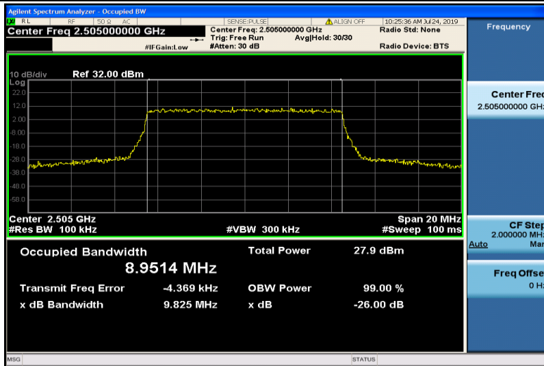
Band7-10MHz-16QAM-20800-50RB#0-8.9514
