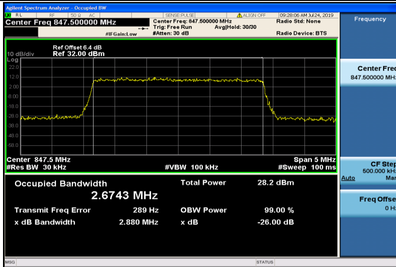
Band5-3MHz-16QAM-20635-15RB#0-2.6743
