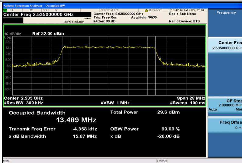
Band7-15MHz-QPSK-21100-75RB#0-13.489
