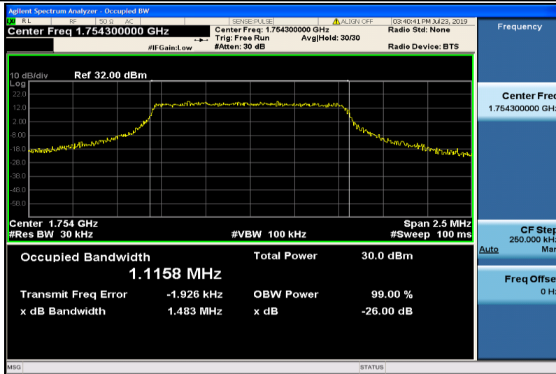
Band4-1.4MHz-QPSK-20393-6RB#0-1.1158
