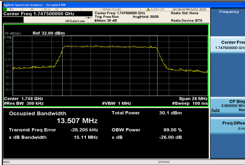
Band4-15MHz-QPSK-20325-75RB#0-13.507
