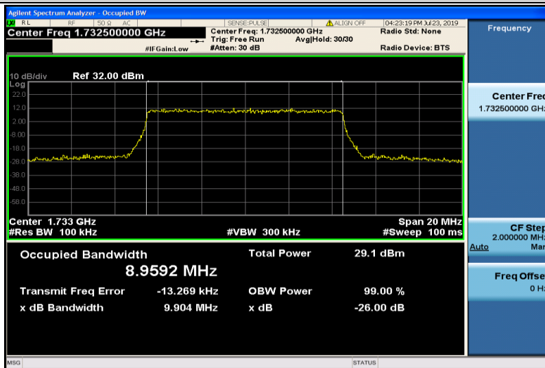
Band4-10MHz-16QAM-20175-50RB#0-8.9592
