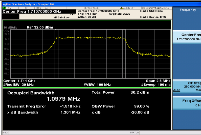
Band4-1.4MHz-QPSK-19957-6RB#0-1.0979
