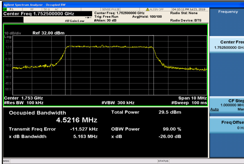
Band4-5MHz-16QAM-20375-25RB#0-4.5216
