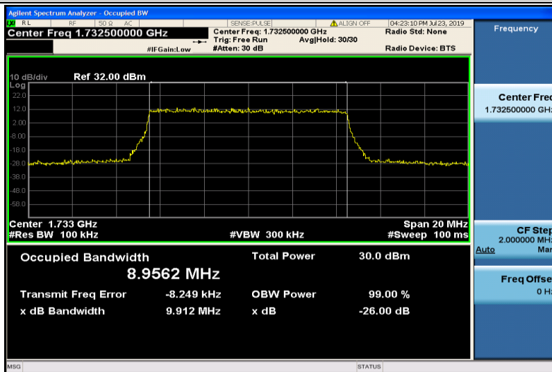
Band4-10MHz-QPSK-20175-50RB#0-8.9562
