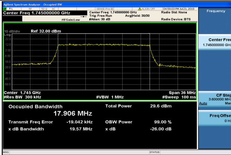
Band4-20MHz-16QAM-20300-100RB#0-17.906
