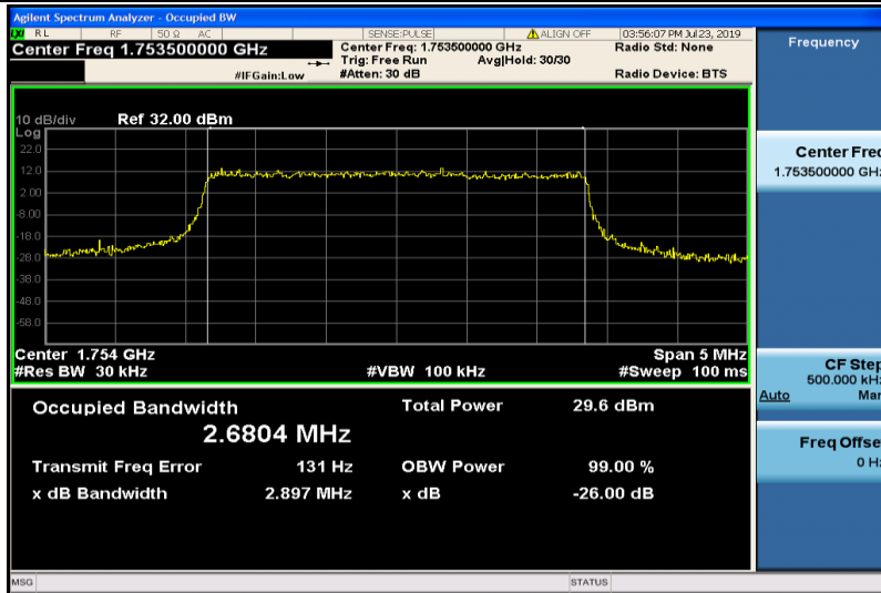
Band4-3MHz-QPSK-20385-15RB#0-2.6804
