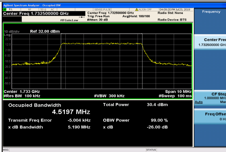
Band4-5MHz-QPSK-20175-25RB#0-4.5197
