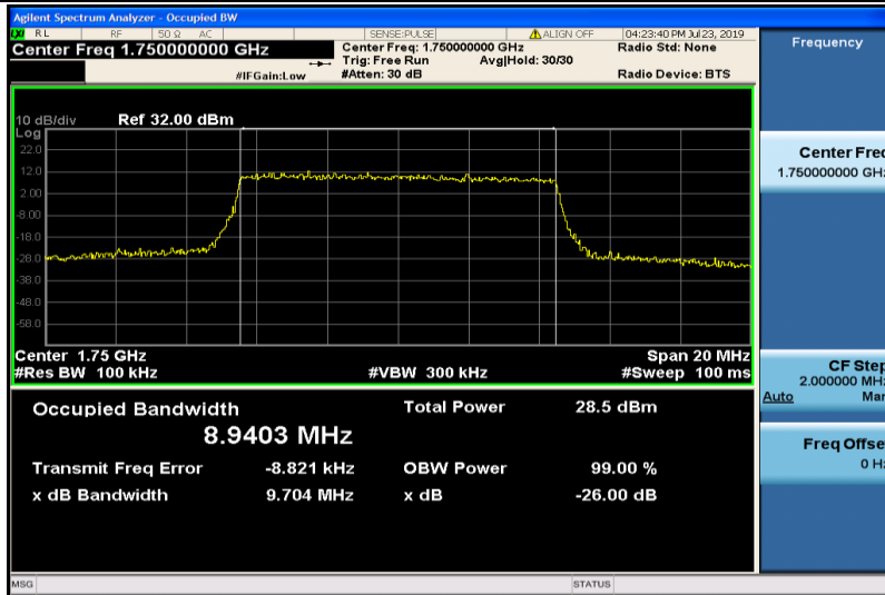
Band4-10MHz-16QAM-20350-50RB#0-8.9403
