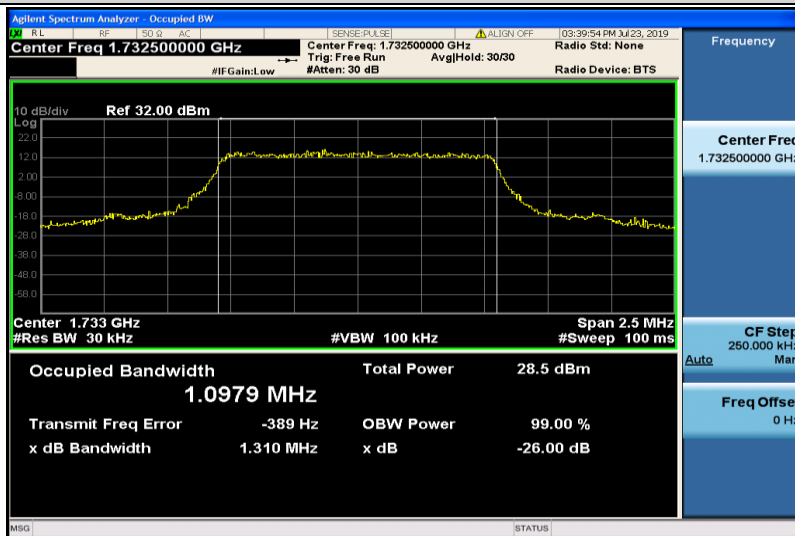
Band4-1.4MHz-16QAM-20175-6RB#0-1.0979
