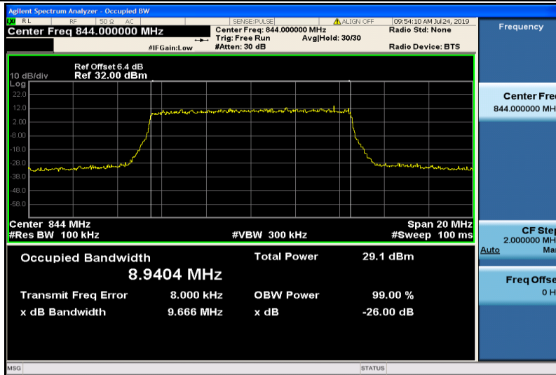
Band5-10MHz-16QAM-20600-50RB#0-8.9404
