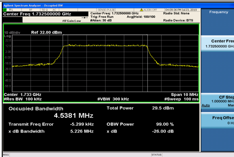
Band4-5MHz-16QAM-20175-25RB#0-4.5381
