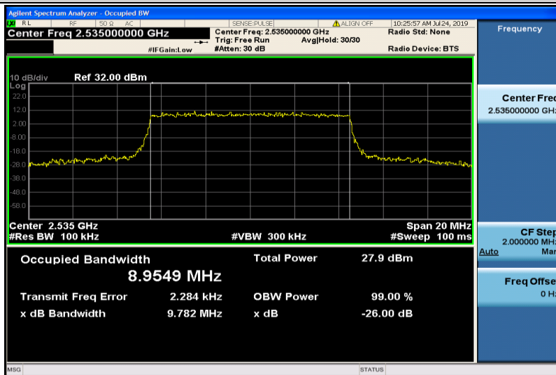
Band7-10MHz-16QAM-21100-50RB#0-8.9549
