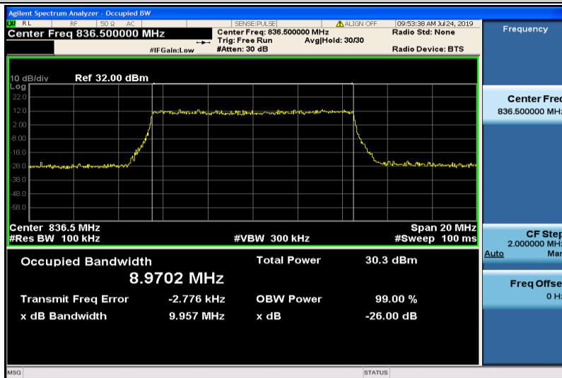
Band5-10MHz-QPSK-20525-50RB#0-8.9702
