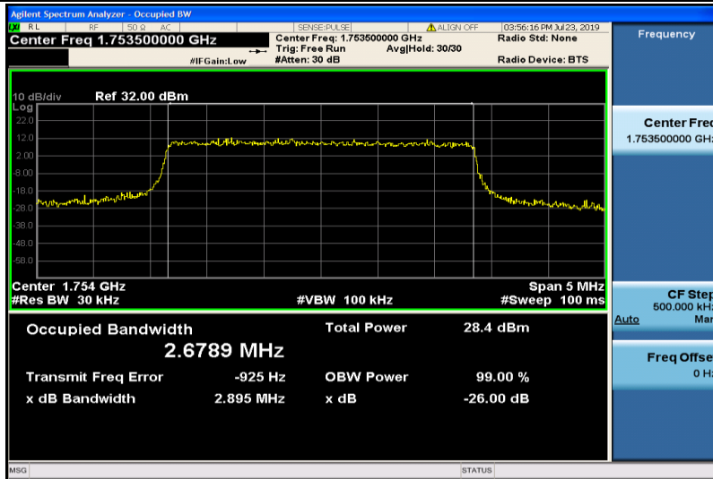
Band4-3MHz-16QAM-20385-15RB#0-2.6789
