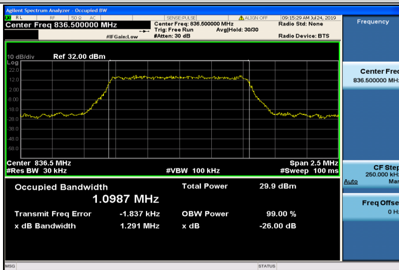
Band5-1.4MHz-QPSK-20525-6RB#0-1.0987
