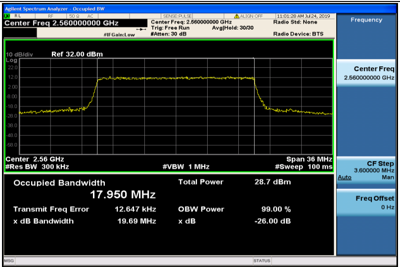
Band7-20MHz-16QAM-21350-100RB#0-17.950
