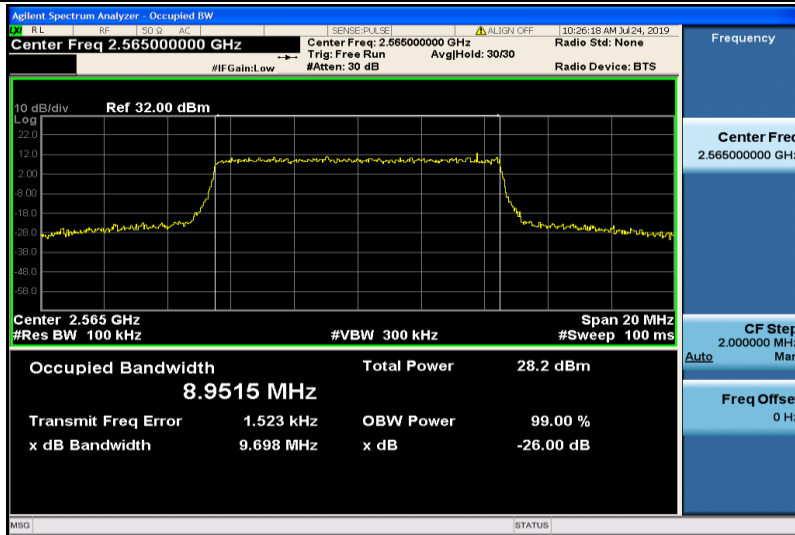
Band7-10MHz-16QAM-21400-50RB#0-8.9515
