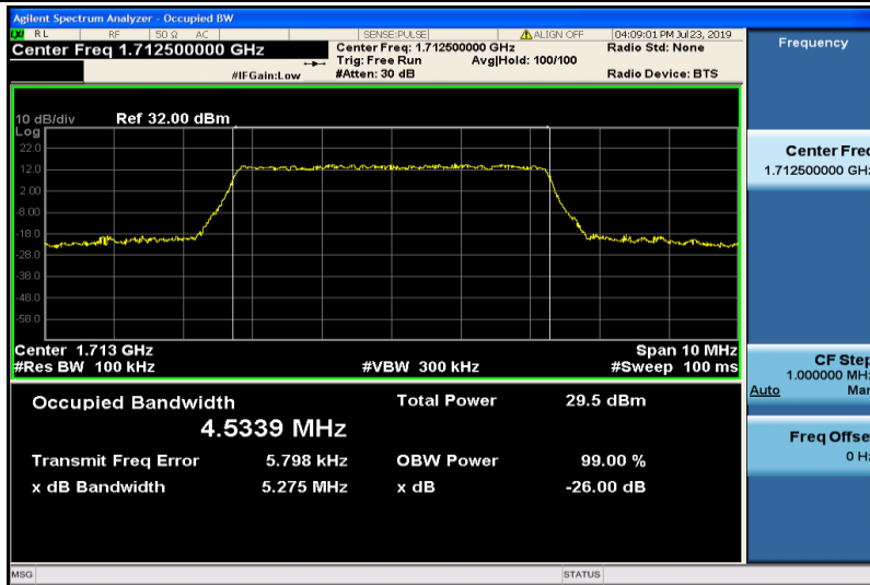
Band4-5MHz-16QAM-19975-25RB#0-4.5339
