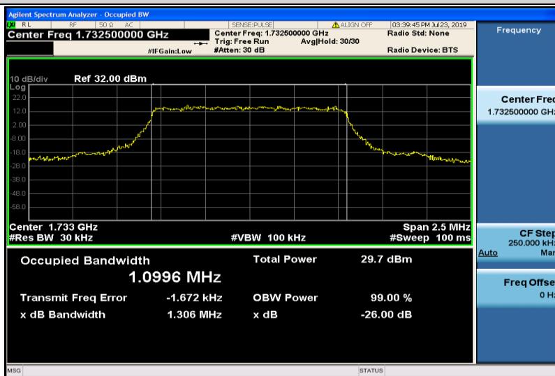
Band4-1.4MHz-QPSK-20175-6RB#0-1.0996
