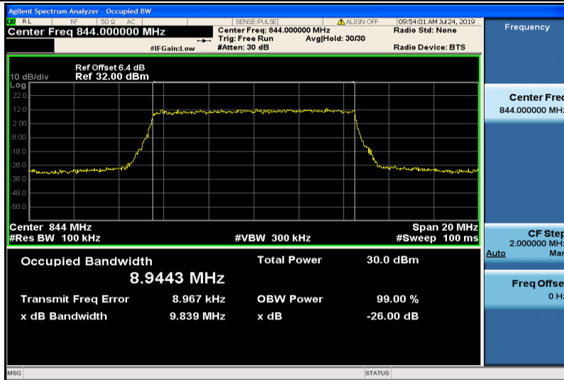
Band5-10MHz-QPSK-20600-50RB#0-8.9443
