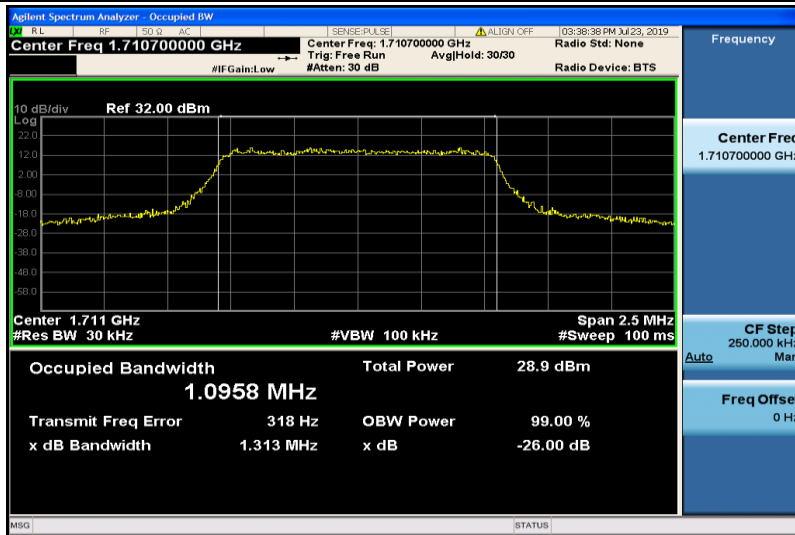
Band4-1.4MHz-16QAM-19957-6RB#0-1.0958
