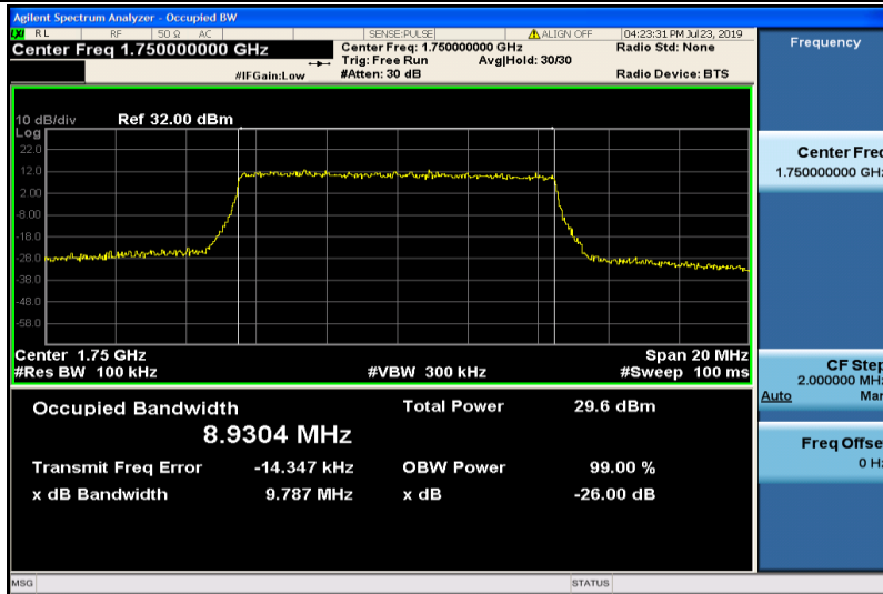
Band4-10MHz-QPSK-20350-50RB#0-8.9304
