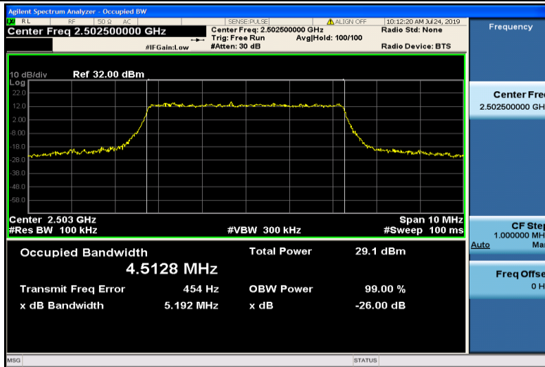
Band7-5MHz-QPSK-20775-25RB#0-4.5128
