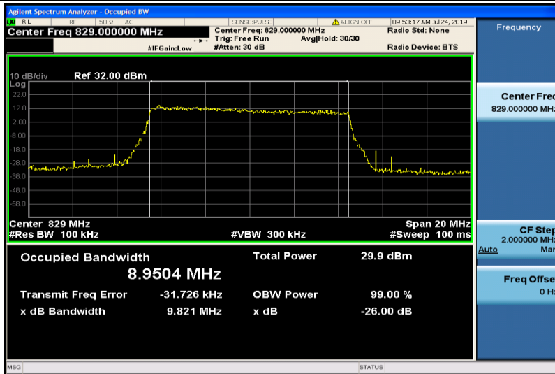
Band5-10MHz-QPSK-20450-50RB#0-8.9504
