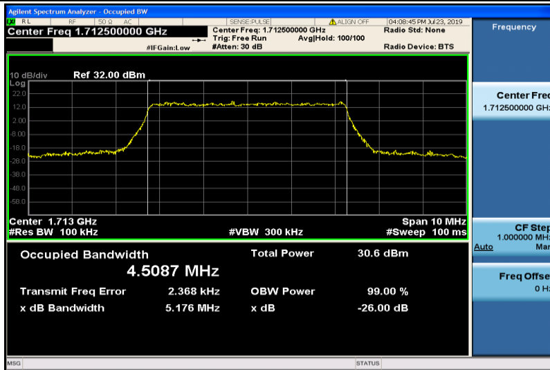
Band4-5MHz-QPSK-19975-25RB#0-4.5087
