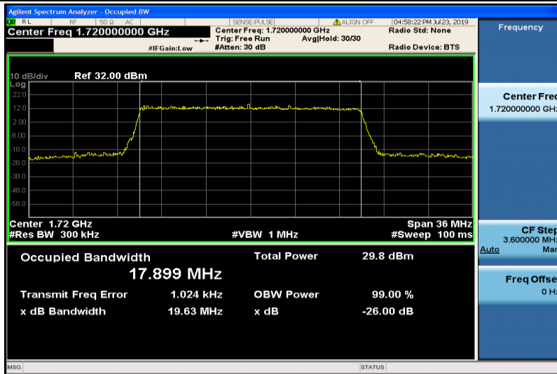
Band4-20MHz-16QAM-20050-100RB#0-17.899
