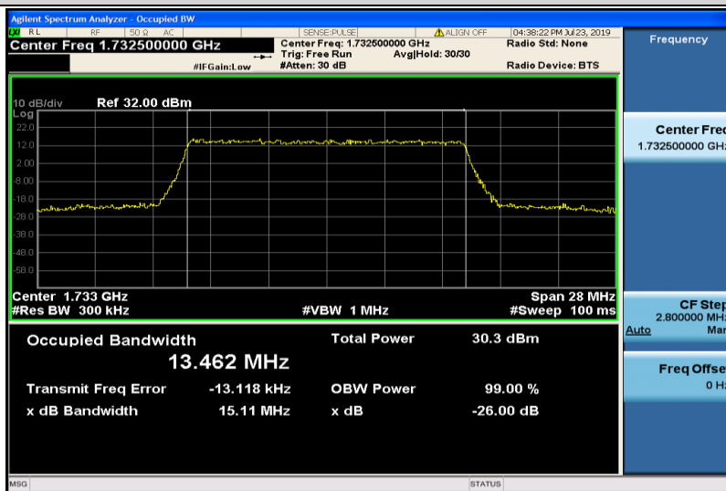
Band4-15MHz-QPSK-20175-75RB#0-13.462
