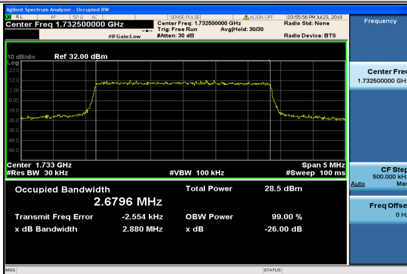
Band4-3MHz-16QAM-20175-15RB#0-2.6796
