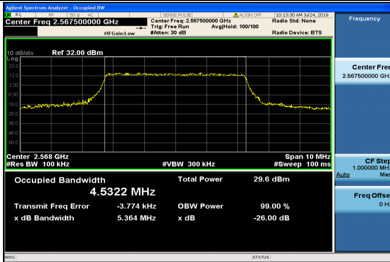
Band7-5MHz-QPSK-21425-25RB#0-4.5322
