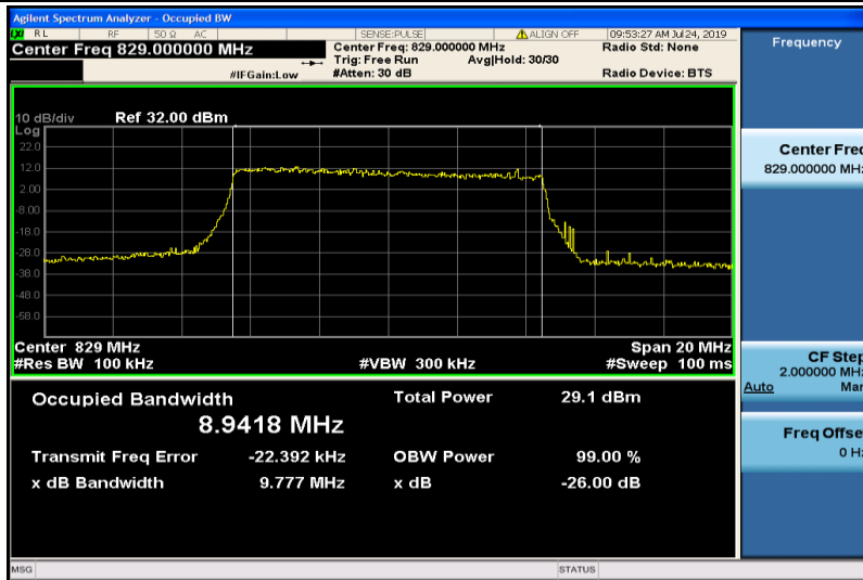
Band5-10MHz-16QAM-20450-50RB#0-8.9418
