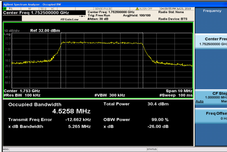
Band4-5MHz-QPSK-20375-25RB#0-4.5258
