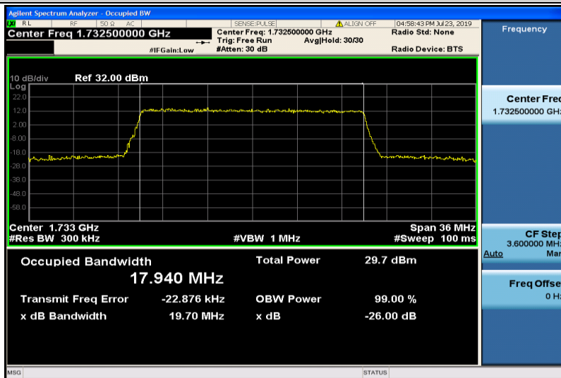
Band4-20MHz-16QAM-20175-100RB#0-17.940
