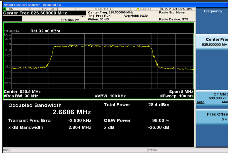
Band5-3MHz-16QAM-20415-15RB#0-2.6686
