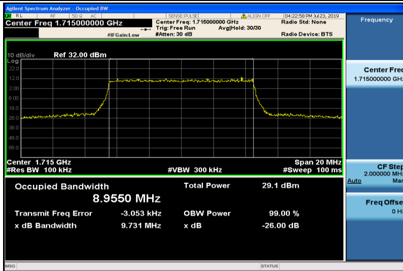
Band4-10MHz-16QAM-20000-50RB#0-8.9550
