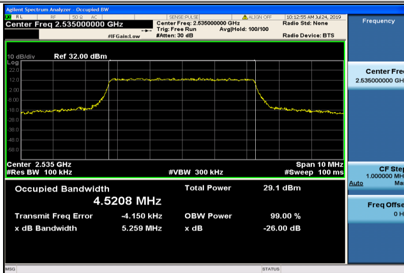
Band7-5MHz-QPSK-21100-25RB#0-4.5208
