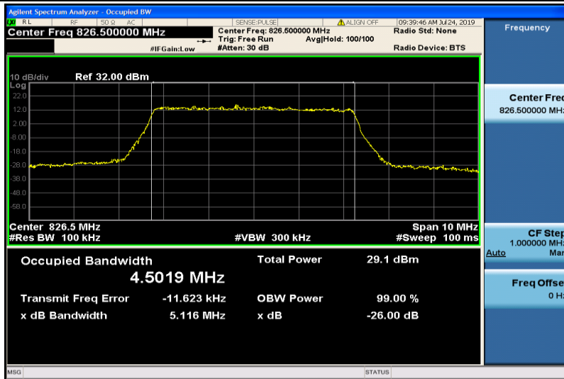
Band5-5MHz-16QAM-20425-25RB#0-4.5019
