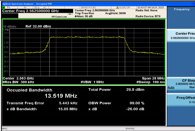
Band7-15MHz-QPSK-21375-75RB#0-13.519
