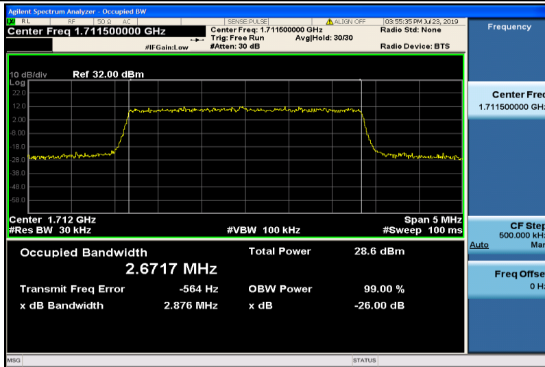
Band4-3MHz-16QAM-19965-15RB#0-2.6717
