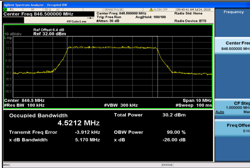
Band5-5MHz-QPSK-20625-25RB#0-4.5212
