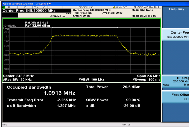
Band5-1.4MHz-QPSK-20643-6RB#0-1.0913
