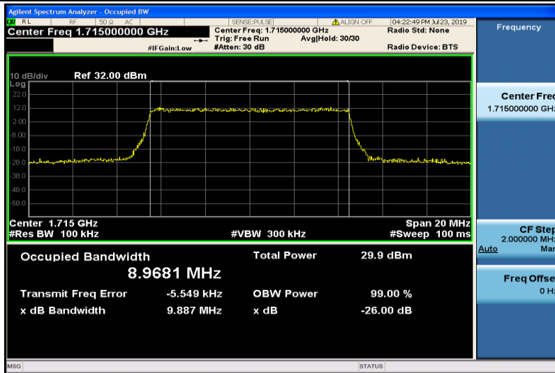
Band4-10MHz-QPSK-20000-50RB#0-8.9681
