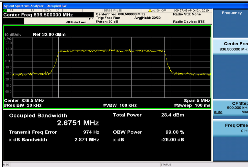
Band5-3MHz-16QAM-20525-15RB#0-2.6751
