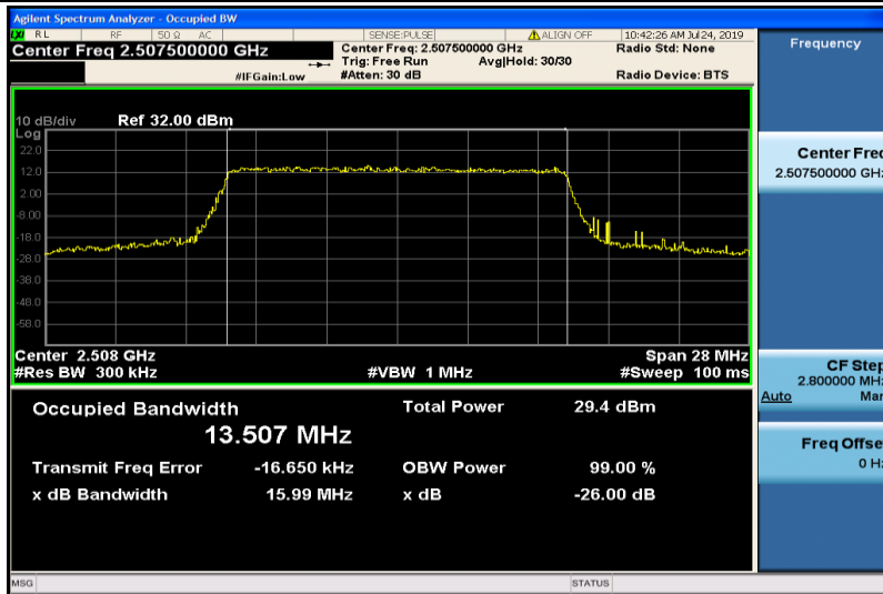
Band7-15MHz-QPSK-20825-75RB#0-13.507
