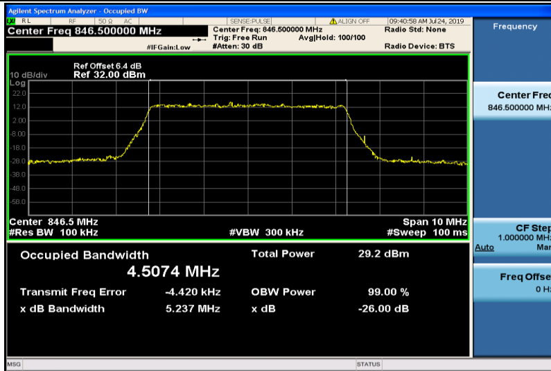
Band5-5MHz-16QAM-20625-25RB#0-4.5074
