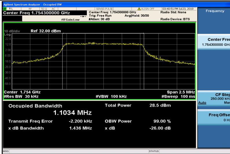
Band4-1.4MHz-16QAM-20393-6RB#0-1.1034
