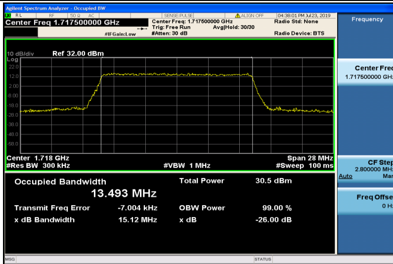
Band4-15MHz-QPSK-20025-75RB#0-13.493
