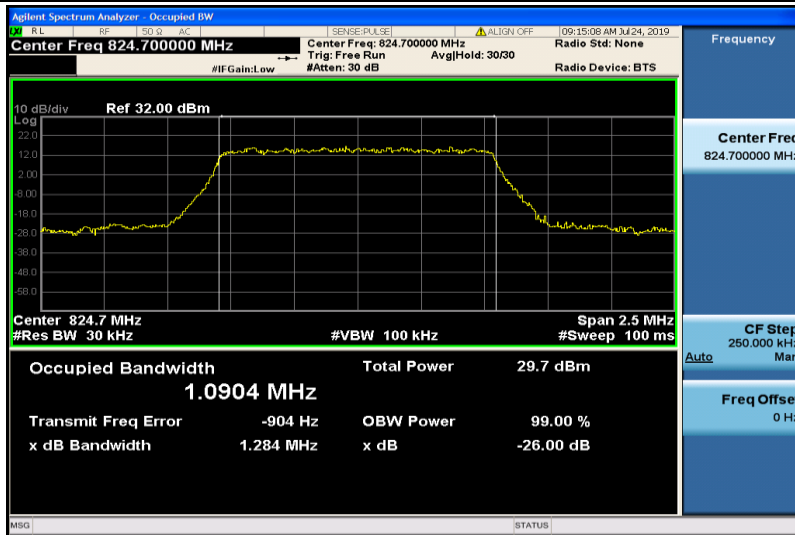
Band5-1.4MHz-QPSK-20407-6RB#0-1.0904
