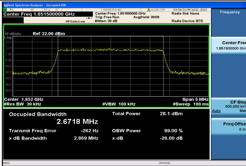
Band2-3MHz-16QAM-18615-15RB#0-2.6718
