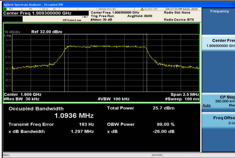
Band2-1.4MHz-16QAM-19193-6RB#0-1.0936
