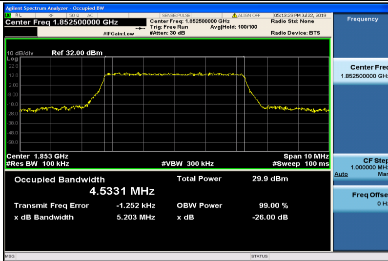
Band2-5MHz-QPSK-18625-25RB#0-4.5331
