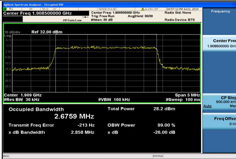
Band2-3MHz-16QAM-19185-15RB#0-2.6759
