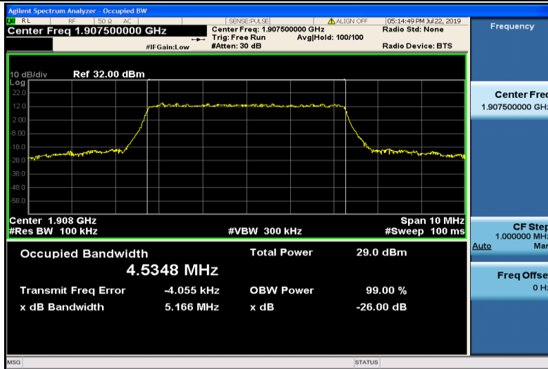
Band2-5MHz-16QAM-19175-25RB#0-4.5348
