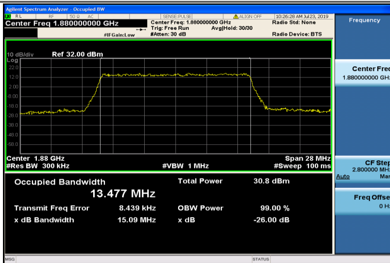
Band2-15MHz-QPSK-18900-75RB#0-13.477
