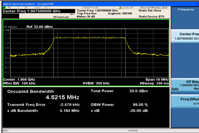
Band2-5MHz-QPSK-19175-25RB#0-4.5215
