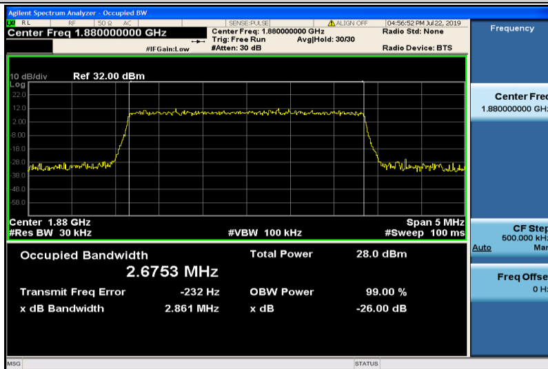
Band2-3MHz-16QAM-18900-15RB#0-2.6753
