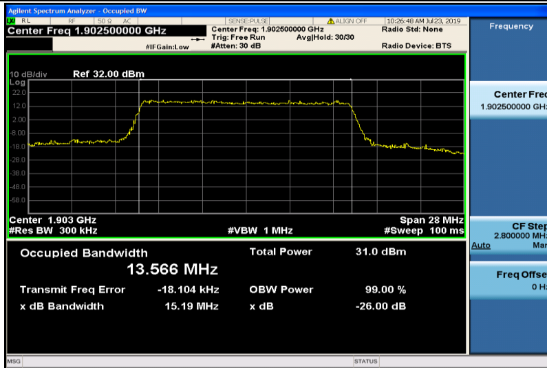
Band2-15MHz-QPSK-19125-75RB#0-13.566
