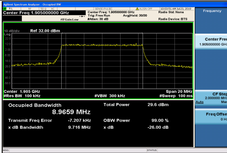
Band2-10MHz-16QAM-19150-50RB#0-8.9659
