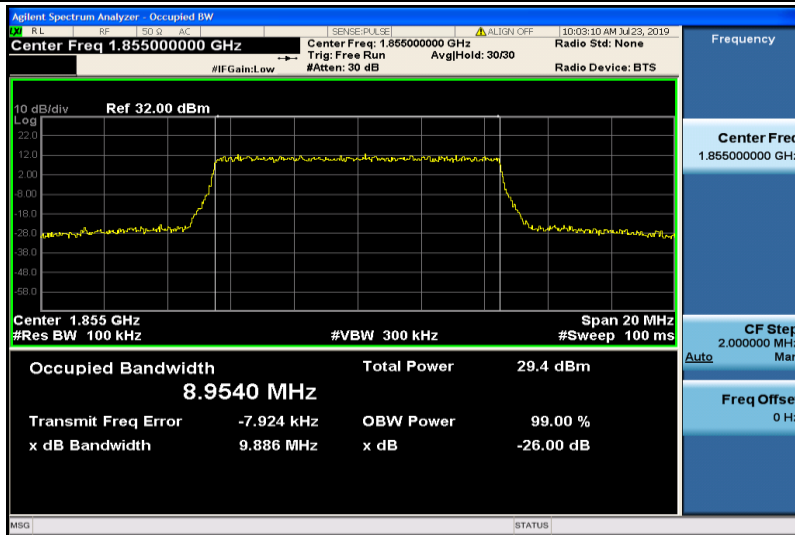
Band2-10MHz-16QAM-18650-50RB#0-8.9540
