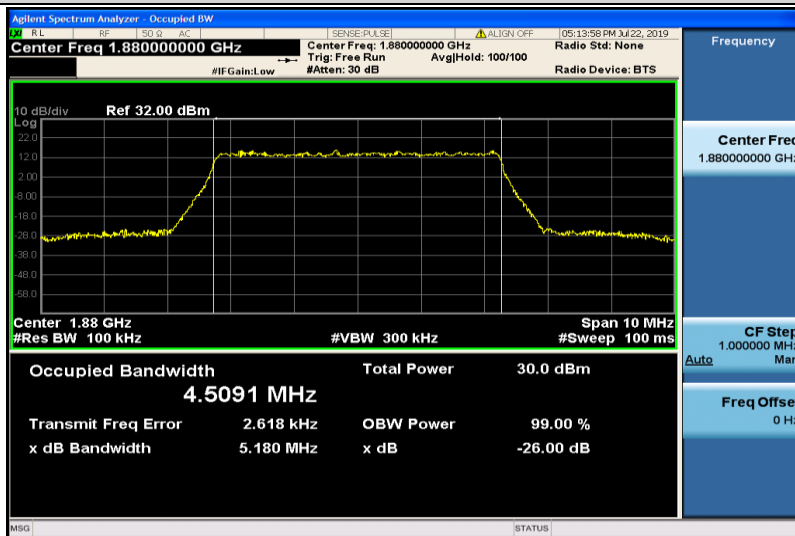
Band2-5MHz-QPSK-18900-25RB#0-4.5091
