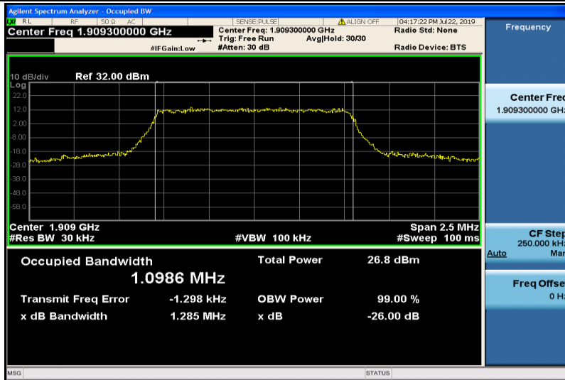
Band2-1.4MHz-QPSK-19193-6RB#0-1.0986
