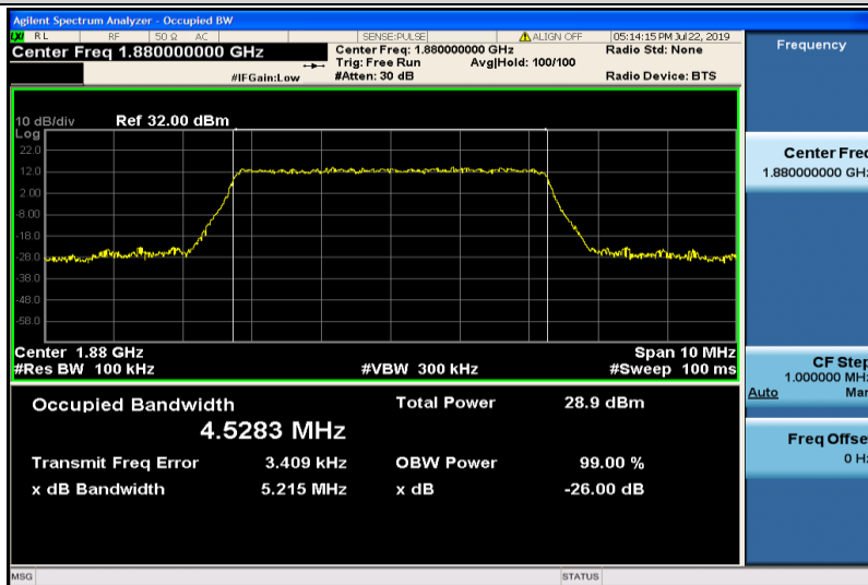
Band2-5MHz-16QAM-18900-25RB#0-4.5283
