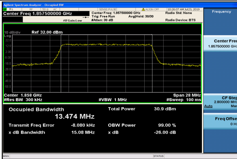
Band2-15MHz-QPSK-18675-75RB#0-13.474
