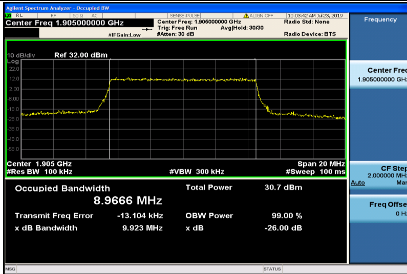
Band2-10MHz-QPSK-19150-50RB#0-8.9666
