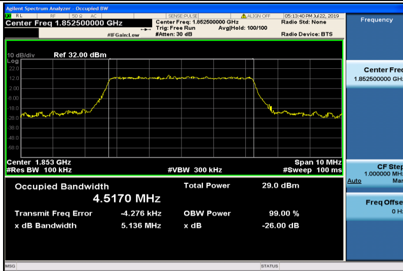
Band2-5MHz-16QAM-18625-25RB#0-4.5170
