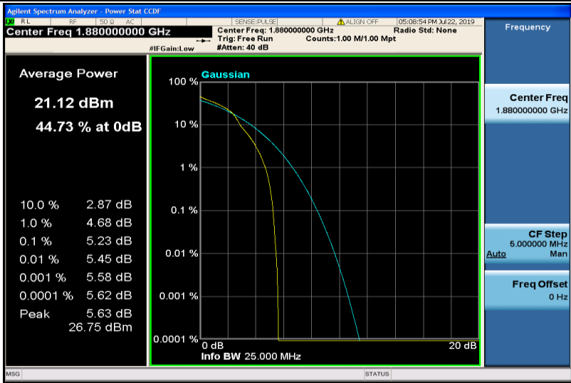
Band2-3MHz-16QAM-18900-1RB#0
