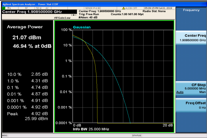
Band2-3MHz-16QAM-19185-1RB#0
