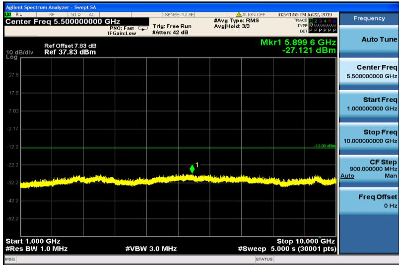
GPRS850-128-1000~10000
