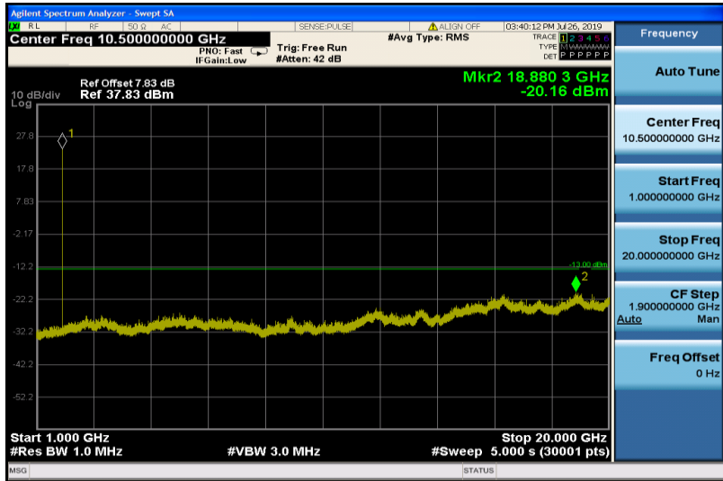
EGPRS1900-512-1000~20000
