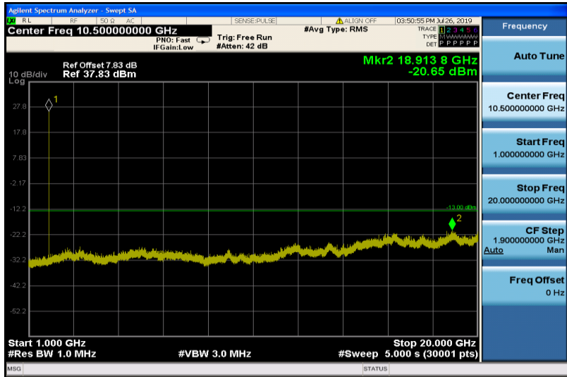
GPRS1900-512-1000~20000
