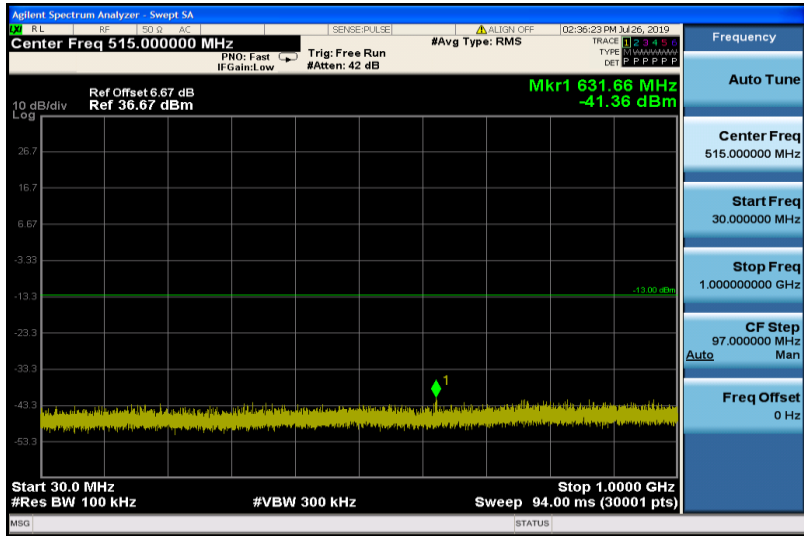
GSM1900-512-30~1000
