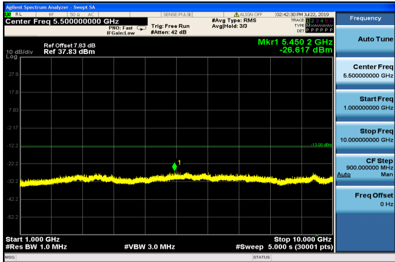
GPRS850-190-1000~10000
