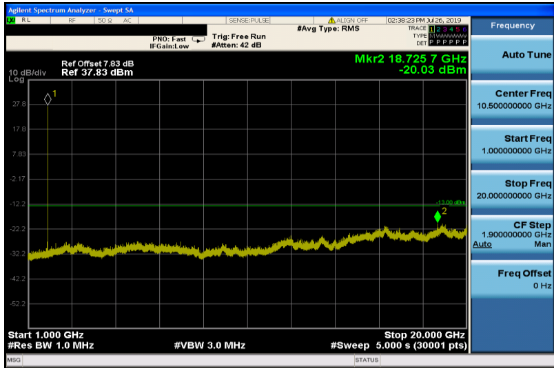
GSM1900-512-1000~20000
