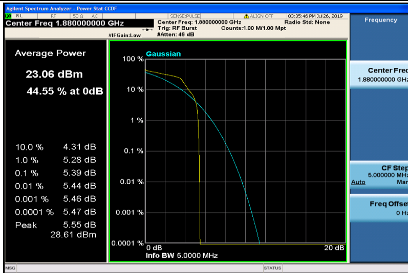
EPR1900-661
