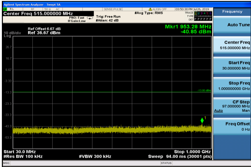
GPRS1900-512-30~1000
