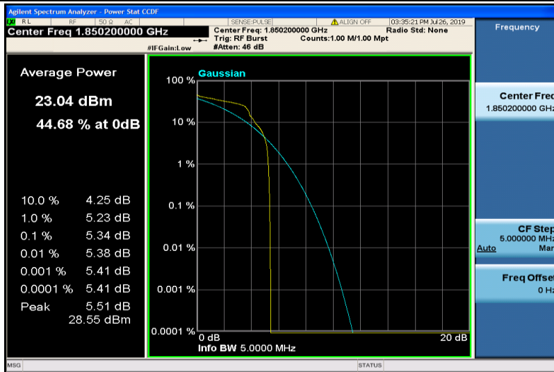
EPR1900-512
