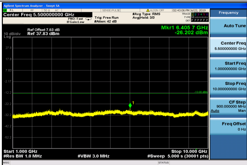
GPRS850-251-1000~10000
