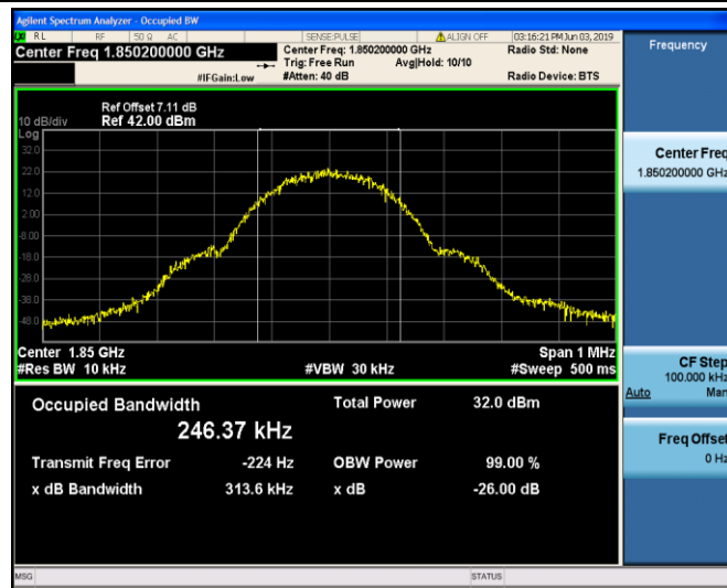
GPRS1900_512
