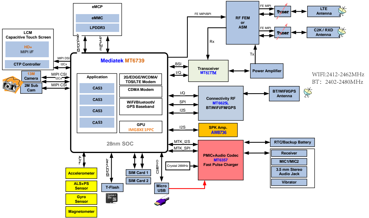
Figure 1-1. High-level MT6739 functional block diagram
