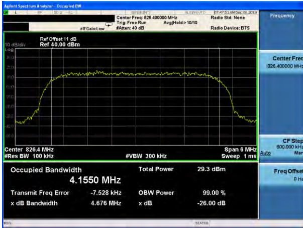
-26dB&99% Bandwidth plot on channel 4132
