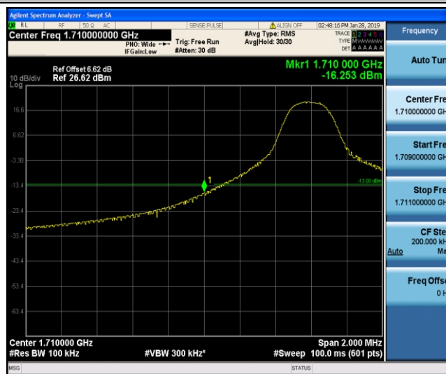
Band4_10MHz_QPSK_2000_1RB#0
