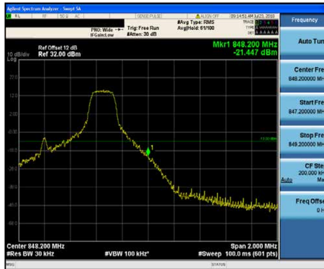
Band5_1.4MHz_QPSK_20635_1RB#5
