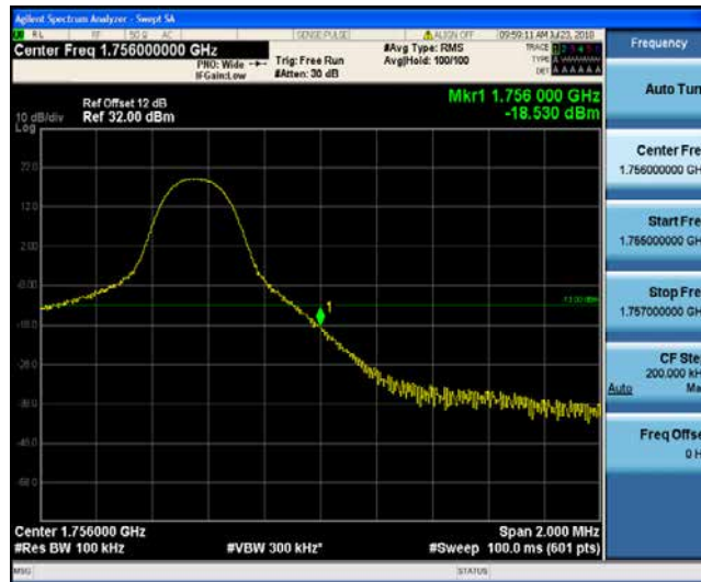
Band4_5MHz_QPSK_20385_1RB#24
