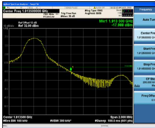
Band2_10MHz_QPSK_19185_1RB#49
