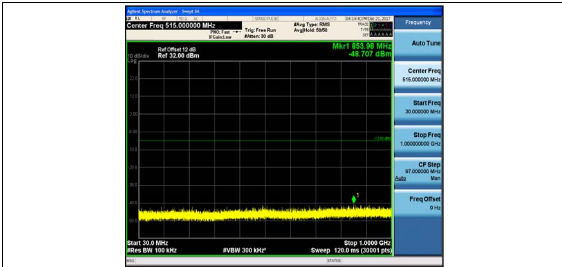
Band4_10MHz_QPSK_2000_1RB#0
