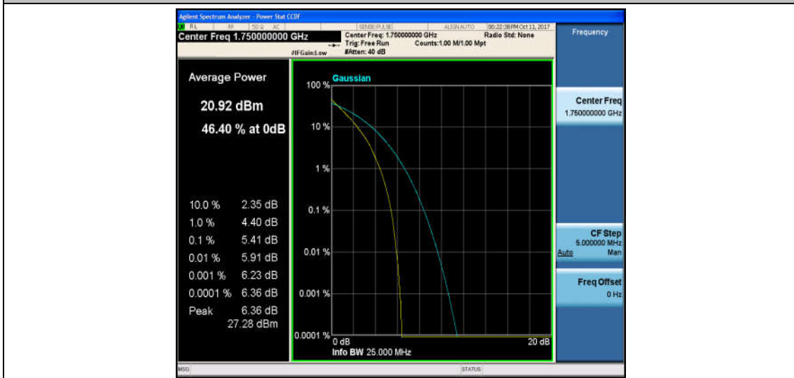
Band4_10MHz_16QAM_20350_50RB#0_6.20_13_PASS
