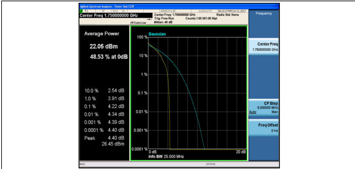
Band4_10MHz_16QAM_20350_1RB#0_5.26_13_PASS
