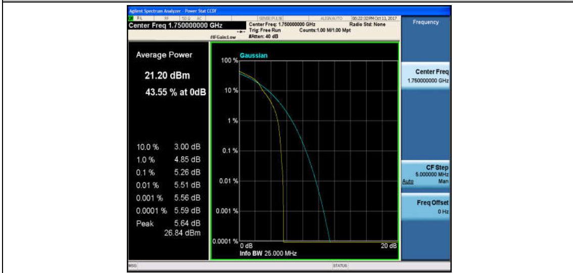
Band4_10MHz_QPSK_20350_50RB#0_5.41_13_PASS
