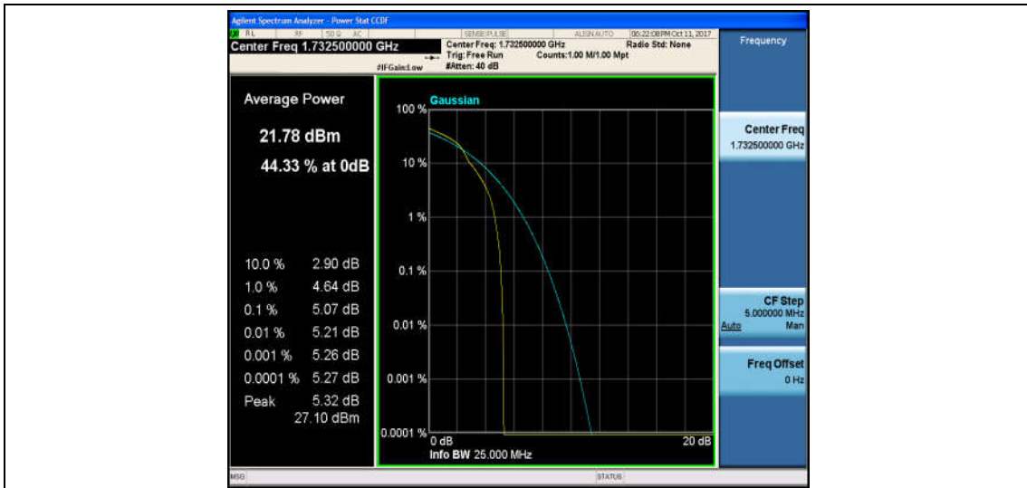
Band4_10MHz_QPSK_20175_50RB#0_5.44_13_PASS
