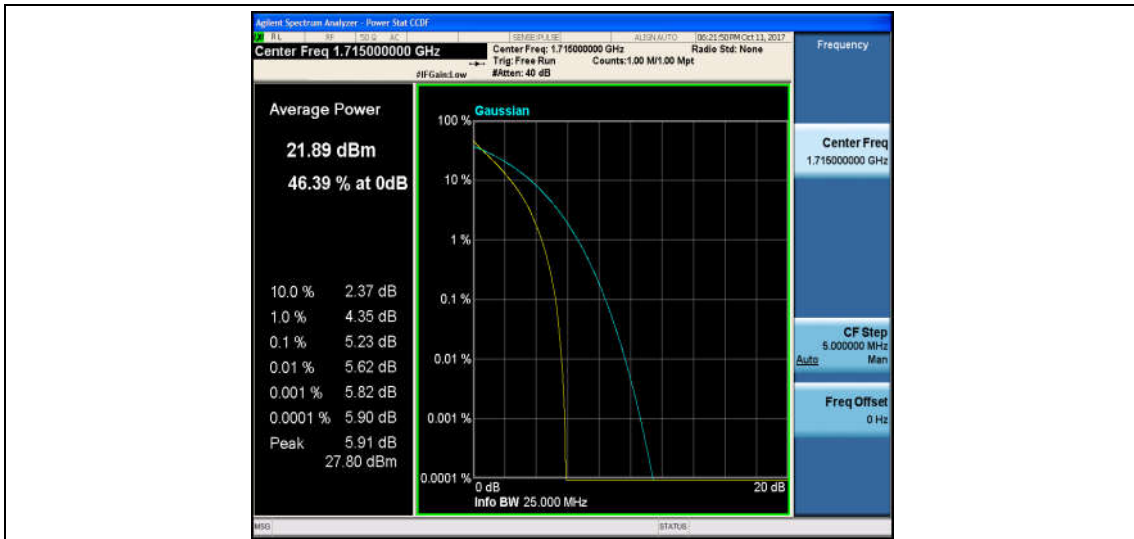
Band4_10MHz_16QAM_20000_50RB#0_6.04_13_PASS
