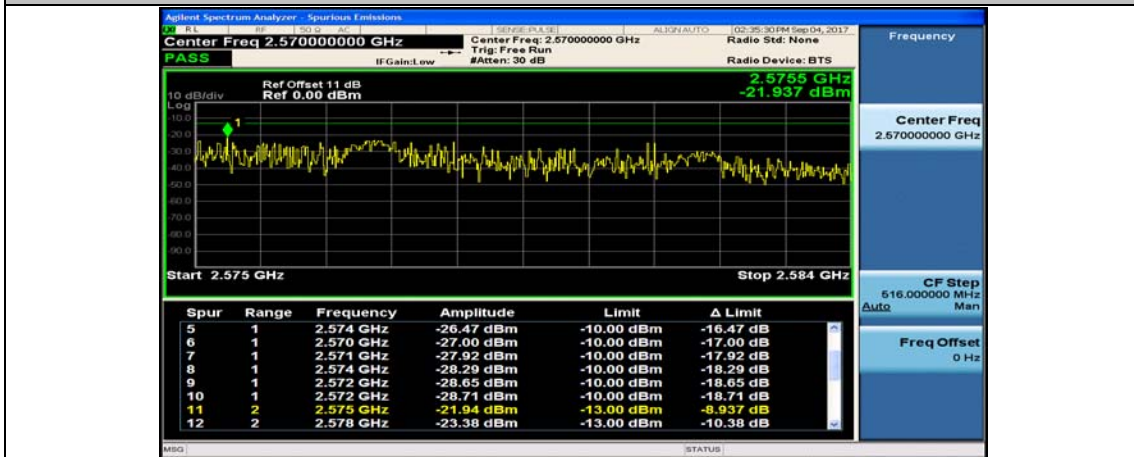
Band7_15MHz_16QAM_21375_75RB#0
