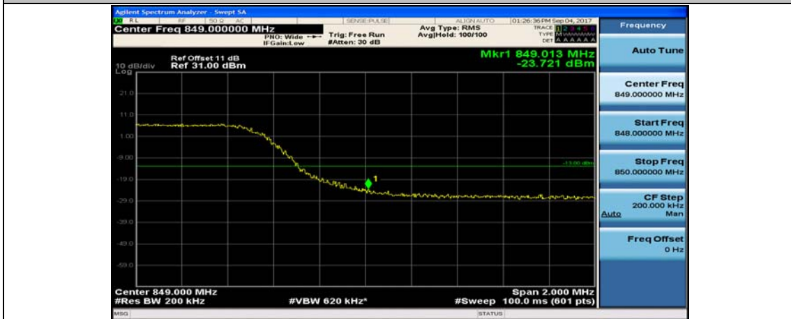
Band5_10MHz_16QAM_20600_50RB#0
