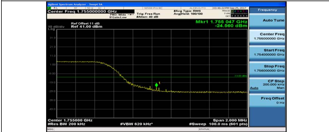
Band4_10MHz_16QAM_20350_50RB#0
