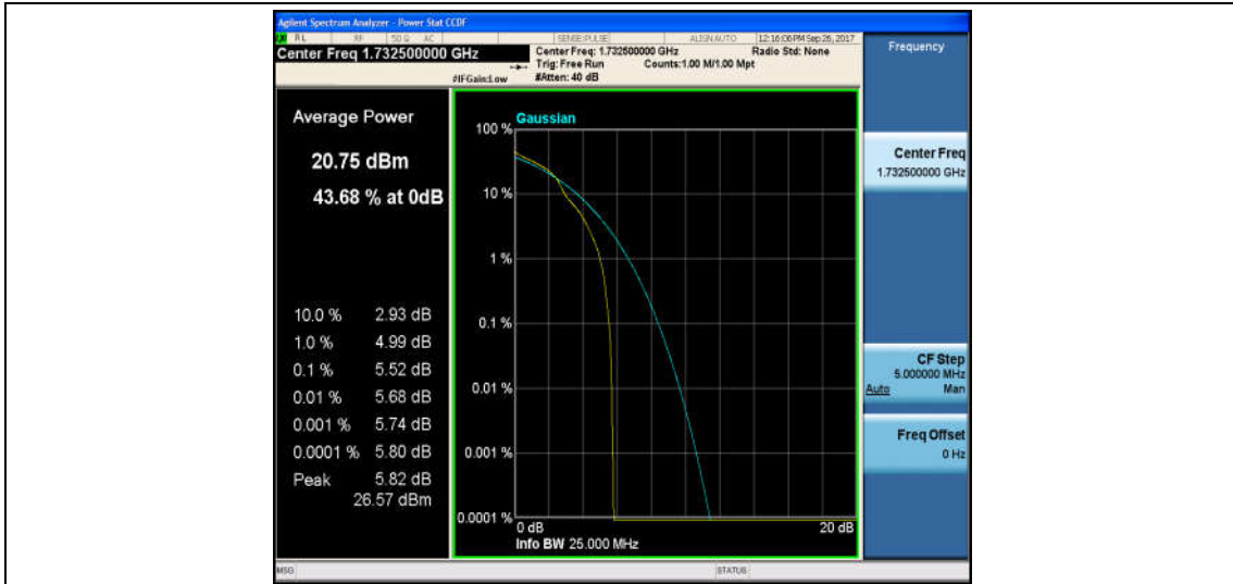
Band4_1.4MHz_QPSK_20175_6RB#0_5.26_13_PASS
