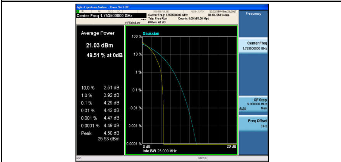
Band4_3MHz_16QAM_20385_1RB#0_5.09_13_PASS
