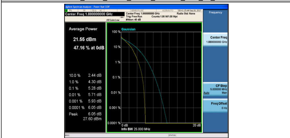
Band2_3MHz_16QAM_18900_15RB#0_6.19_13_PASS
