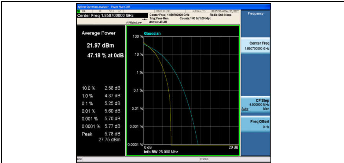
Band2_1.4MHz_16QAM_18607_6RB#0_6.12_13_PASS
