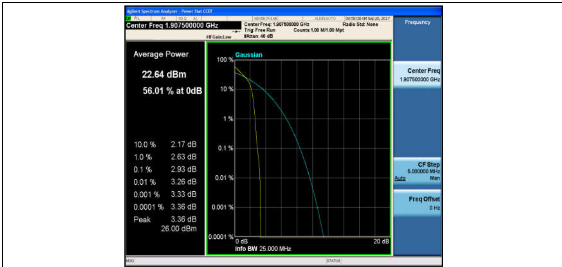
Band2_5MHz_16QAM_19175_1RB#0_3.84_13_PASS
