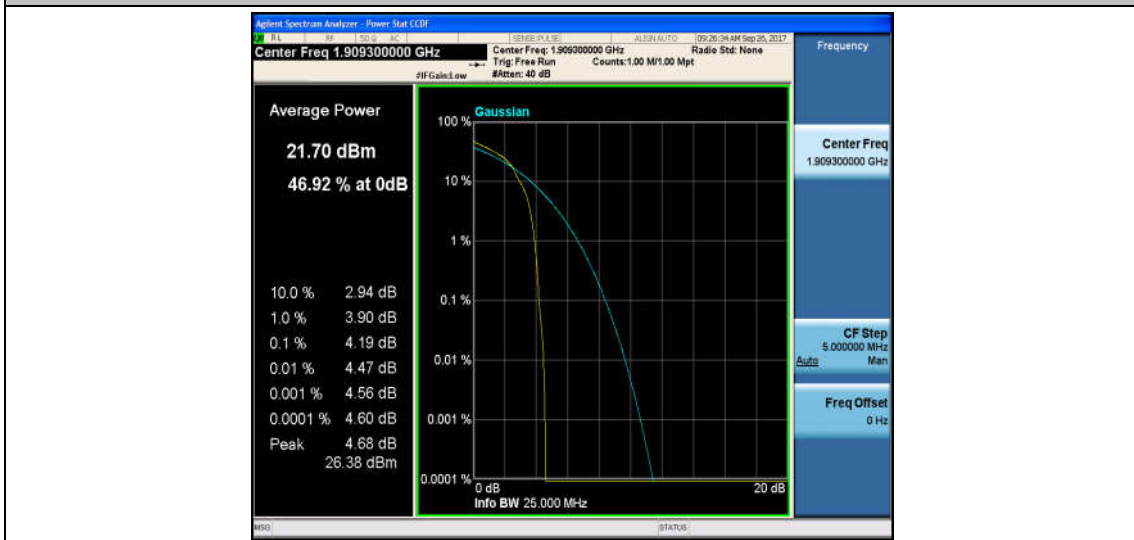
Band2_1.4MHz_QPSK_19193_6RB#0_4.60_13_PASS
