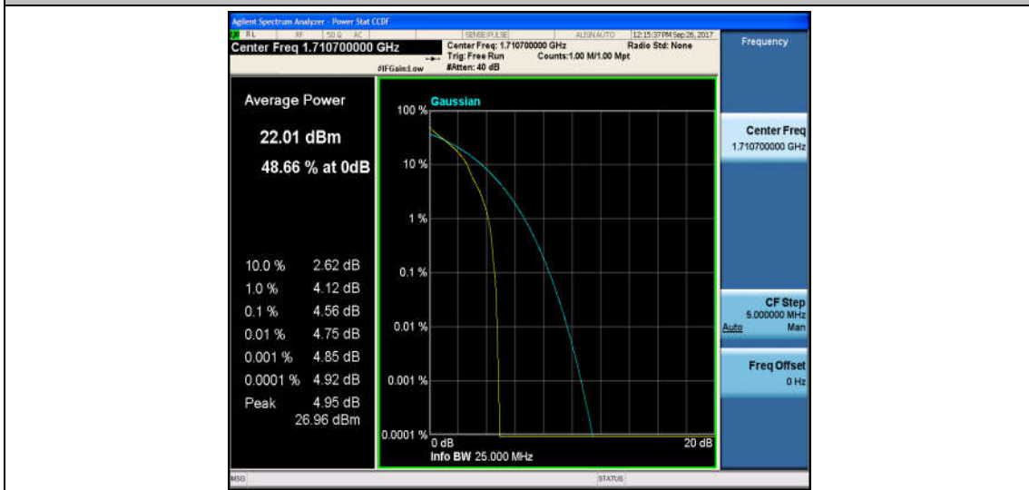
Band4_1.4MHz_16QAM_19957_1RB#0_5.51_13_PASS
