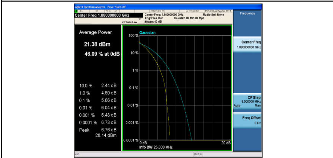
Band2_15MHz_16QAM_18900_75RB#0_6.22_13_PASS
