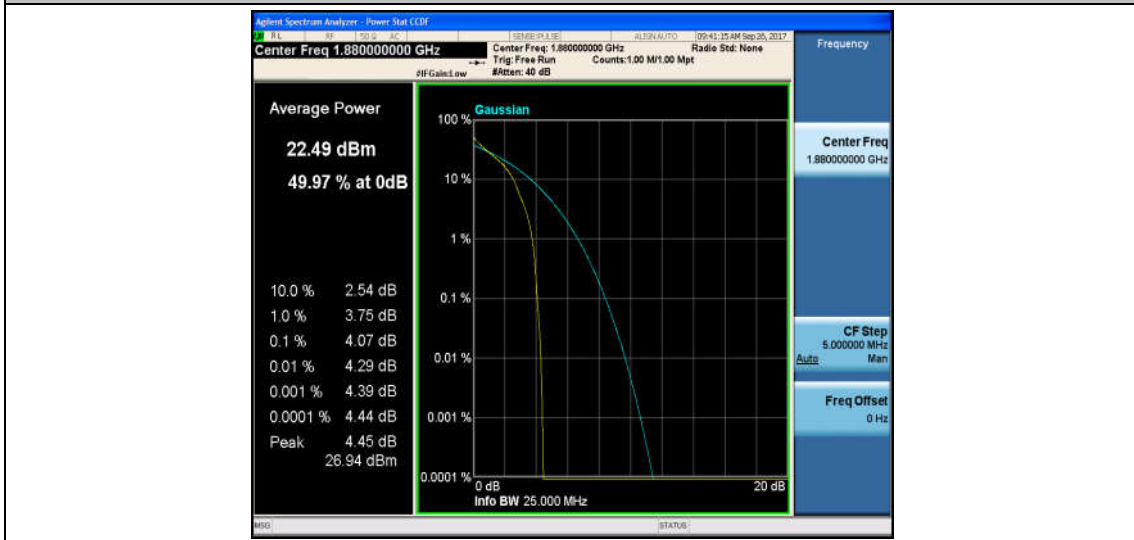
Band2_3MHz_16QAM_18900_1RB#0_4.99_13_PASS
