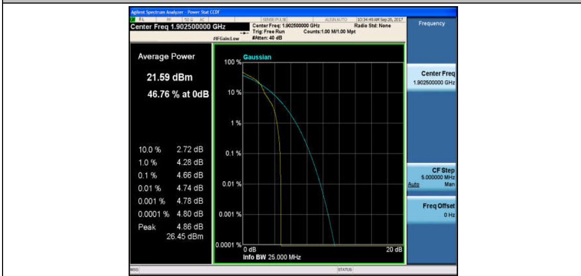
Band2_15MHz_QPSK_19125_75RB#0_4.92_13_PASS
