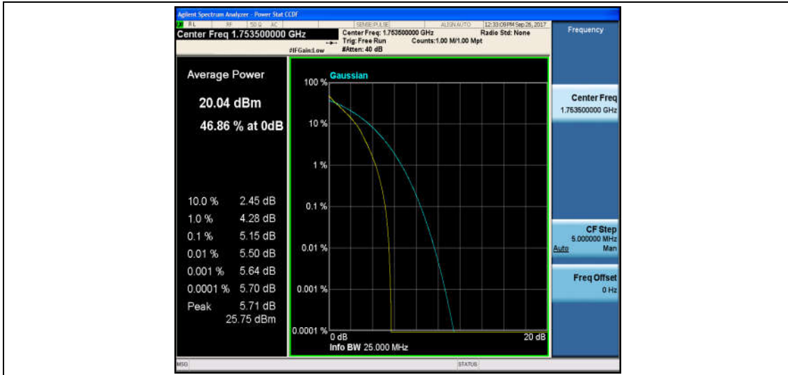
Band4_3MHz_16QAM_20385_15RB#0_5.97_13_PASS
