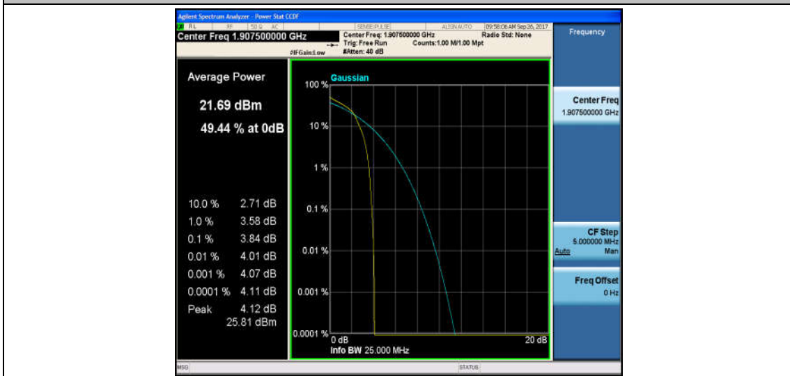
Band2_5MHz_QPSK_19175_25RB#0_4.48_13_PASS
