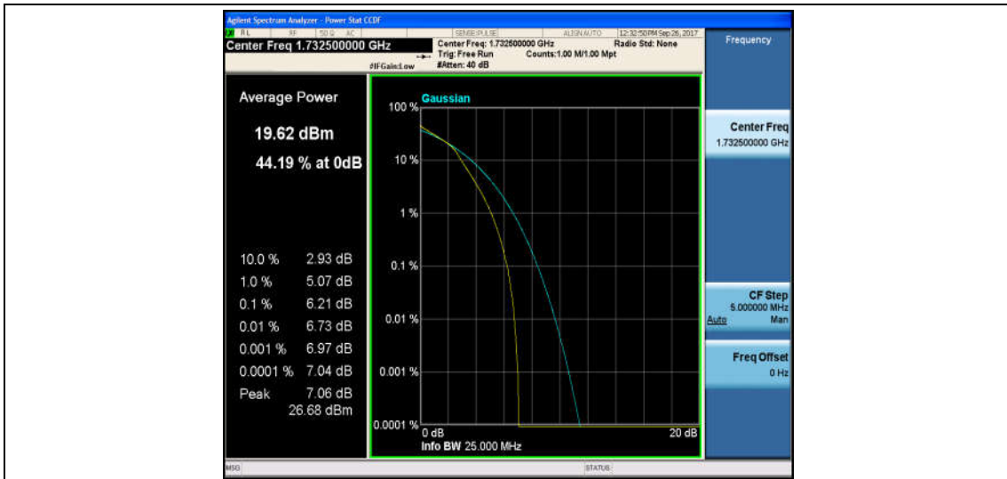
Band4_3MHz_QPSK_20175_1RB#0_4.50_13_PASS
