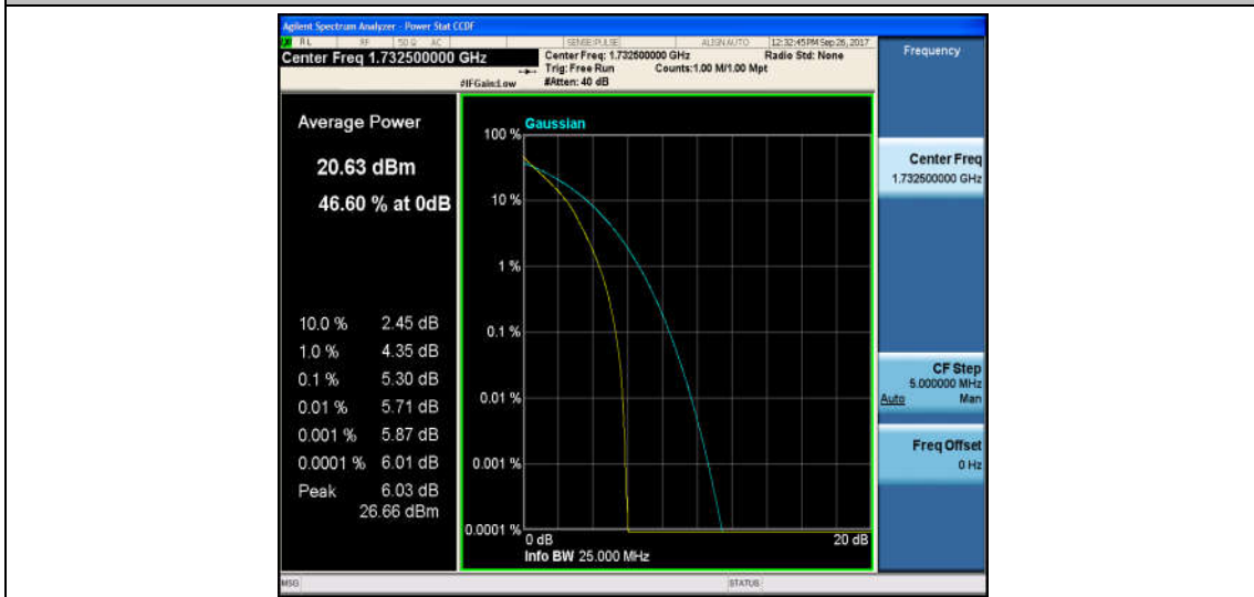
Band4_3MHz_16QAM_20175_15RB#0_6.21_13_PASS
