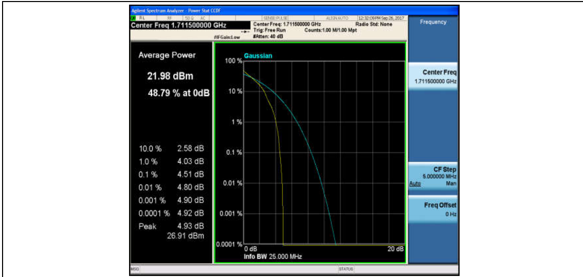
Band4_3MHz_16QAM_19965_1RB#0_5.53_13_PASS
