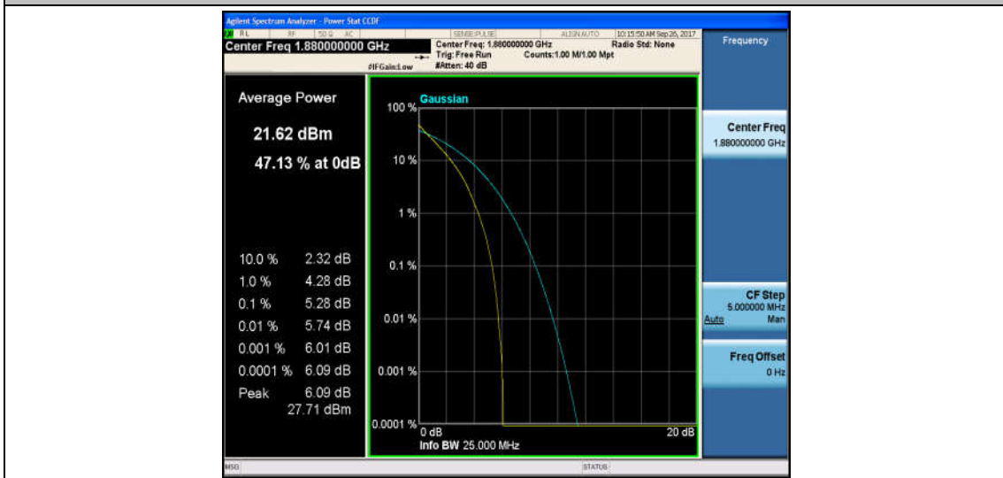
Band2_10MHz_16QAM_18900_50RB#0_6.01_13_PASS
