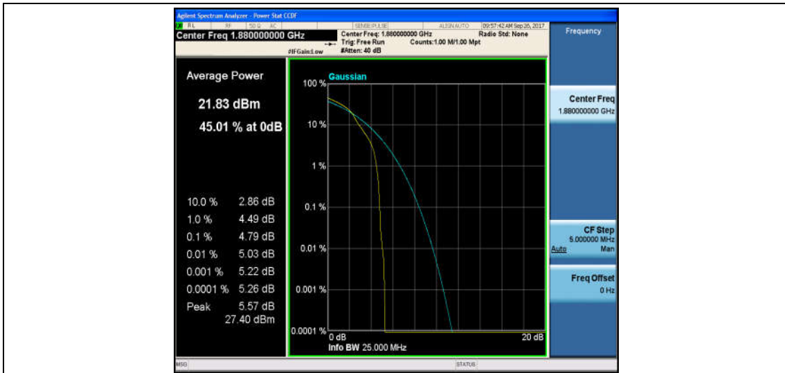
Band2_5MHz_QPSK_18900_25RB#0_5.35_13_PASS
