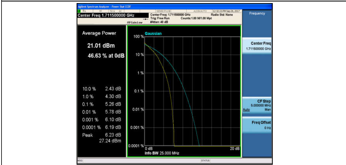
Band4_3MHz_16QAM_19965_15RB#0_6.12_13_PASS
