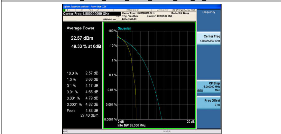
Band2_5MHz_16QAM_18900_1RB#0_4.79_13_PASS
