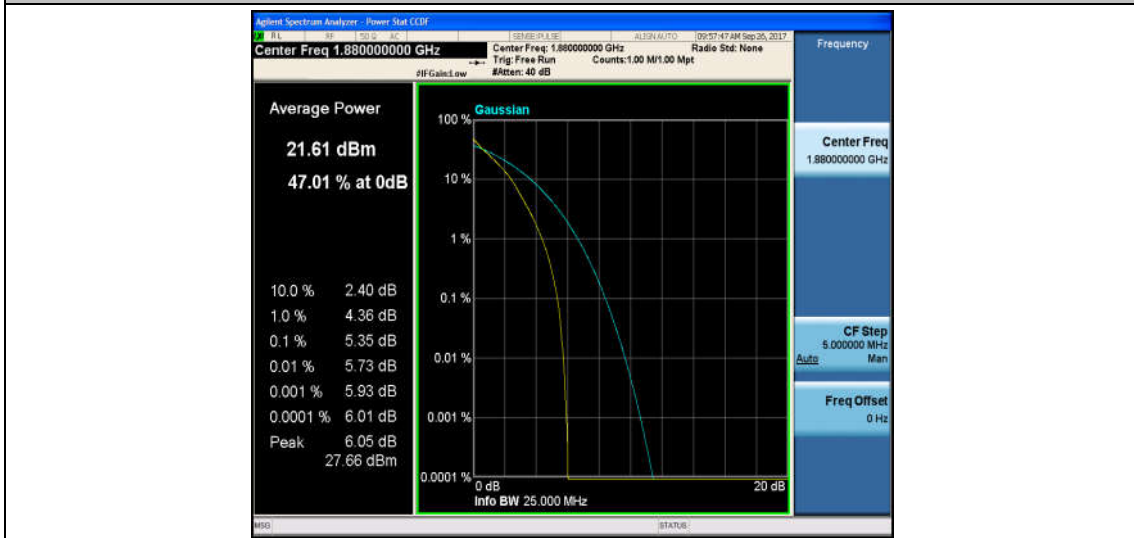
Band2_5MHz_16QAM_18900_25RB#0_6.02_13_PASS
