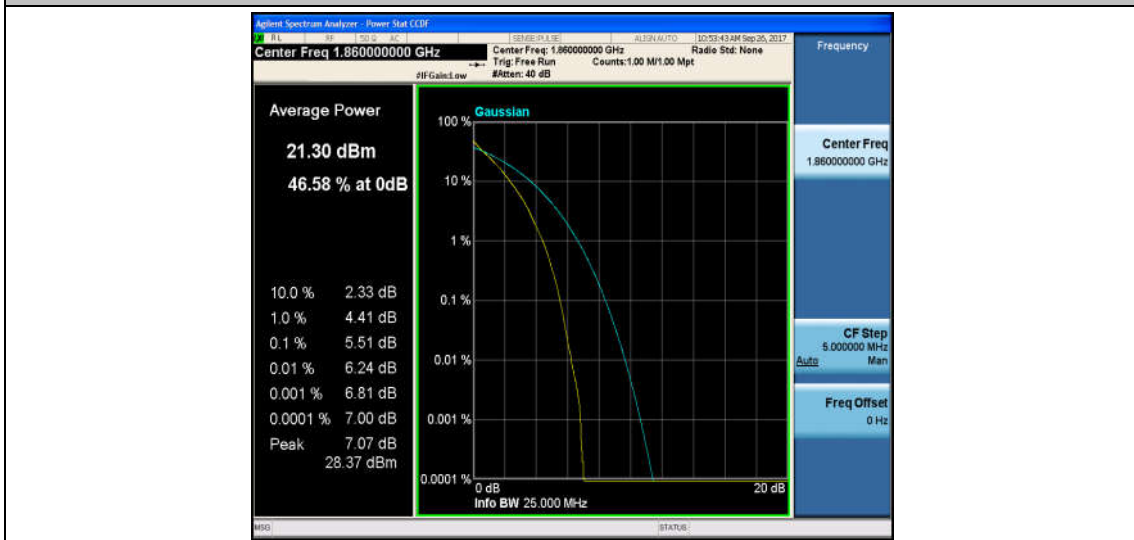
Band2_20MHz_16QAM_18700_100RB#0_6.27_13_PASS
