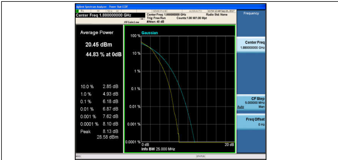
Band2_20MHz_QPSK_18900_1RB#0_4.18_13_PASS
