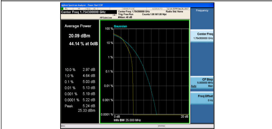
Band4_1.4MHz_QPSK_20393_6RB#0_5.02_13_PASS
