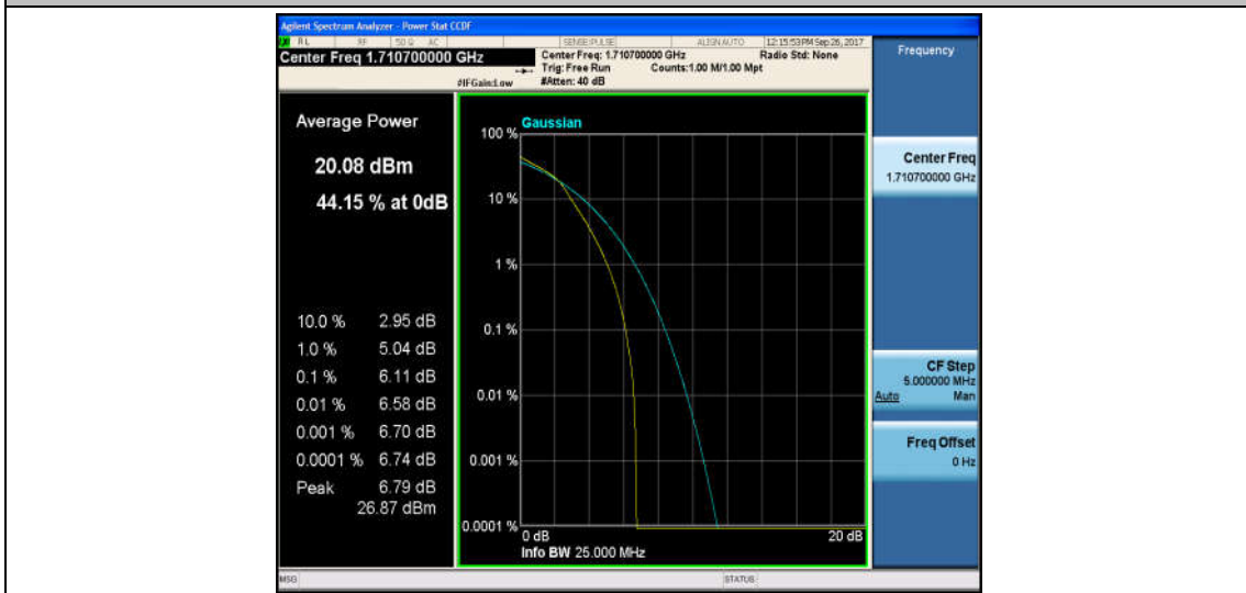
Band4_1.4MHz_QPSK_20175_1RB#0_4.54_13_PASS
