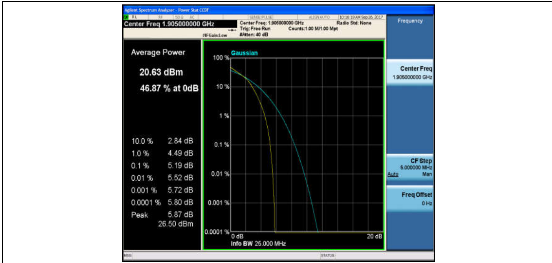
Band2_15MHz_QPSK_18675_1RB#0_4.39_13_PASS
