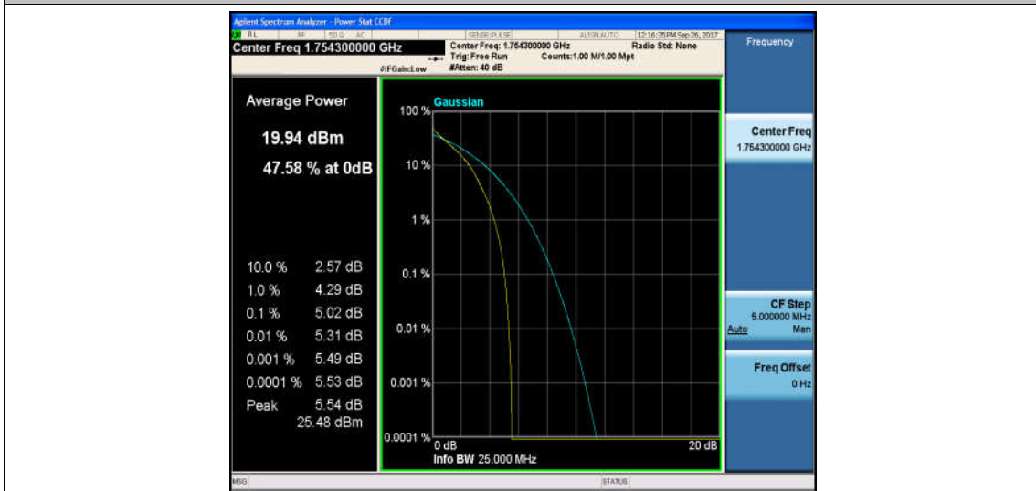
Band4_1.4MHz_16QAM_20393_6RB#0_5.93_13_PASS
