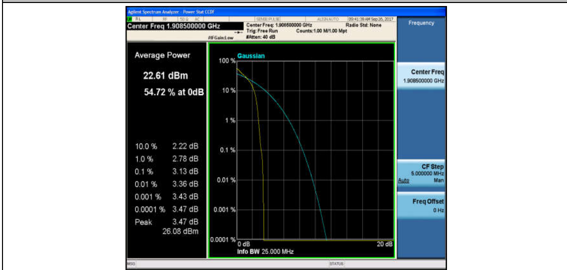
Band2_3MHz_16QAM_19185_1RB#0_4.04_13_PASS
