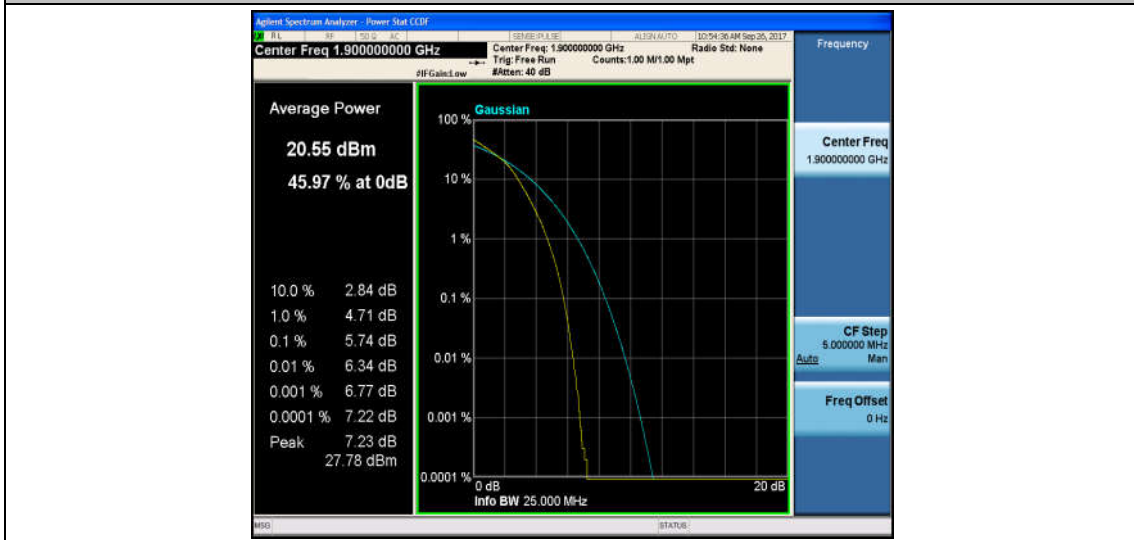
Band2_20MHz_QPSK_19100_1RB#0_4.21_13_PASS
