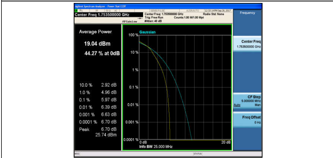
Band4_3MHz_QPSK_20385_1RB#0_4.29_13_PASS
