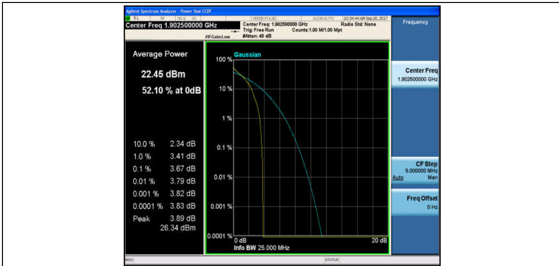
Band2_15MHz_16QAM_19125_1RB#0_4.66_13_PASS
