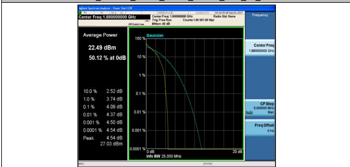
Band2_1.4MHz_16QAM_18900_1RB#0_4.99_13_PASS
