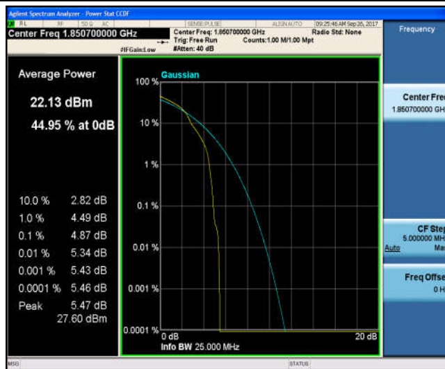
Band2_1.4MHz_QPSK_18607_6RB#0_5.25_13_PASS
