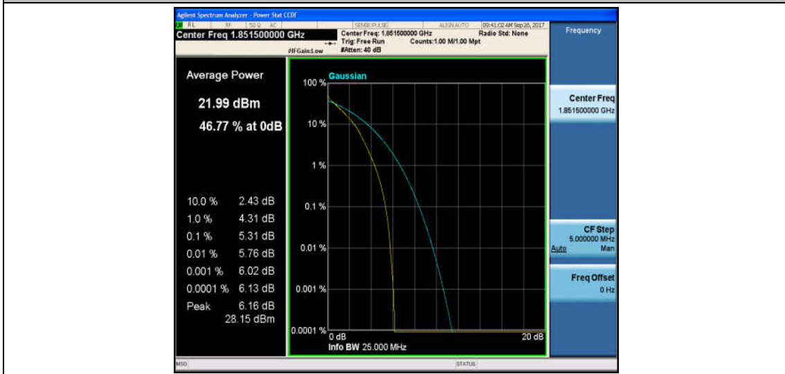
Band2_3MHz_16QAM_18615_15RB#0_6.16_13_PASS
