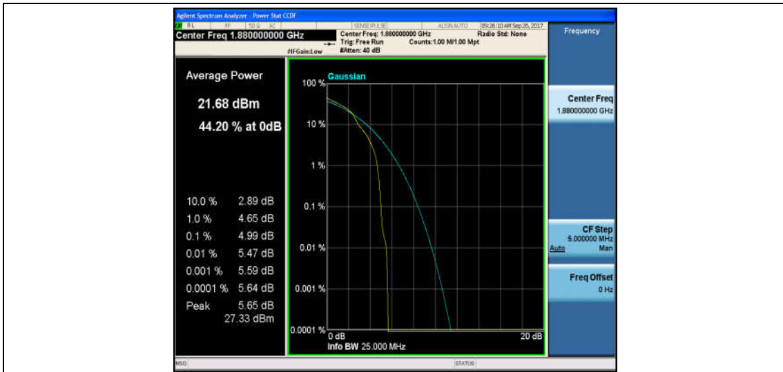
Band2_1.4MHz_QPSK_18900_6RB#0_5.23_13_PASS
