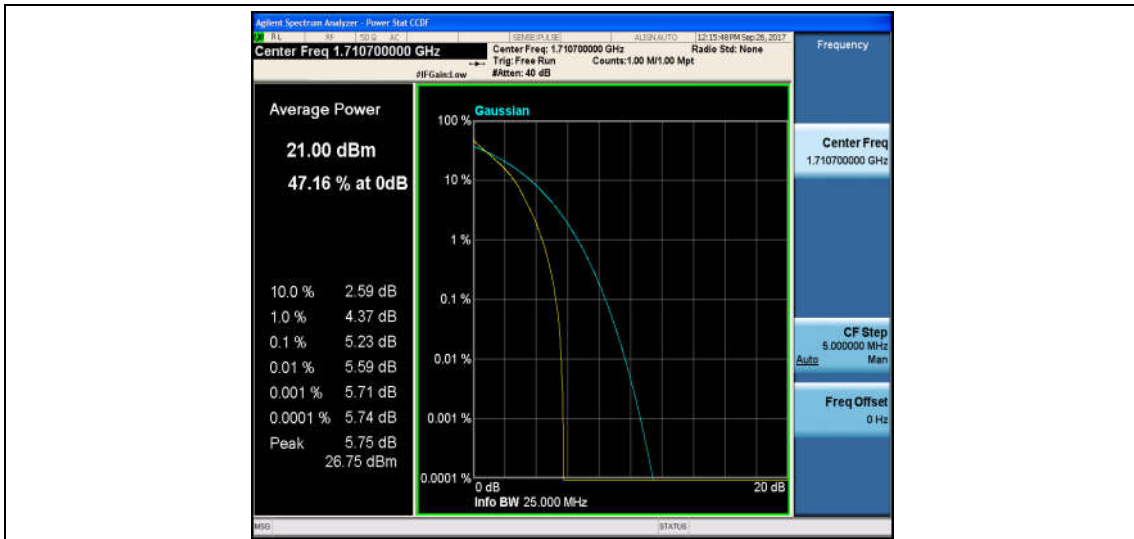
Band4_1.4MHz_16QAM_19957_6RB#0_6.11_13_PASS
