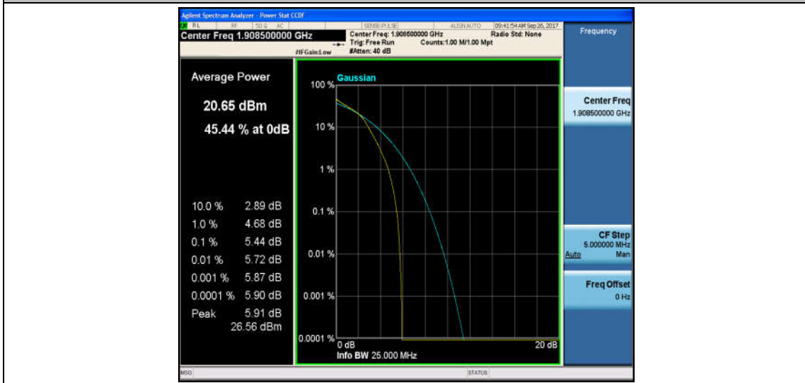
Band2_3MHz_QPSK_19185_1RB#0_3.13_13_PASS
