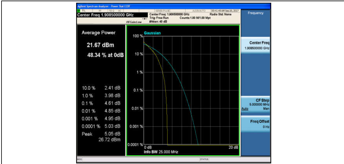
Band2_3MHz_16QAM_19185_15RB#0_5.44_13_PASS
