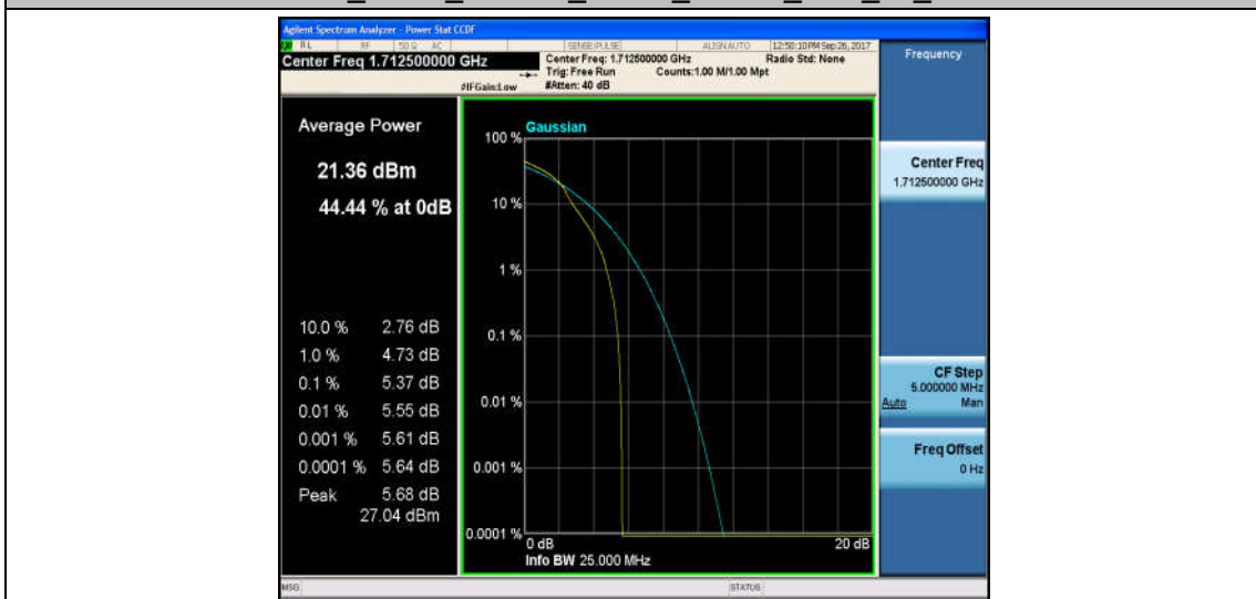
Band4_5MHz_QPSK_19975_25RB#0_5.46_13_PASS
