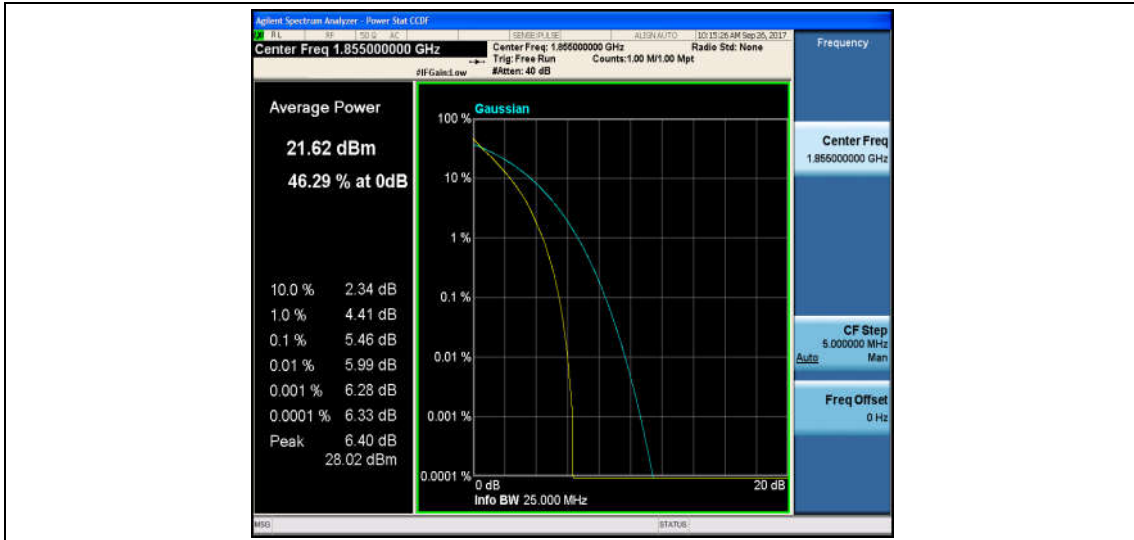
Band2_10MHz_16QAM_18650_50RB#0_6.24_13_PASS
