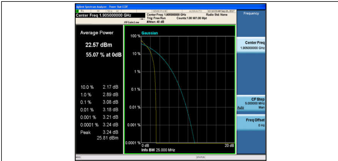
Band2_10MHz_16QAM_19150_1RB#0_4.03_13_PASS
