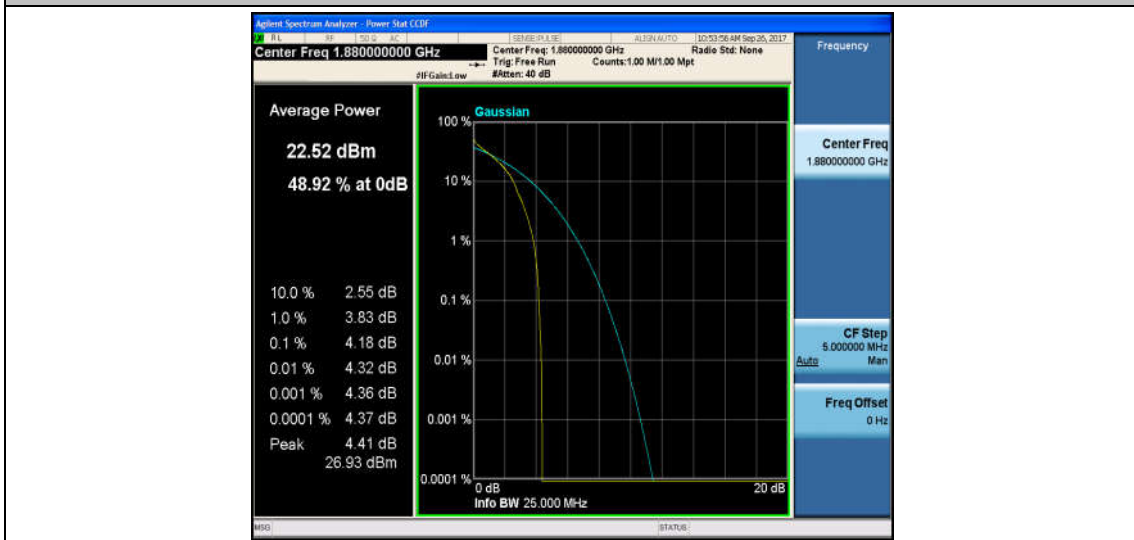
Band2_20MHz_16QAM_18900_1RB#0_4.93_13_PASS
