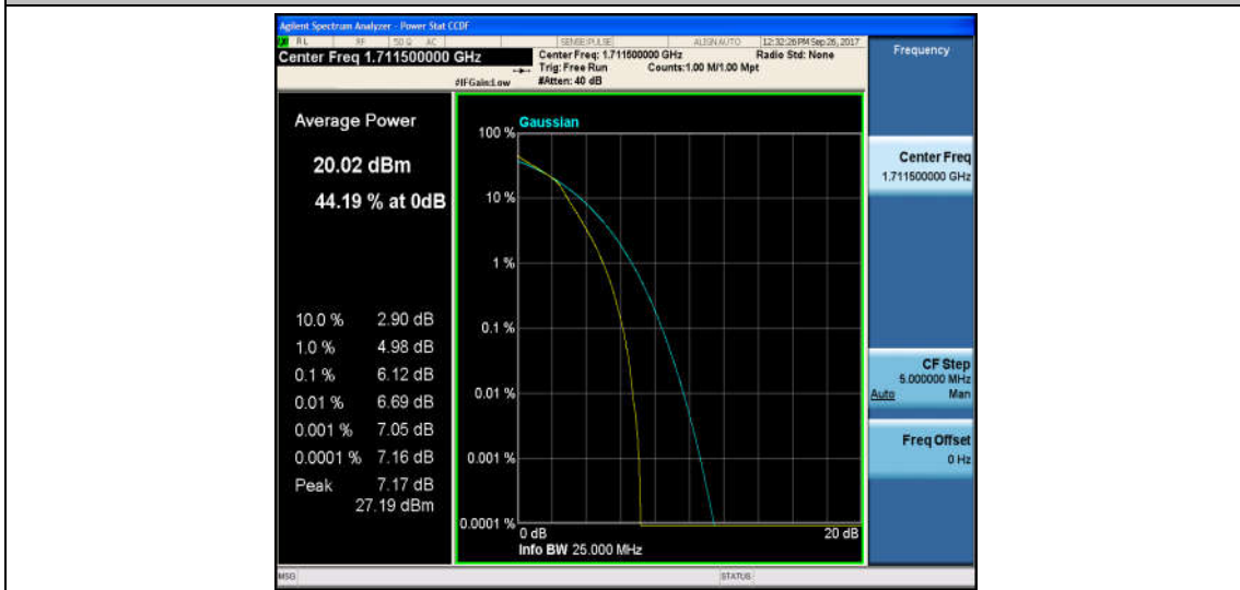
Band4_3MHz_QPSK_19965_1RB#0_4.51_13_PASS
