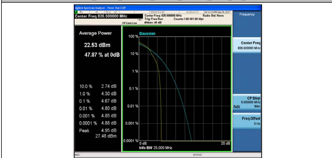
Band5_5MHz_QPSK_20425_25RB#0_4.73_13_PASS
