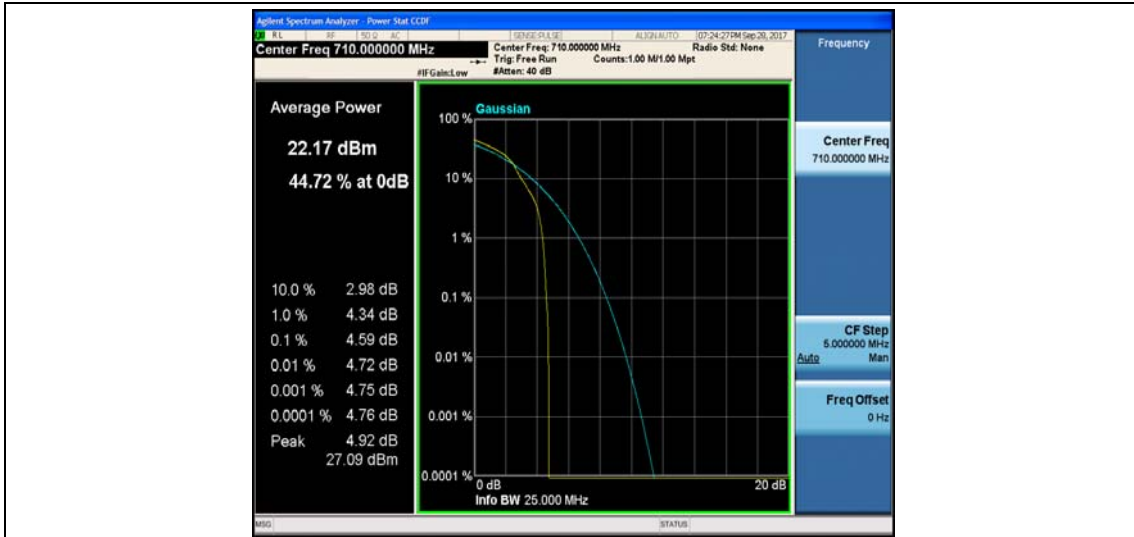
Band17_5MHz_QPSK_23790_25RB#0_4.68_13_PASS
