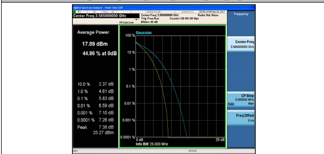
Band7_10MHz_16QAM_21400_50RB#0_6.60_13_PASS
