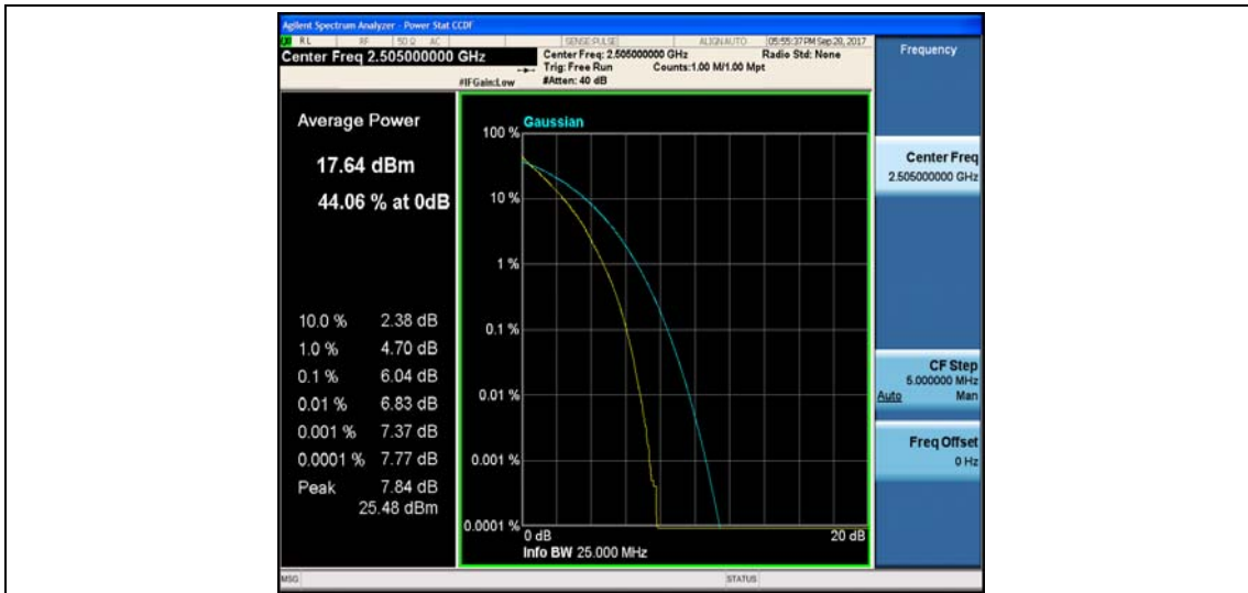
Band7_10MHz_16QAM_20800_50RB#0_6.77_13_PASS
