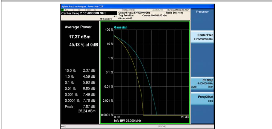
Band7_20MHz_16QAM_21100_100RB#0_6.66_13_PASS
