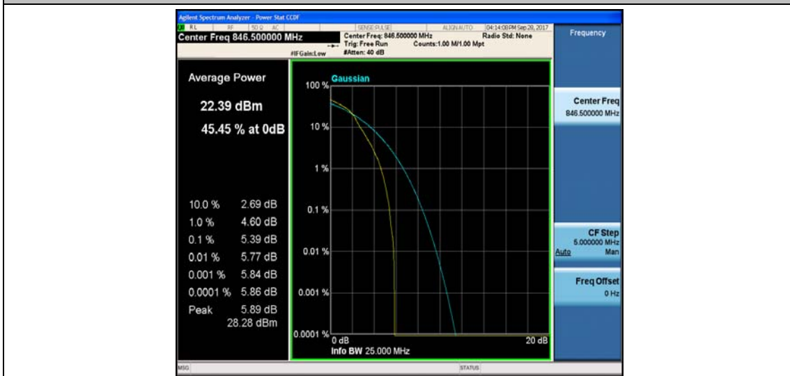
Band5_5MHz_QPSK_20625_25RB#0_5.08_13_PASS
