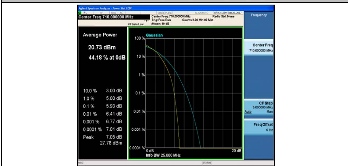
Band17_10MHz_QPSK_23800_1RB#0_4.12_13_PASS
