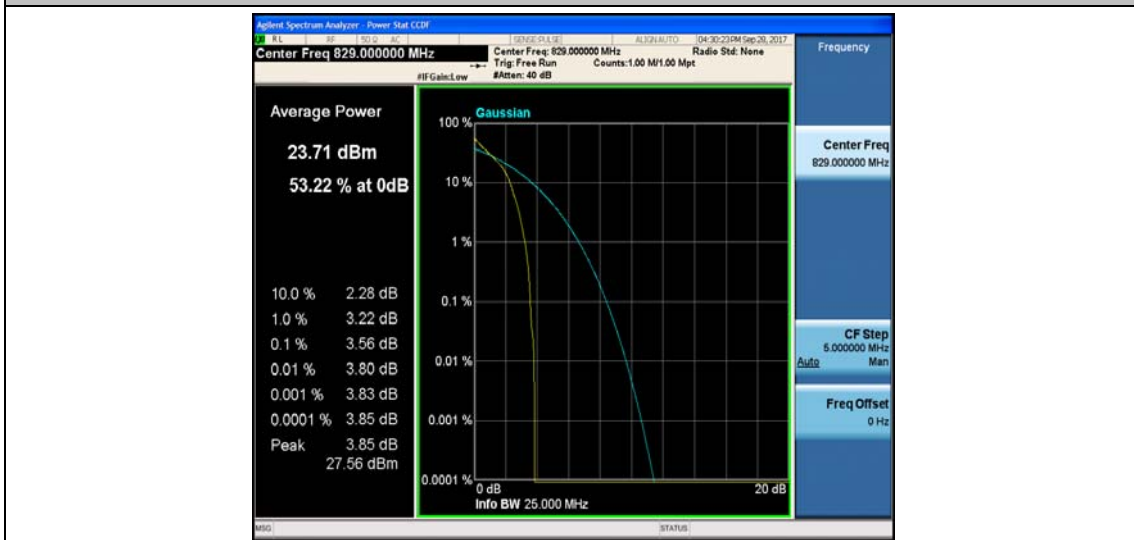
Band5_10MHz_16QAM_20450_1RB#0_4.42_13_PASS
