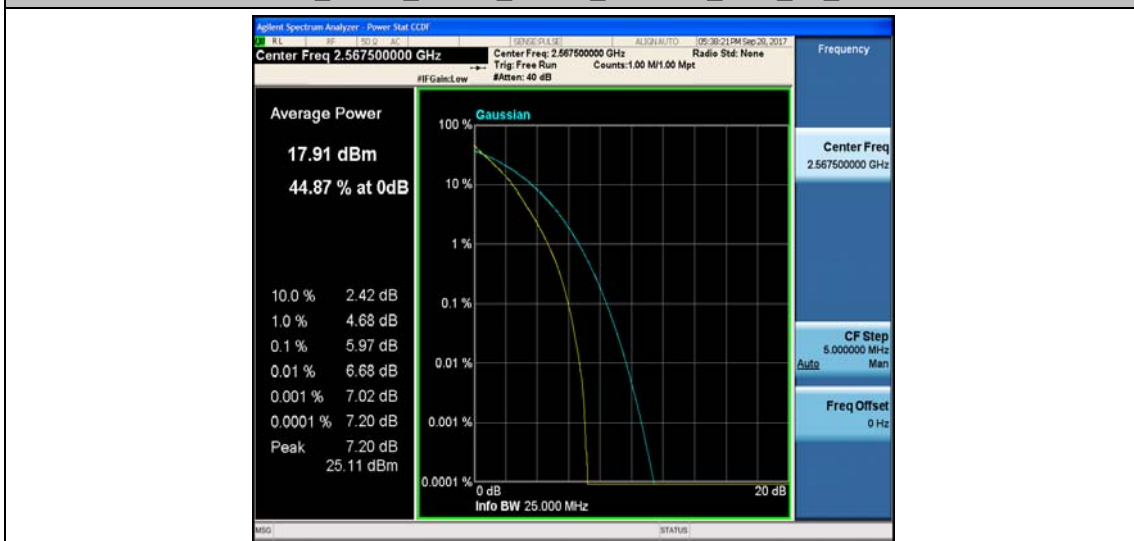
Band7_5MHz_16QAM_21425_25RB#0_6.61_13_PASS
