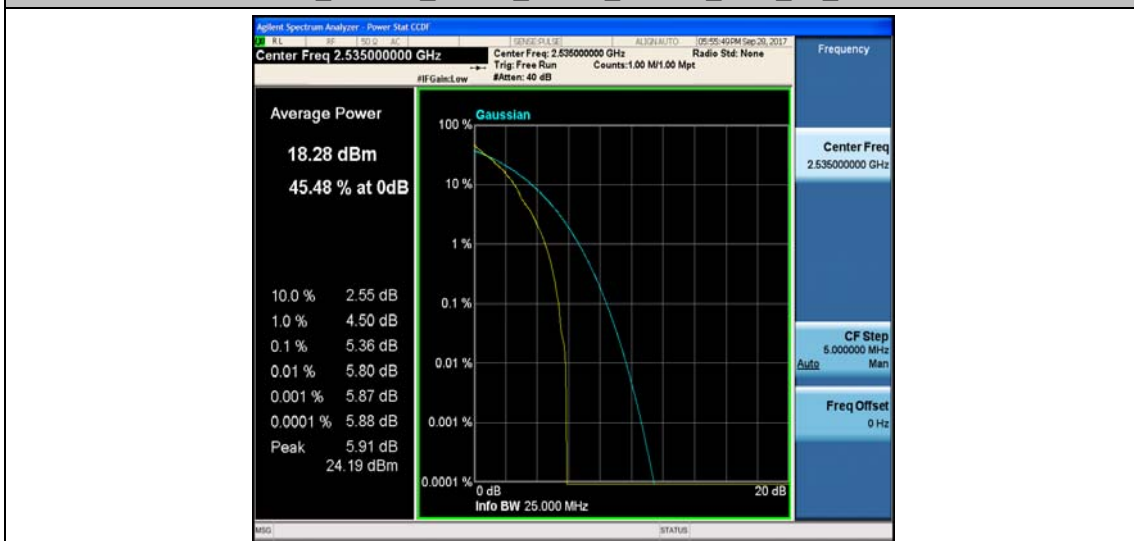
Band7_10MHz_16QAM_21100_1RB#0_6.34_13_PASS
