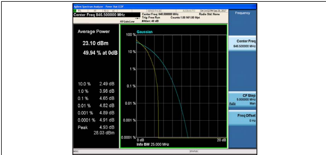
Band5_5MHz_16QAM_20625_1RB#0_5.39_13_PASS
