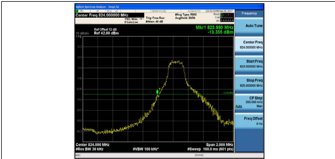
Band5_3MHz_QPSK_20635_15RB#0_-26.23_PASS
