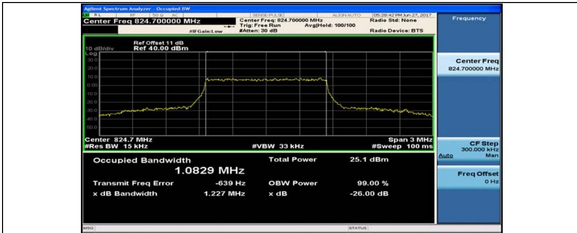
Band5_1.4MHz_16QAM_20407_6RB#0
