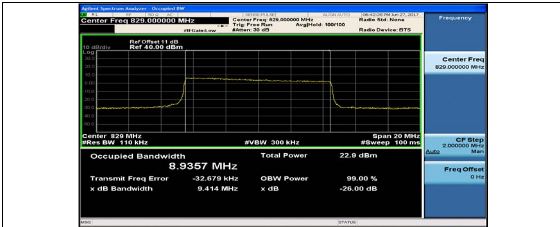
Band5_10MHz_16QAM_20450_50RB#0
