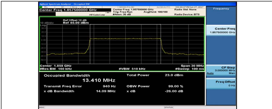
Band2_15MHz_16QAM_18675_75RB#0
