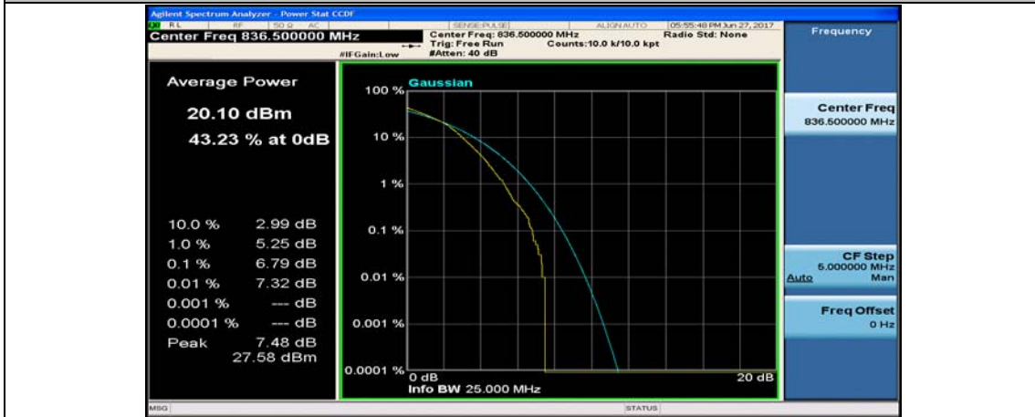
Band5_10MHz_QPSK_20525_50RB#0
