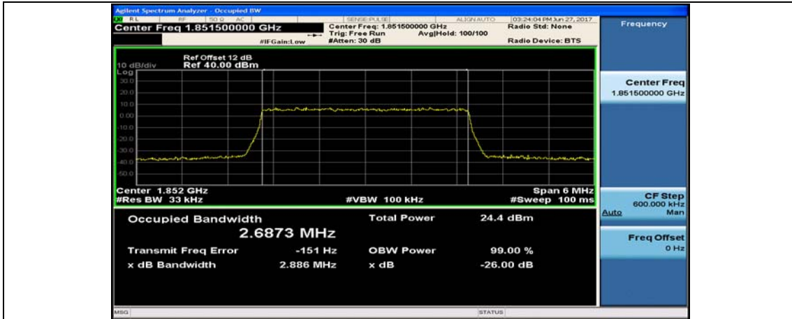
Band2_3MHz_16QAM_18615_15RB#0
