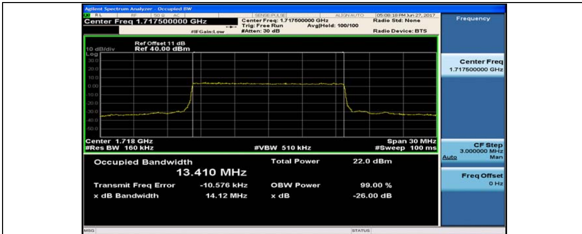
Band4_15MHz_16QAM_2025_75RB#0
