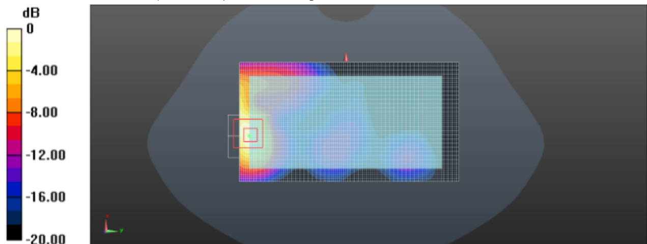
Body- worn Rear Side (LTE Band VII Middle Channel)
