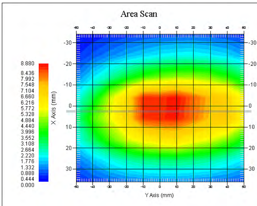
750 MHz System Validation with Body Tissue
