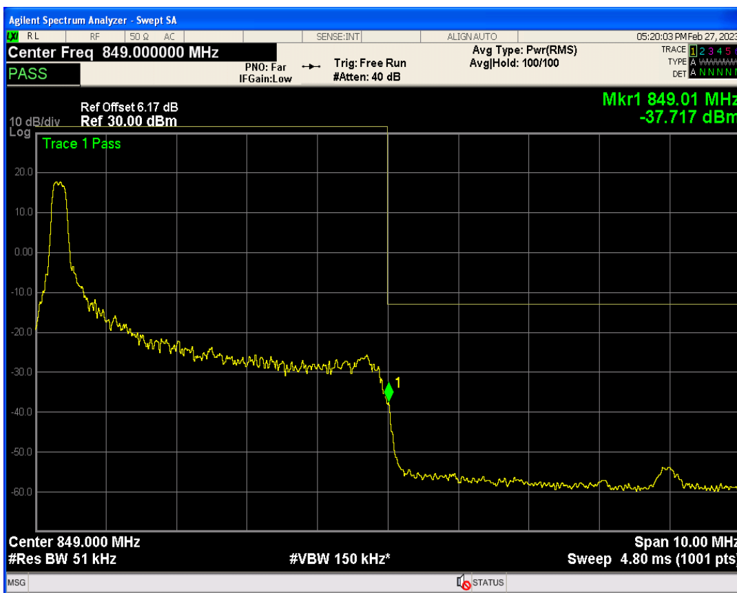
Band26b QAM16 BW=5MHz Channel=27015 RB Size=1 Position=#Max
