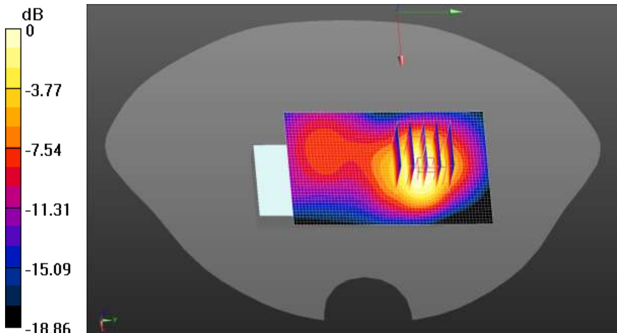
0 dB = 1.84 W/kg = 2.65 dBW/kg
