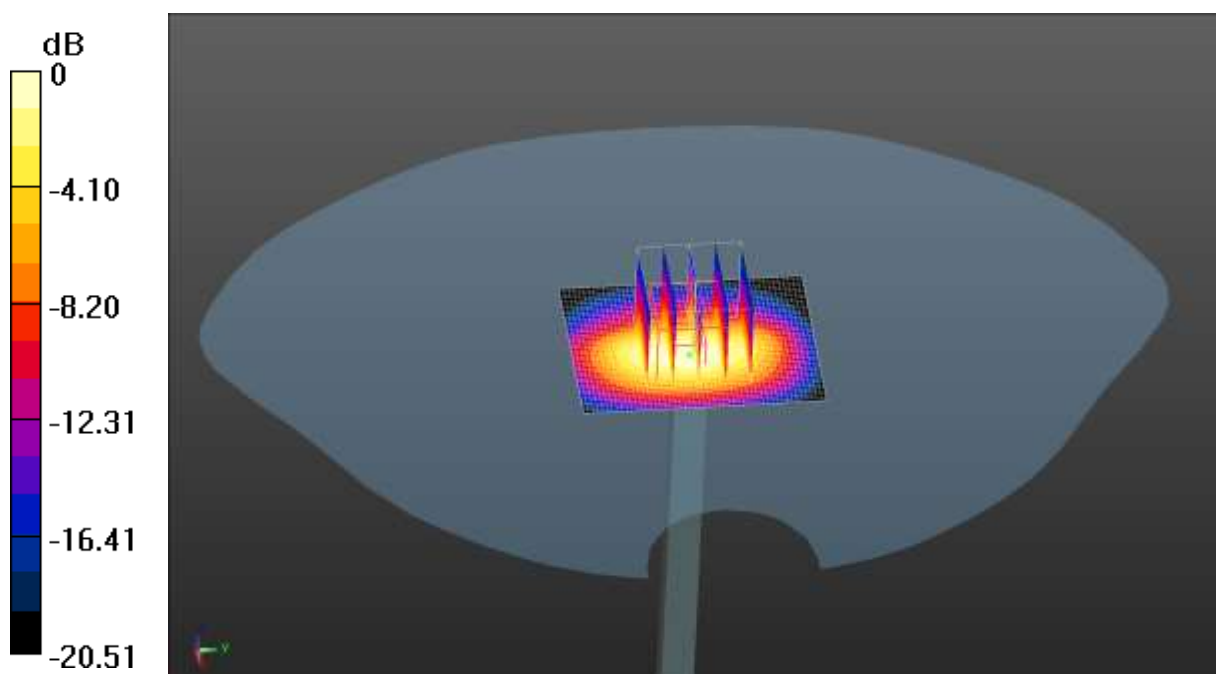
0 dB = 2.29 W/kg = 4.00 dBW/kg
