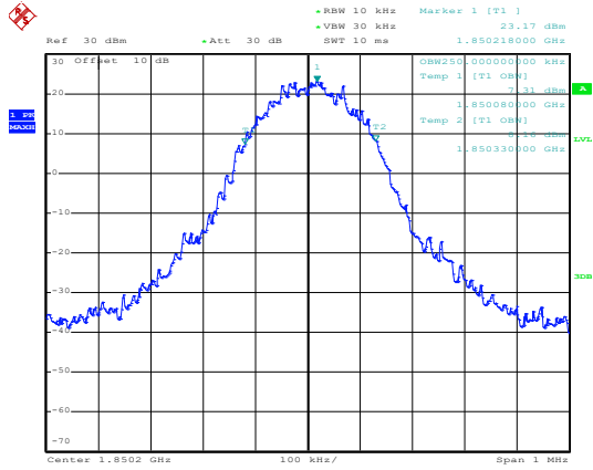
99% Occupancy bandwidth
