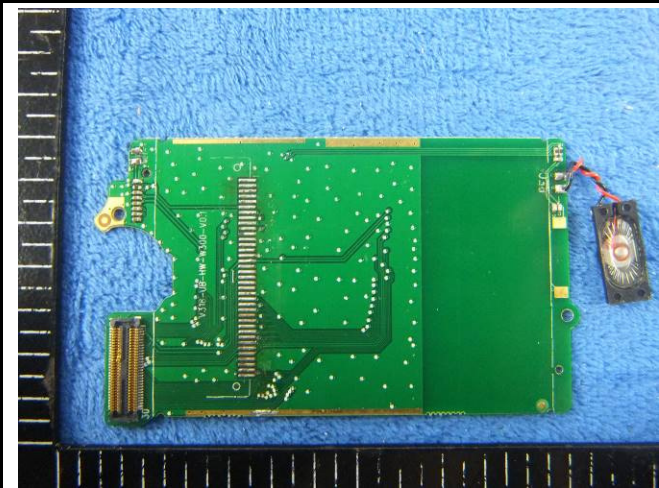
Connecting plate - Rear View
