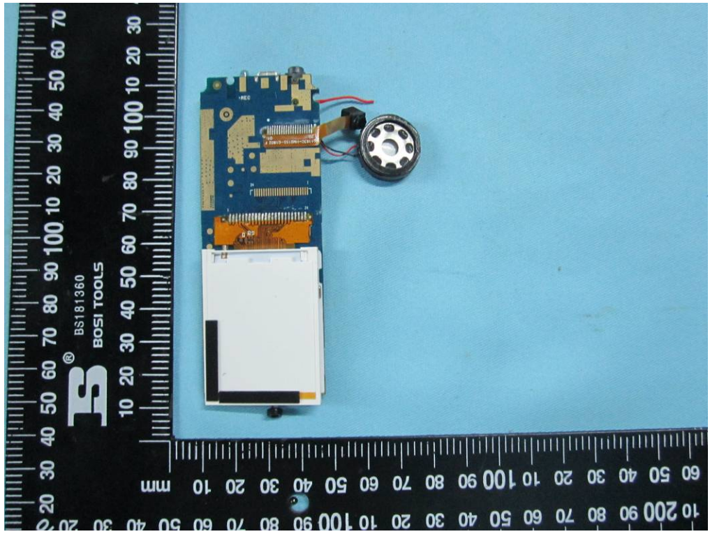
Mainborad Without Shielding– Rear View
