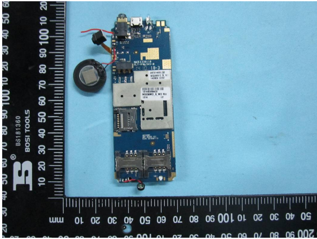
Mainboard With Shielding - Front View
