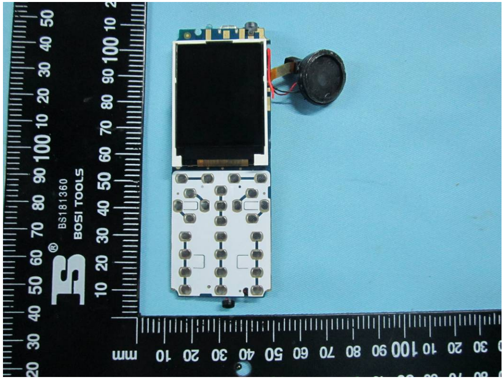
Mainborad With Shielding– Rear View
